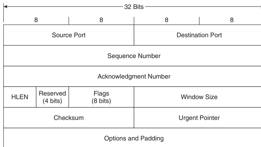
Example 1-14 Analyzer display of a TCP header.
