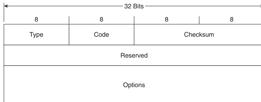
Figure 2-10 The Router Solicitation message format.
