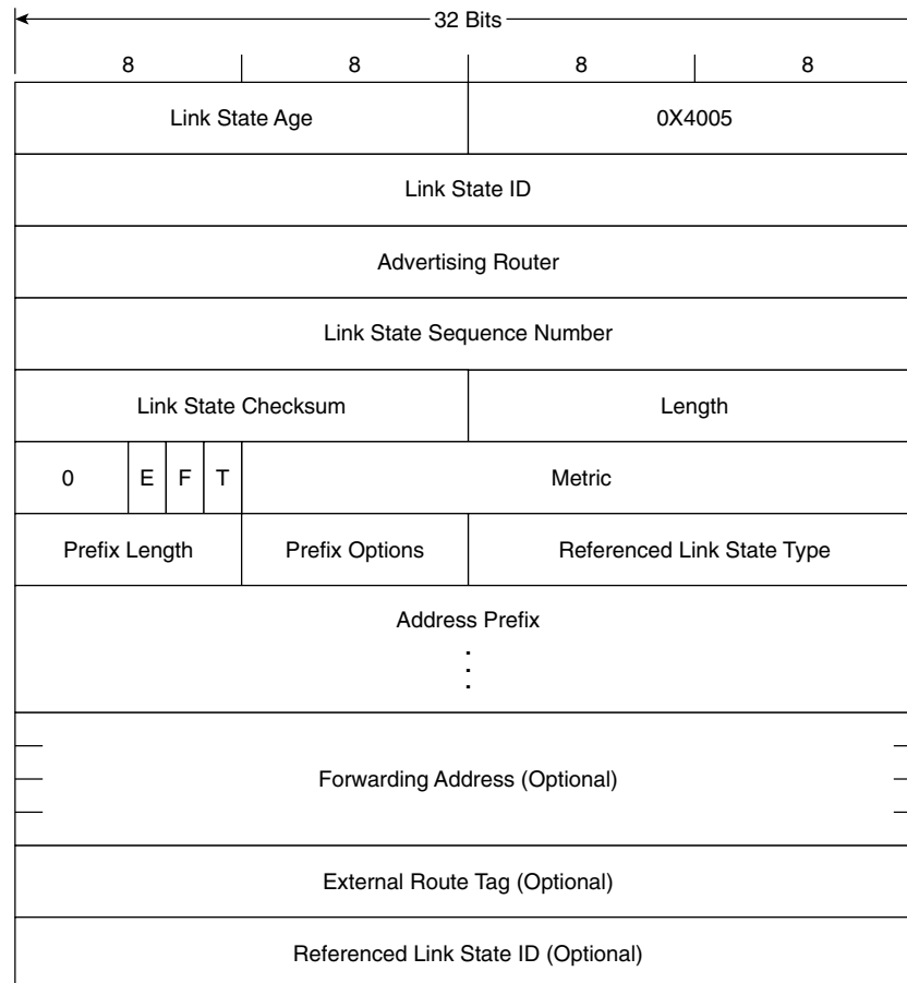
Figure 9-10 OSPFv3 AS-External LSA.
