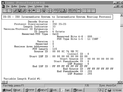
Figure 10-30 This analyzer capture shows the header of an L1 CSNP.
