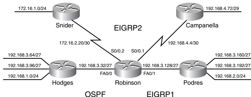
Figure 11-9 Hodges is running OSPF, and Podres is running EIGRP 1. Snider and Campanella are running EIGRP 2.
