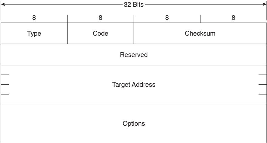
Figure 2-11 The Neighbor Solicitation message format.
