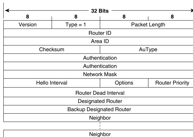
Figure 8-31 The OSPF Hello packet.
