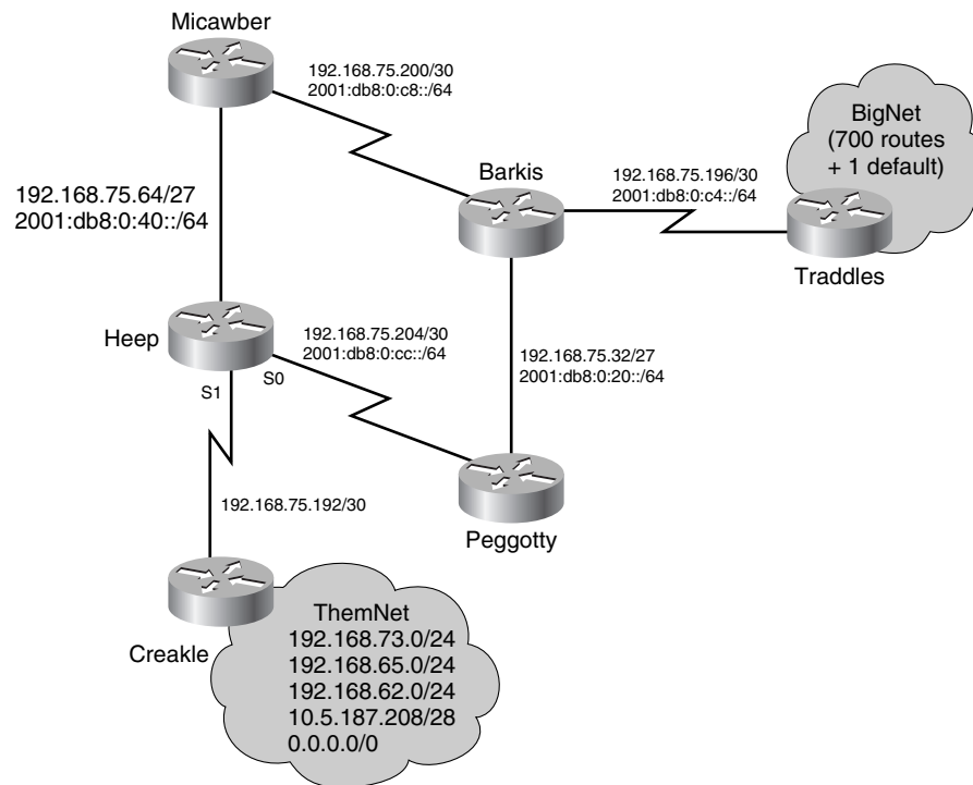
Figure 13-3 The network ThemNet is not under the control of the BigNet administrator.
