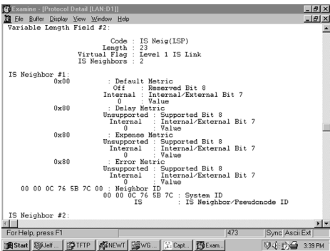
Figure 10-25 Part of an IS Neighbors TLV in an LSP.
