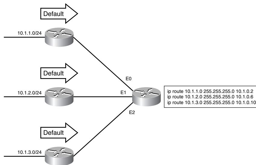
Figure 12-1 Default routes greatly simplify the administration of static routing in a hub-and-spoke network.
