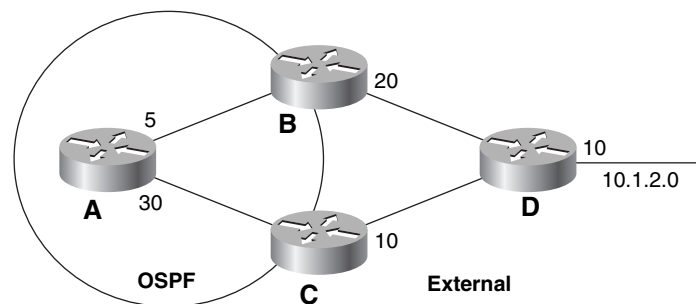
Figure 8-27 If the route to external network 10.1.2.0 is advertised with an E1 metric, router A will choose B as the “closest” ASBR. If the destination is advertised with an E2 metric, C will be chosen as the ASBR.
