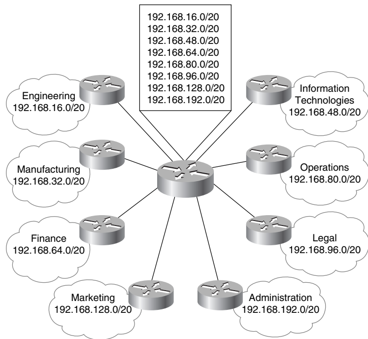
Figure 7-30 Although there are 128 major network addresses and possibly more than 32,000 hosts in this network, the backbone router has only eight aggregate addresses in its route table.
