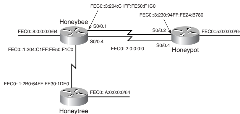
Figure 3-6 Backup link added between two IPv6 routers can be used to recover from a primary link failure with floating static routes.
