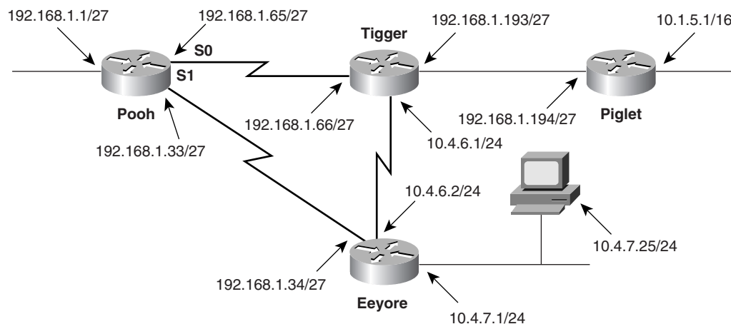
Figure 3-4 A more direct path from Pooh to the 10.4.0.0 subnets is added to the network.
