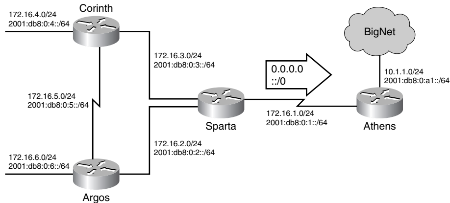
Example 12-10 The default-network command can be used by RIP to create a default route.
