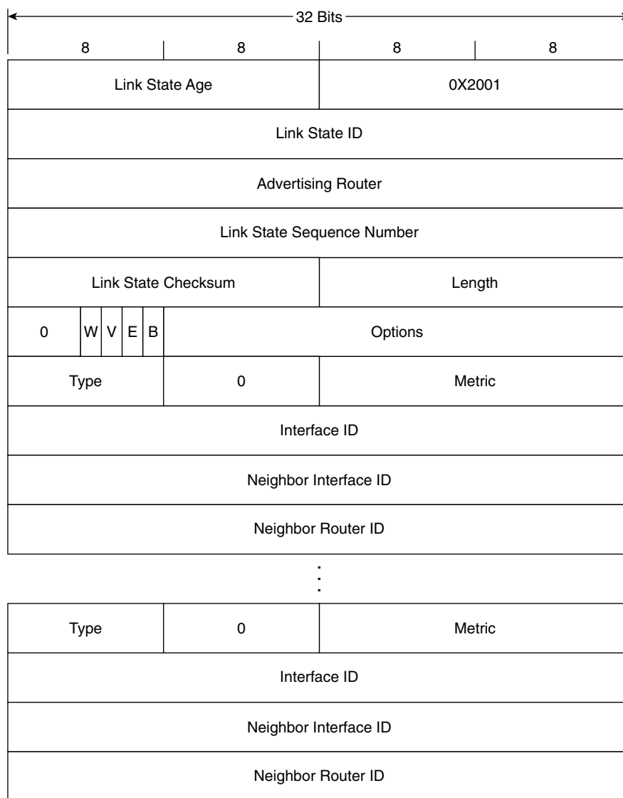
Figure 9-6 OSPFv3 Router LSA.
