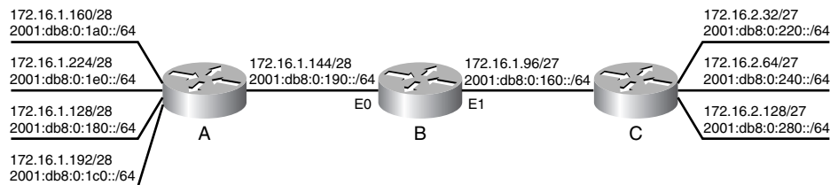
Figure 11-13 The network for Configuration Exercises 1, 2, and 3.
