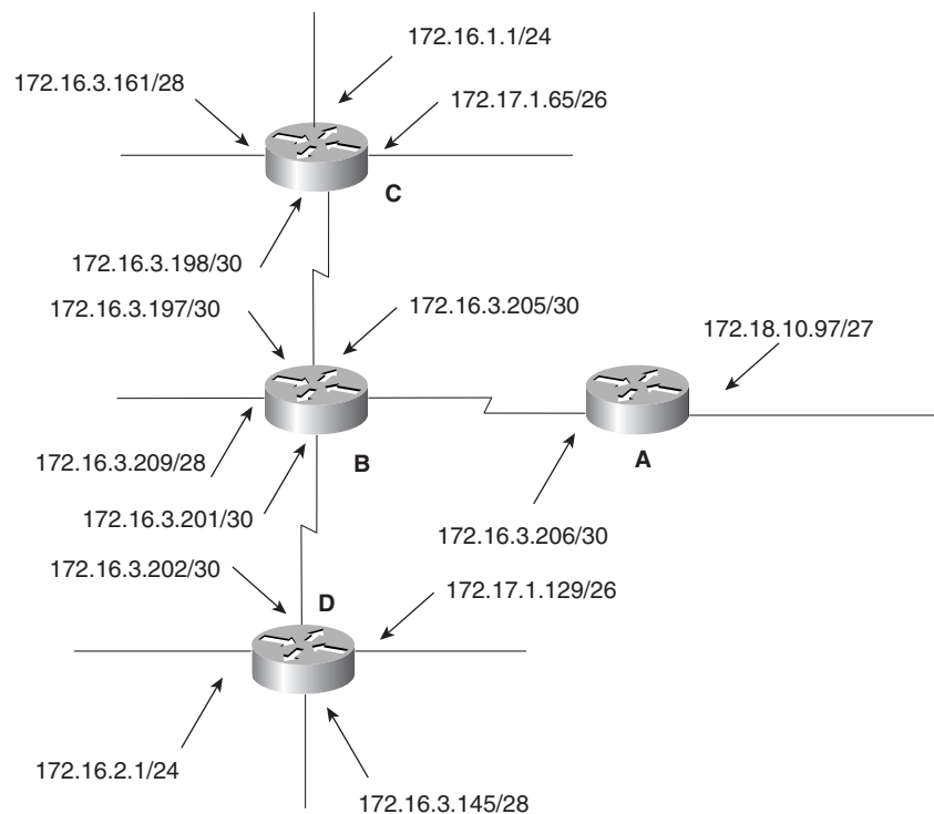
Figure 7-42 Network for Configuration Exercise 3.
