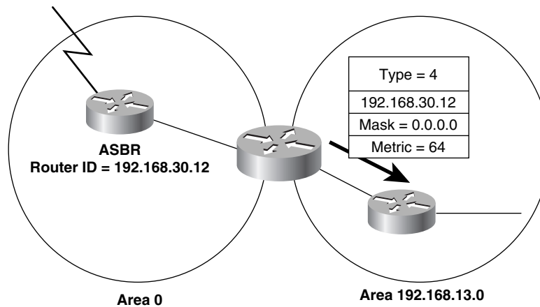
Example 8-14 ASBR Summary LSAs can be observed with the command show ip ospf database asbr-summary .
