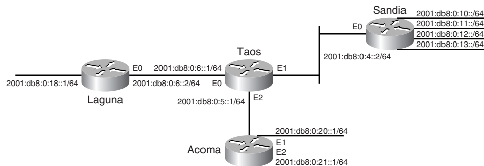
Figure 6-16 Acoma has been added to the network, with two IPv6-enabled Ethernet user LAN segments.
