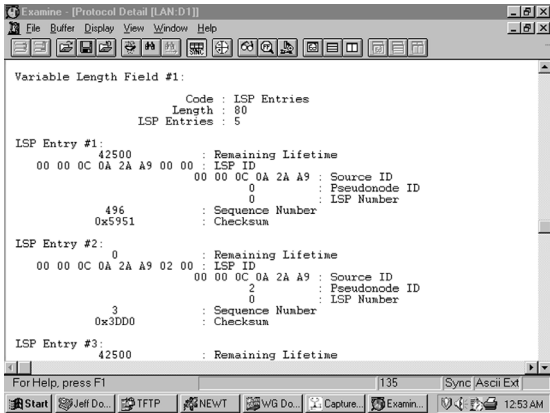
Figure 10-33 Part of the LSP Entries TLV of the CSNP in Figure 10-30.
