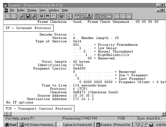
Figure 14-7 Pogo's policy route has set the Precedence bits of this packet to priority (001b) and the TOS bits to minimum delay and maximum reliability (1010b).
