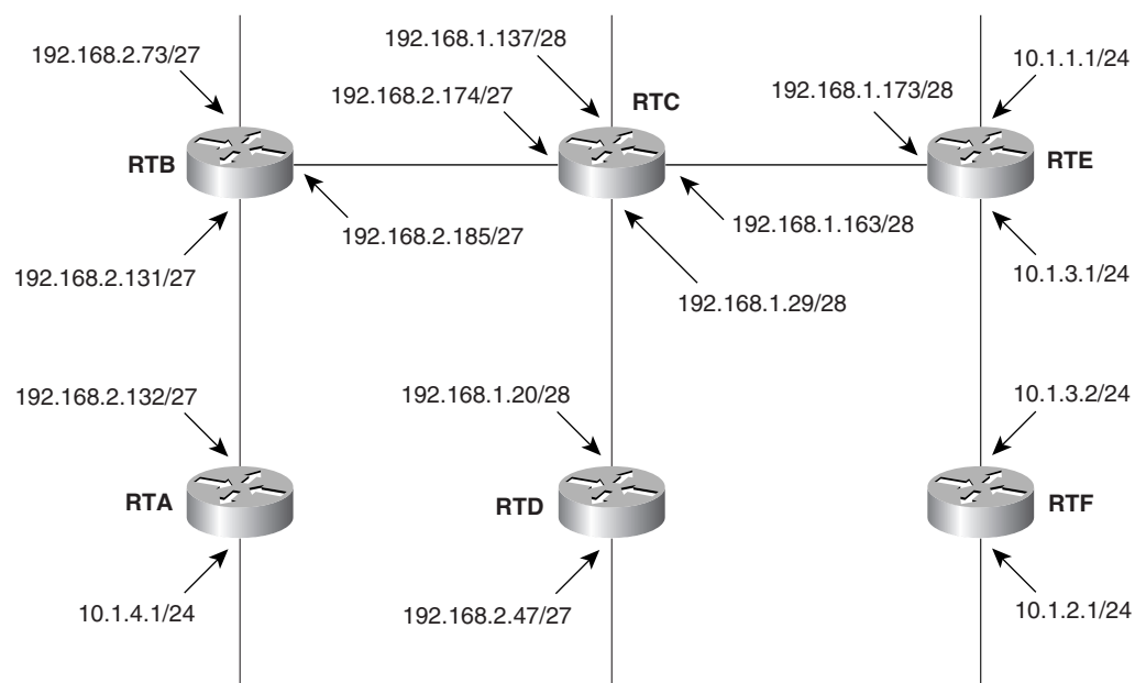
Figure 3-13 The network for Configuration Exercises 1 and 2.
