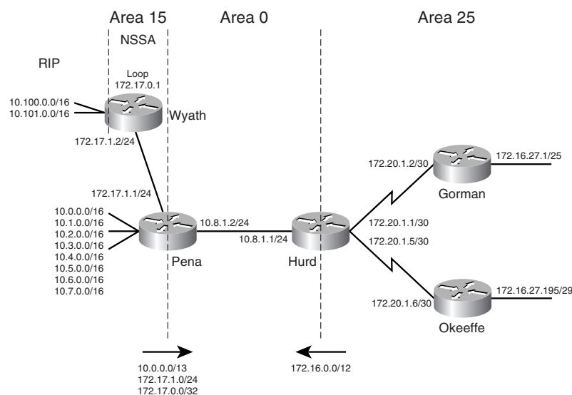
Figure 8-48 The addresses in areas 15 and 25 can be summarized into the backbone area.
