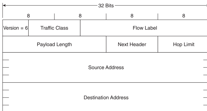
Figure 2-5 The IPv6 packet header.
