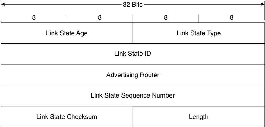
Figure 9-4 OSPFv3 LSA header.
