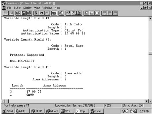
Figure 10-15 An Area Addresses TLV is shown as Variable Length Field #3. The analyzer also indicates the total addresses listed in the TLV (2) for convenience, but this information is not one of the TLV fields.
