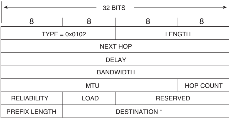
Figure 7-25 The IP Internal Routes TLV.
