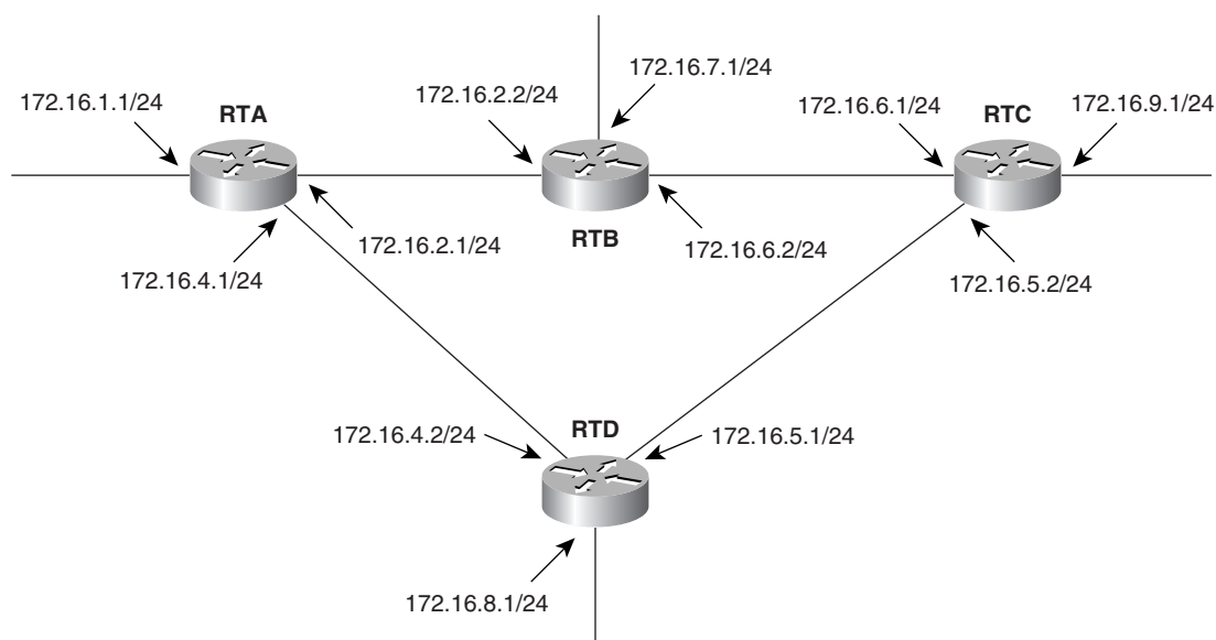
Figure 3-14 The network for Configuration Exercise 3.
