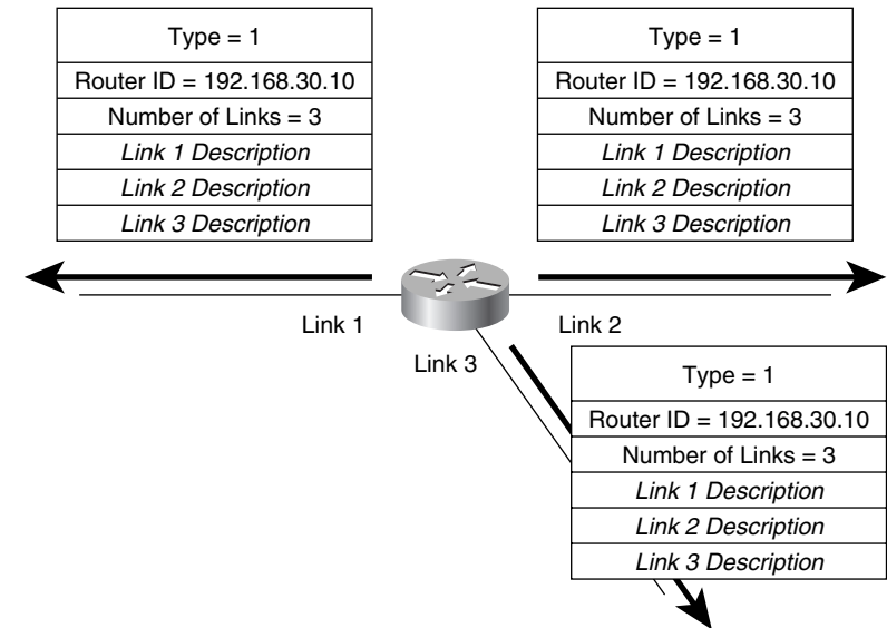
Figure 8-19 The Router LSA describes all of a router’s interfaces.
