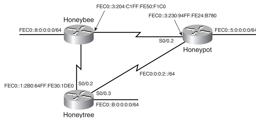
Figure 3-12 Alternative route added to the IPv6 network creates a triangle, with alternate paths to reach each router.
