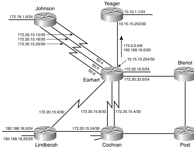
Figure 7-37 A new link is added between Lindbergh and Cochran to add redundancy for traffic connected to Lindbergh's LAN traveling into the core of the network.
