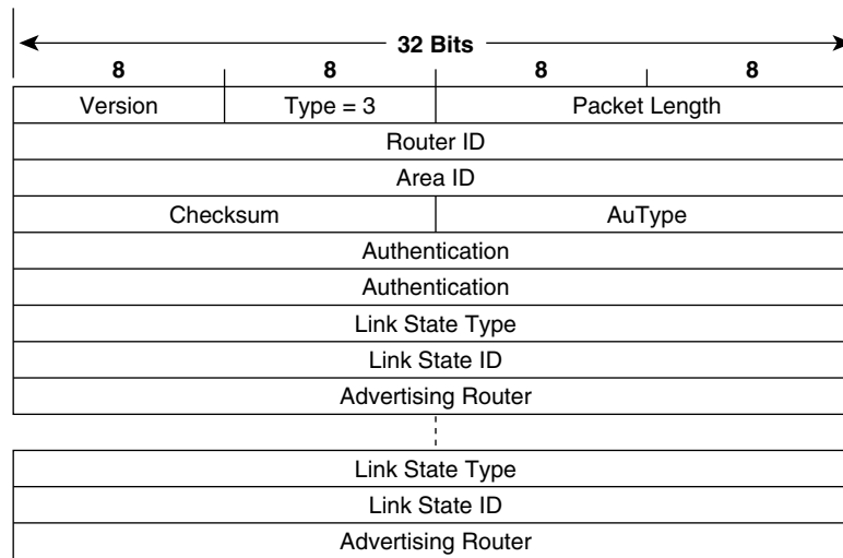
Figure 8-33 The OSPF Link State Request packet.
