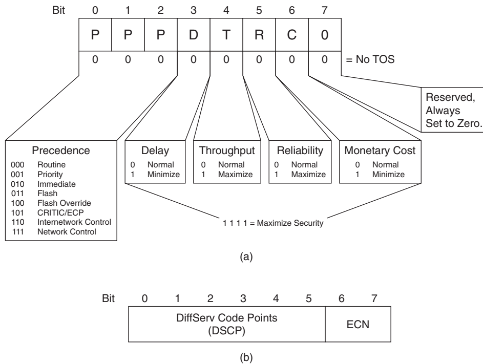
Figure 1-3 Type of Service (a) or DiffServ and ECN (b) field.
