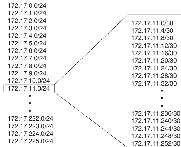
Figure 6-6 This class B address has been subnetted with a 24-bit mask. 172.17.11.0 has been sub-subnetted with a 30-bit mask; the resulting 64 subnets can be assigned to point-to-point links.
