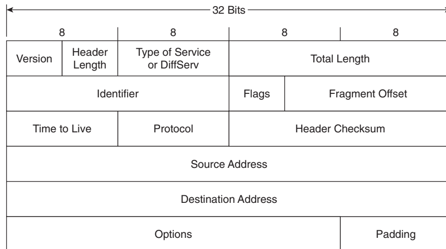
Figure 1-2 IP packet protocol.
