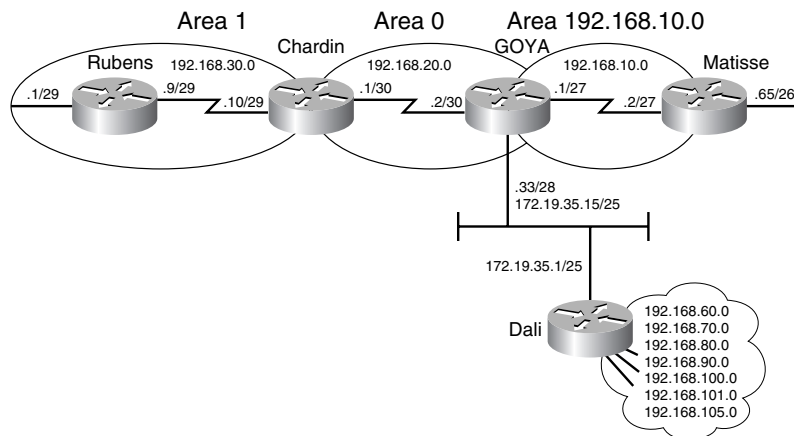
Example 8-53 An ABR that is also an ASBR will advertise the external routes into an NSSA with type 7 LSAs. In this example, Goya is advertising the external routes with an N1 metric type.
