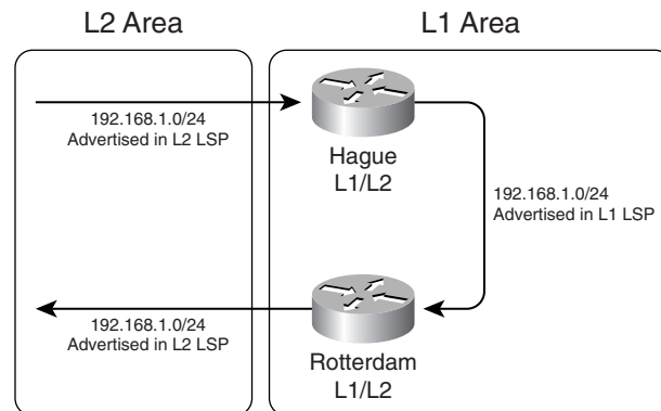
Figure 10-35 Under basic RFC 1195 rules, a prefix leaked from L2 to L1 is at risk of being advertised back to L2, creating a routing loop.
