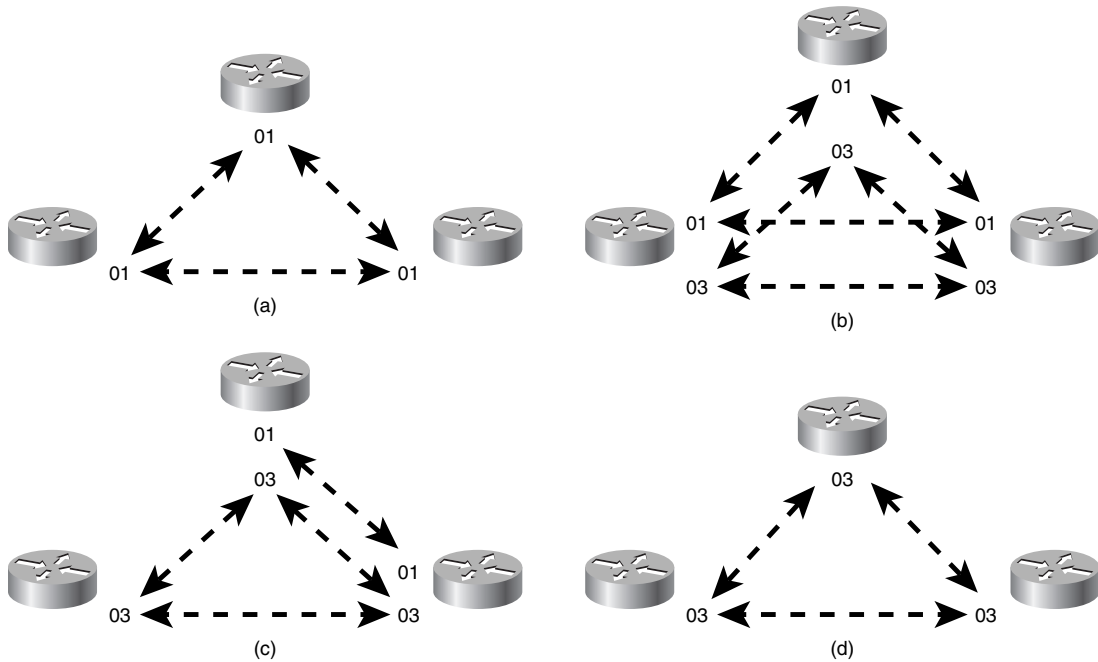
Figure 10-52 The support of multiple area addresses per router eases area changes.
