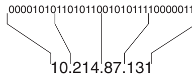
Figure 1-4 The dotted-decimal format is a convenient way to write IPv4 addresses, but it should not be confused with what the router (or host) sees: a 32-bit string.
