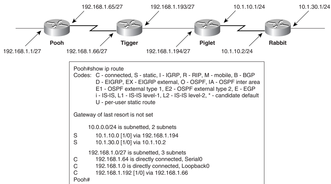
Figure 3-7 To reach network 10.1.30.0, Pooh must perform three route table lookups.
