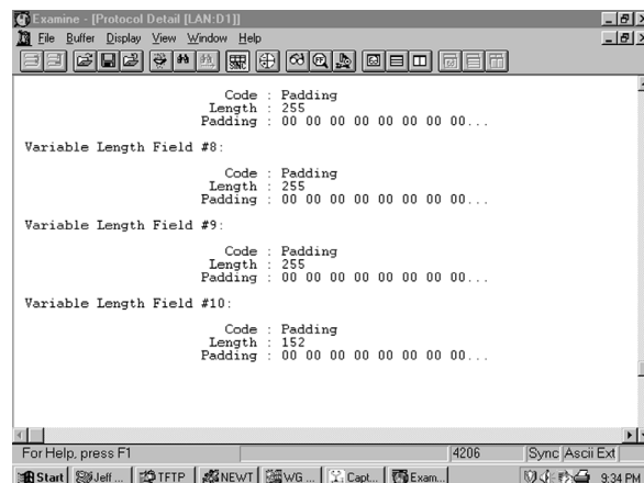
Figure 10-18 The last Variable Length Fields of the Hello PDU shown in Figure 10-12 are Padding TLVs, which bring the size of the PDU to the 1497-octet length shown in Figure 10-12. With the addition of the 3-octet LLC header and the 18-octet Ethernet header, the entire frame size is the 1518-octet Ethernet MTU.
