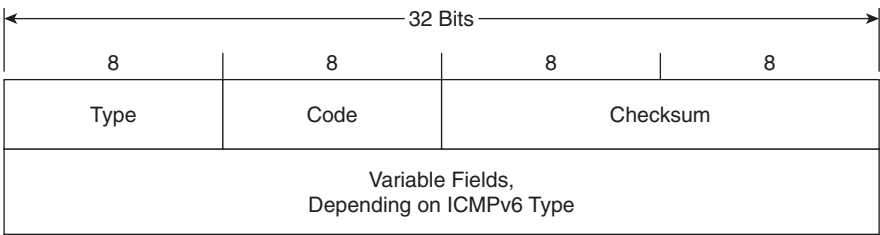
Figure 2-8 The ICMPv6 header format.
