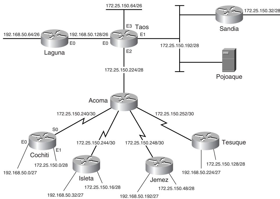
Figure 6-14 Cochiti, Isleta, Jemez, and Tesuque are each attached to two Ethernets. One Ethernet at each router is a member of subnet 172.25.150.0/24, and the other is a member of network 192.168.50.0/24.
