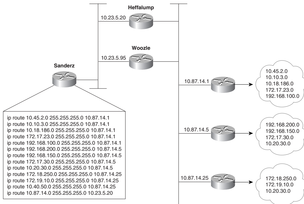
Figure 3-8 Configuring Sanderz for recursive lookups enables the network administrator to redirect all of that router's exit traffic from Heffalump to Woozle by changing one route entry.
