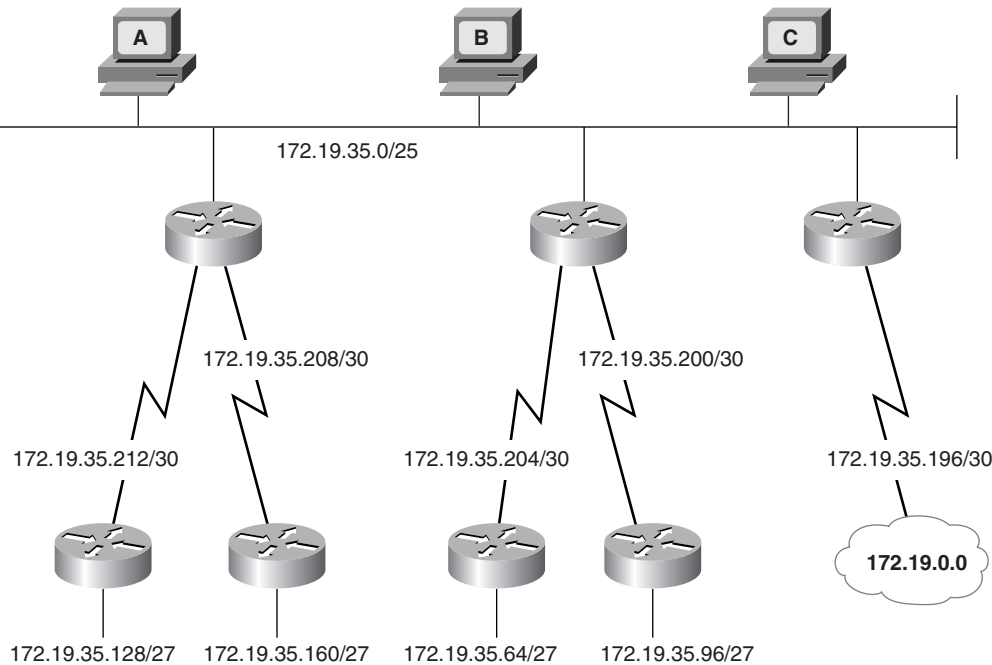
Figure 6-21 When analyzing any addressing scheme, and especially a VLSM design, the subnets for every data link should be determined so that conflicts and overlaps may be discovered.
