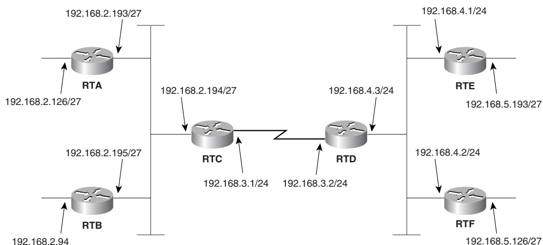
Figure 5-11 Network for Configuration Exercises 1 through 4.
