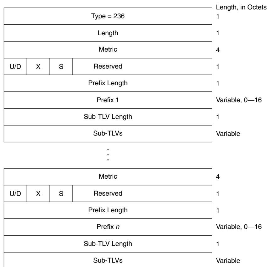
Figure 10-39 IPv6 Reachability TLV.
