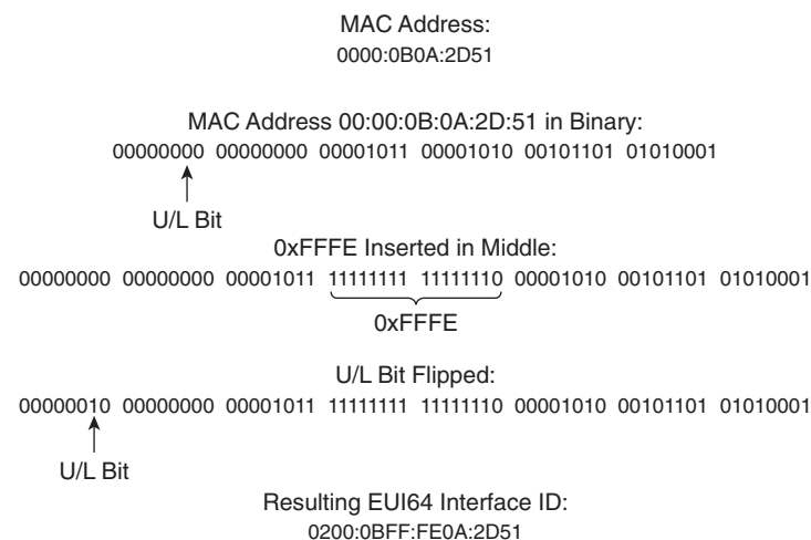
Figure 2-15 MAC-to-EUI64 conversion is used to create a 64-bit Interface ID from an interface’s 48-bit MAC address.
