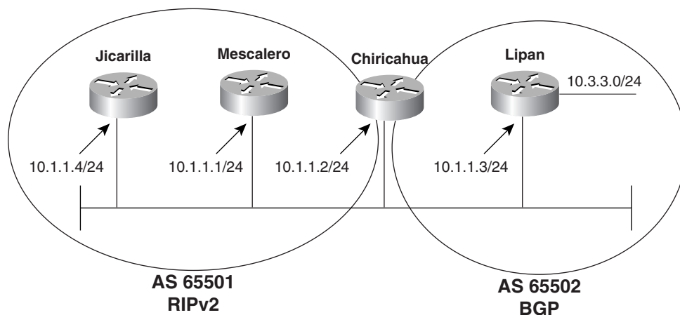
Figure 6-2 Although they share a common data link, Jicarilla and Mescalero speak only RIPv2; Lipan speaks only BGP. Chiricahua is responsible for informing the first two routers of any routes learned from the latter.
