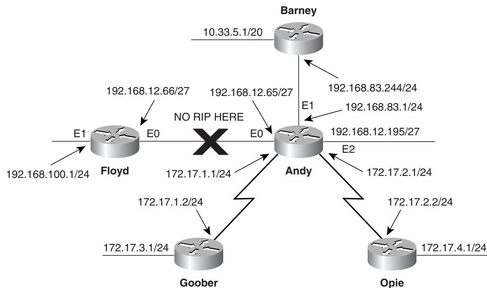
Figure 5-6 Network policy calls for no RIP exchanges between Andy and Floyd.
