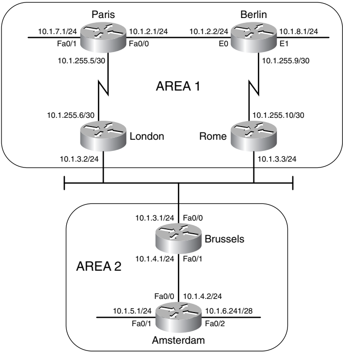
Figure 10-51 Area 1 is encoded as 00.0001 in the NET, and area 2 is encoded as 00.0002. The System ID of each NET is the E0 or T00 MAC identifier.
