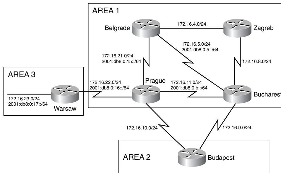
Figure 10-55 A network with multiple L1/L2 routers in area 1 could result in inefficient routing from area 1 to other areas.
