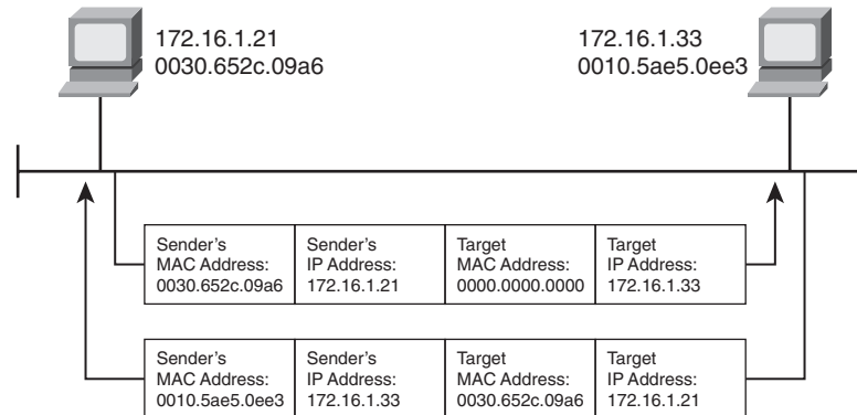
Figure 1-13 ARP is used to map a device's data-link identifier to its IP address.
