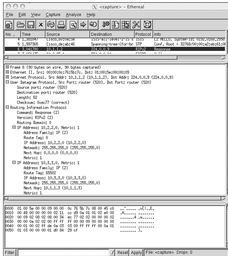
Figure 6-3 This protocol capture of a RIPv2 update from Chiricahua shows the Route Tag, Subnet Mask, and Next Hop fields being used to advertise subnet 10.3.3.0.
