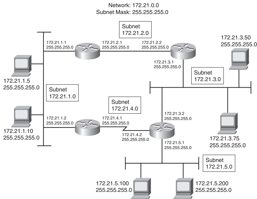
Figure 1-7 Subnet masks allow a single network address to be used on multiple data links by “borrowing” some of the host bits for use as subnet bits.
