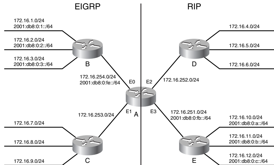
Figure 13-7 The network for Configuration Exercises 1 through 4.
