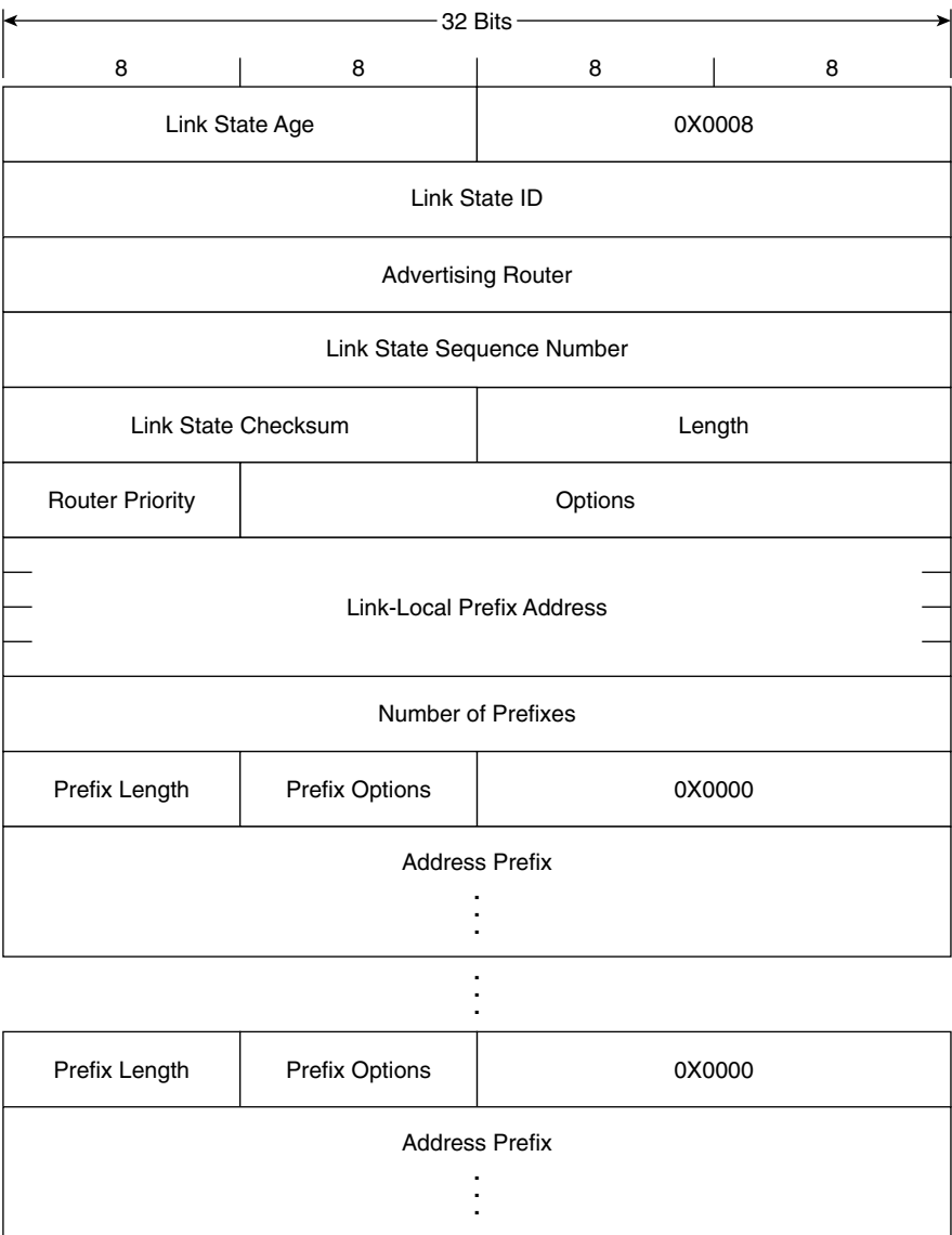
Figure 9-11 OSPFv3 Link LSA.
