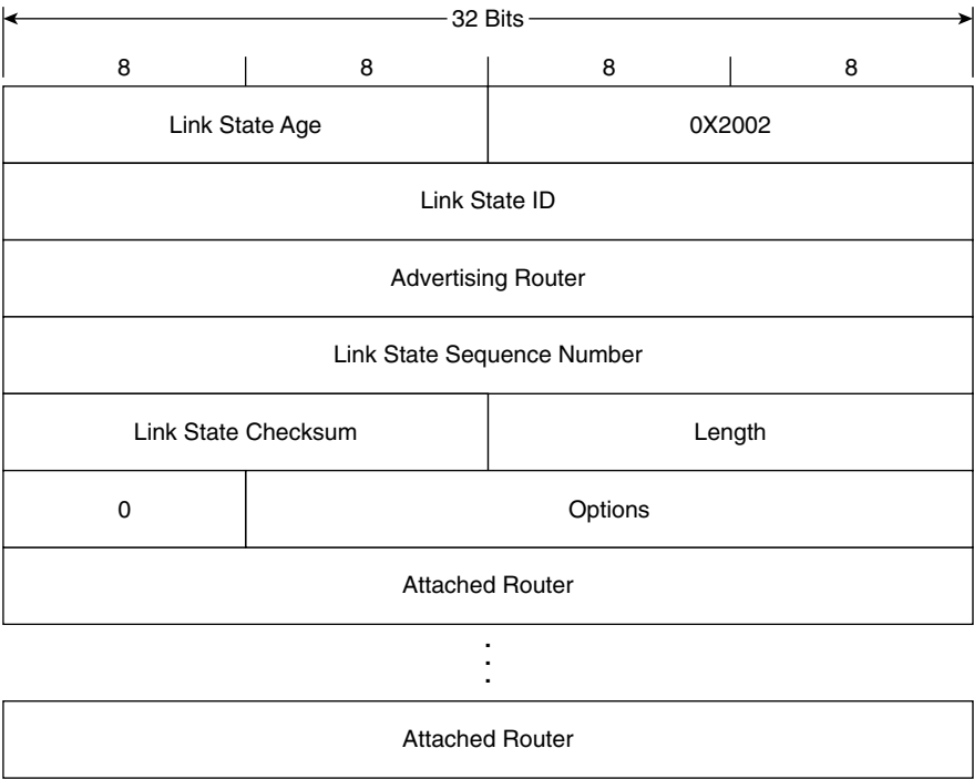
Figure 9-7 OSPFv3 Network LSA.
