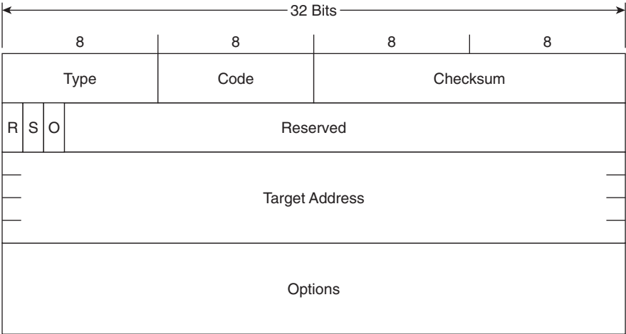
Figure 2-12 The Neighbor Advertisement message format.
