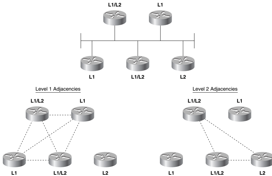
Figure 10-7 Separate adjacencies are established for level 1 and for level 2, so separate DRs must be elected for level 1 and level 2.
