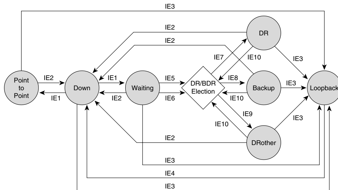
Figure 8-3 The OSPF interface state machine; see Table 8-1 for a description of input events (IEs).
