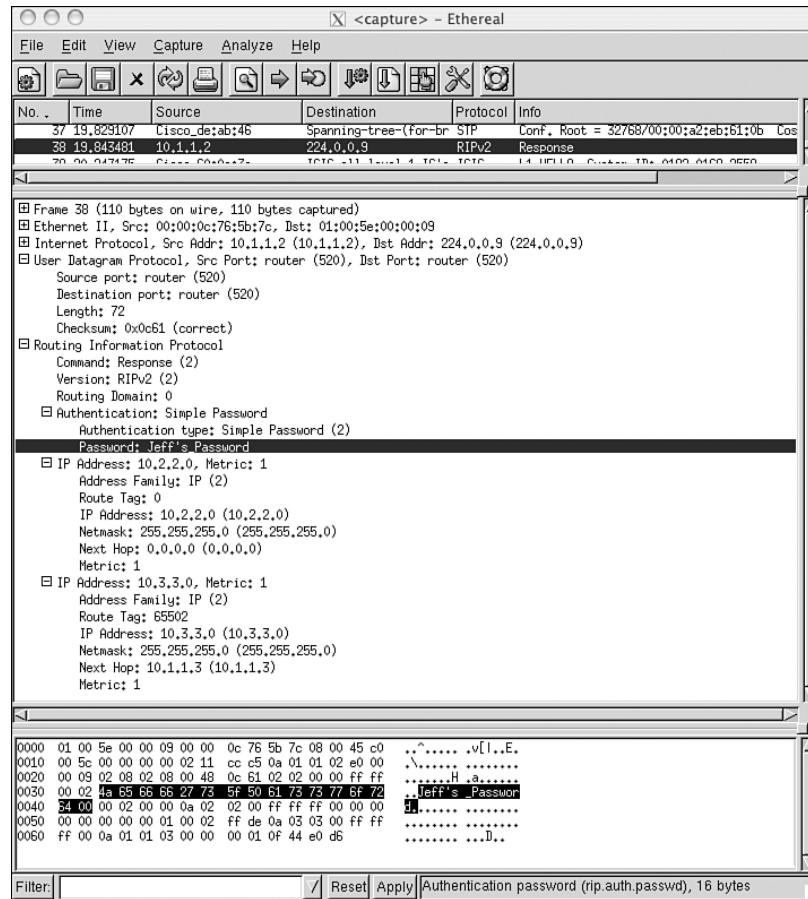
Figure 6-8 When simple password authentication is used, the password is carried in plain text and can be read by anyone who can “sniff” the packet carrying the update.
