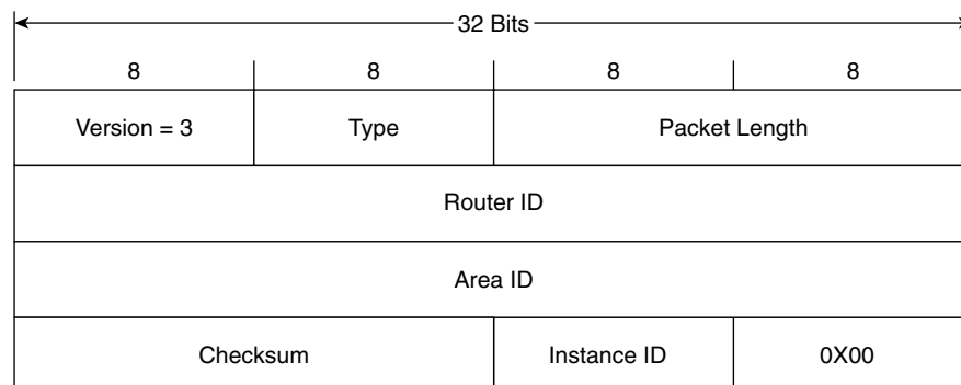
Figure 9-1 OSPFv3 packet header.
