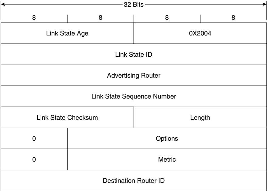
Figure 9-9 OSPFv3 Inter-Area Router LSA.
