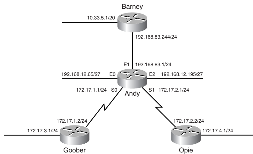
Figure 5-5 Both Andy and Barney are border routers between class-level networks.
