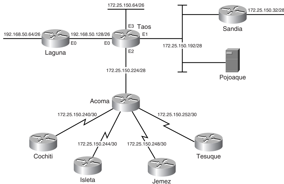
Figure 6-13 VLSM can be used to adapt addresses to the requirements of individual data links.
