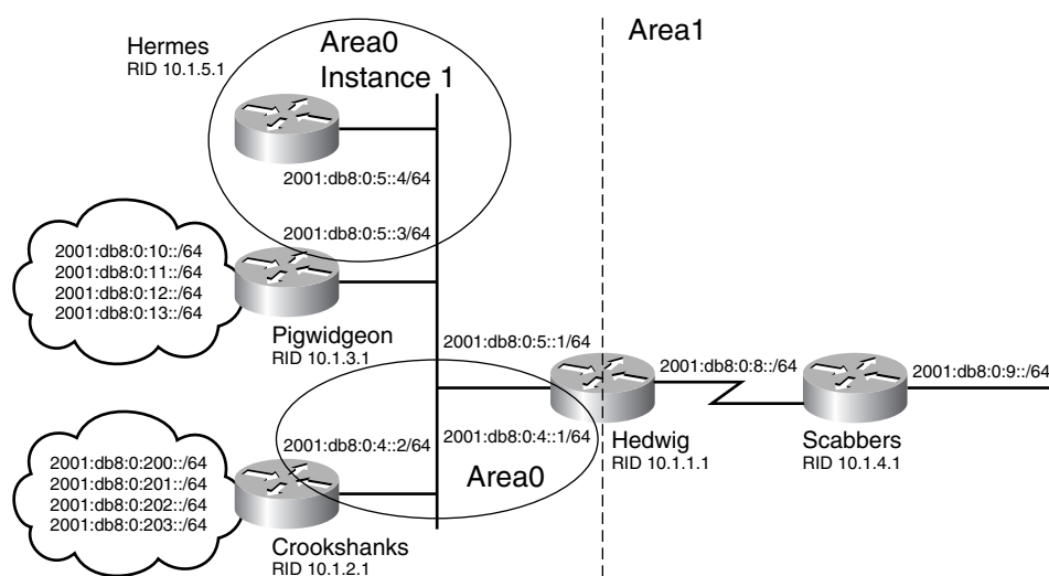
Figure 9-16 A new router is added to the network of Figure 9-15.
