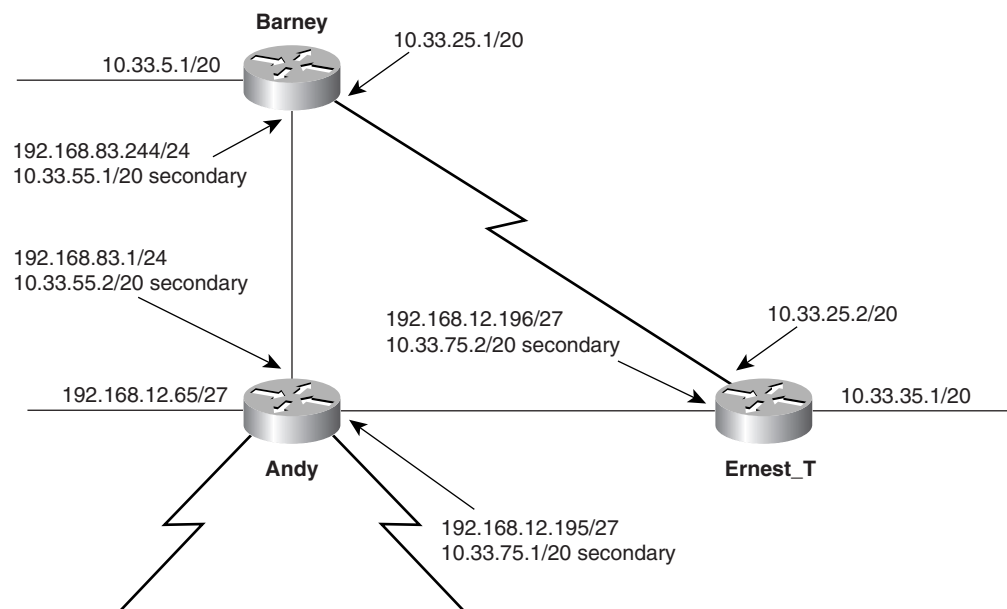
Figure 5-10 RIP metrics must be manipulated so that the two-hop Ethernet route between Barney and Ernest_T will be preferred over the one-hop serial route.
