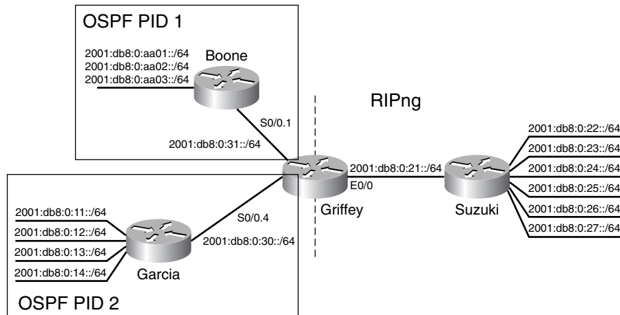
Figure 11-11 IPv6 is being routed with both OSPFv3 and RIPv6, and a single router is redistributing between the routing protocols.
