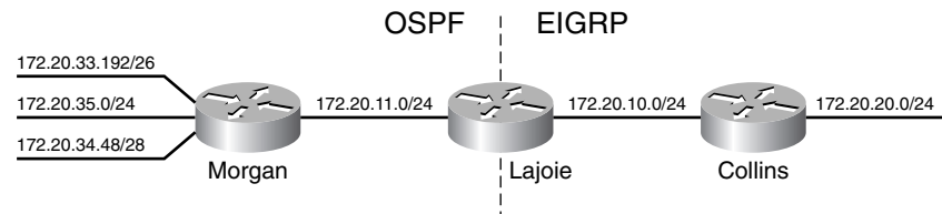
Example 11-12 Lajoie's EIGRP configuration shows OSPF being redistributed into the EIGRP process.
