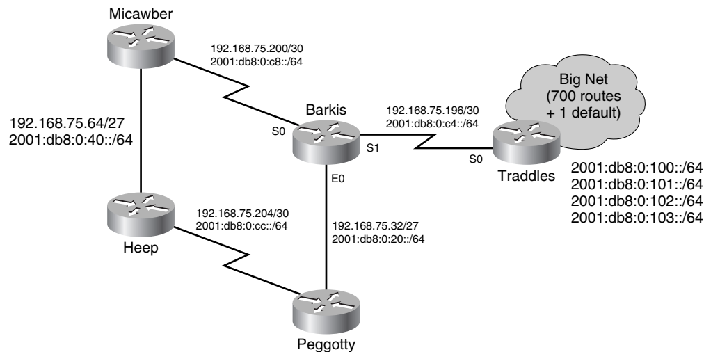
Figure 13-2 A route filter at Barkis will accept only the default route from Traddles and will reject all other BigNet routes.
