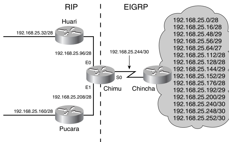
Figure 12-4 A default route enables RIP to route into the variably subnetted EIGRP domain.
