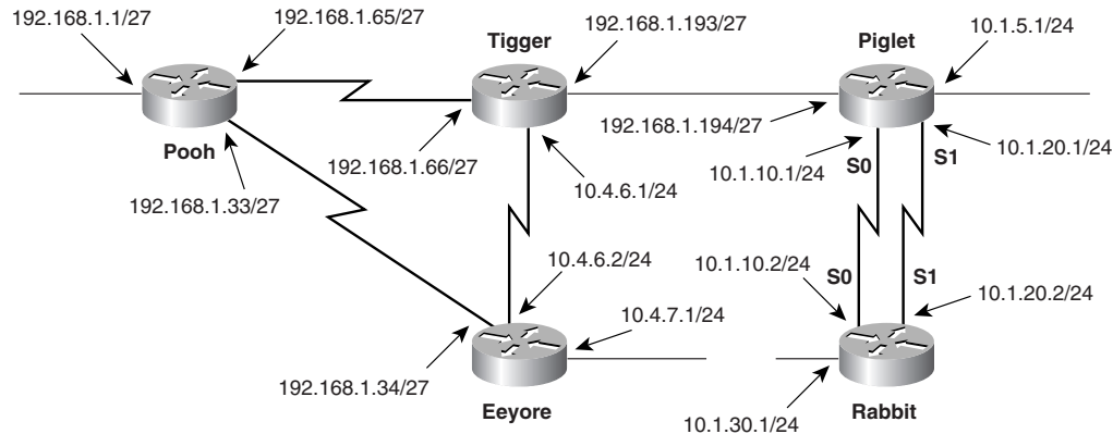
Figure 3-5 A new router has been connected to Piglet. Two serial links are used: one for the primary link and one for the backup link.
