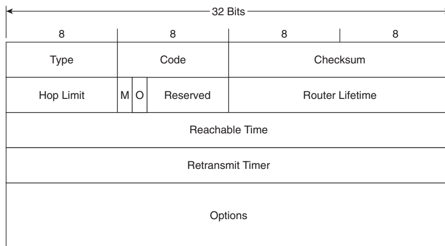
Figure 2-9 The Router Advertisement message format.
