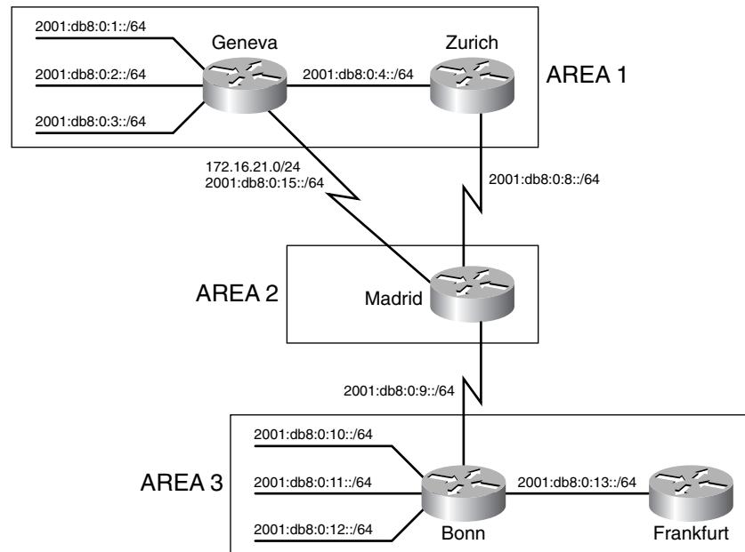
Figure 10-54 IS-IS for IPv6 is added to the network.
