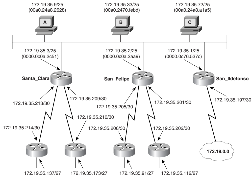
Figure 6-18 When host B pings host C, the first ping is successful and subsequent pings fail.
