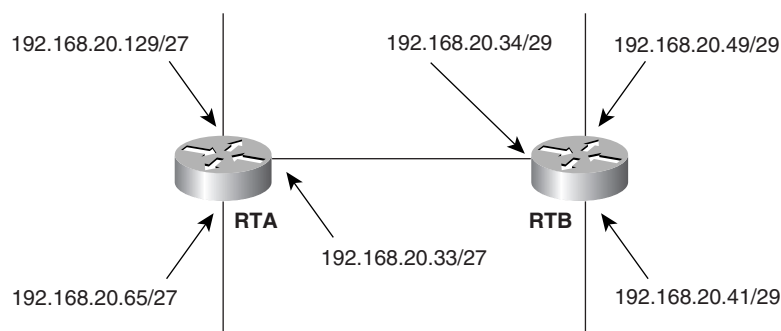
Figure 5-12 Network for Configuration Exercise 5.
