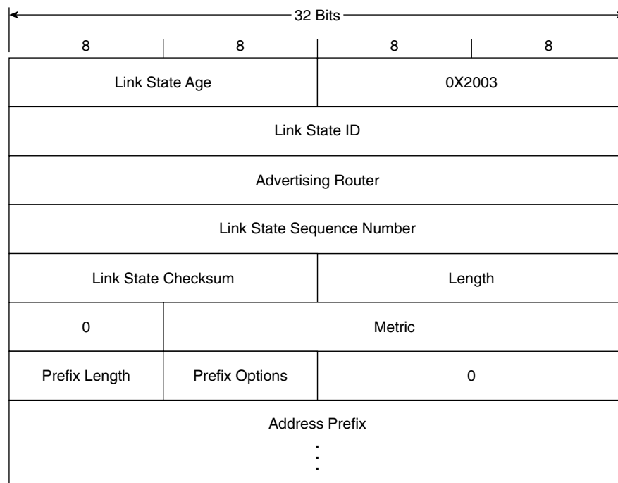
Figure 9-8 OSPFv3 Inter-Area Prefix LSA.
