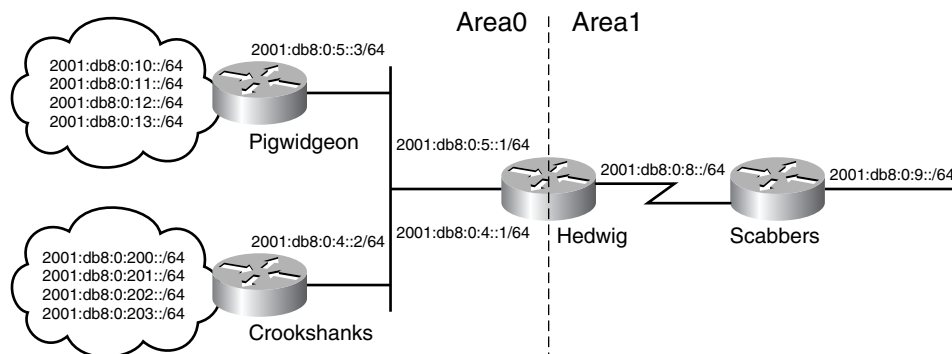
Figure 9-15 Example of an OSPFv3 network.
