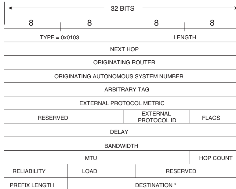
Figure 7-26 The IP External Routes TLV.
