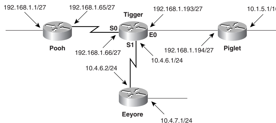
Figure 3-2 Routing protocols such as RIP and IGRP cannot easily route this discontiguous, variably subnetted network, but static routing will work.
