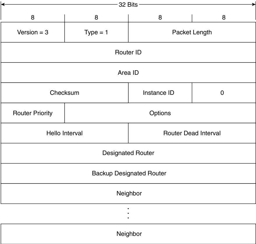
Figure 9-2 OSPFv3 Hello message.
