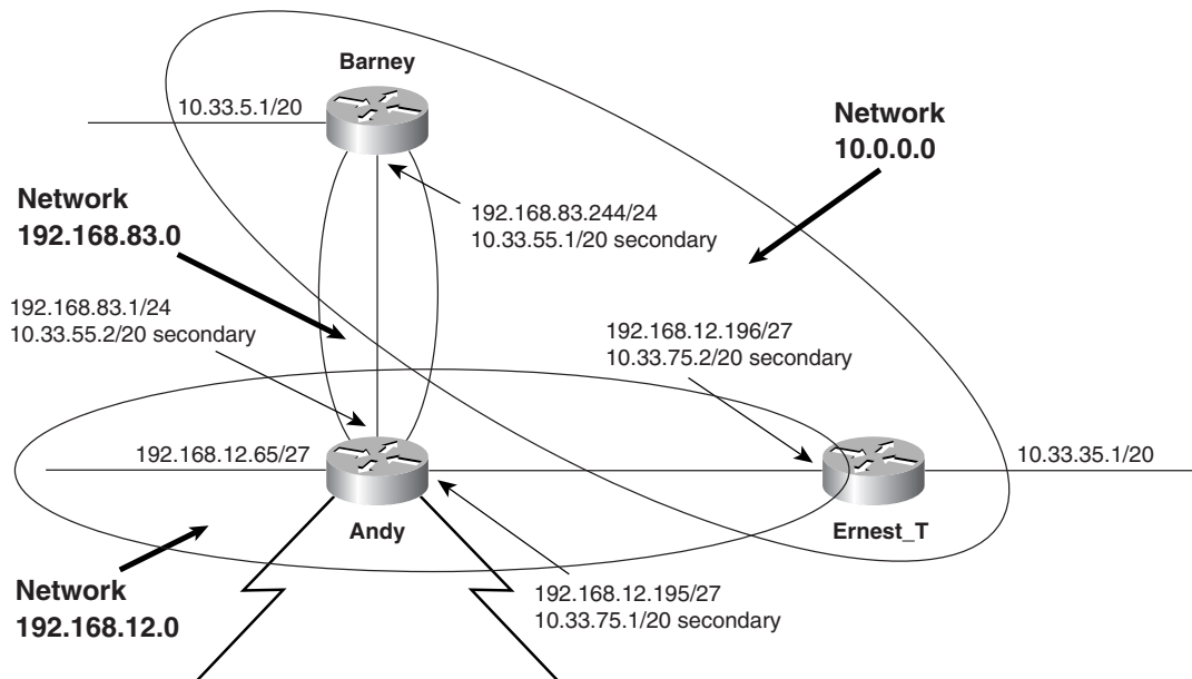
Figure 5-9 Secondary addresses are used to connect the subnets of network 10.0.0.0 across the same links on which other network addresses exist.
