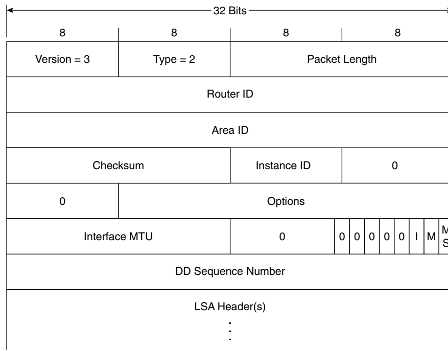
Figure 9-3 OSPFv3 Database Description message.
