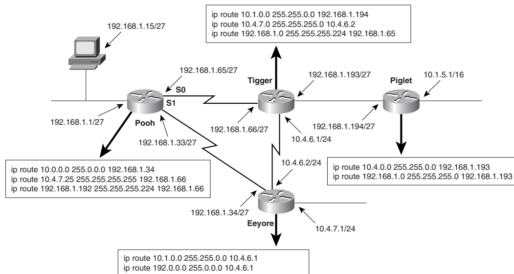
Figure 3-9 Packets from subnet 192.168.1.0/27 to subnet 10.1.0.0/16 are routed correctly, but Pooh itself cannot ping any device on 10.1.0.0/16.
