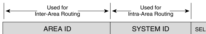
Figure 10-4 The NET specifies the Area ID and the System ID of an IS or ES.
