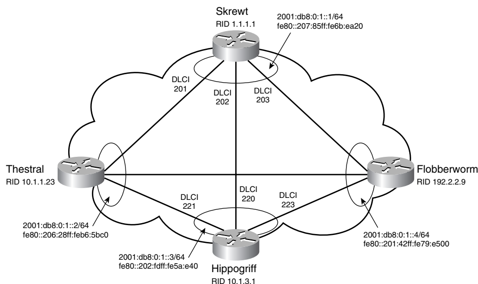
Figure 9-17 Several options exist for configuring OSPFv3 for IPv6 on this Frame Relay network.
