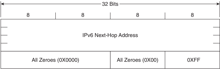
Figure 6-11 A metric value of all ones specifies that the route entry is a next-hop route entry. All route entries following this one, until the end of the message or until another next-hop route entry is encountered, use this next-hop address.
