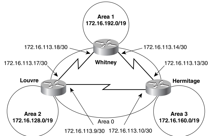
Figure 8-55 The summary addresses shown for each area will be advertised into area 0. Area 0 will also be summarized into the other areas.
