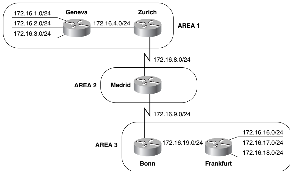
Figure 10-53 Zurich and Bonn are summarizing areas 1 and 3 into area 2.
