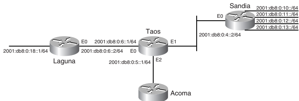
Figure 6-15 IPv6 addresses are configured on Laguna, Taos, and Sandia's interfaces that are to run RIPvng.
