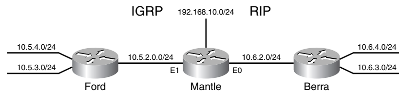
Example 11-17 Mantle is running both IGRP and RIP and performing redistribution between the two protocols, using both the default metric and the metric assigned with the redistribution command.
