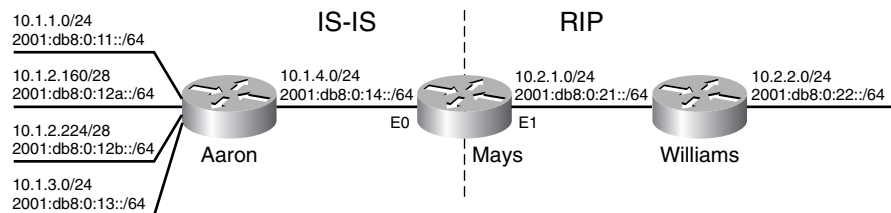
Figure 11-12 Router Mays is redistributing RIP into IS-IS and IS-IS into RIP.
