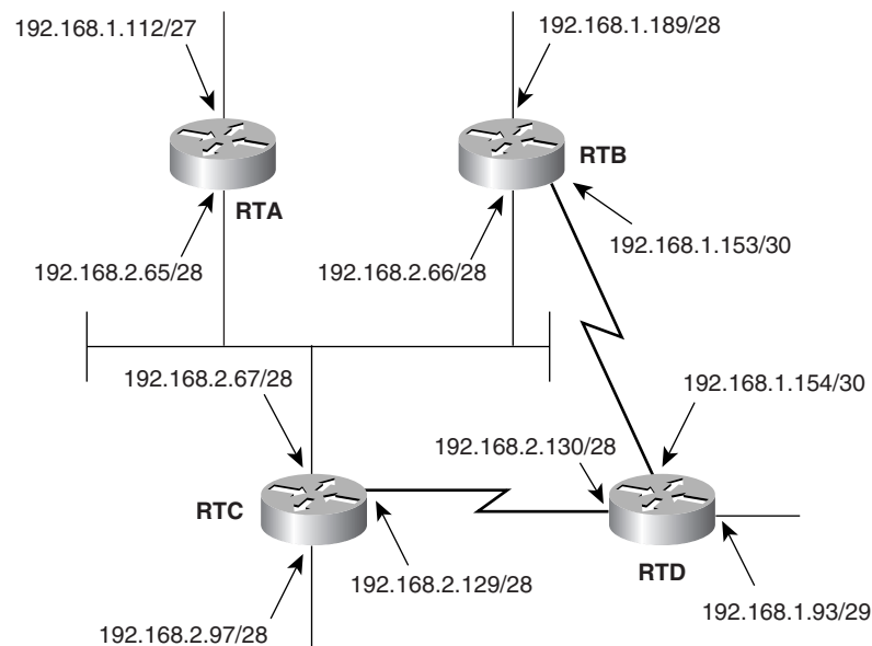
Figure 6-22 The network for Configuration Exercises 3 through 6.
