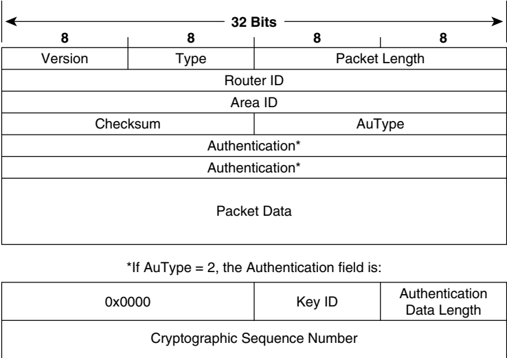
Figure 8-30 The OSPF packet header.
