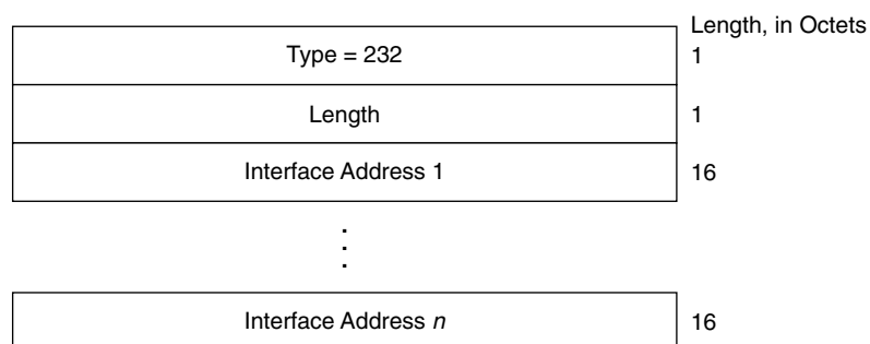
Figure 10-40 IPv6 Interface Address TLV.
