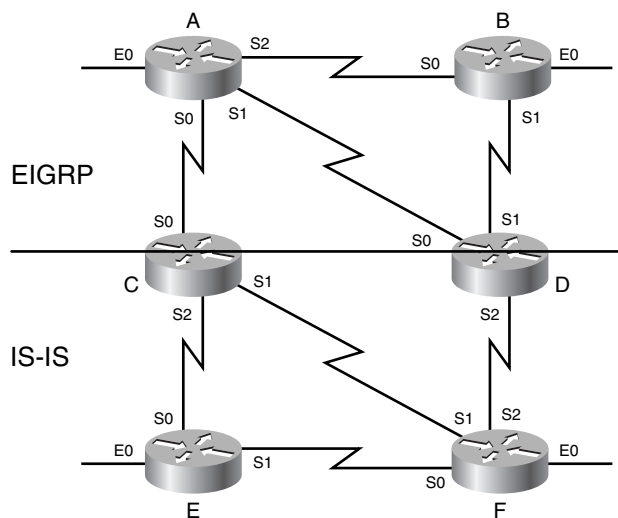
Figure 13-8 The network for Configuration Exercises 6 through 8.
