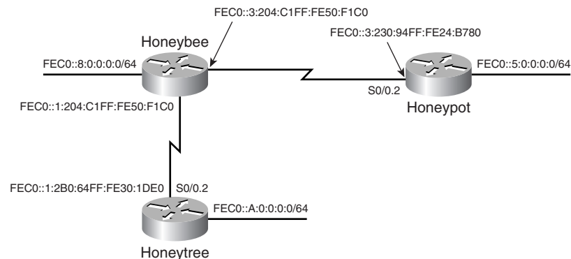
Figure 3-3 Static routing also works with IPv6.
