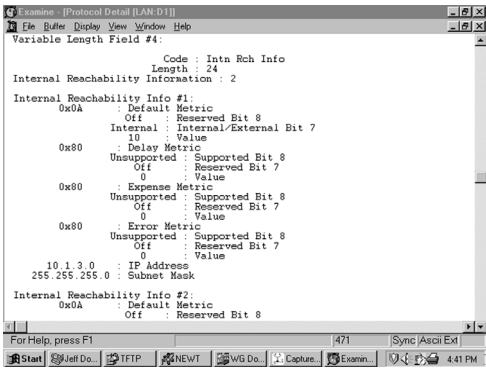
Figure 10-27 Analyzer capture of an IP Internal Reachability Information TLV.
