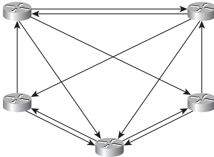
Figure 10-50 A received LSP is flooded on all interfaces except those belonging to the same mesh group as the interface on which it was received.
