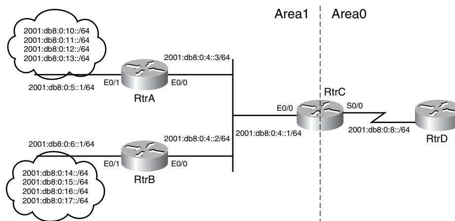
Figure 9-19 IPv6 OSPFv3 network.
