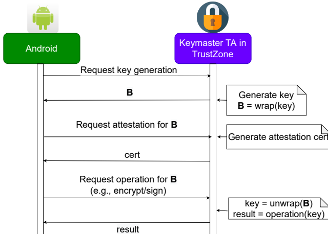
Figure 2: A usage example of an Android application using a Hardware-Backed Keystore (i.e., the Keymaster TA) for cryptographic key management: key generation, attestation, and encryption/signature. 2
