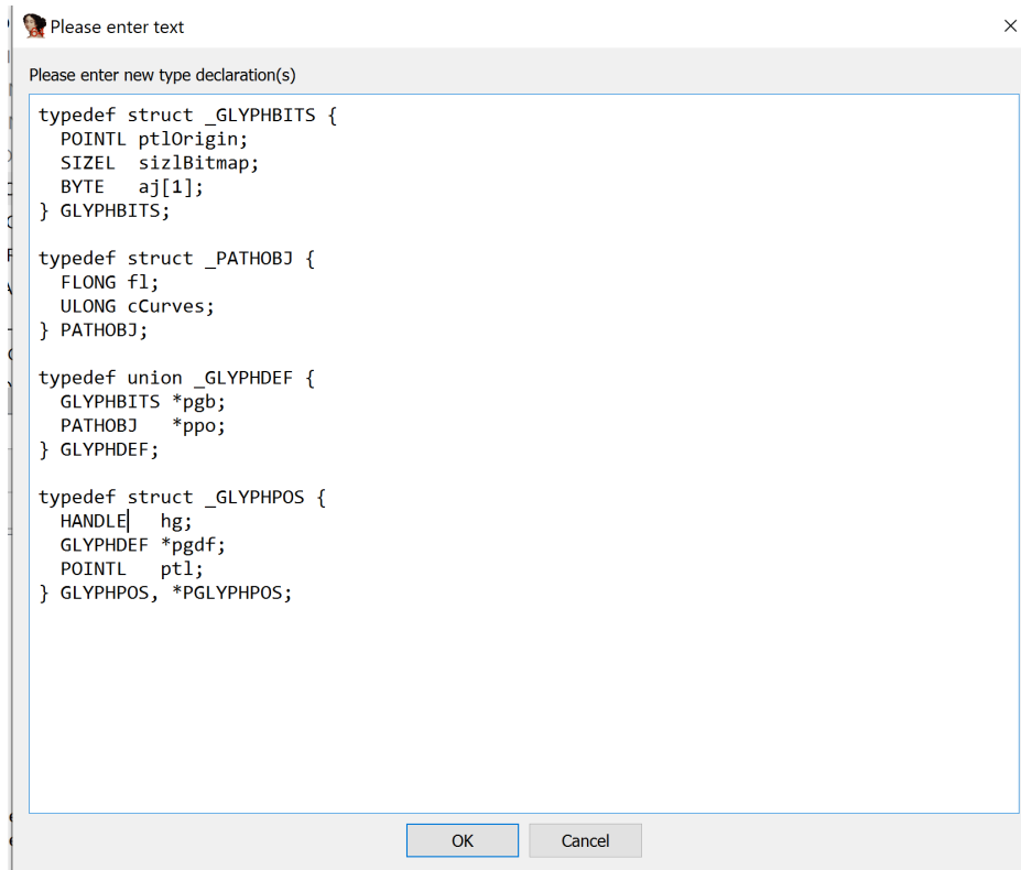
Figure 3 – Declaring multiple structure definitions in IDA Pro's type editor
