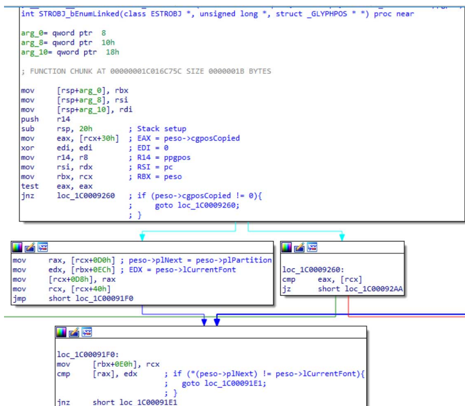
Figure 9 – Disassembly of opening lines of STROBJ_bEnumLinked
