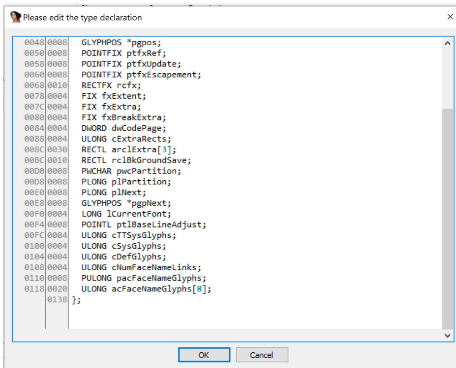
Figure 7 – Viewing outdated ESTROBJ structure
