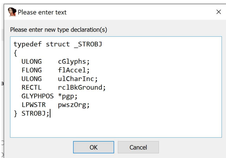
Figure 4 – Defining the STROBJ structure in IDA Pro's type editor
