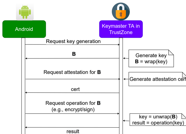
Figure 2: A usage example of an Android application using a Hardware-Backed Keystore (i.e., the Keymaster TA) for cryptographic key management: key generation, attestation, and encryption/signature. 2
