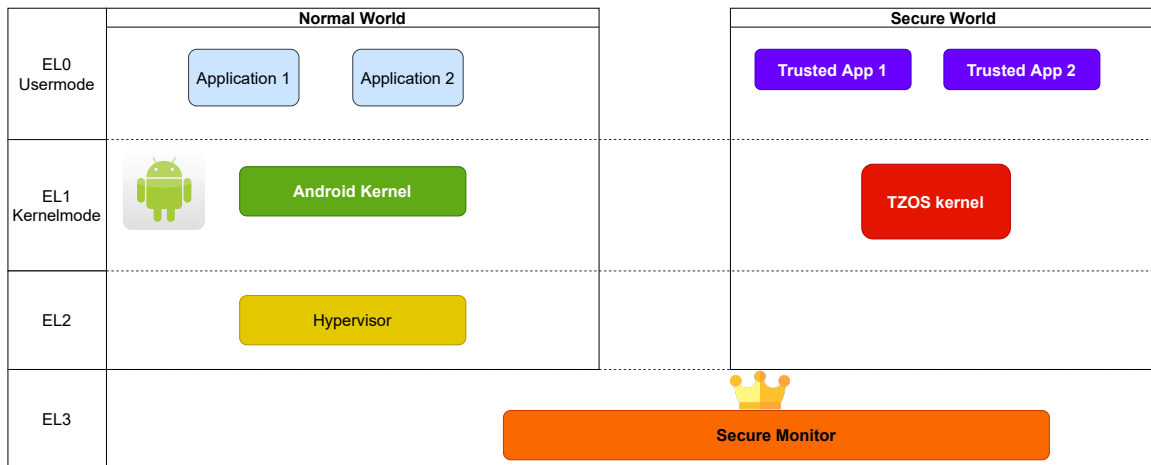
Figure 1: The TrustZone software and hardware isolation architecture 2
