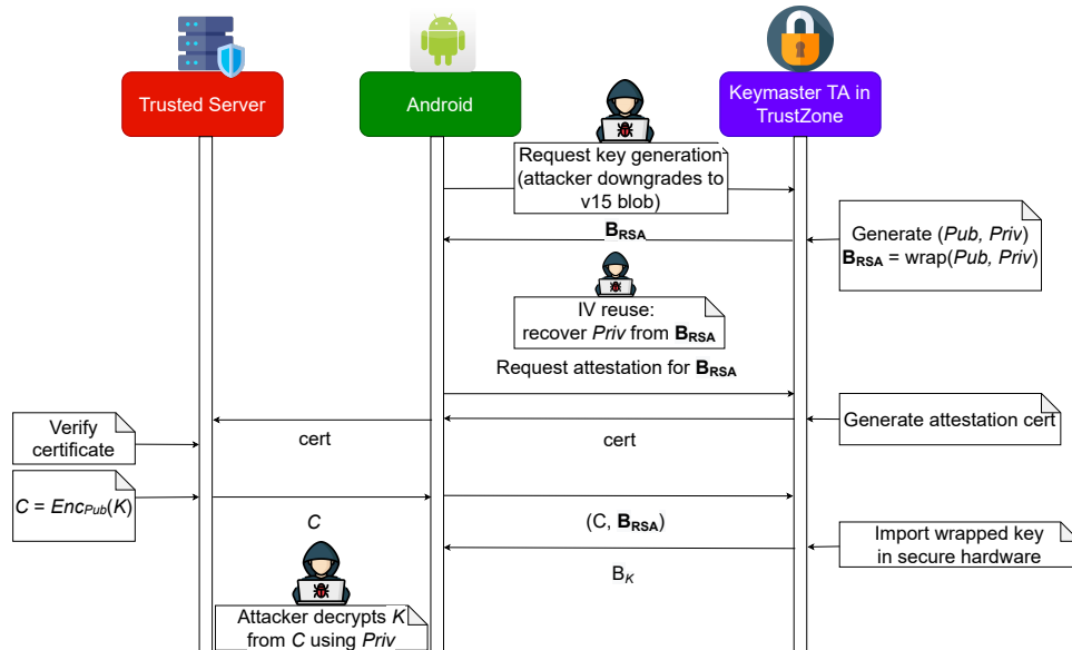
Figure 5: Simplified Secure Key Import: the “hacker” icons indicate the interception points used in our attack 2
