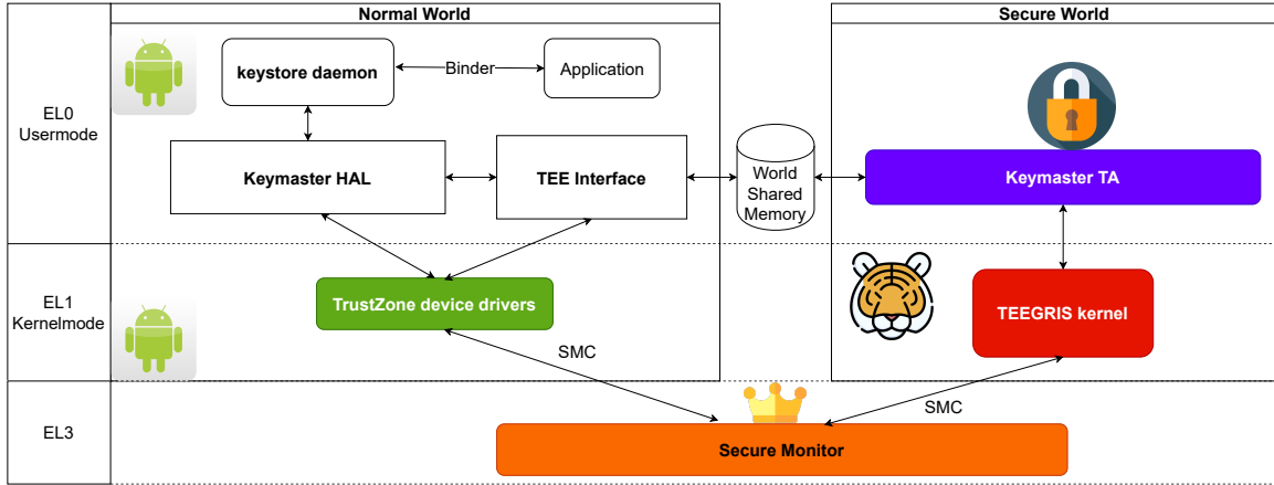
Figure 3: Overview of the Hardware backed keystore 2
