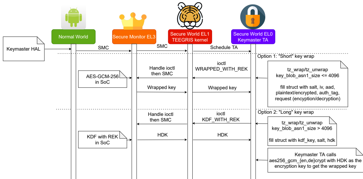
Figure 8: Key wrapping in Keymaster TA in TEEGRIS 2
