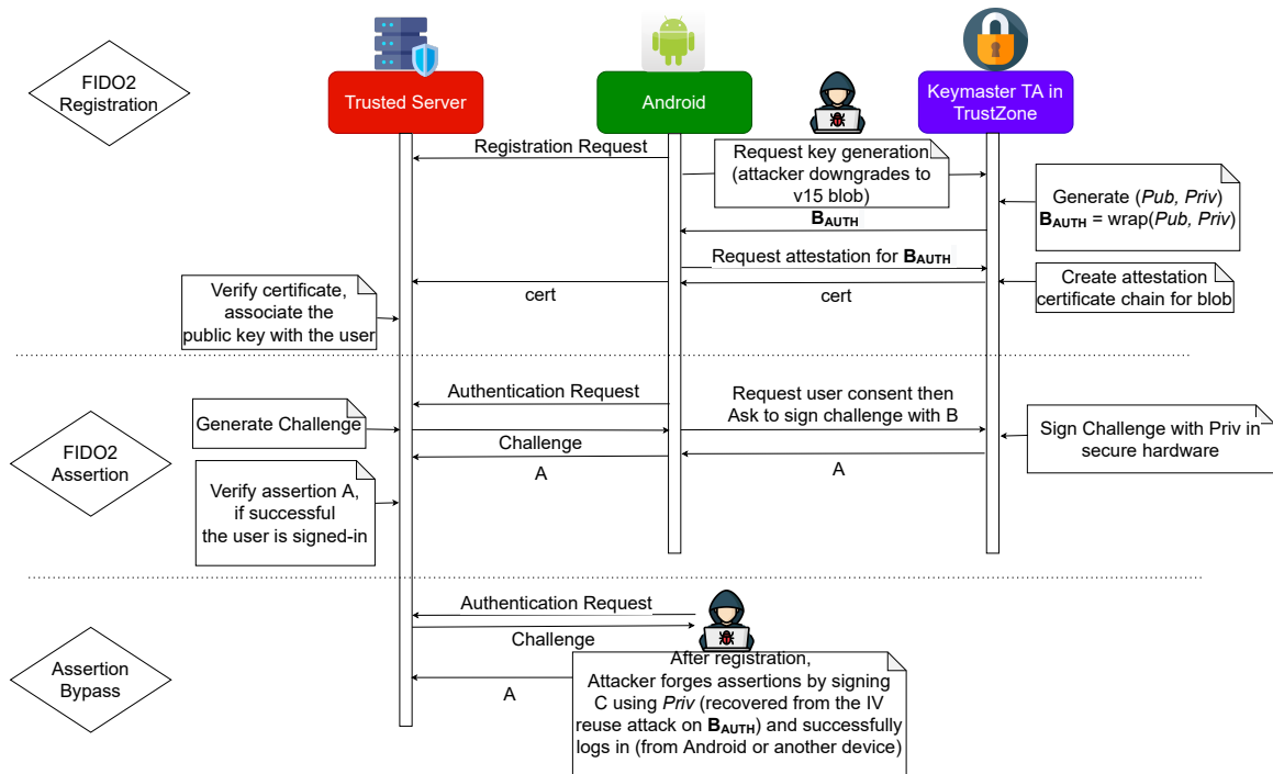
Figure 6: FIDO2 WebAuthn: the “hacker” icons indicate the interception points used in our attack 2
