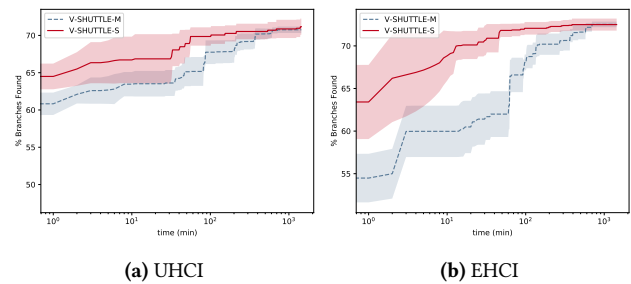
Figure 8: Ant Group-QEMU’s branch coverage results found by V-SHUTTLE during a 24-hours run. The line indicates averages while the shaded area represents the 95% confidence intervals across 10 runs.
