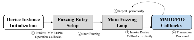
Figure 6: V-SHUTTLE’s fuzzing loop.
