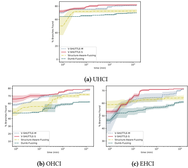
Figure 7: QEMU’s branch coverage results of V-SHUTTLE during a 24-hour run. The line indicates the averages while the shaded area represents the 95% confidence intervals across 10 runs.
