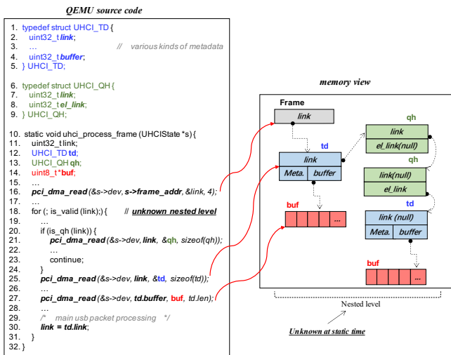
Figure 2: An example presenting nested structures in Universal Host Controller Interface (UHCI). Here td, qh, buf represent three different types of objects, respectively (td and qh are the structures containing the amounts of metadata, while buf is the raw data).
