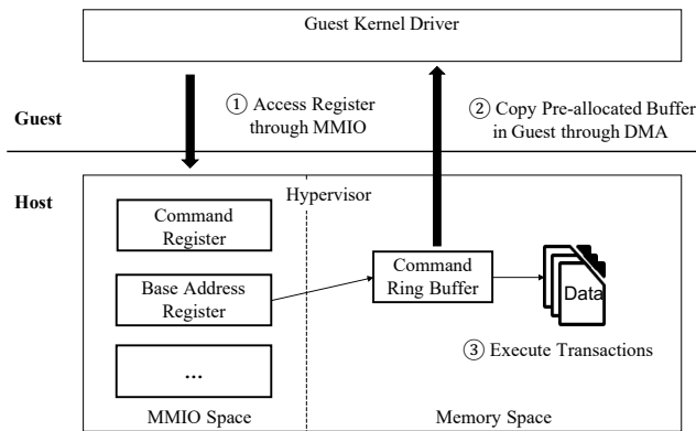
Figure 1: General workflow of the virtual machine transaction.
