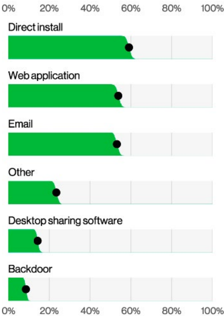
Figure 29. Top Action vectors in System Intrusion incidents (n=1,789)
