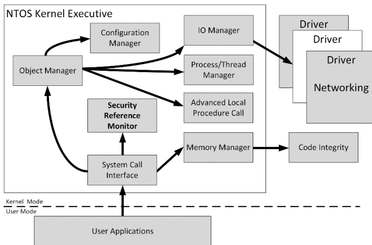
Figure 2-1 The Windows kernel executive modules
