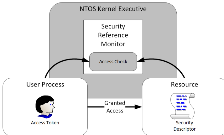
Figure 2-2 Components of the security reference monitor
