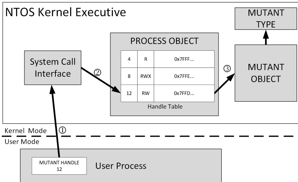
Figure 2-4 The handle table lookup process
