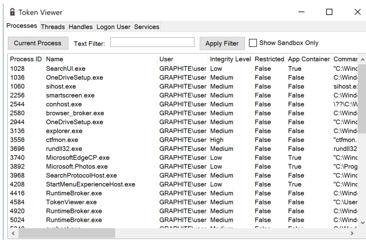
Figure 4-1 The Token Viewer, which lists all accessible processes and their tokens
