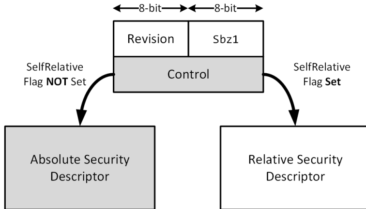
Figure 5-2 Selecting the security descriptor format based on the SelfRelative control flag
