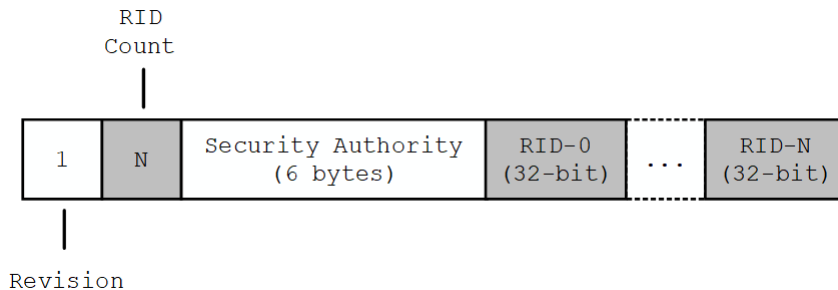
Figure 5-1 The security identifier (SID) structure in memory
