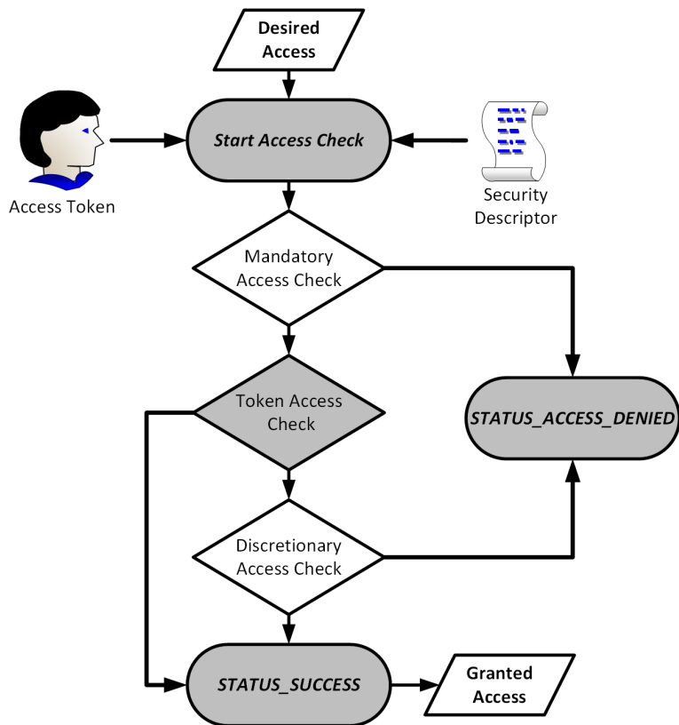
Figure 7-3 The access-check process
