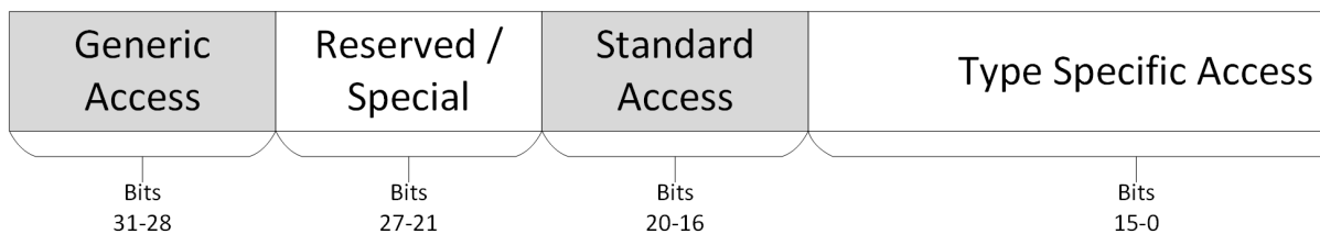
Figure 2-5 The structure of access mask bitfields
