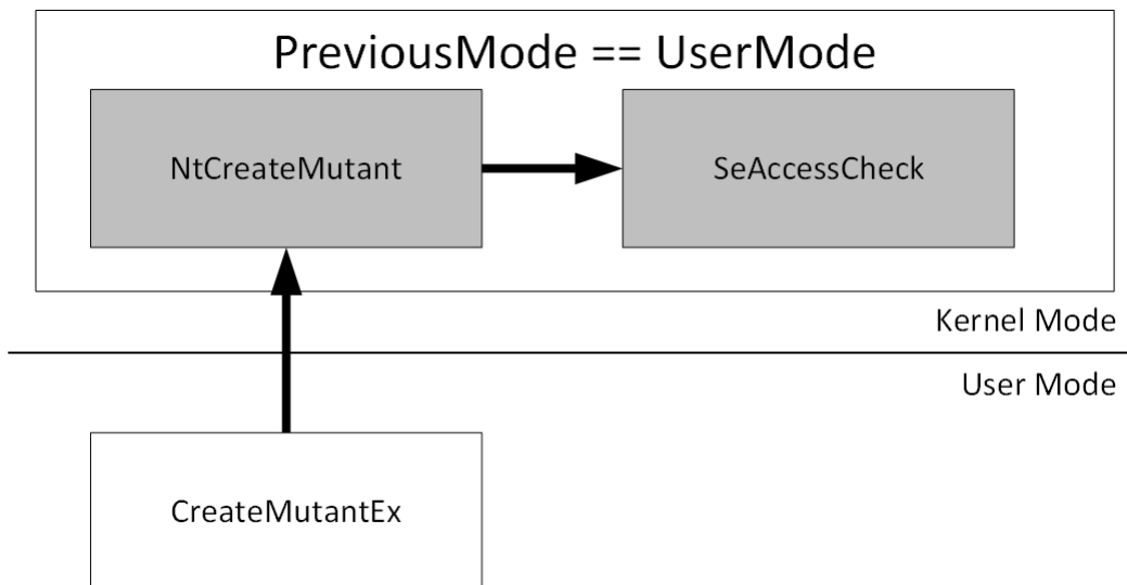
Figure 7-1 A thread's PreviousMode value when calling the NtCreateMutant system call
