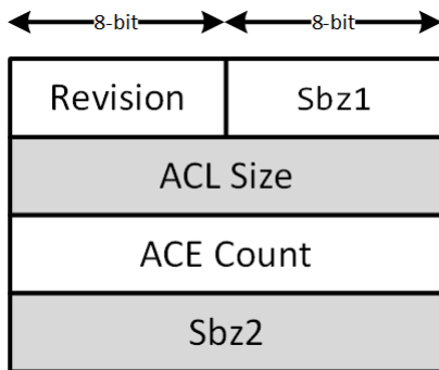
Figure 5-6 The ACL header
