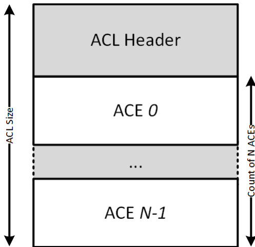
Figure 5-5 A top-level overview of the ACL structure
