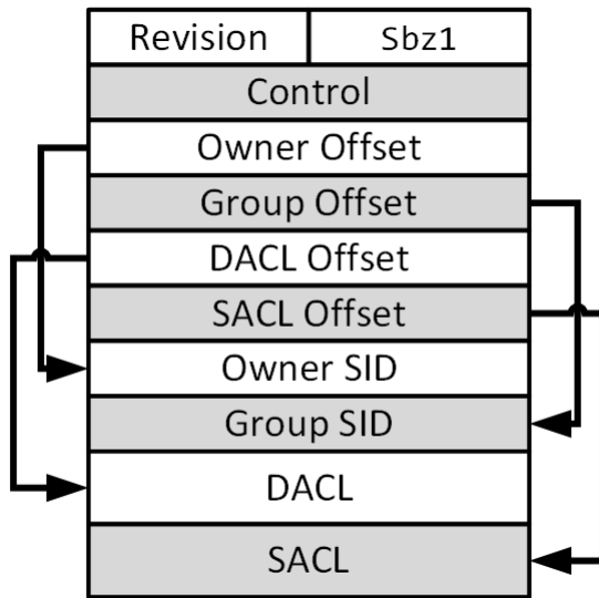
Figure 5-4 An example of a relative security descriptor
