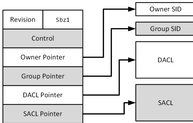
Figure 5-3 The structure of the absolute security descriptor
