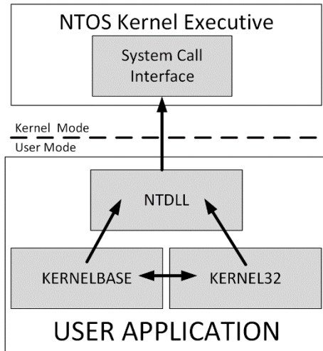
Figure 3-1 The Win32 API modules
