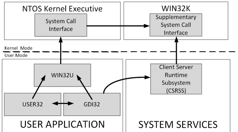
Figure 3-2 The Win32 GUI modules
