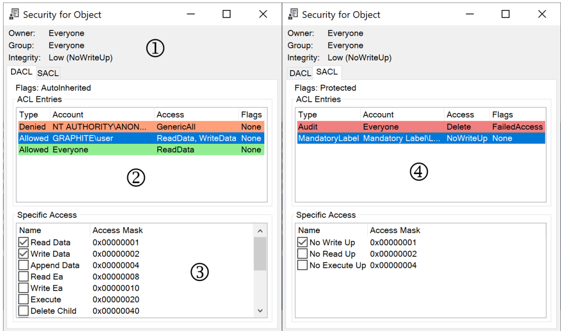
Figure 5-8 A GUI displaying the security descriptor
