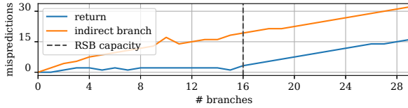
Figure 4: Return instructions behave like indirect branch instructions when reaching the threshold of more than 16 calls.
