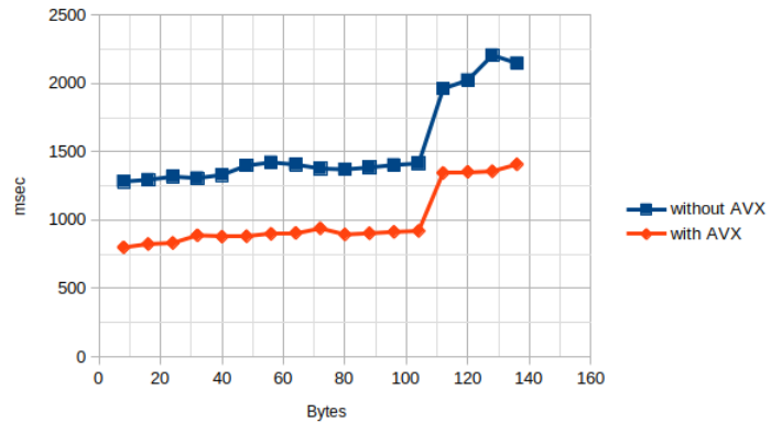
Fig. 2. Dependence of the checksum calculation time on the size of the message being hashed.
