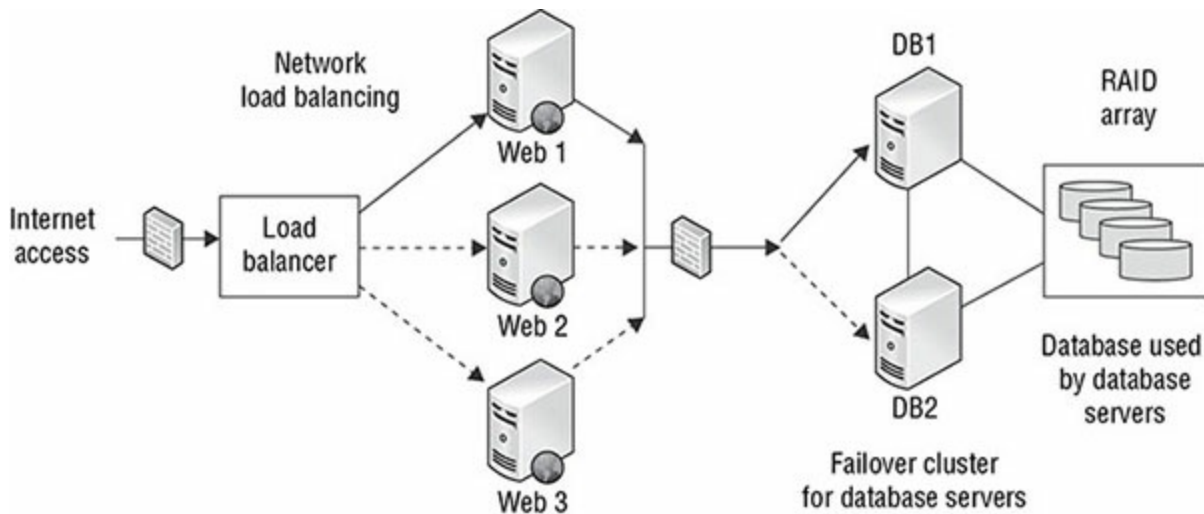
FIGURE 18.2 Failover cluster with network load balancing
