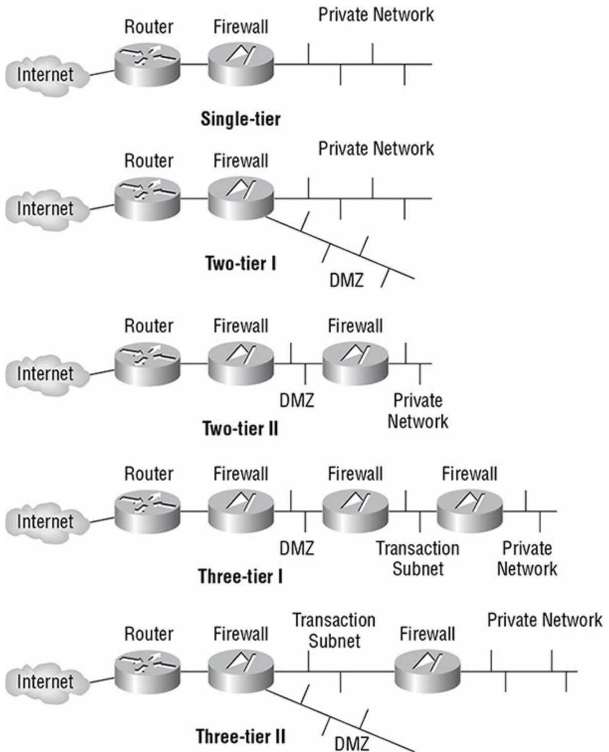
FIGURE 11.8 Single-, two-, and three-tier firewall deployment architectures
