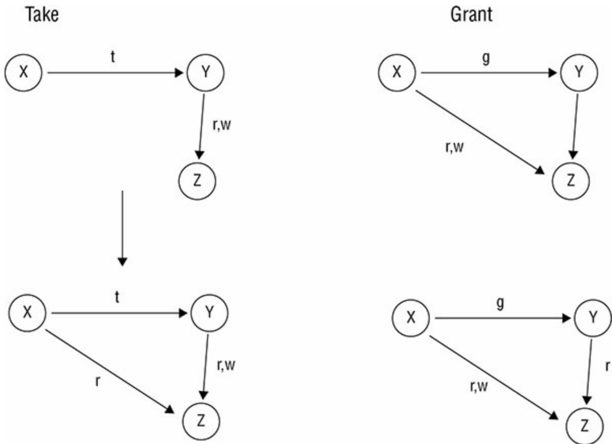
FIGURE 8.2 The Take-Grant model's directed graph
