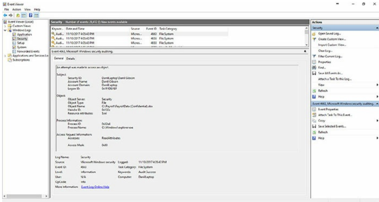
FIGURE 17.5 Viewing a log entry
