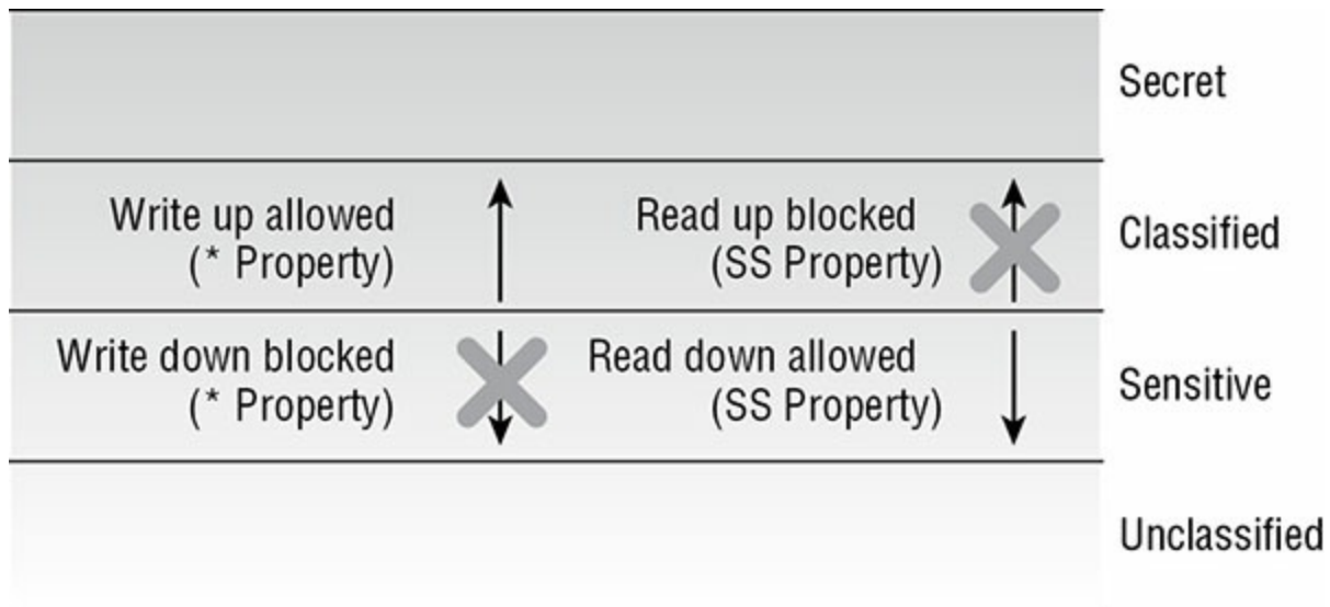
FIGURE 8.3 The Bell-LaPadula model
