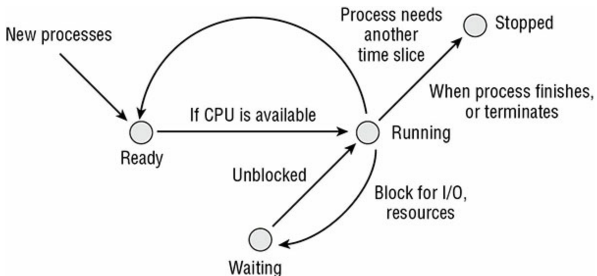
FIGURE 9.2 The process scheduler
