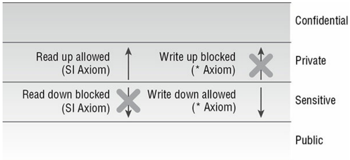
FIGURE 8.4 The Biba model
