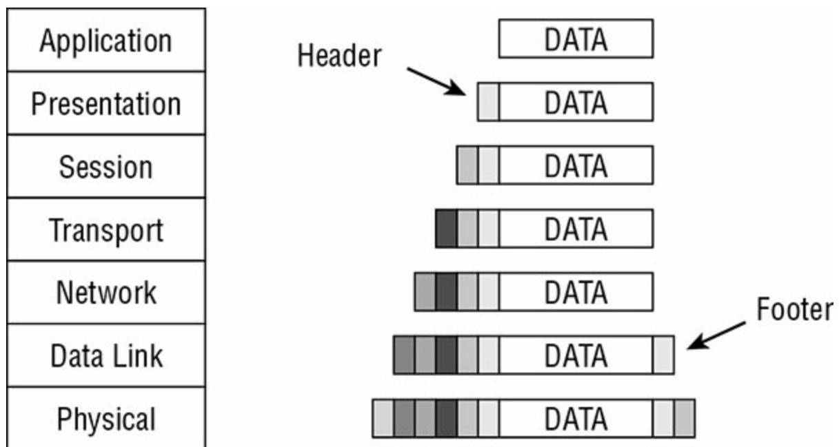
FIGURE 11.2 Representation of OSI model encapsulation
