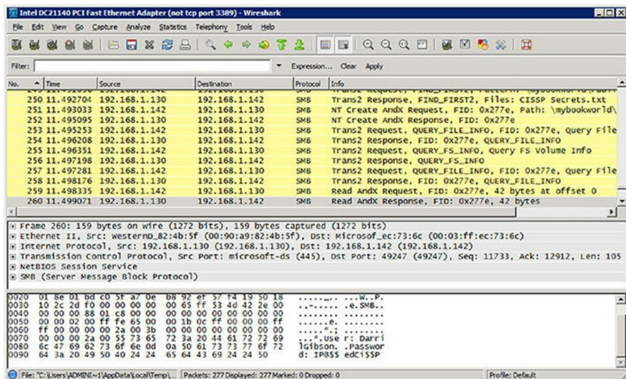
FIGURE 14.4 Wireshark capture
