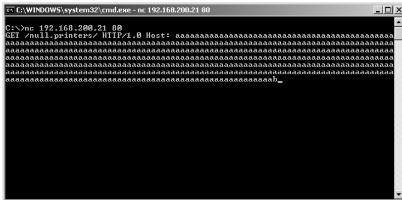
Figure 14-5 Using NetCat
