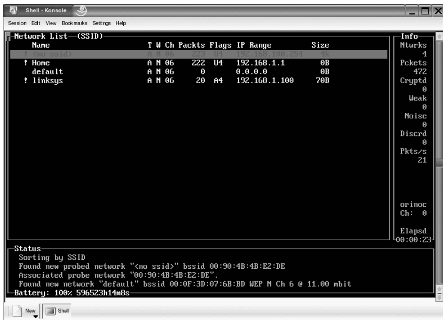
Figure 11-2 Kismet
