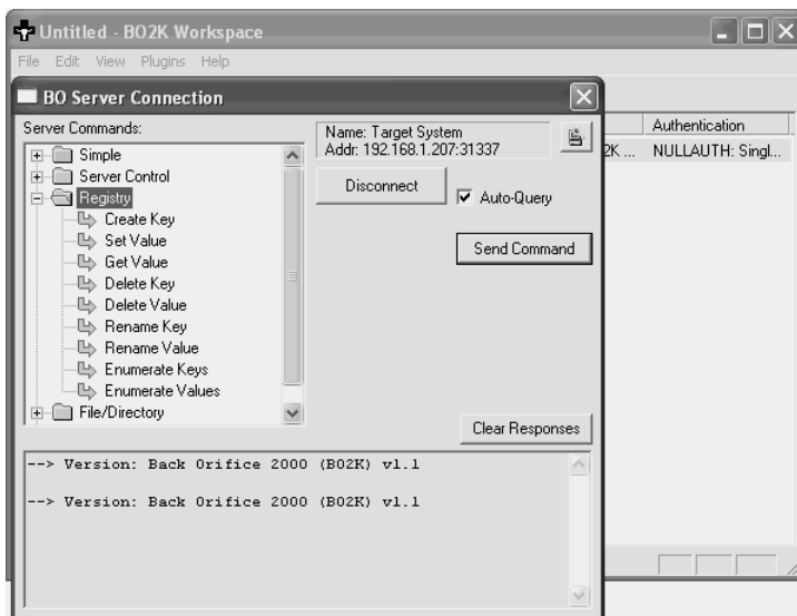
Figure 12-13 BO Registry Control
