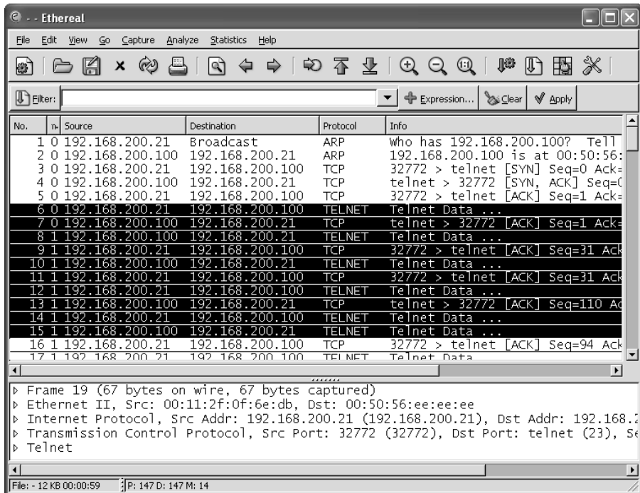
Figure 6-22 Ethereal: Normal Telnet Data
