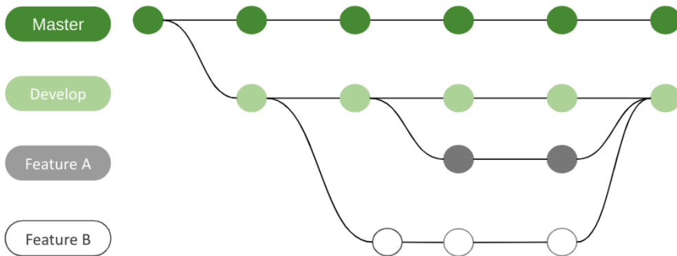
Figure 2.9 – Git feature branch workflow with a Develop branch
