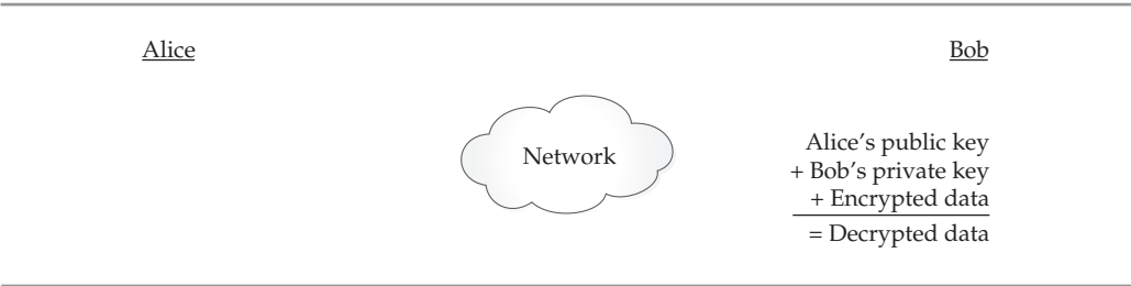
Figure 21-5. Bob uses Alice's public key, along with his private key, to verify and decrypt the data, respectively.
