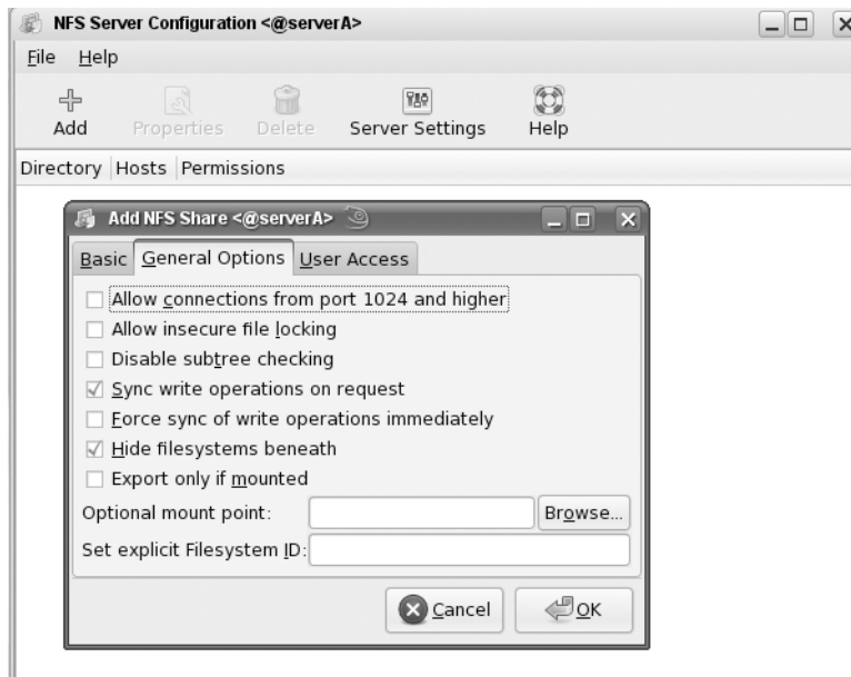
Figure 22-1. NFS server configuration utility
