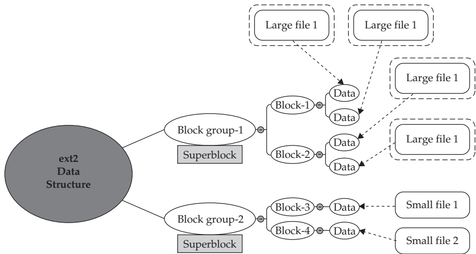
Figure 7-2. Data structure on ext2 file systems
