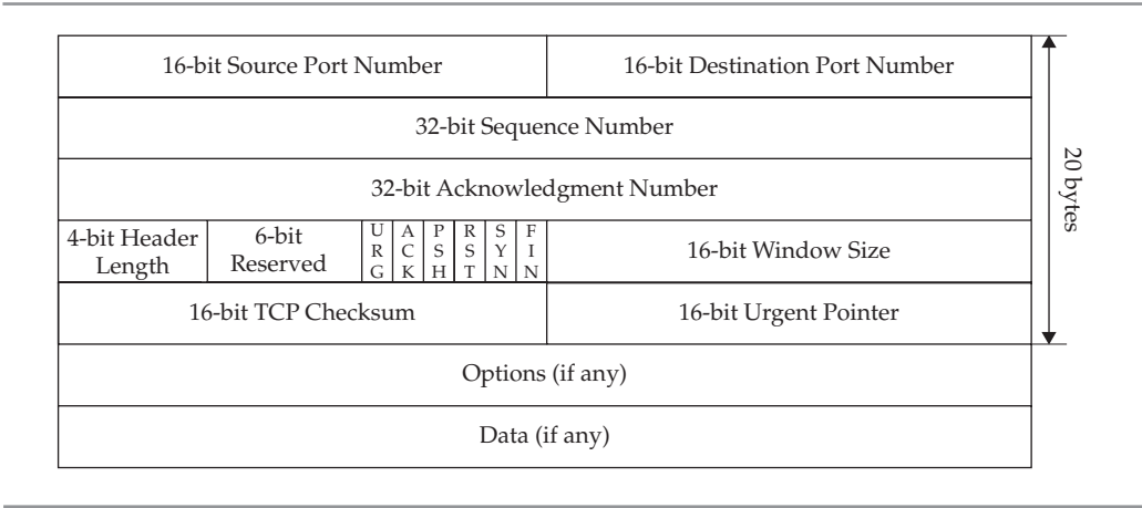
Figure 11-6. The TCP header
