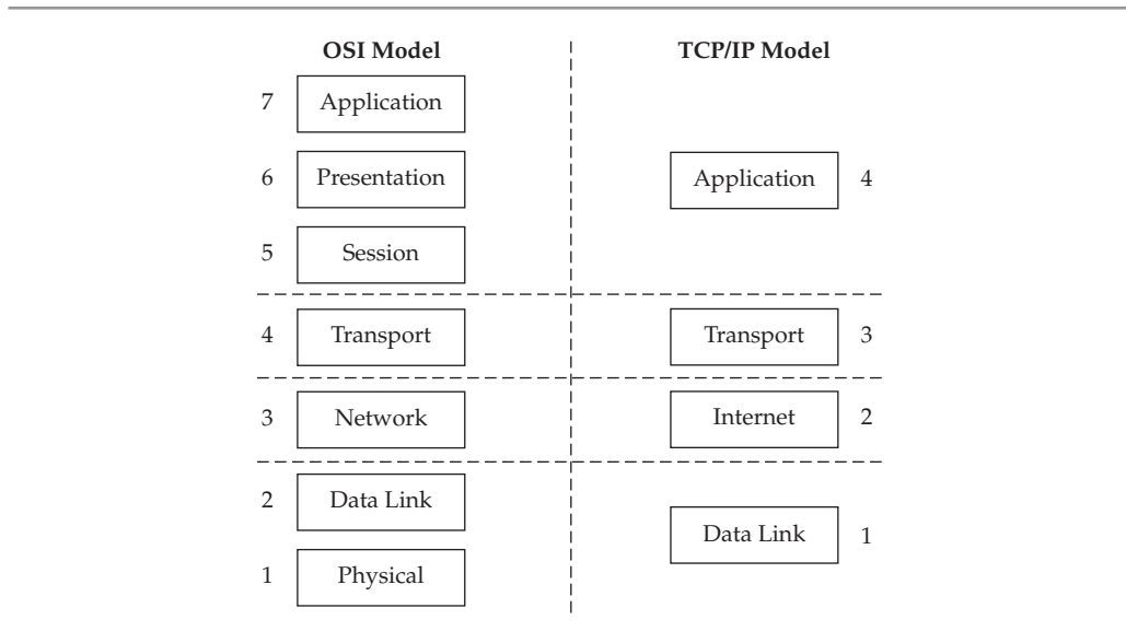
Figure 11-3. The OSI reference model and the TCP/IP model
