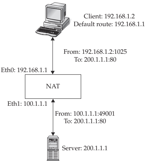
Figure 13-1. Using SNAT on a connection
