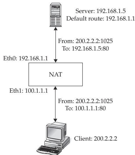
Figure 13-2. Using DNAT on a connection
