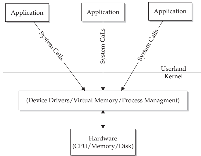
Figure 9-1. A visual representation of how the Linux kernel fits into a complete system
