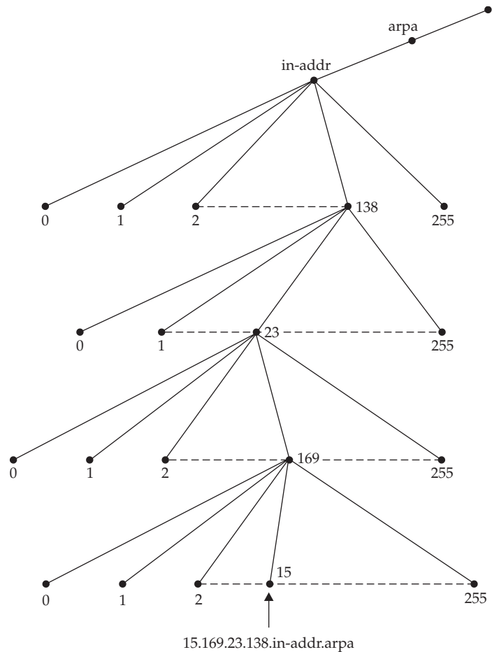
Figure 16-4. Reverse DNS resolution of 138.23.169.15
