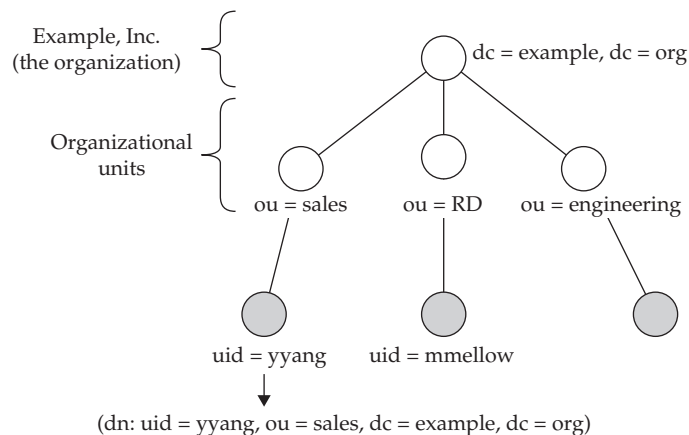
Figure 26-1. LDAP tree for example.org
