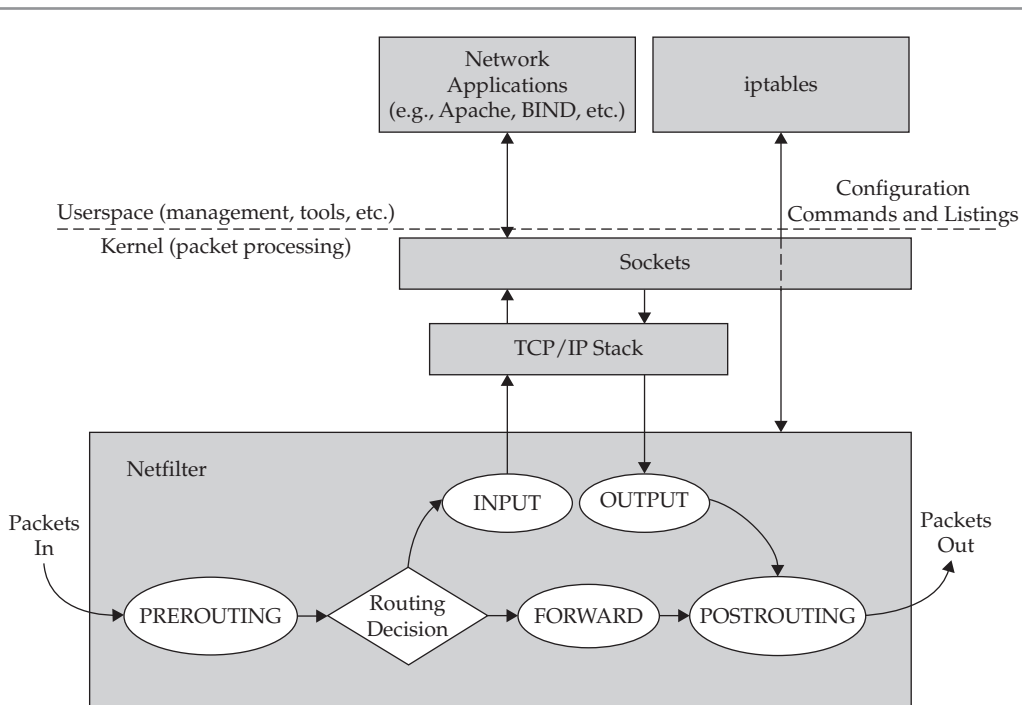
Figure 13-3. The relationship between the predefined chains in Netfilter
