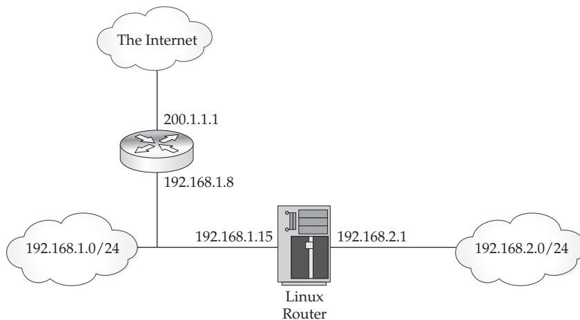
Figure 12-1. Our sample network
