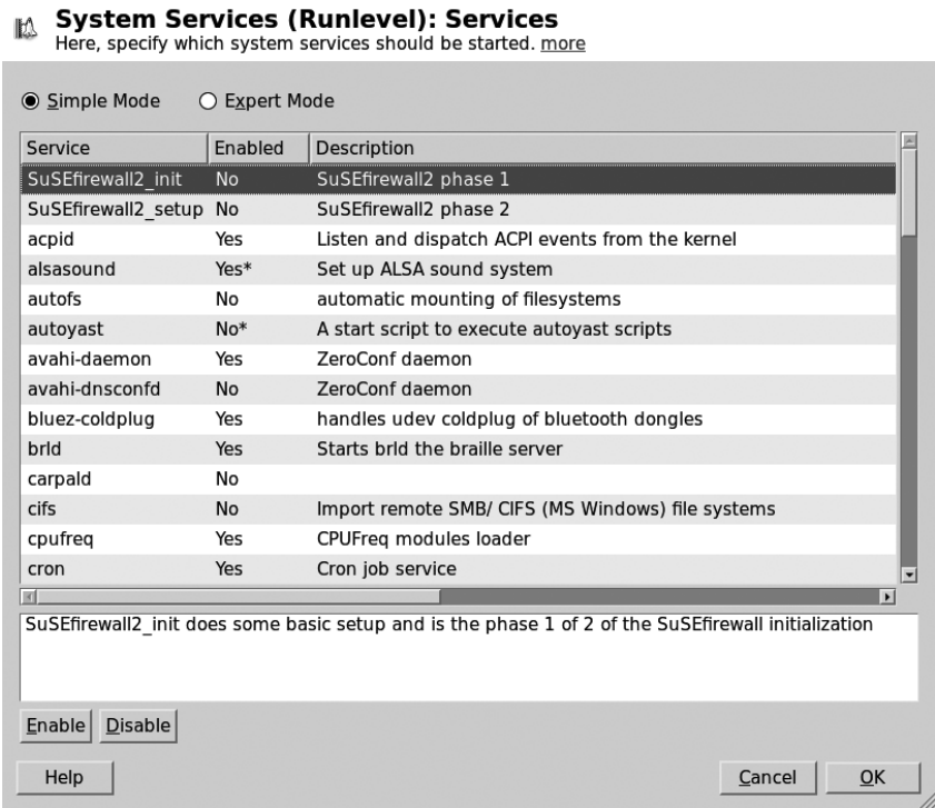
Figure 6-2. openSUSE’s System Services (Runlevel) editor
