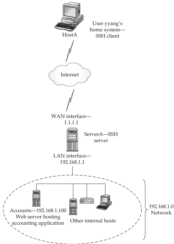
Figure 21-6. Port forwarding with SSH
