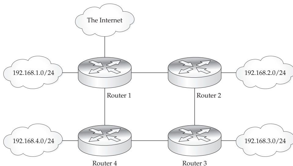
Figure 11-10. A small campus network using RIP
