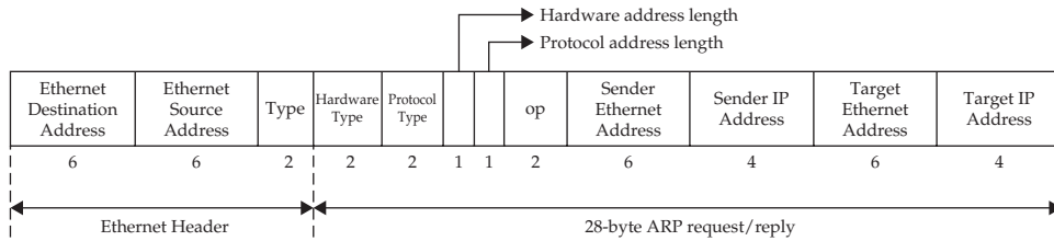
Figure 11-8. The ARP packet header
