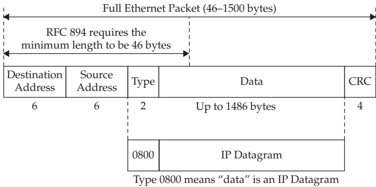
Figure 11-4. The Ethernet header
