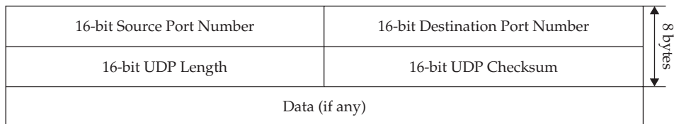
Figure 11-7. The UDP packet header
