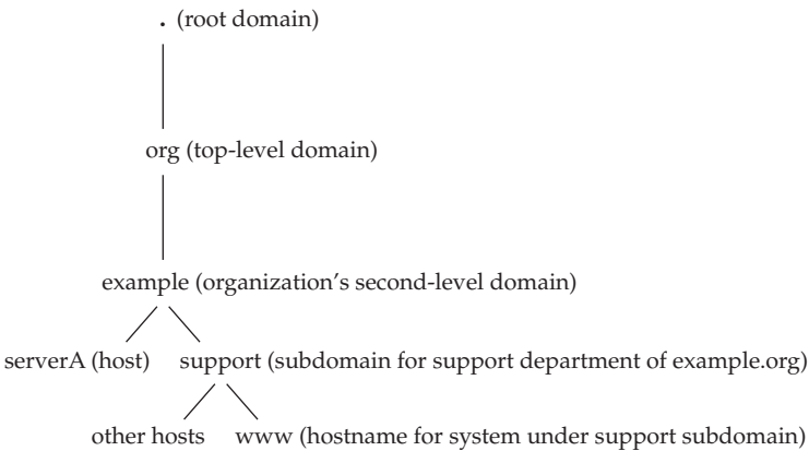
Figure 16-3. Concept of subdomains
