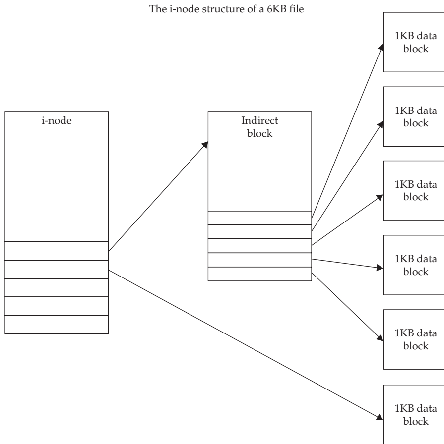
Figure 7-1. The i-nodes and data blocks in the ext2 file system
