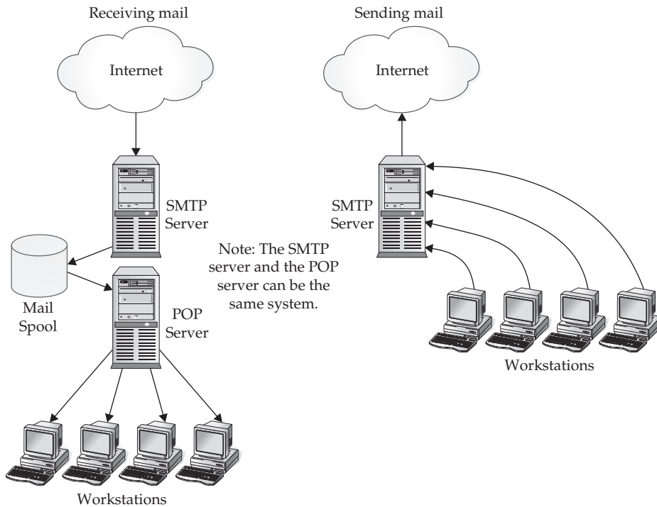
Figure 20-1. Sending and receiving mail with SMTP and POP
