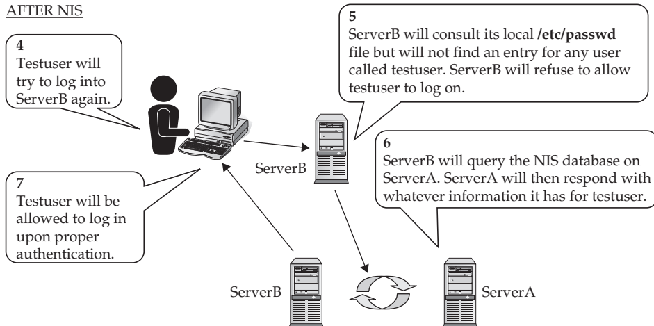
Figure 25-1. Before and after NIS
