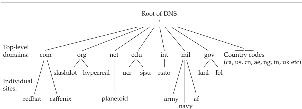
Figure 16-2. The DNS tree, two layers deep
