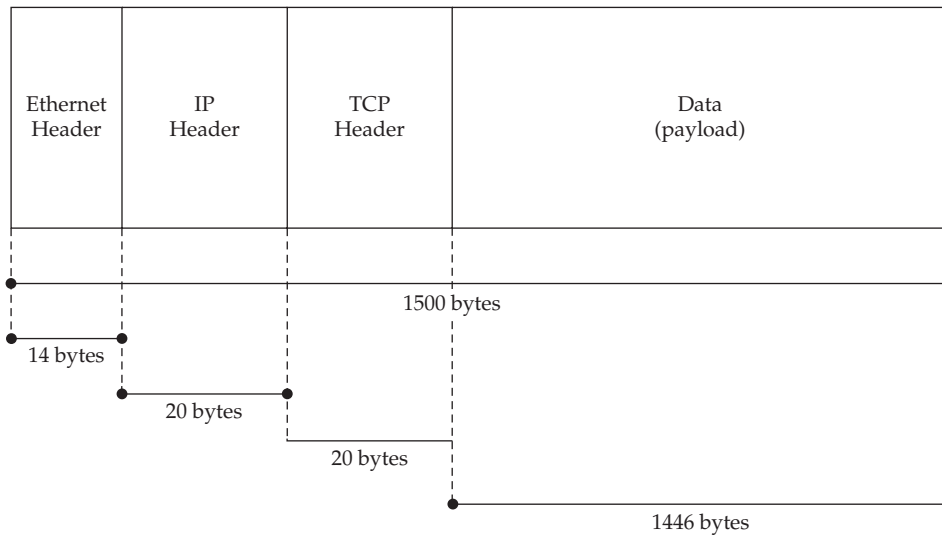
Figure 11-1. A TCP/IP packet on an Ethernet network
