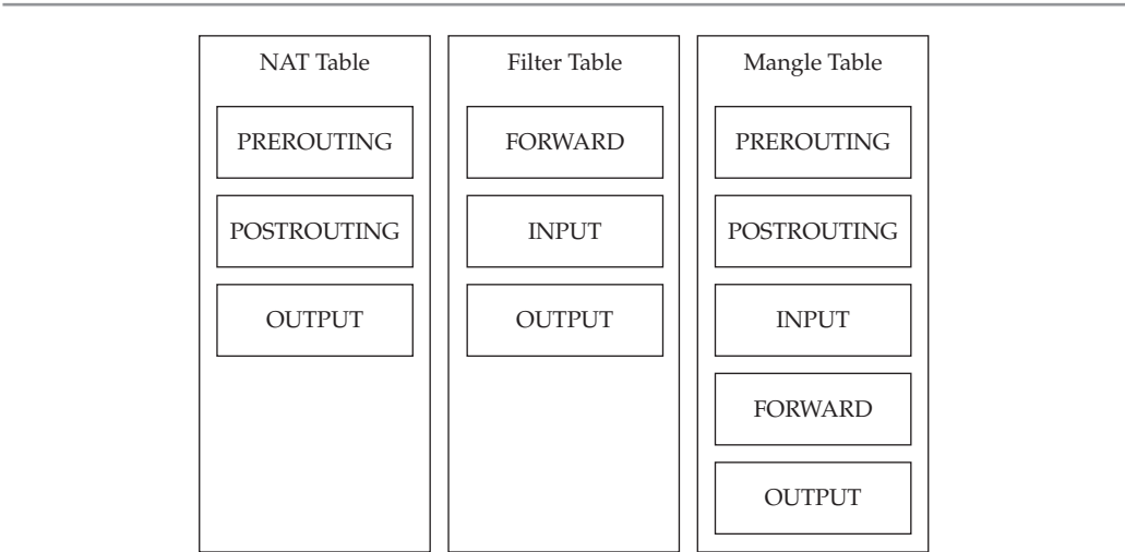
Figure 13-4. The relationship among predefined chains and predefined tables
