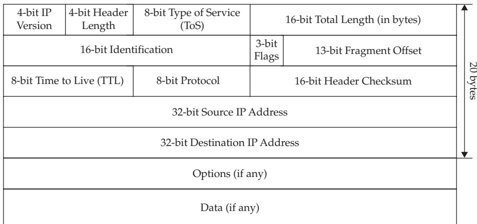
Figure 11-5. The IP header
