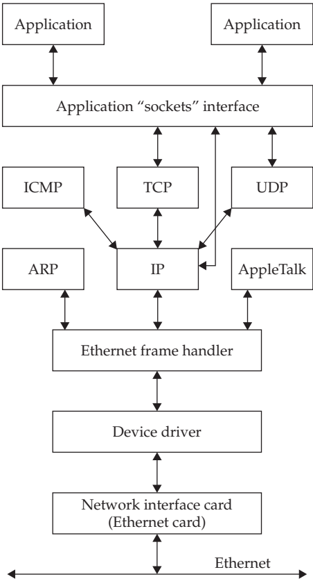
Figure 11-2. The path of a packet through the Linux networking stack
