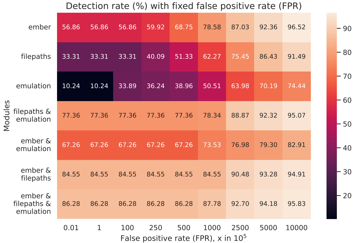
Figure 3. Detection rate (%) on out-of-sample test set with fixed false positive rate based on different combinations of enabled modules in hybrid solution.
