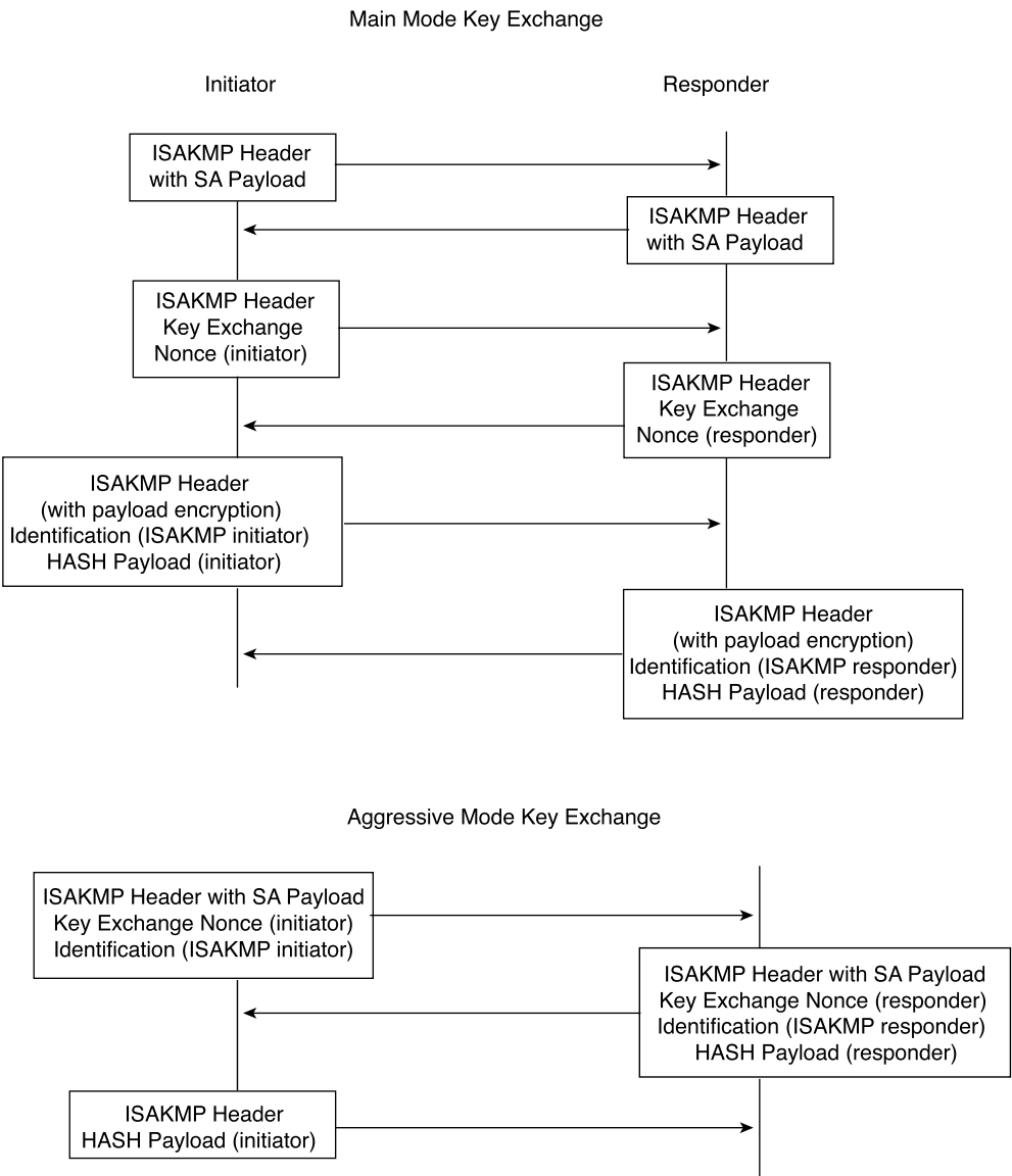
Figure 10-5 Key Exchanges
