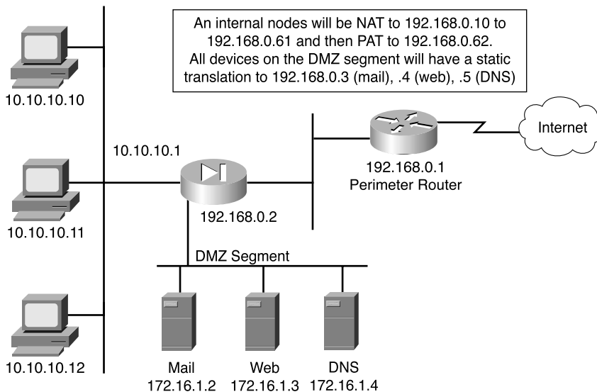
Figure 5-7 Combined NAT, PAT, and Static Translation
