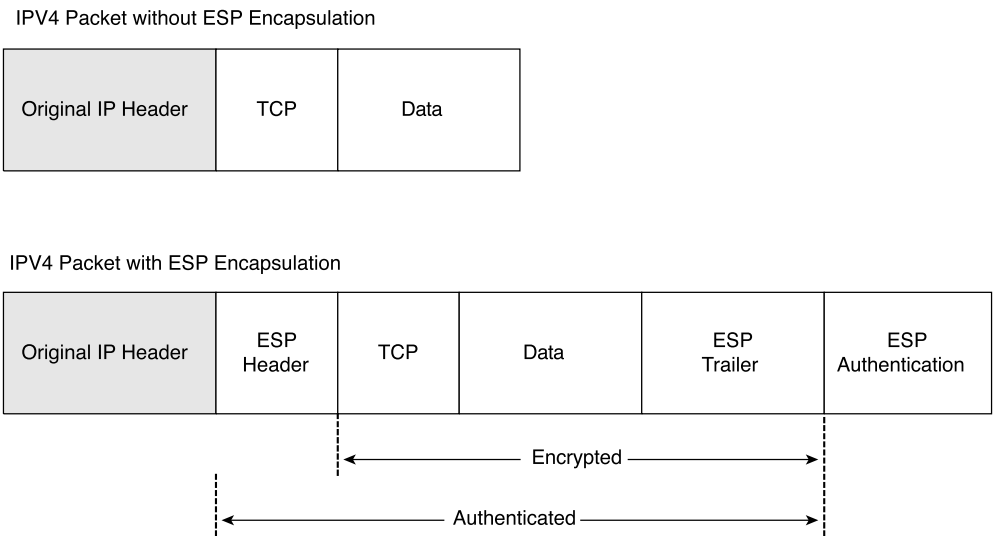
Figure 10-3 ESP Encapsulation
