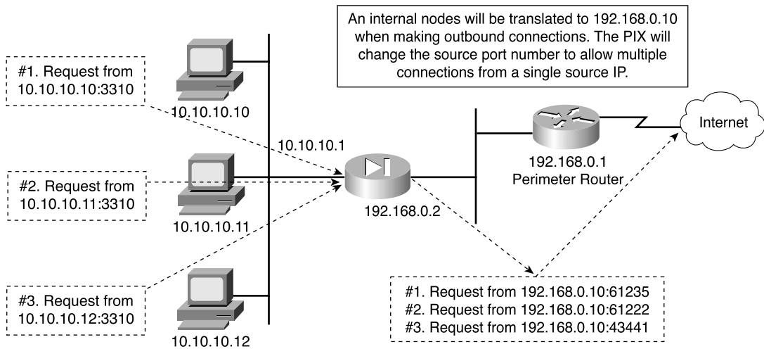
Figure 5-5 Port Address Translation
