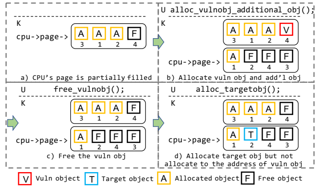
Figure 8: UAF and DF vulnerability exploitation failure case
