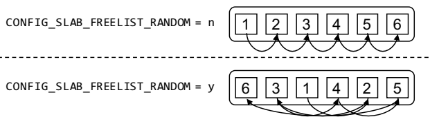
Figure 3: Mechanism of slab freelist random
