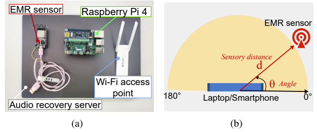
Fig. 14. (a) The eavesdropping system of Periscope . (b) The definition of EMR sensor’s relative position to the target device.
