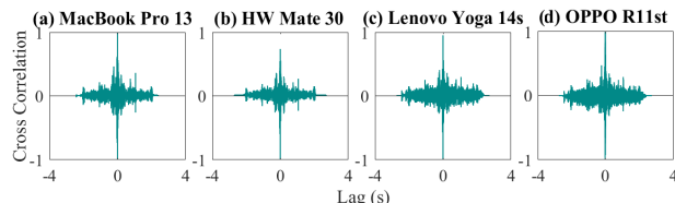
Fig. 4. Sharp peaks appear when lag = 0 indicating the strong correlations between the original audios and the device’s EMR measures.
