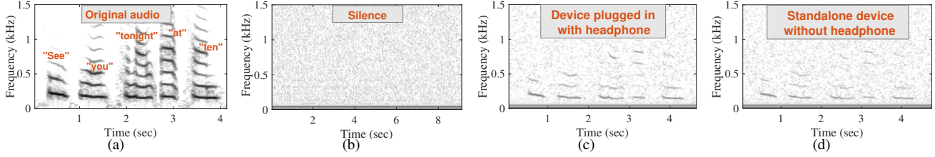
Fig. 6. Comparisons of EMR measurements when the device is connected w/o headphones. (a) Spectrogram of the original audio. (b) EMR measures when the device is in silence. (c) EMR measures of the device plugged in with headphones. (d) EMR measures of the standalone device.
