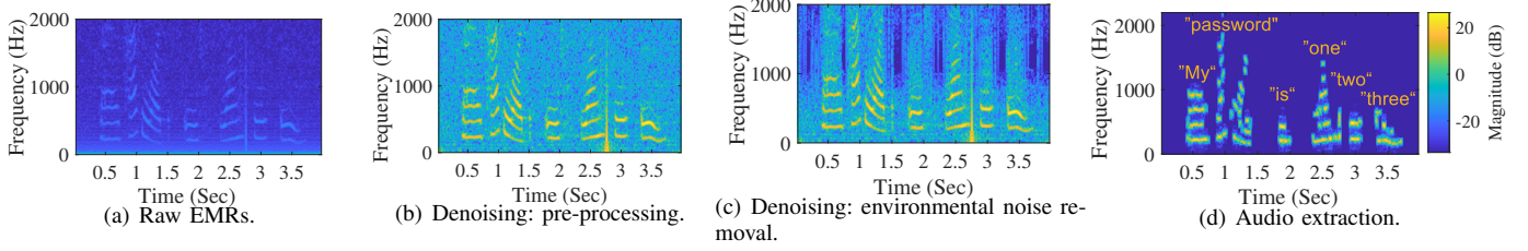
Fig. 10. Intermediate results of audio recovery procedures (The speech is “my password is one two three”).
