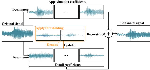
Fig. 11. Signal denoise with Discrete Wavelet Transform.
