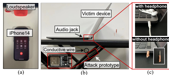
Fig. 3. We use iPhone 14 to call the target devices via Skype. The EMR sensory prototype collects the victim device’s EMRs when it is processing the audio.
