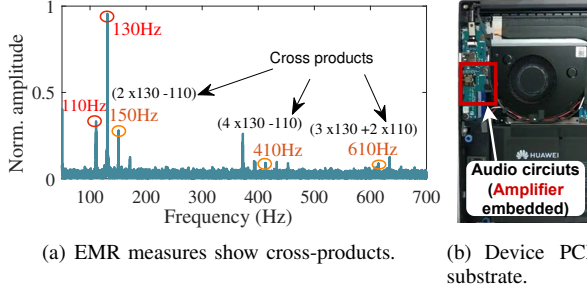
Fig. 7. Amplifier induces cross-products which are traced in EMR measures. (tested on MateBook D14).
