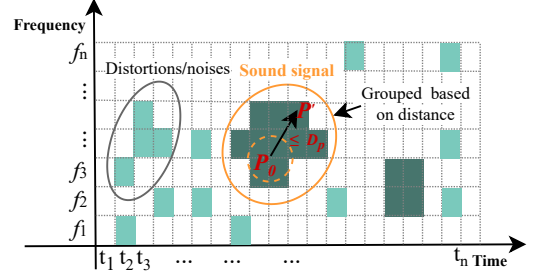
Fig. 12. DBSCAN extracts audio components from the EMR’s STFT spectrogram: STFT bins (points) within the orange circle representing the audio signal.
