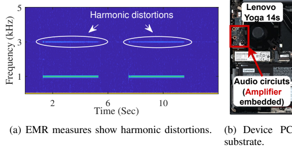
Fig. 8. Amplifier induces harmonics. The 1kHz fundamental frequency results in the 3kHz harmonic. (tested on Lenovo Yoga14s).
