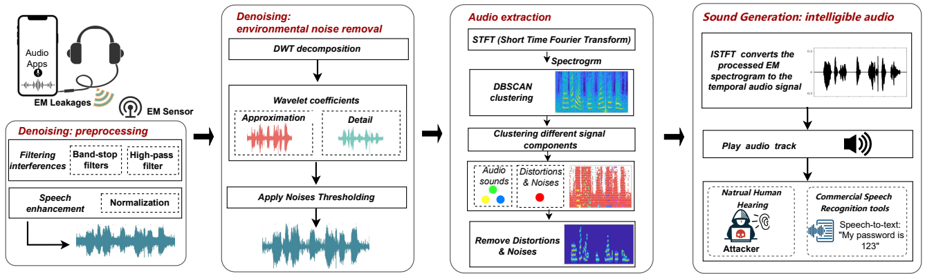
Fig. 9. Framework of Audio Recovery.
