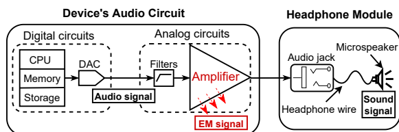
Fig. 2. The workflow of mobile device’s audio circuit when connected with a wired headphone.
