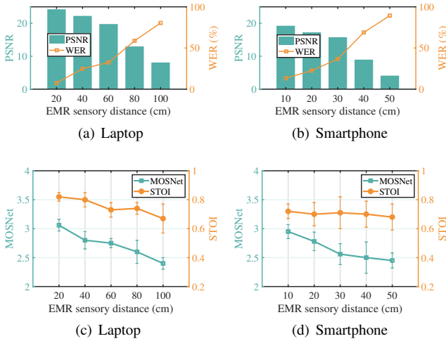
Fig. 18. Impact of EMR sensory distance.
