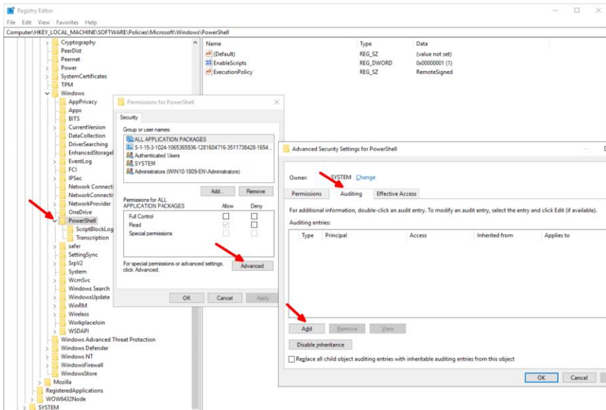
Editing the SACL for registry keys under PowerShell
