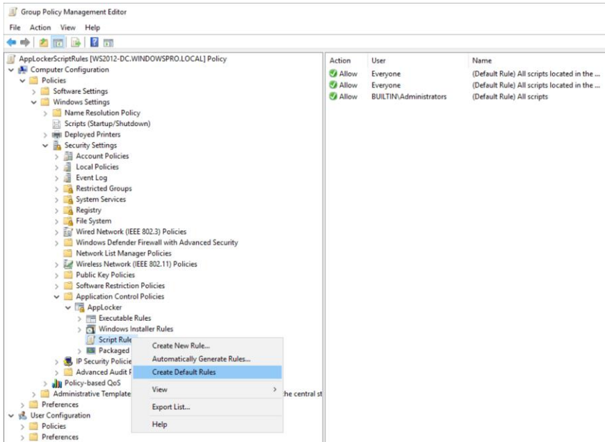
Creating default rules for scripts in AppLocker
