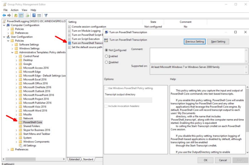
Enabling Transcription Logging for PowerShell 7 via Group Policy
