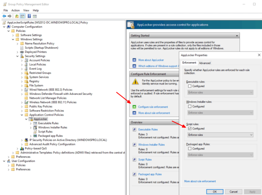
Enabling rule enforcement for scripts in AppLocker
