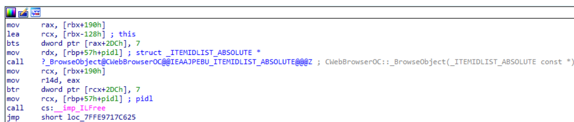
Figure 1: ID list from ShellLink structure is passed to CWebBrowserOC::BrowseObject()
