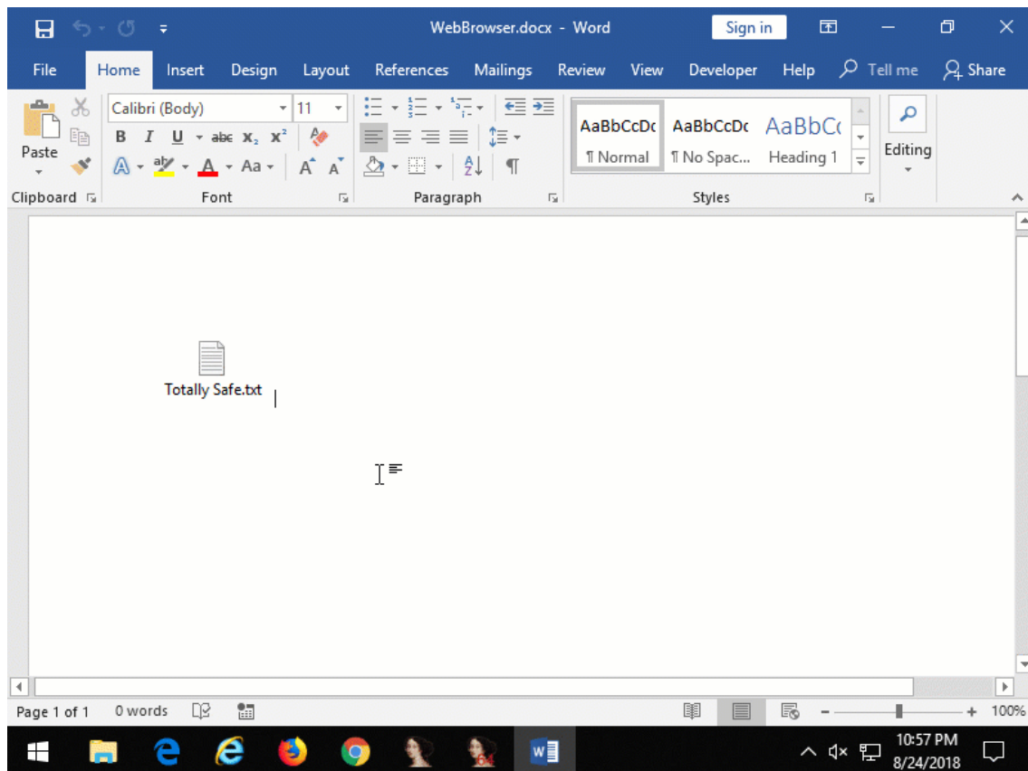
Figure 5: embedded Internet Explorer that opens an Internet Shortcut file from a remote website that launches Calculator
