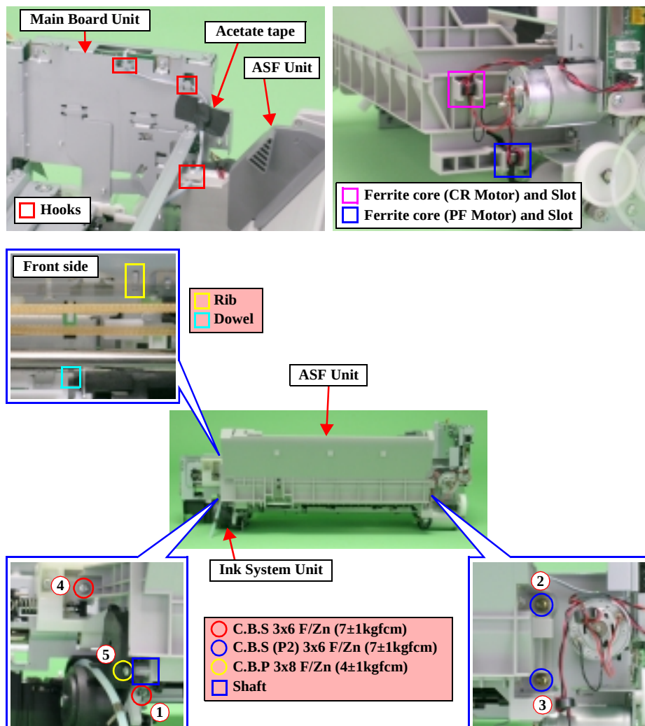
Figure 4-29. ASF Unit Removal (1)
