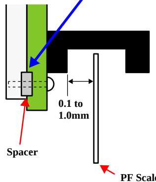
Figure 4-25. PF Scale Sensor positioning adjustment
