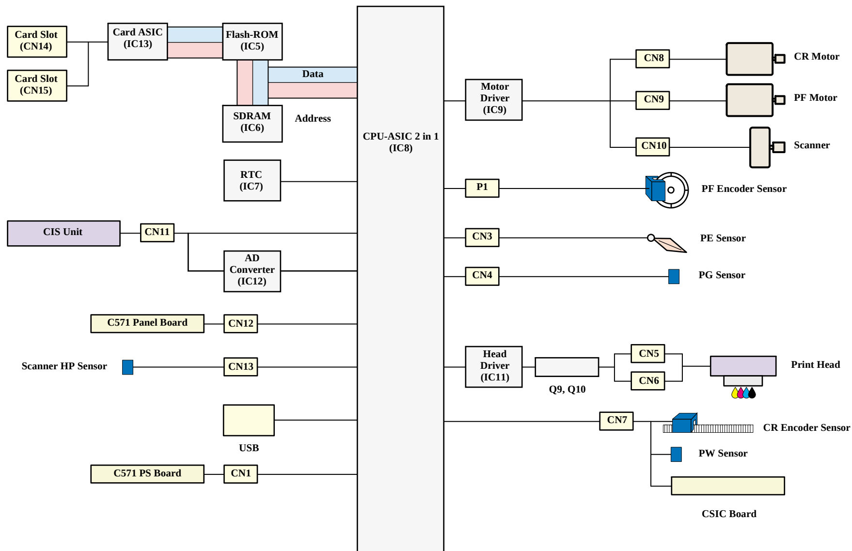
Figure 2-18. Block Diagram For The C579 Main Board
