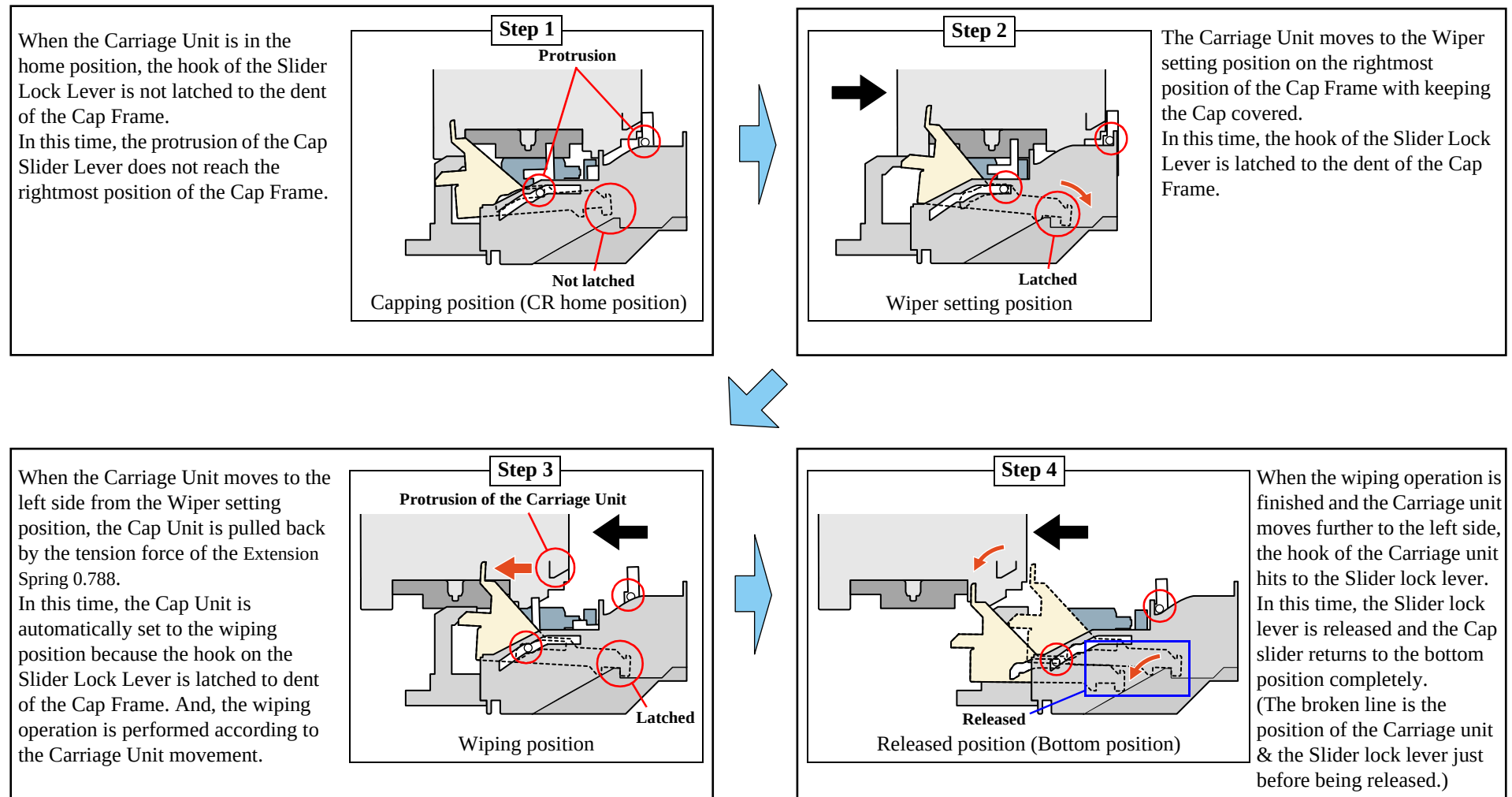
Figure 2-10. Wiper mechanism
