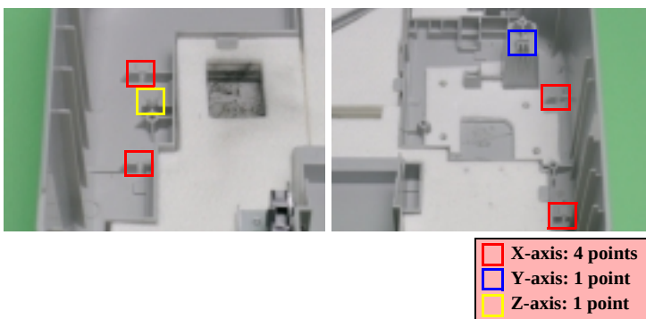
Assembled standard position of Printer Mechanism
