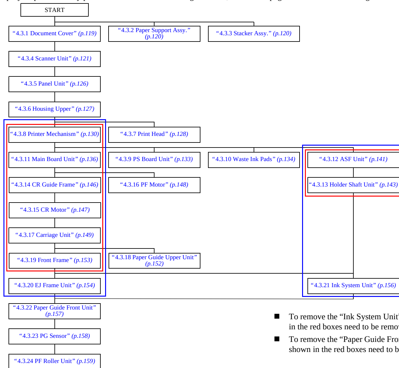
Figure 4-1. Disassembling flowchart
