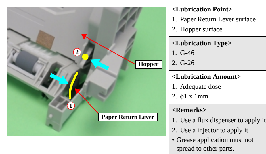
Figure 6-5. Lubrication
