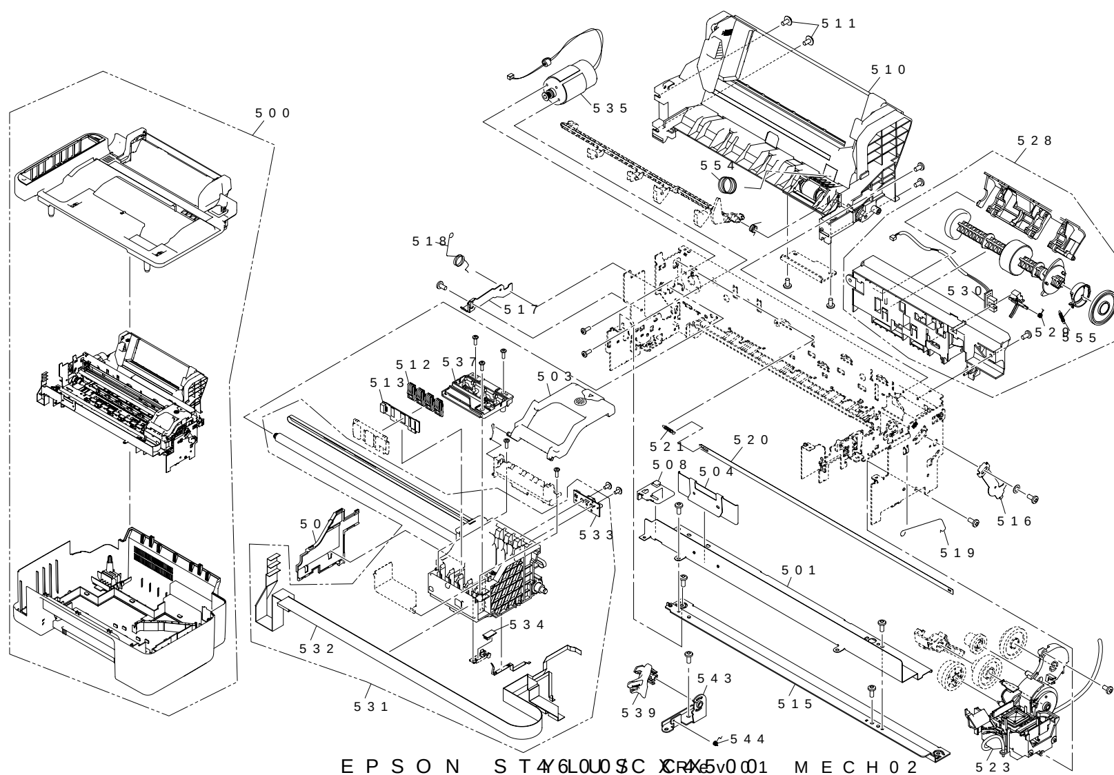
EPSON STYLUS CX3500/CX3600/CX3650/CX4500/CX4600 MECH 02 Figure 7-12. Stylus CX3500/CX3600/CX3650/CX4500/CX4600 Exploded Diagram 4
