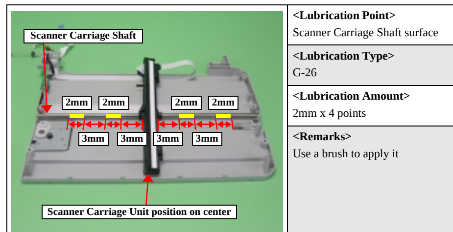
Figure 6-4. Lubrication
