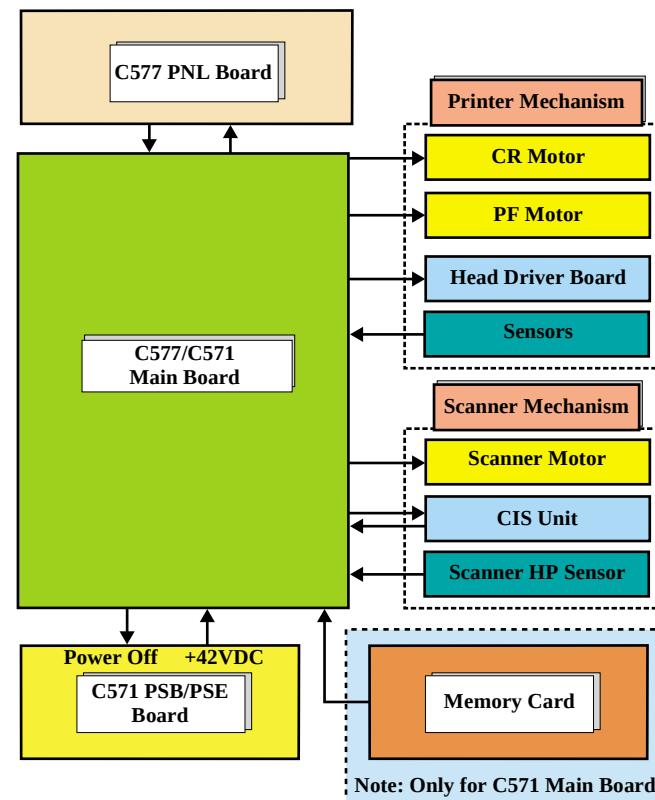
Figure 2-17. Electric circuit
