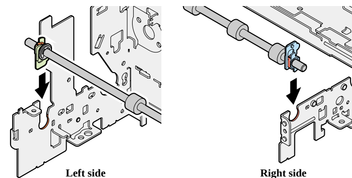
Figure 4-45. Installation of Bush 5
