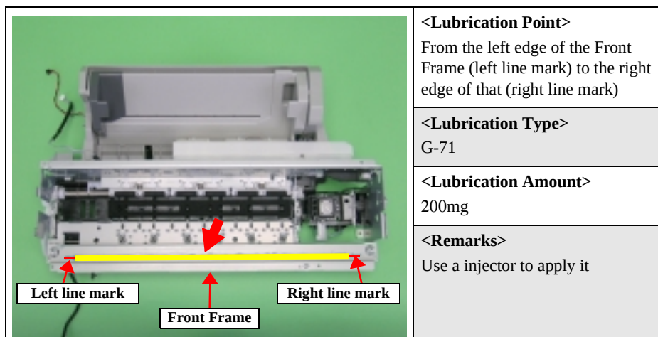
Figure 6-10. Lubrication
