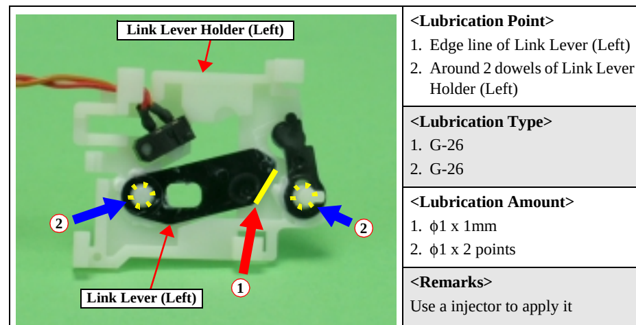
Figure 6-11. Lubrication
