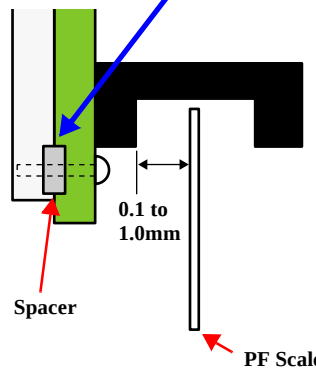
Figure 4-28. PF Scale Sensor positioning adjustment
