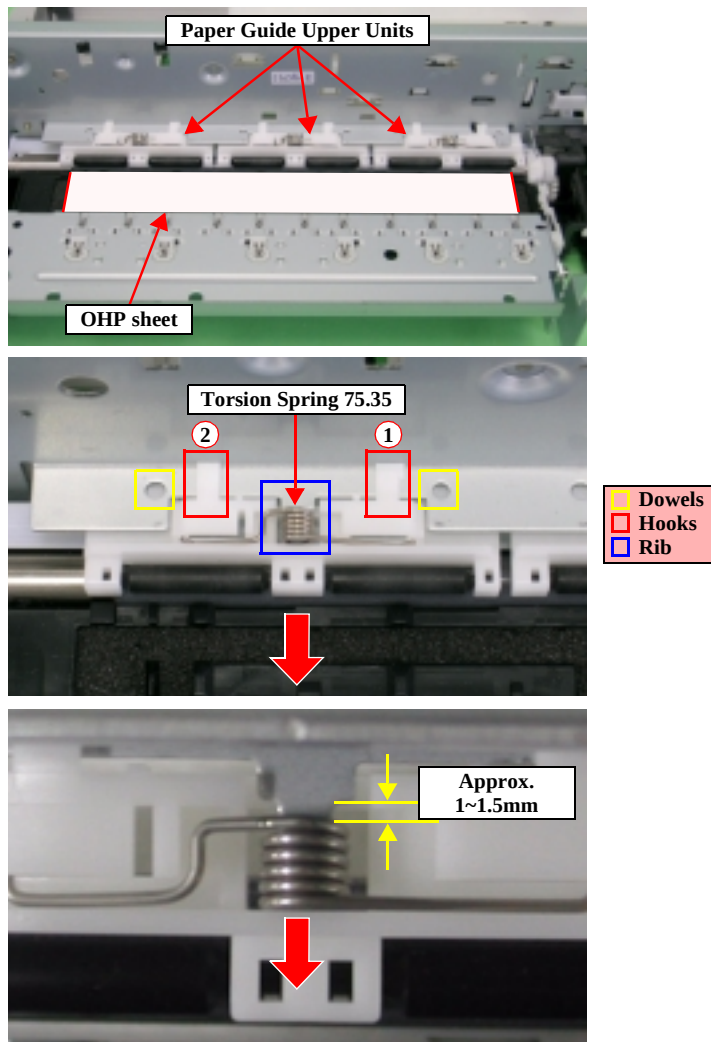
Figure 4-42. Paper Guide Upper Unit Removal
