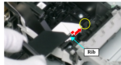
Figure 4-16. Installation of Sub FFC Guide
