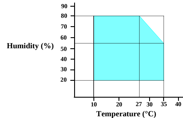
Figure 1-8. Temperature/Humidity range
