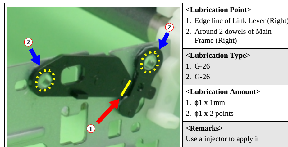
Figure 6-12. Lubrication
