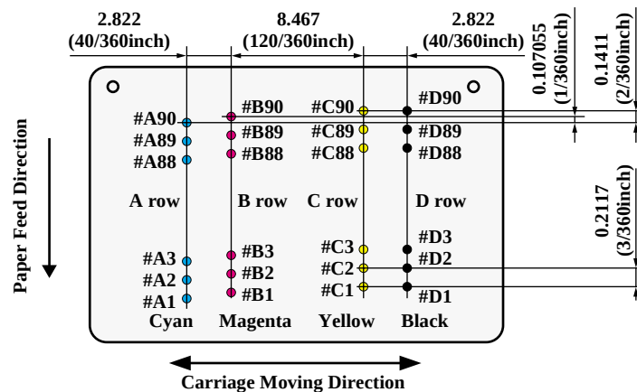
Figure 1-2. Nozzle configuration
