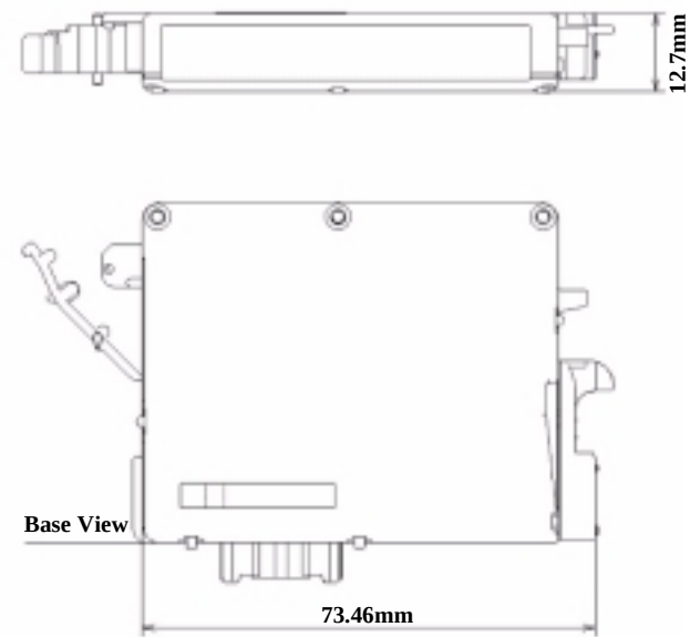
Figure 1-6. Ink cartridge
