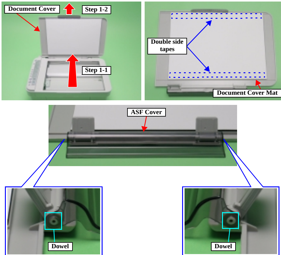
Figure 4-2. Document Cover Removal
