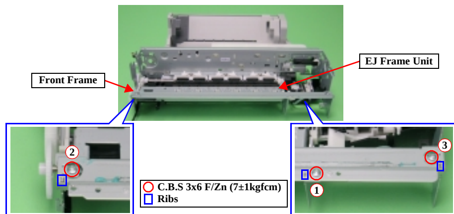
Figure 4-43. Front Frame Removal
