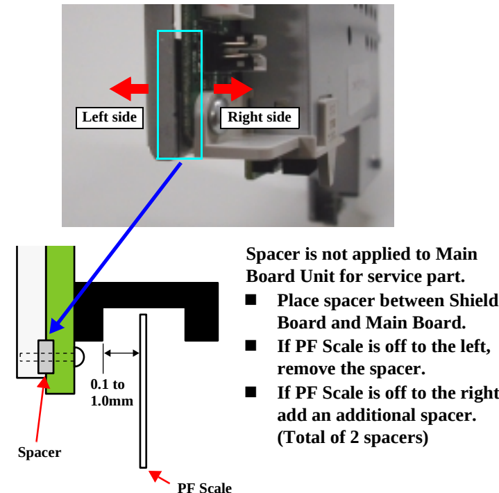
Figure 5-17. PF Scale Sensor positioning adjustment
