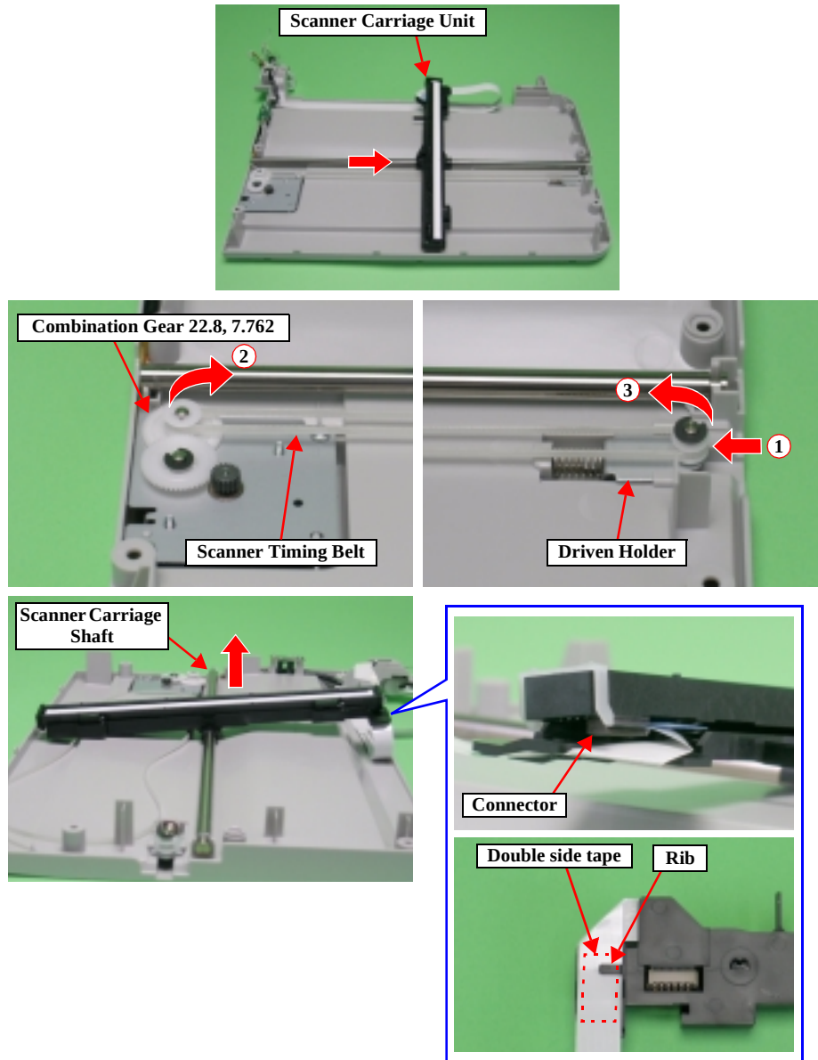
Figure 4-8. Scanner Carriage Unit Removal (1)
