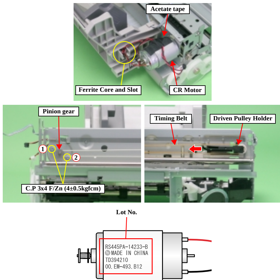
Figure 4-37. CR Motor Removal
