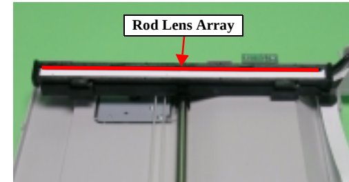
Figure 4-9. Handling of Scanner Carriage Unit
