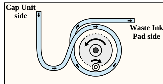
Figure 2-11. Pump mechanism
