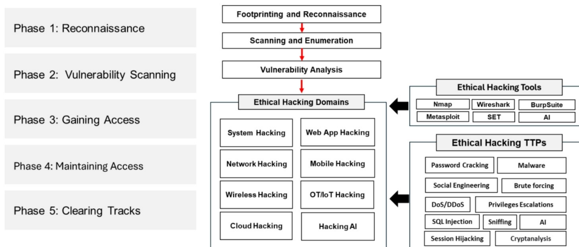
Figure 1.3: EC-council's CEH ethical hacking framework
