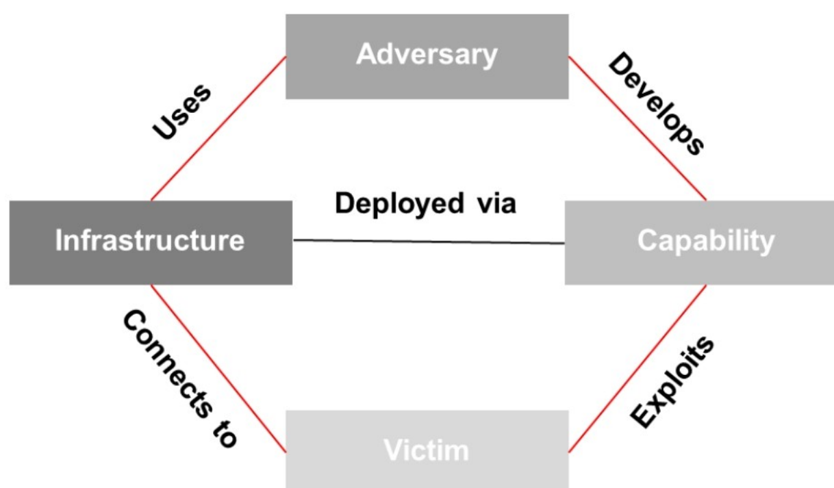
Figure 1.6: Meta features of the Diamond Model
