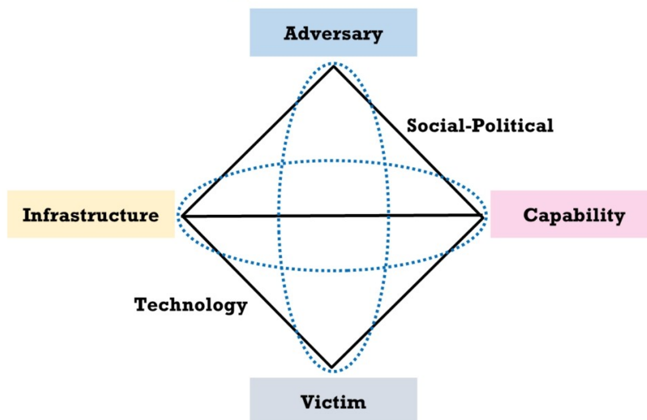
Figure 1.7: Extended Diamond Model of Intrusion Analysis
