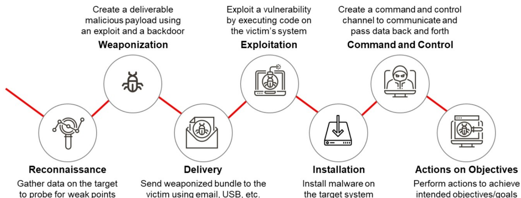
Figure 1.4: Cyber kill chain methodology
