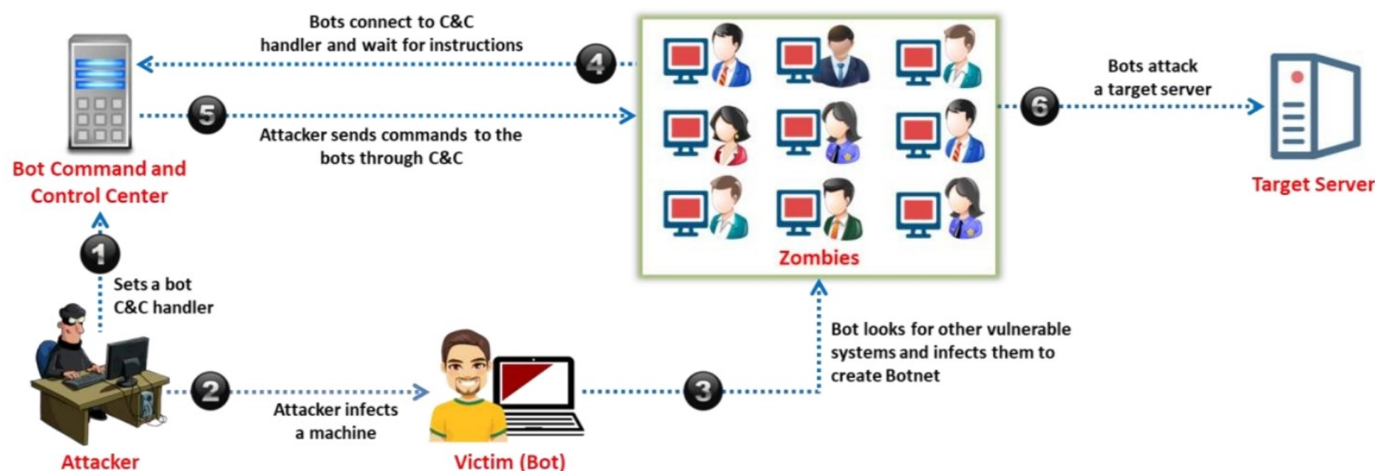
Figure 10.4: Botnet-based DDoS attack
