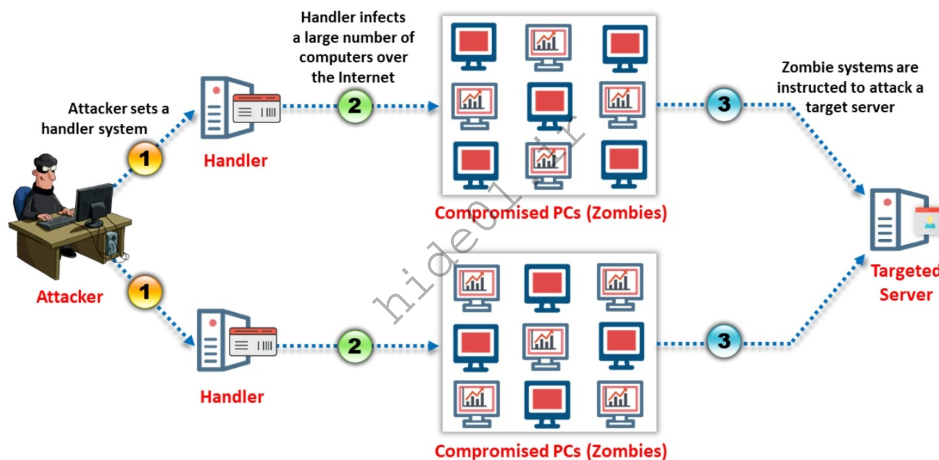
Figure 10.2: Schematic of a DDoS attack
