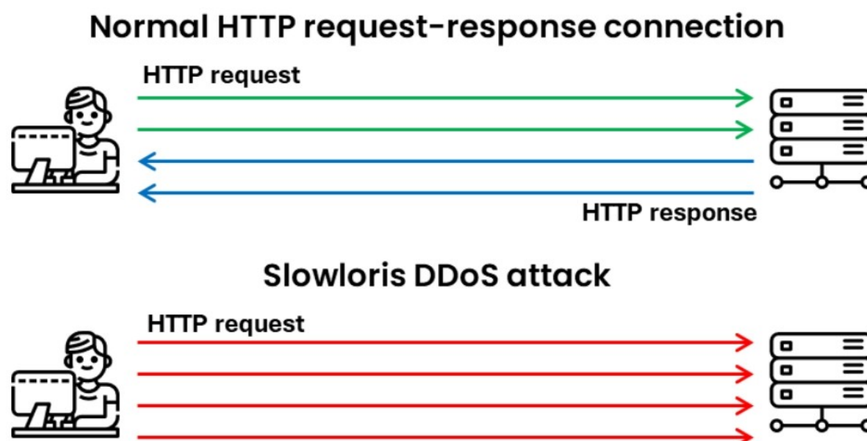
Figure 10.24: Slowloris attack
