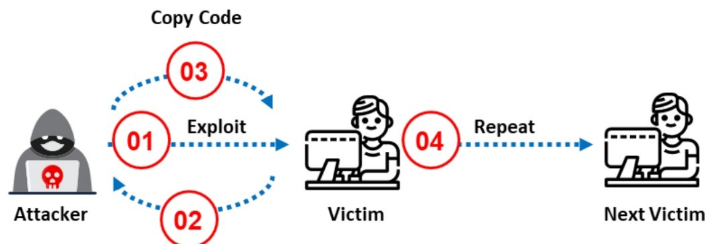
Figure 10.8: Back-chaining propagation
