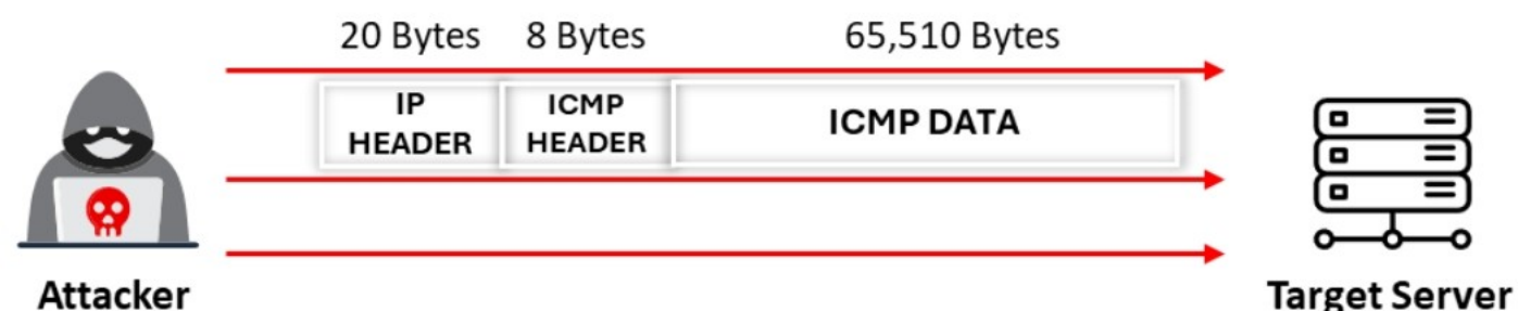
Figure 10.16: Ping-of-death attack
