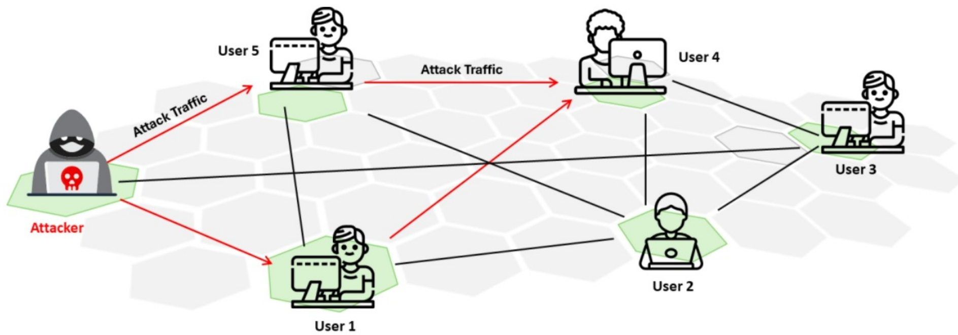
Figure 10.26: Peer-to-peer attack
