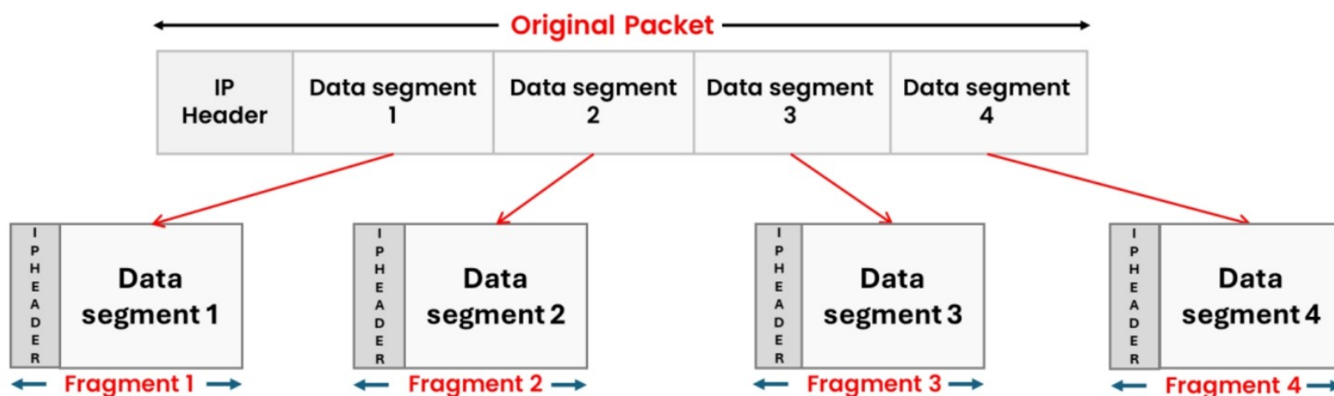
Figure 10.22: Fragmentation attack
