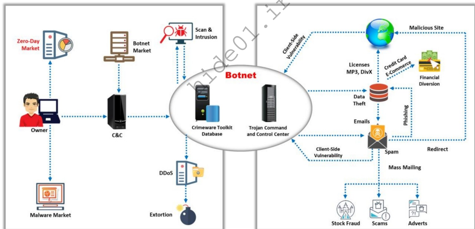
Figure 10.6: Botnet ecosystem
