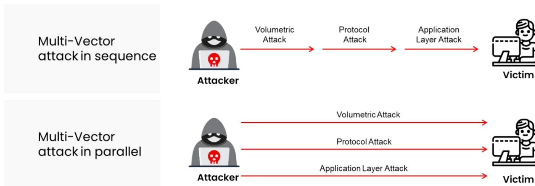
Figure 10.25: Multi-vector attack
