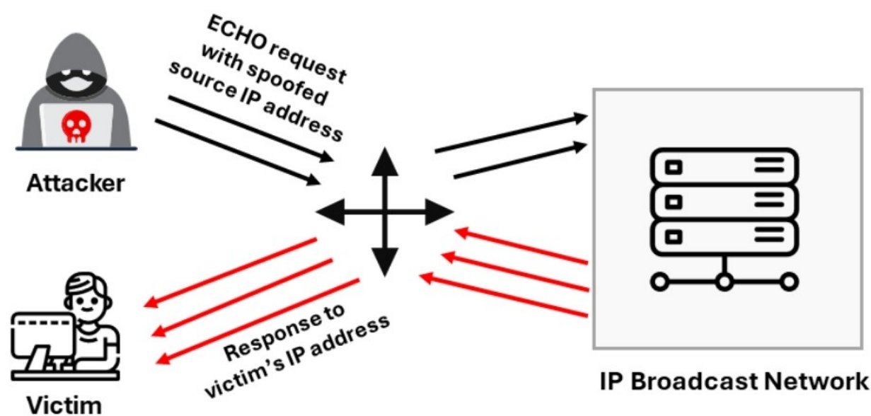
Figure 10.17: Smurf attack
