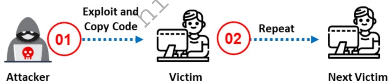
Figure 10.9: Autonomous Propagation
