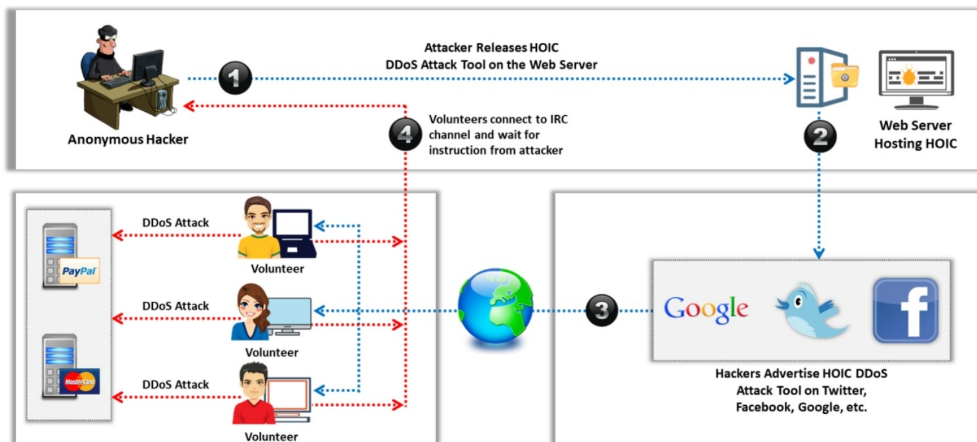
Figure 10.10: DDoS attack scenario
