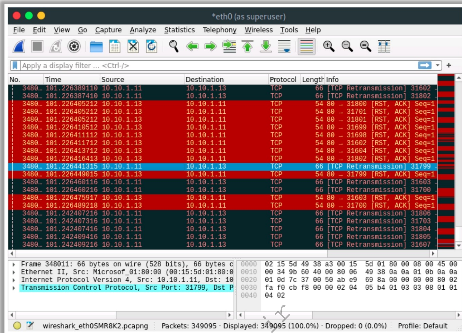
Figure 10.33: Flood recorded on the target machine
