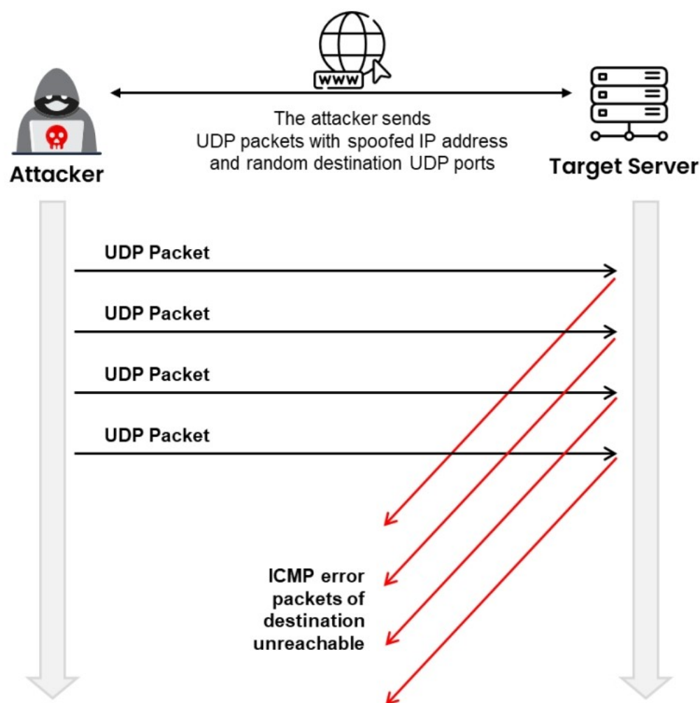
Figure 10.14: UDP flood attack
