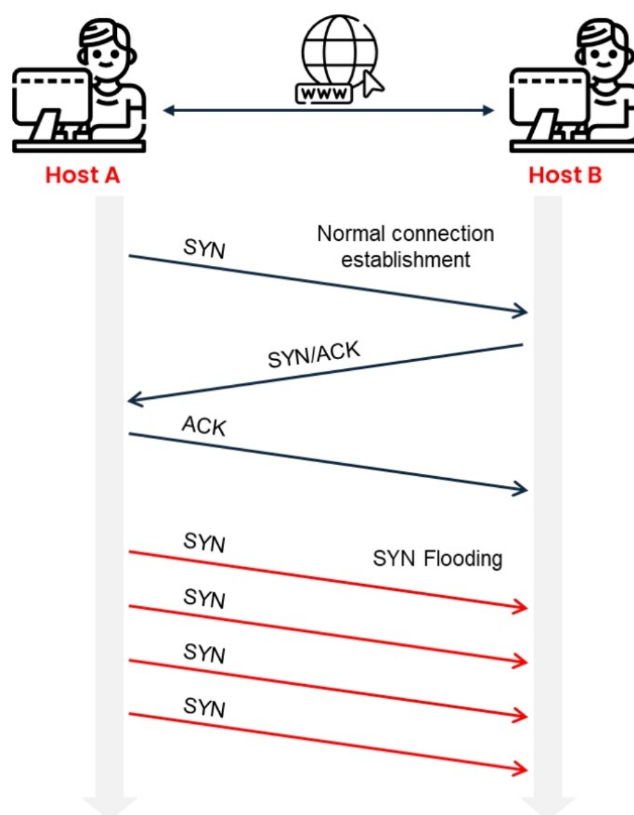
Figure 10.21: SYN flood attack
