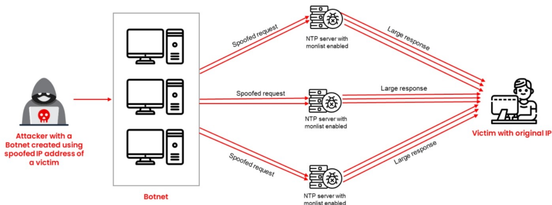
Figure 10.19: Illustration of NTP server amplification attack
