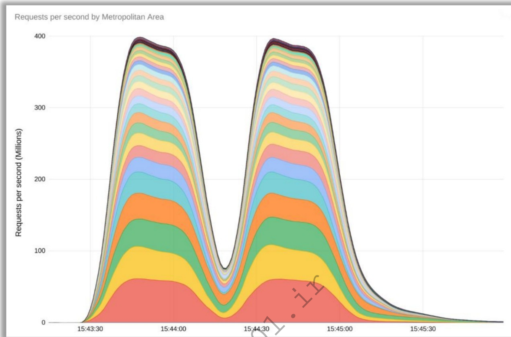
Figure 10.12: DDoS attack where it peaked at 398 million requests per second
