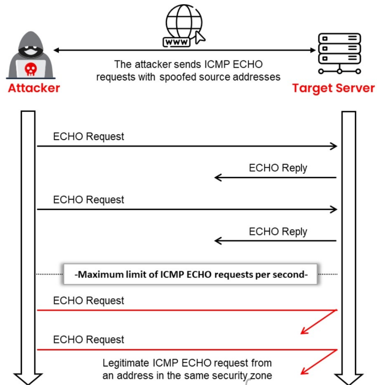
Figure 10.15: ICMP flood attack
