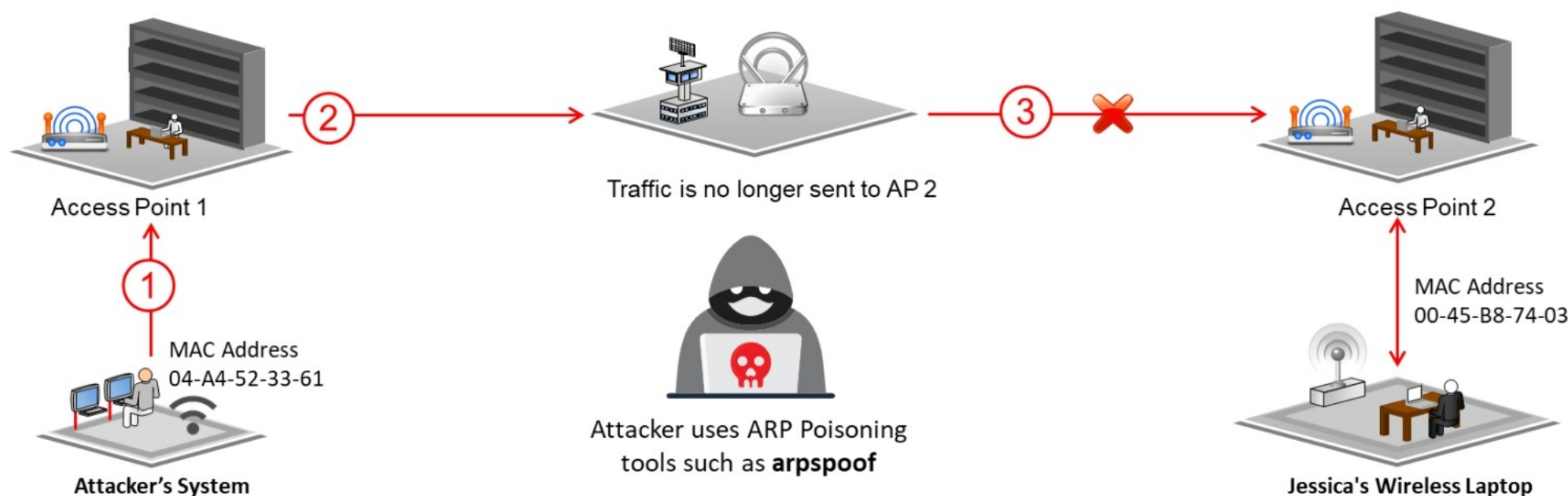
Figure 16.51: ARP poisoning attack
