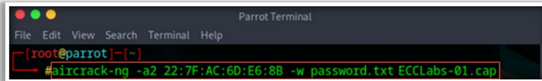
Figure 16.87: Screenshot displaying the execution of aircrack-ng
