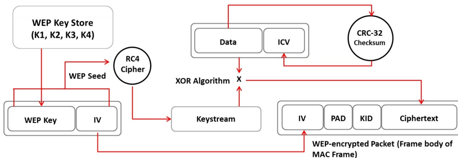
Figure 16.10: Operational flow of WEP
