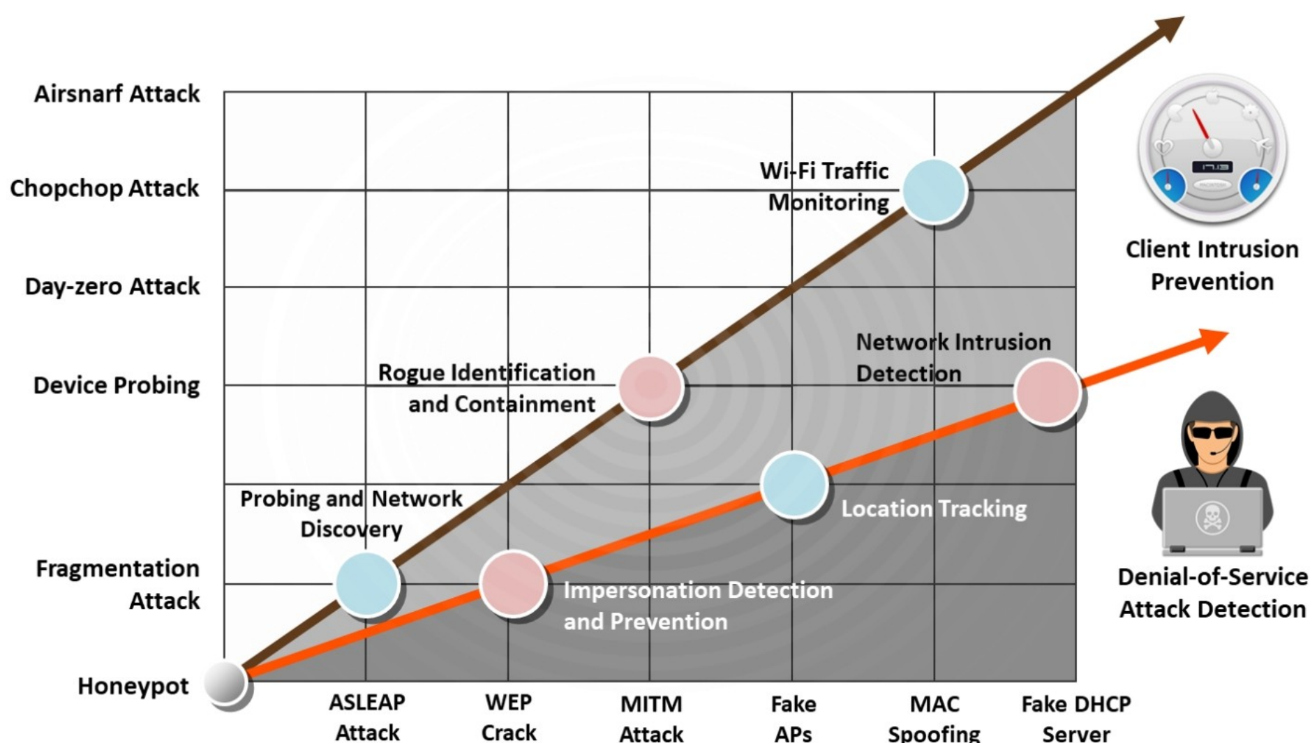
Figure 16.96: Wireless attacks and their prevention methods
