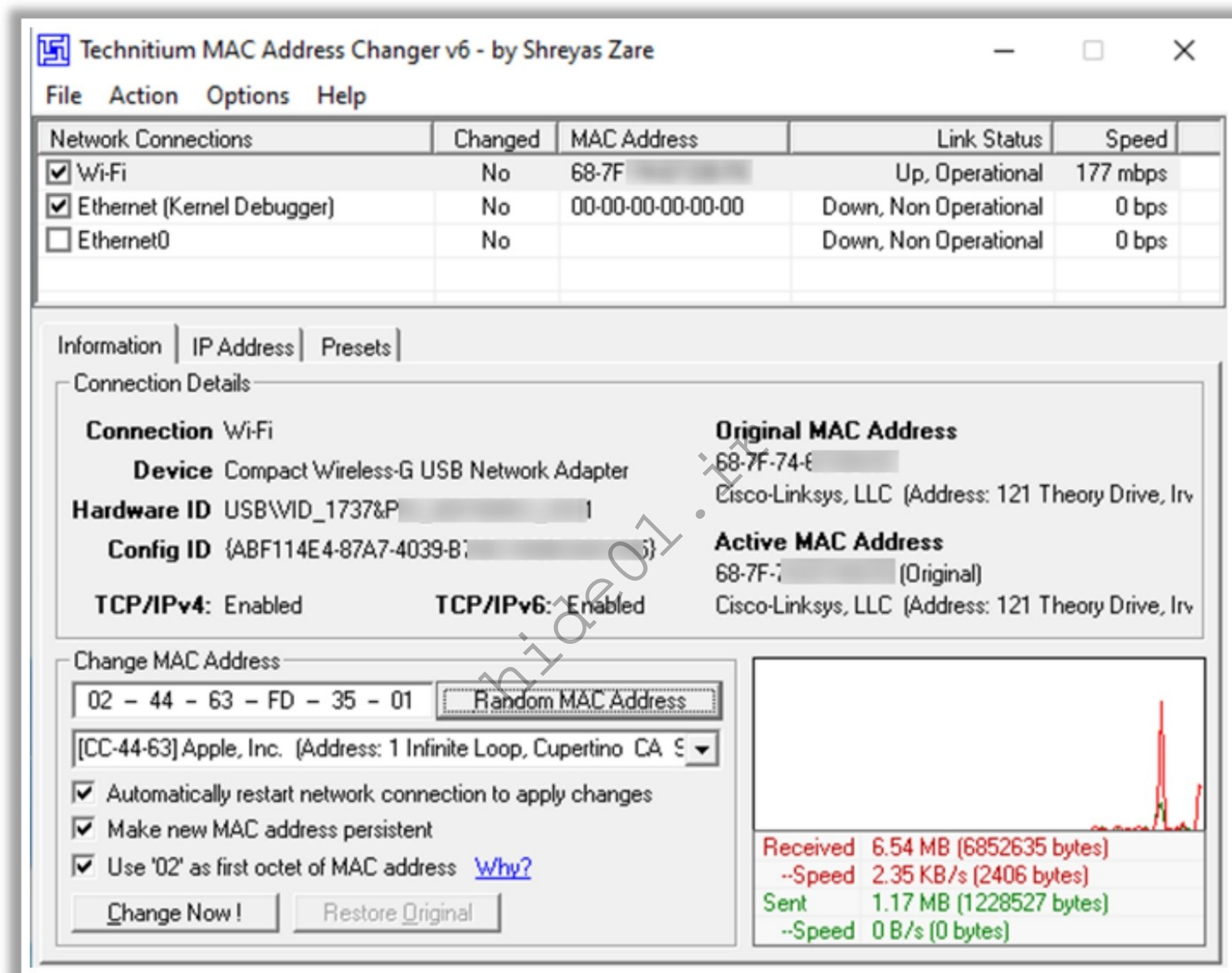
Figure 16.50: Screenshot of Technitium MAC Address Changer
