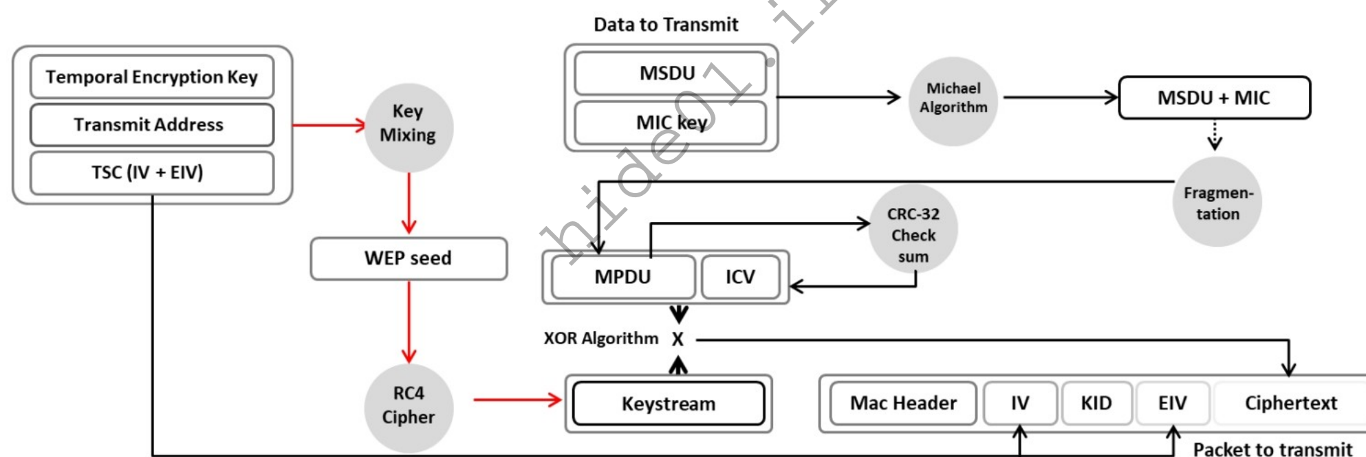
Figure 16.12: Operational flow of WPA
