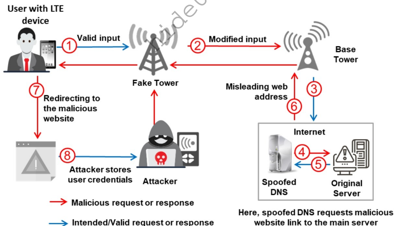
Figure 16.77: Attack phase of an aLTER attack
