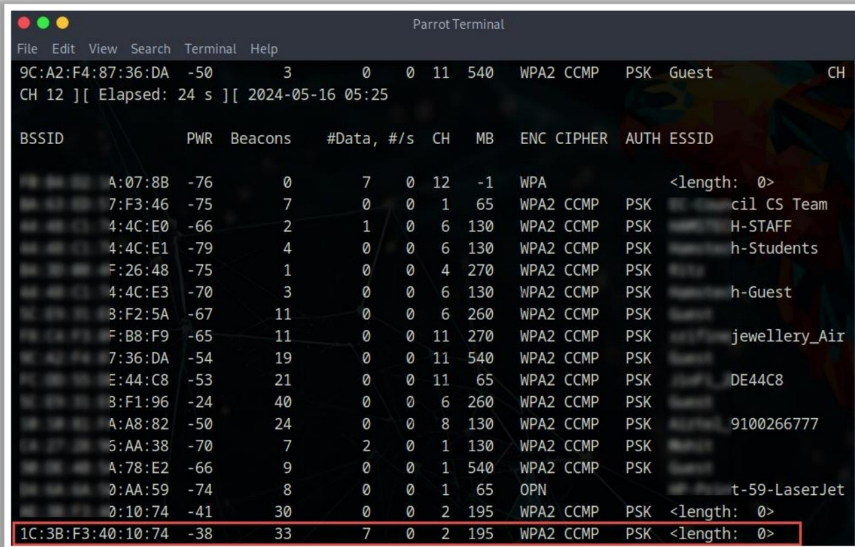
Figure 16.34: Screenshot of the execution of airodump-ng
