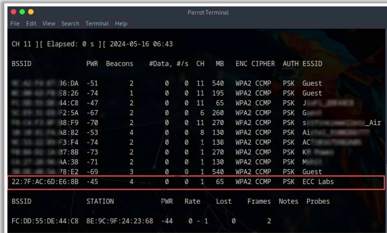
Figure 16.83: Screenshot showing list of detected access points
