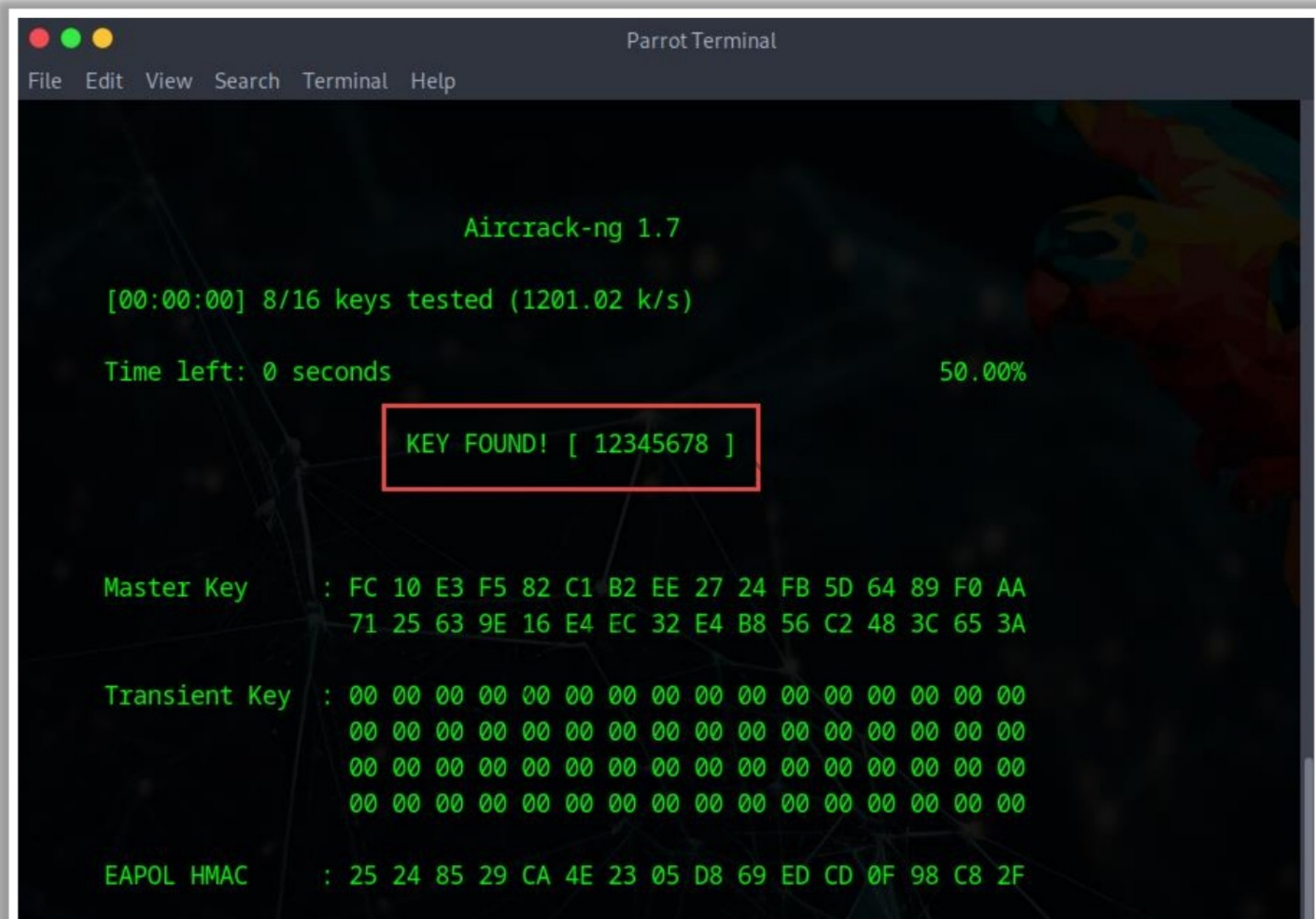
Figure 16.88: Screenshot displaying the result of aircrack-ng cracking the WPA/WPA2 password
