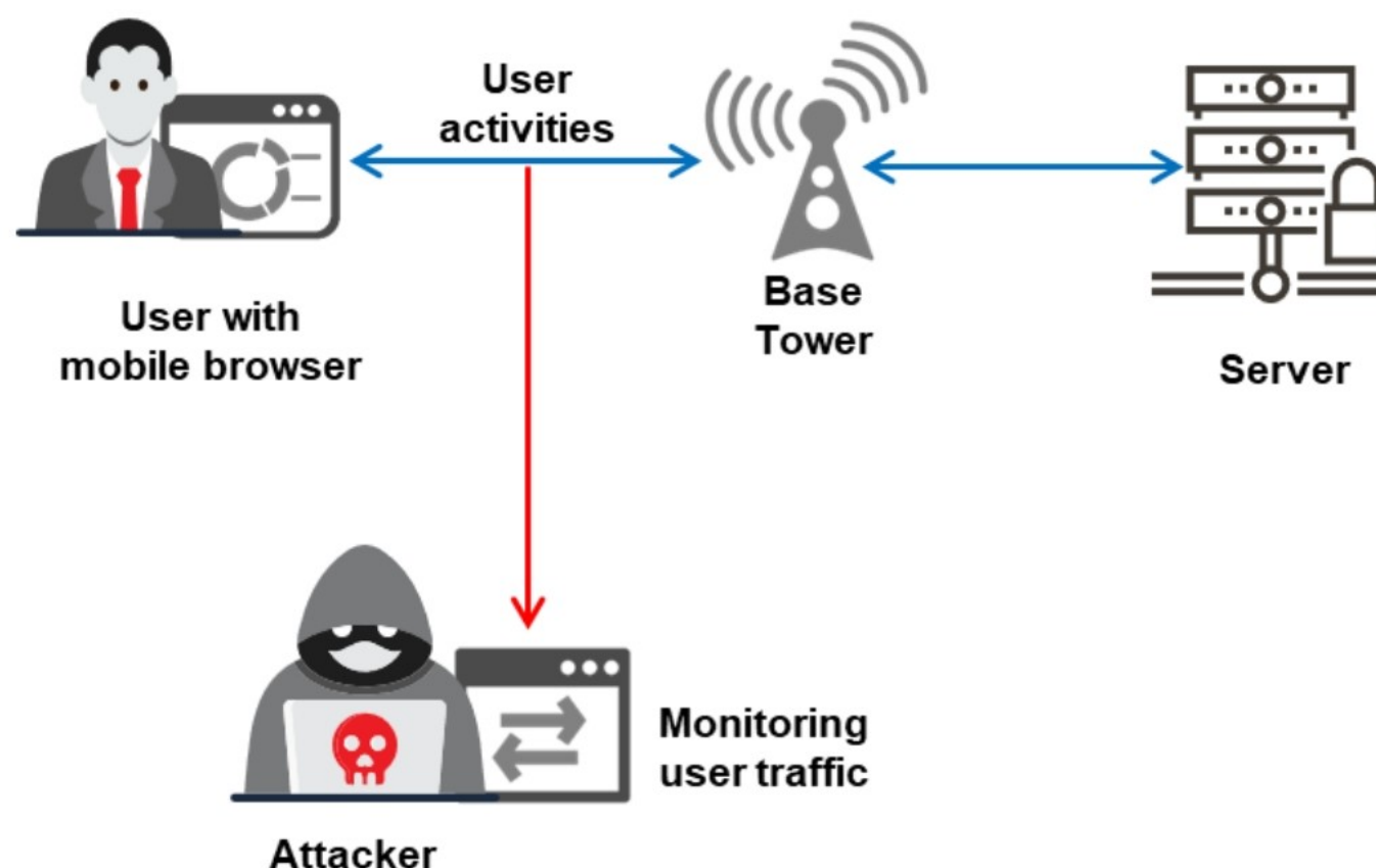
Figure 16.76: Information-gathering phase of an aLTER attack
