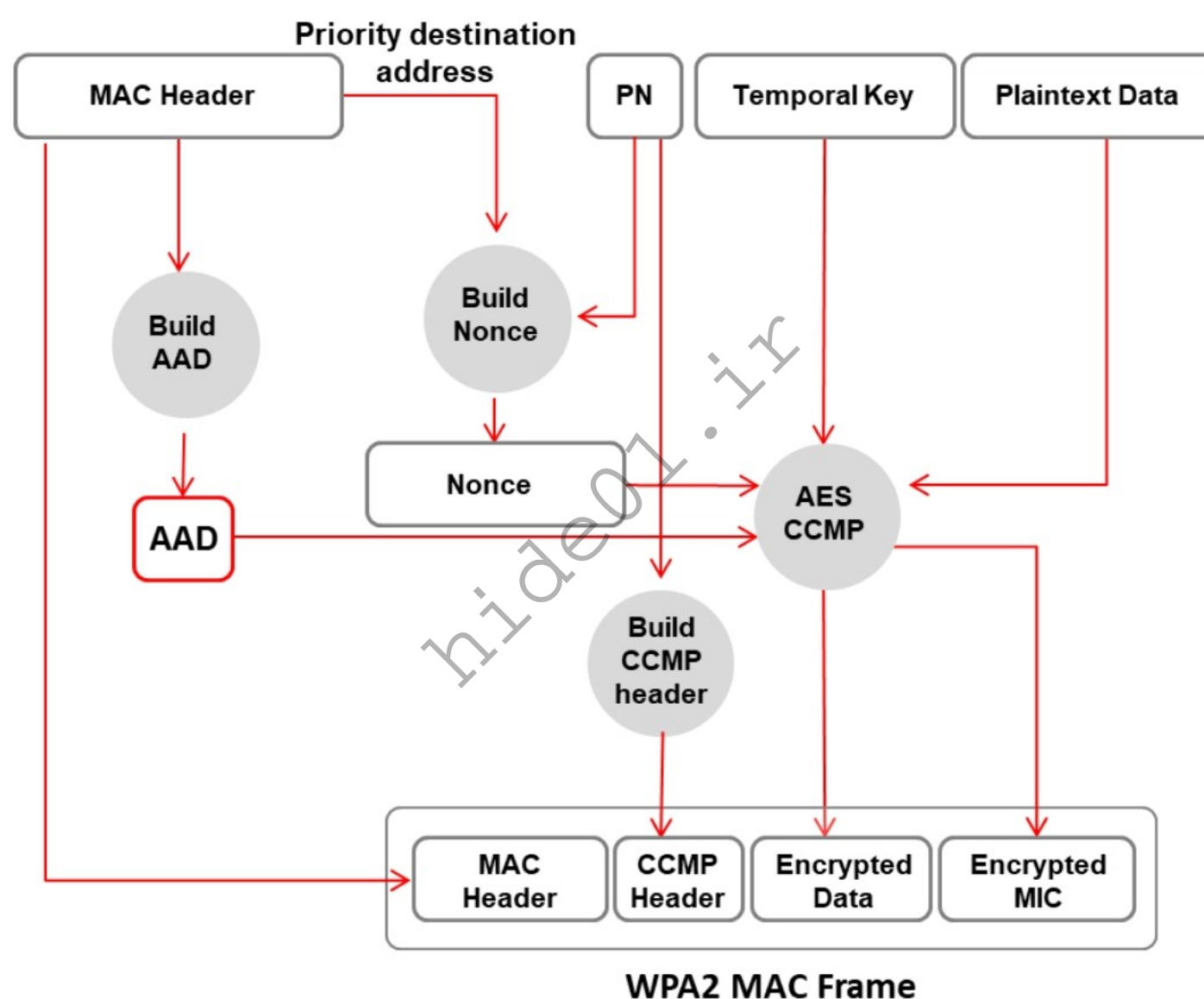
Figure 16.13: Operational flow of WPA2
