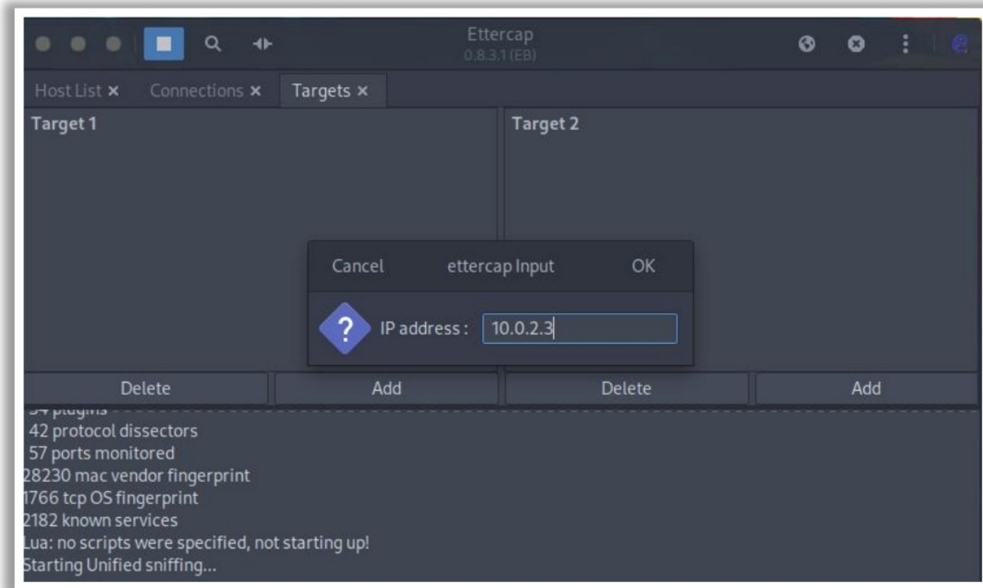
Figure 16.55: Screenshot of Ettercap showing targets
