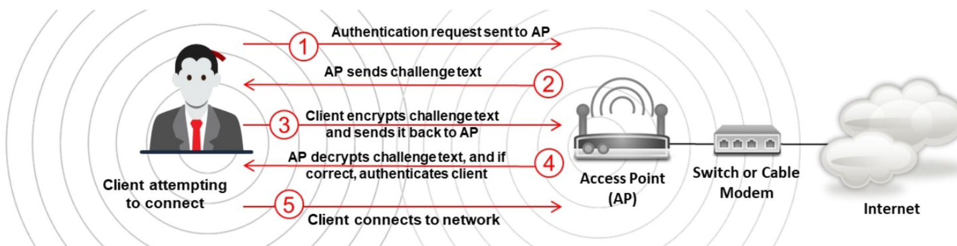
Figure 16.5: PSK Wi-Fi authentication process
