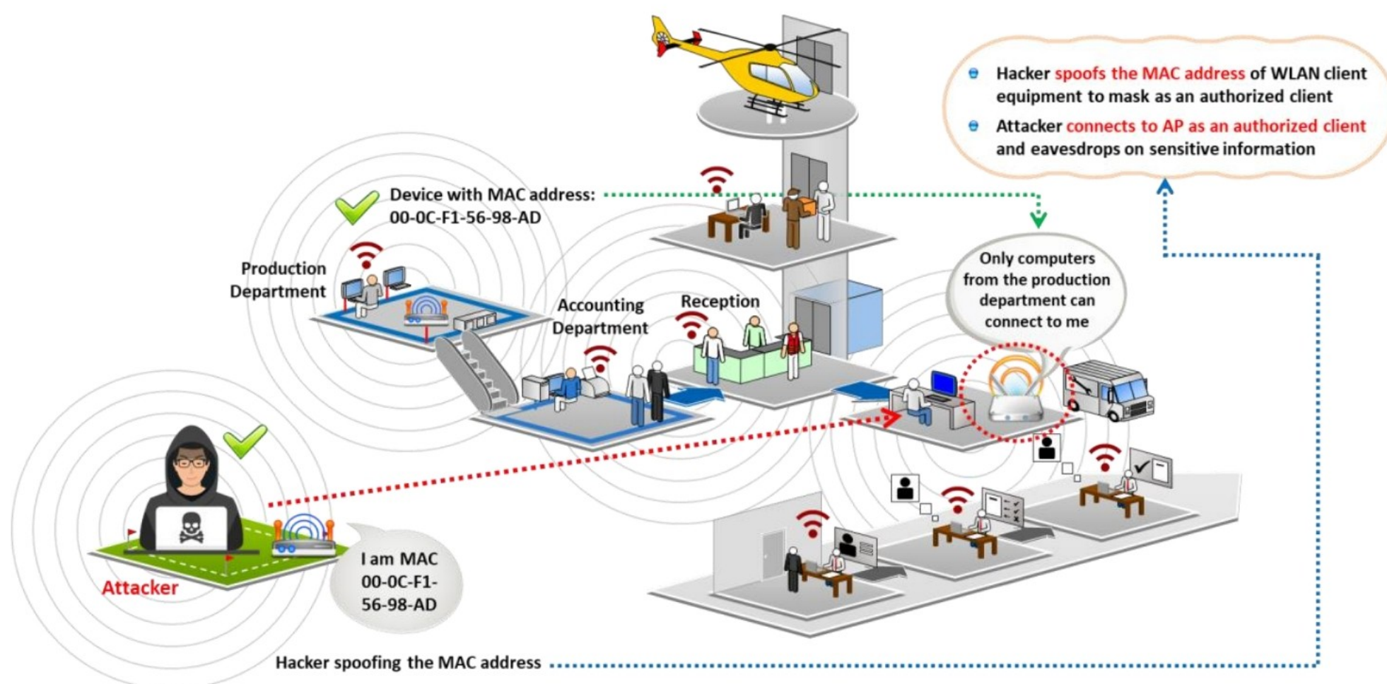
Figure 16.48: AP MAC spoofing
