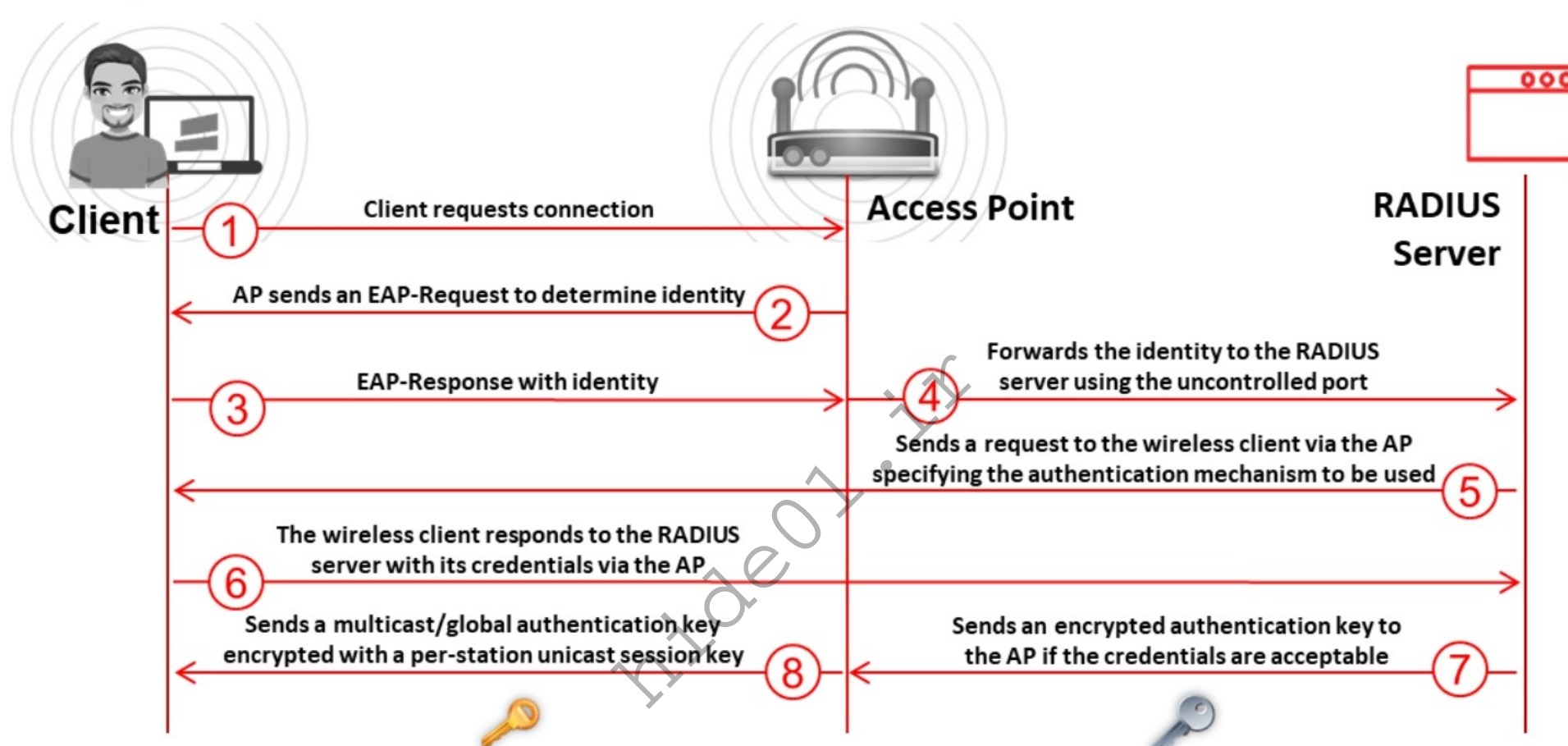
Figure 16.6: Centralized authentication process
