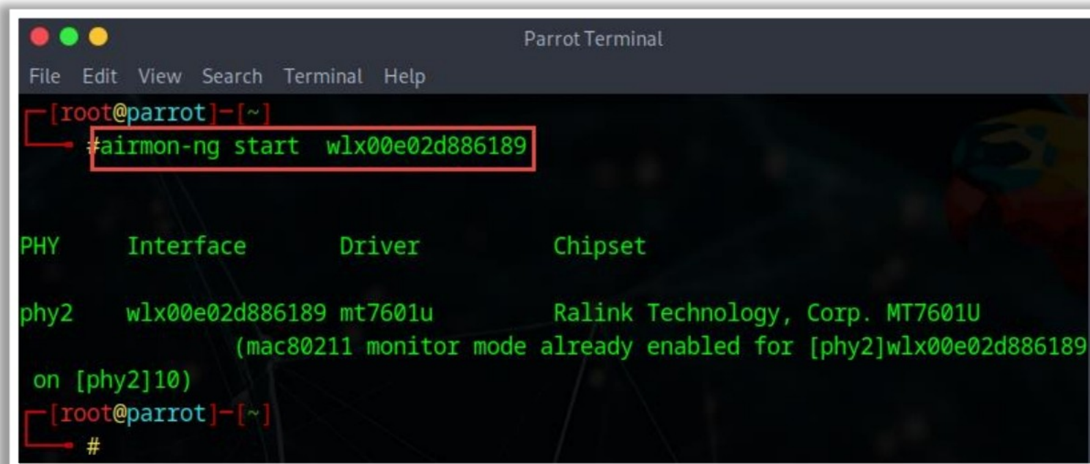
Figure 16.32: Screenshot of the execution of airmon-ng start
