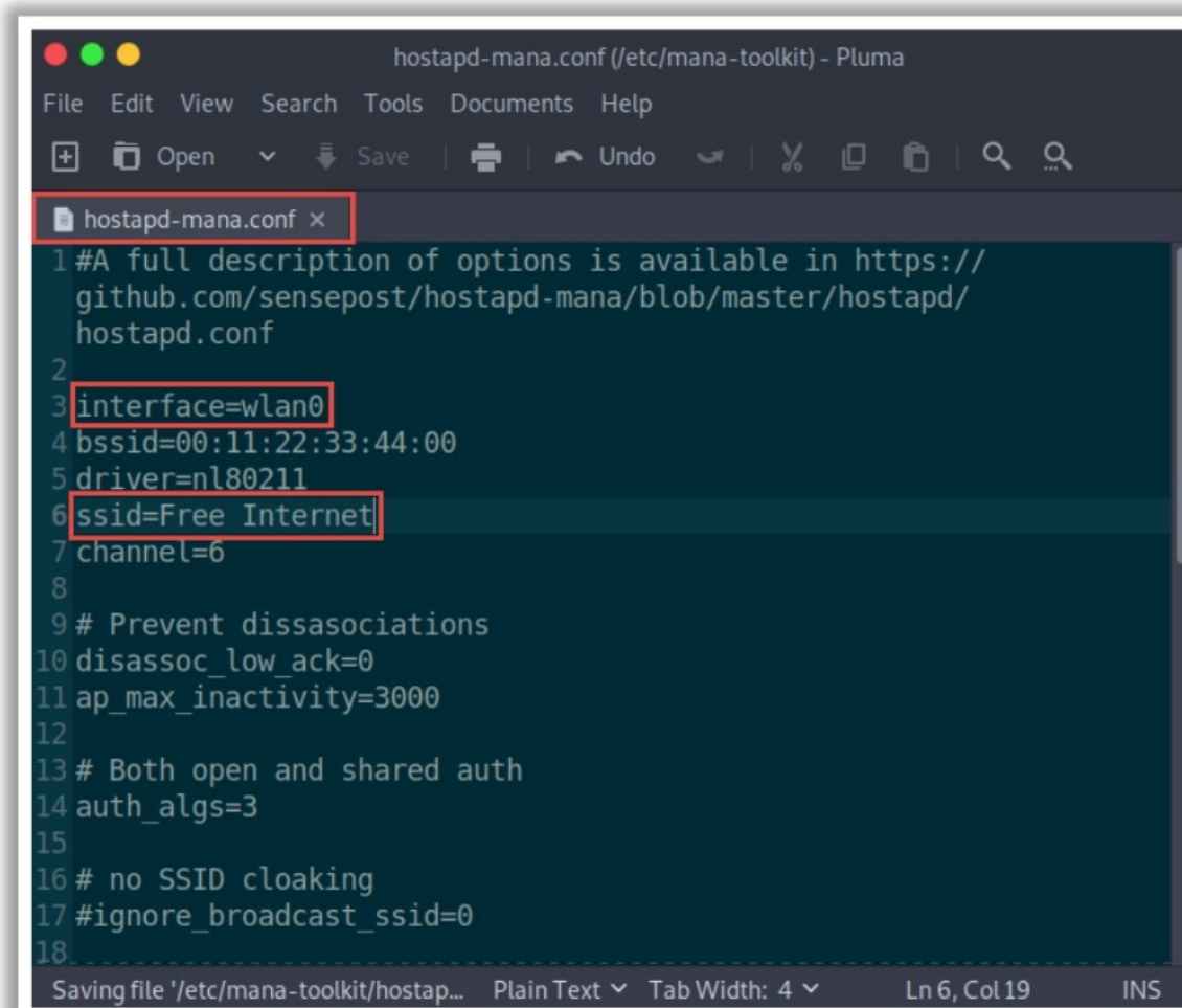
Figure 16.59: Screenshot showing hostapd-mana.conf
