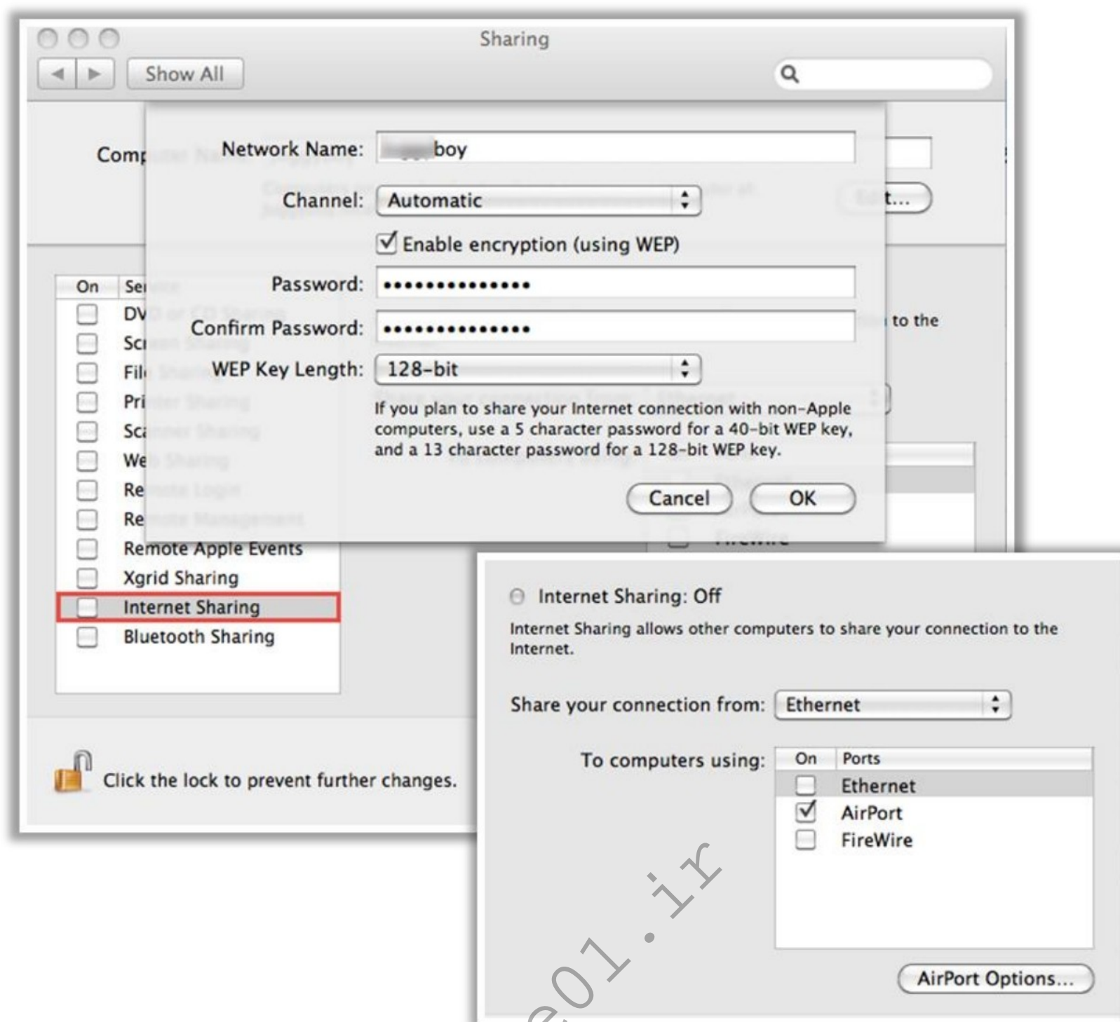
Figure 16.64: Screenshot of the Internet Sharing window in macOS
