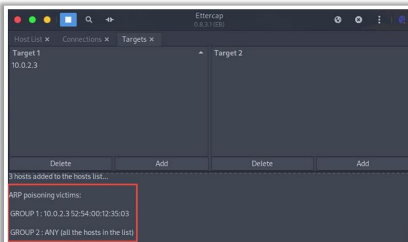
Figure 16.57: Screenshot of Ettercap launching an ARP poisoning attack
