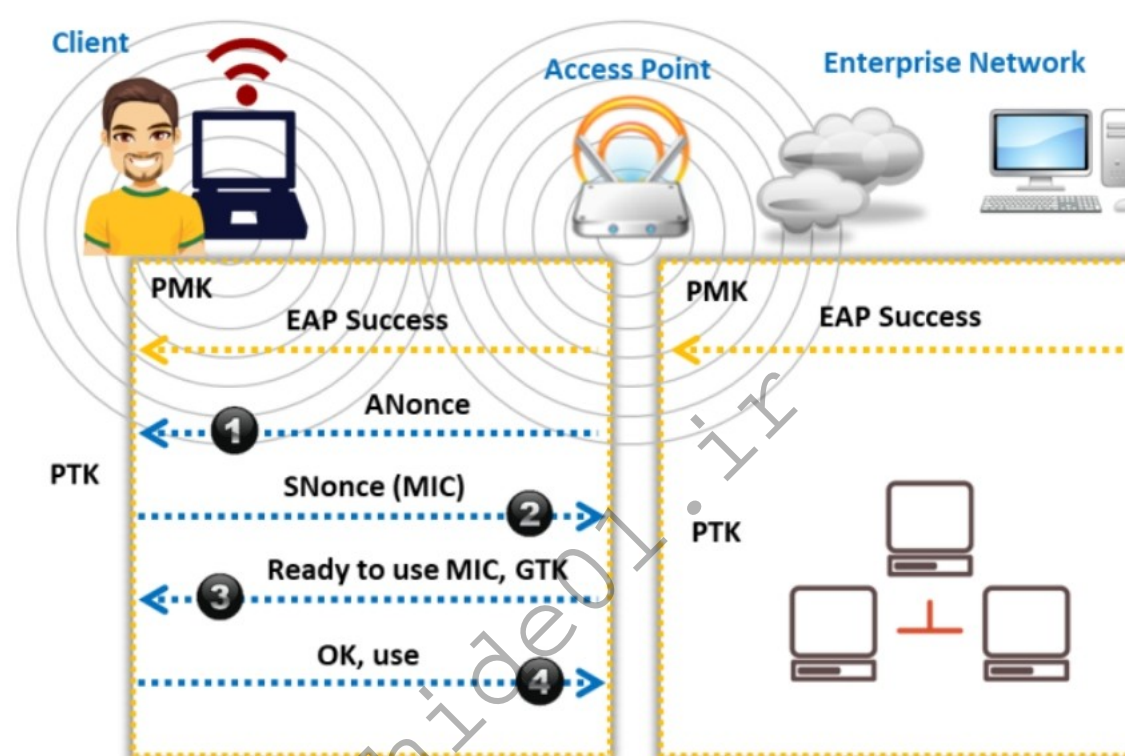
Figure 16.11: Operational flow of temporal keys
