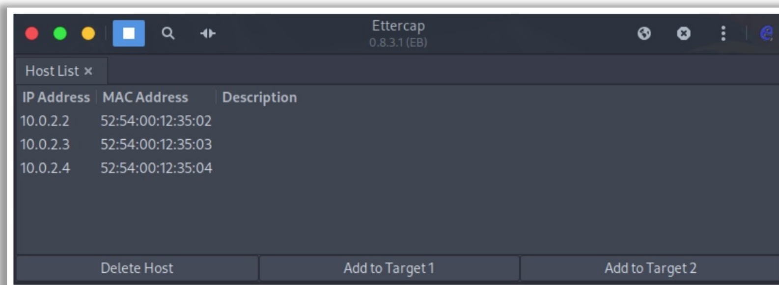
Figure 16.53: Screenshot of Ettercap showing the host list
