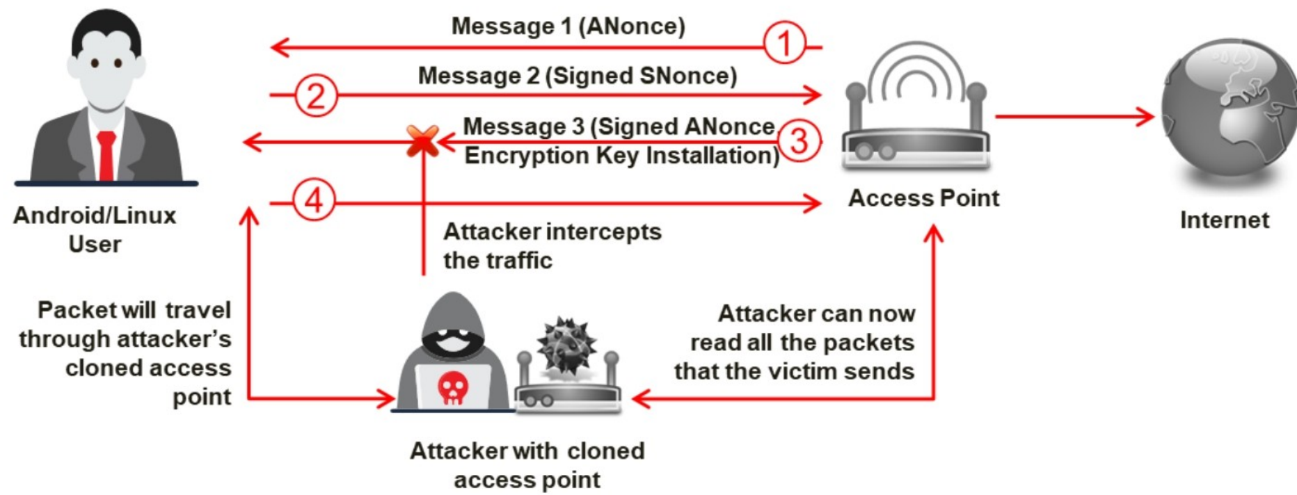
Figure 16.67: KRACK attack exploiting the four-way handshake process in WPA2
