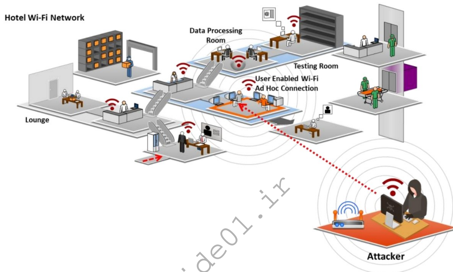
Figure 16.15: Ad-Hoc connection attack
