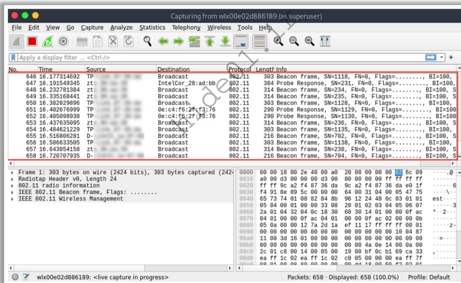
Figure 16.29: Screenshot showing Wireshark capturing wireless traffic
