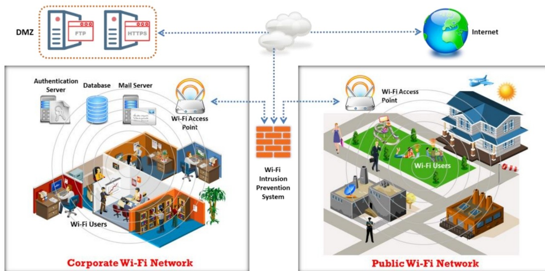
Figure 16.97: WIPS deployment
