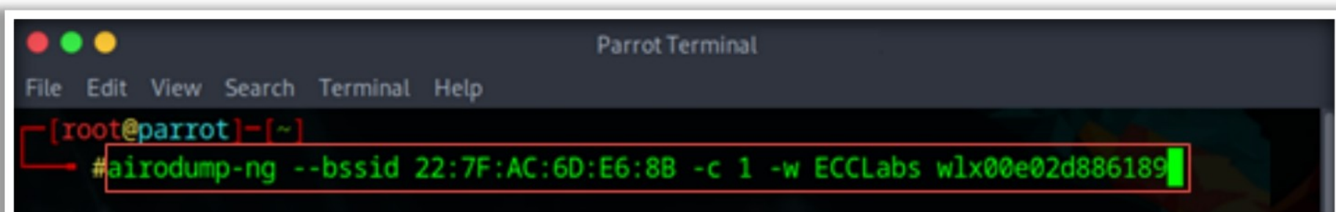
Figure 16.84: Screenshot displaying the execution of airodump-ng
