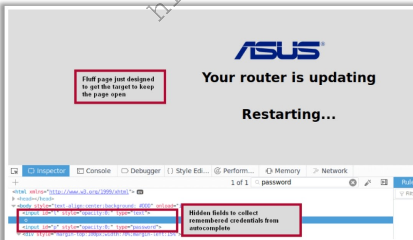
Figure 16.79: Screenshot showing the update and restarting of the router
