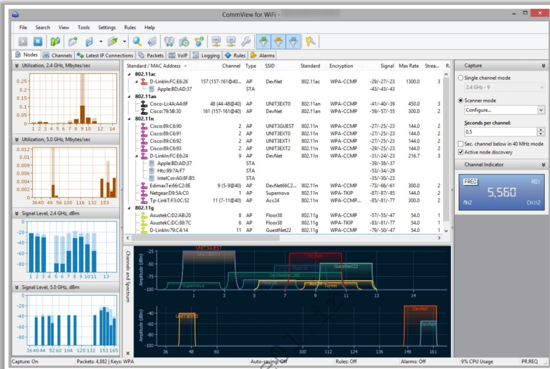
Figure 16.30: Screenshot of CommView for Wi-Fi
