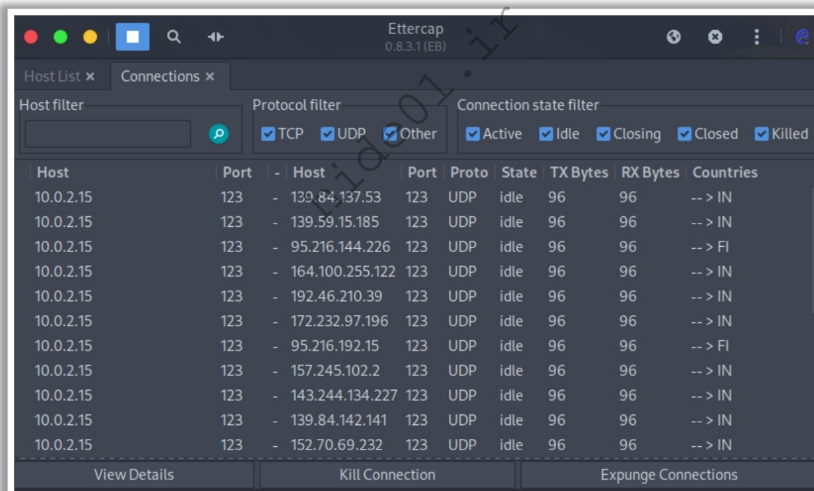
Figure 16.54: Screenshot of Ettercap showing the host list
