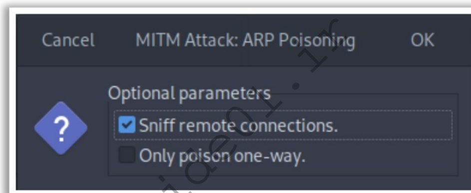
Figure 16.56: Screenshot of optional parameter selection in Ettercap when launching an ARP poisoning attack
