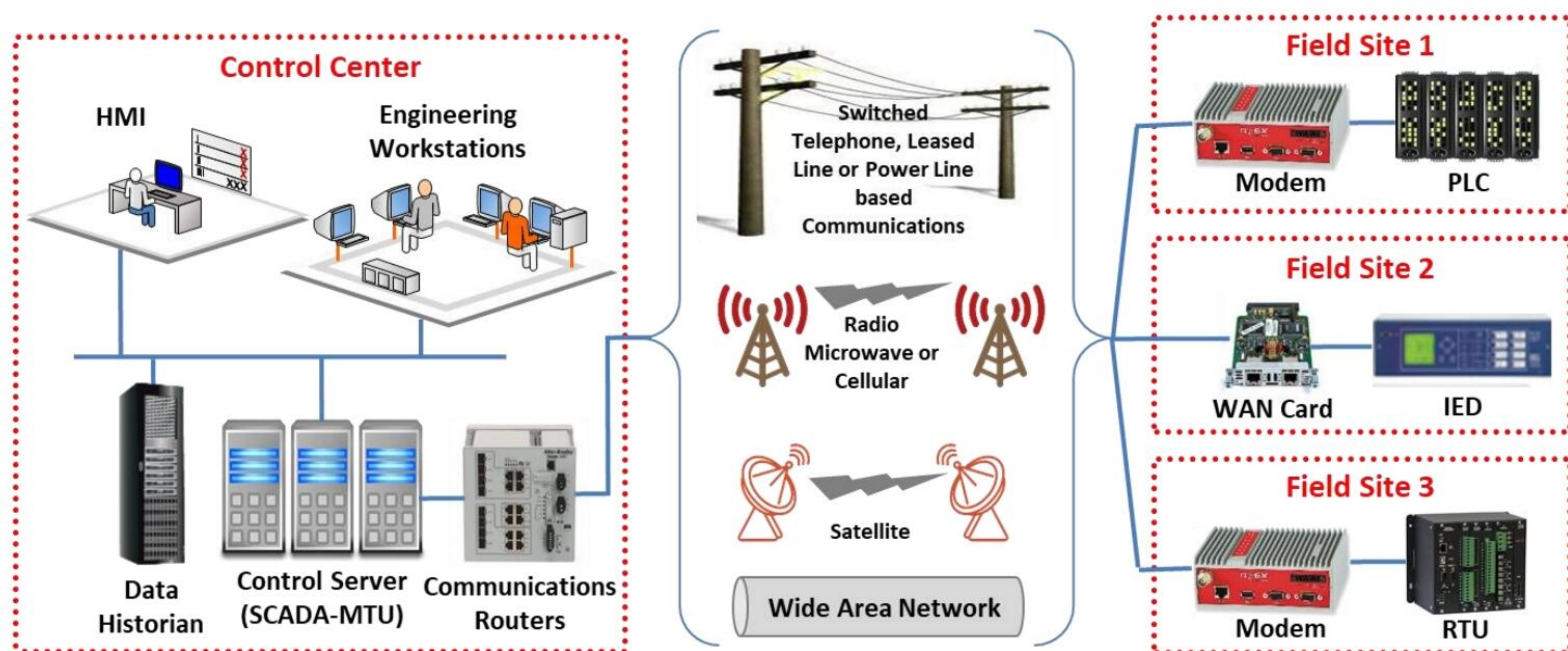
Figure 18.75: SCADA architecture
