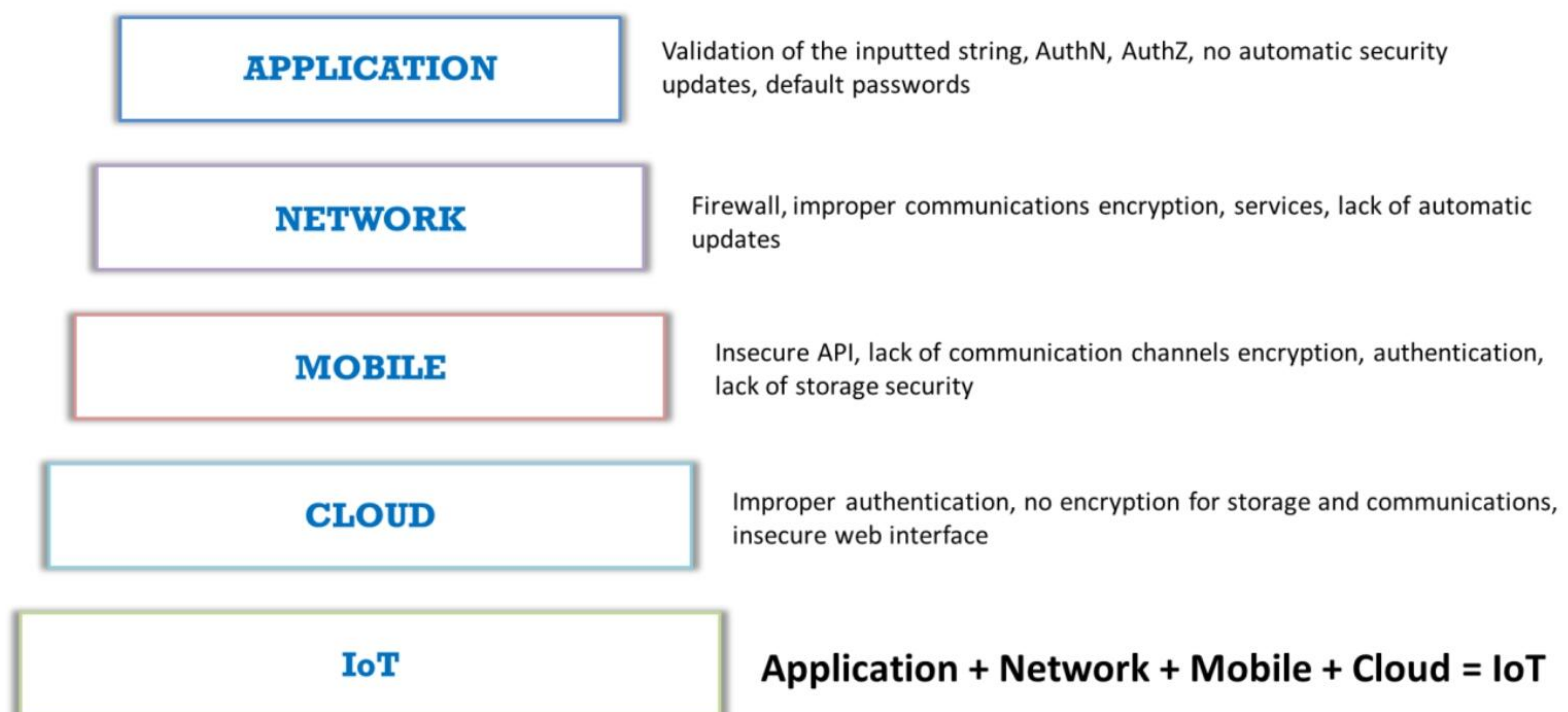
Figure 18.7: Security problems in IoT architecture
