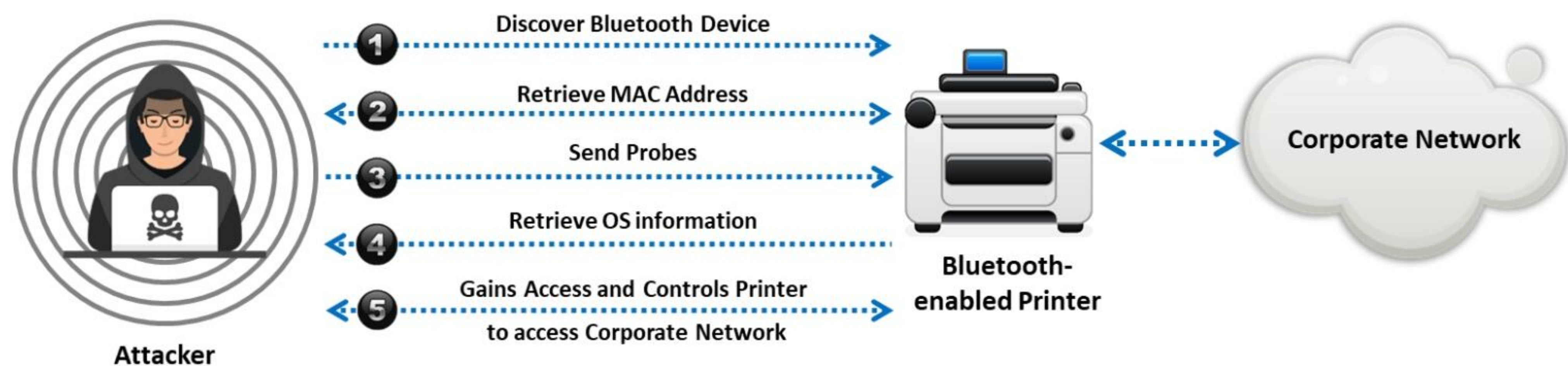
Figure 18.12: Illustration of BlueBorne attack
