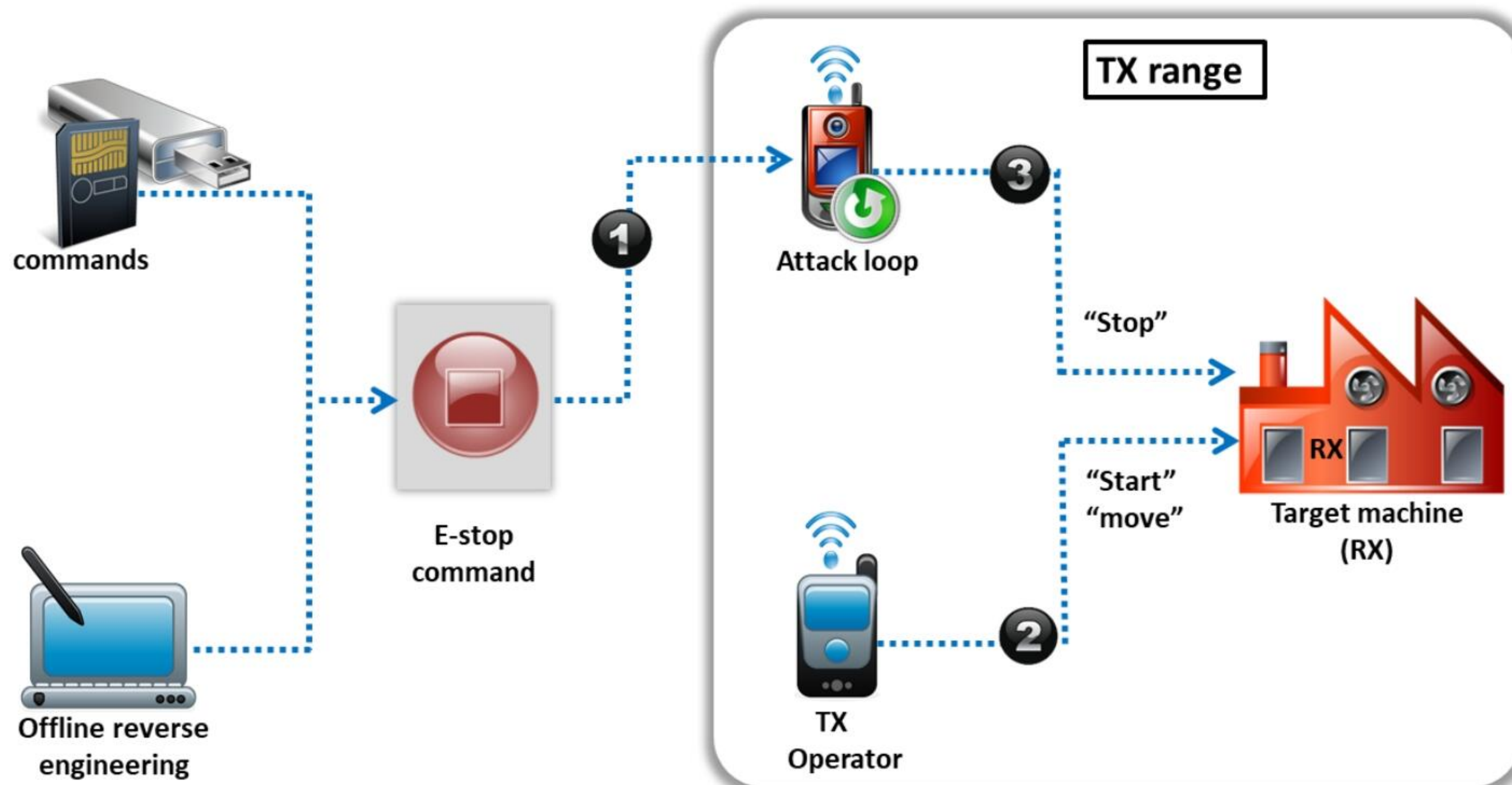
Figure 18.85: Abusing e-stop to perform a DoS attack
