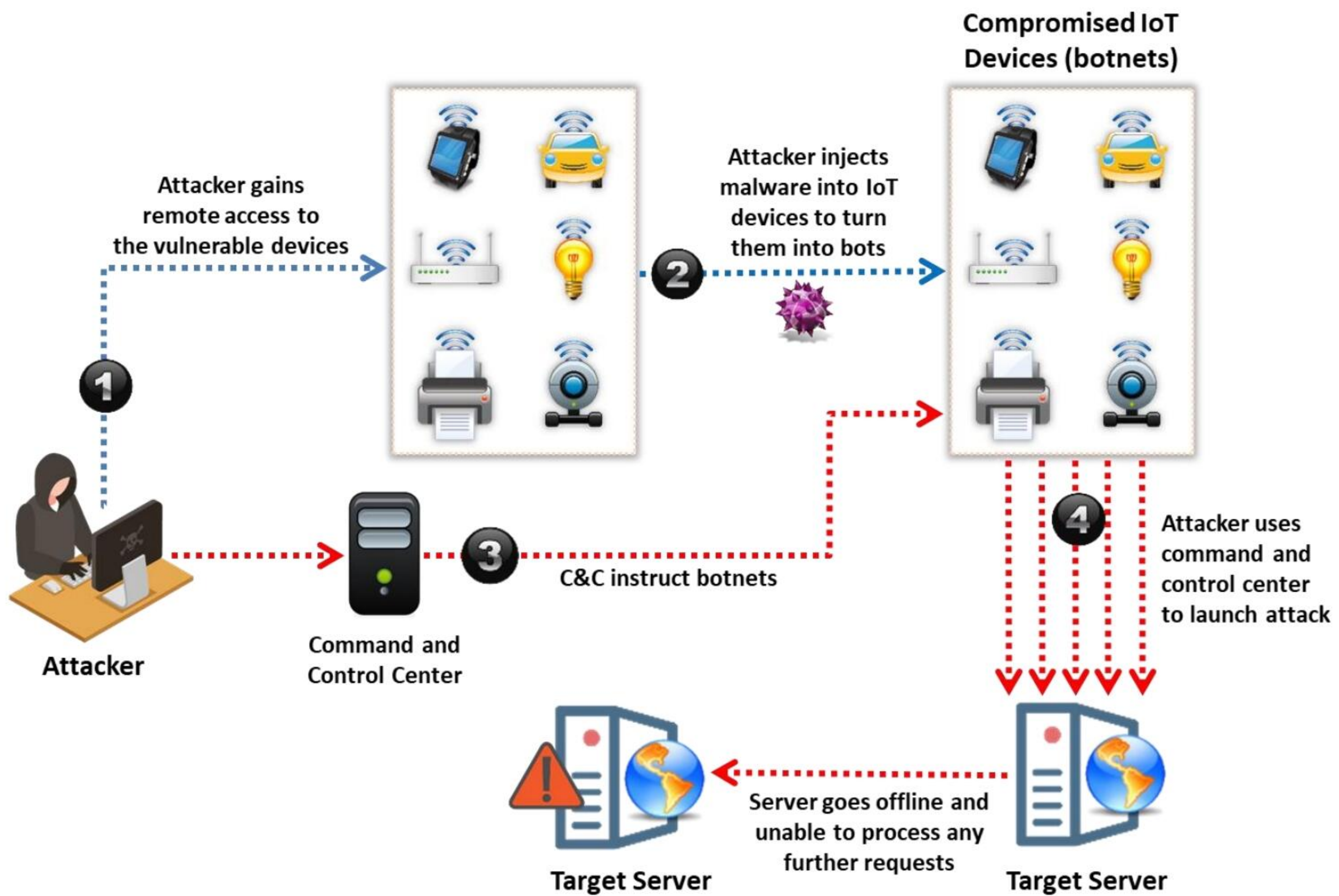
Figure 18.9: DDoS attack on IoT devices
