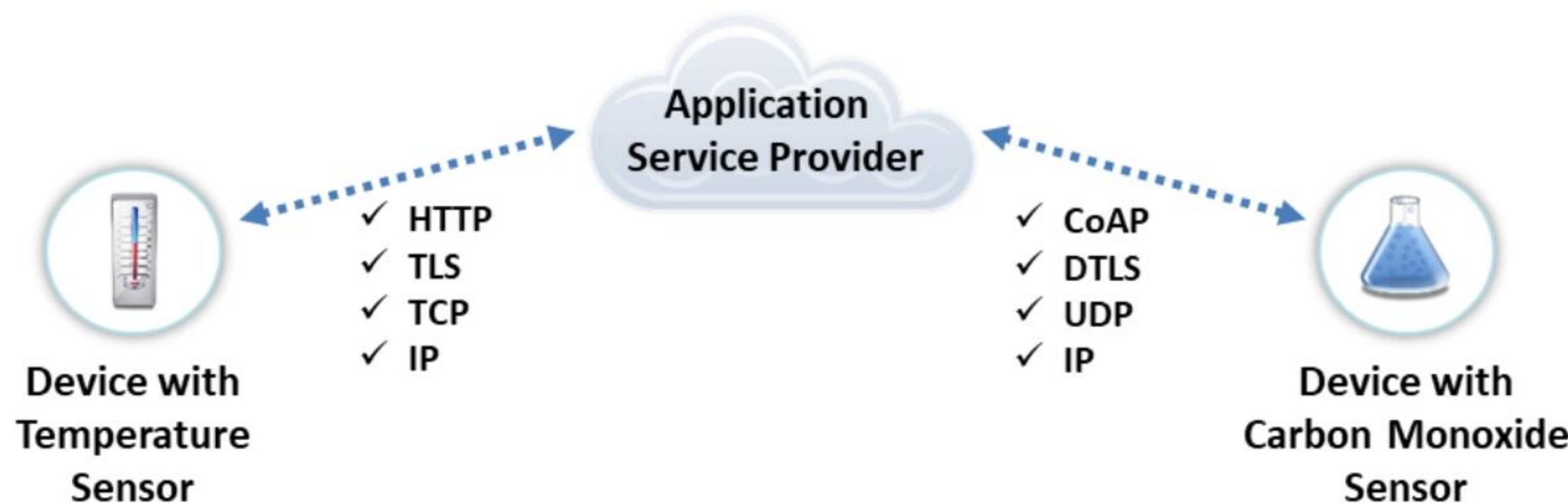
Figure 18.4: IoT device-to-cloud communication model
