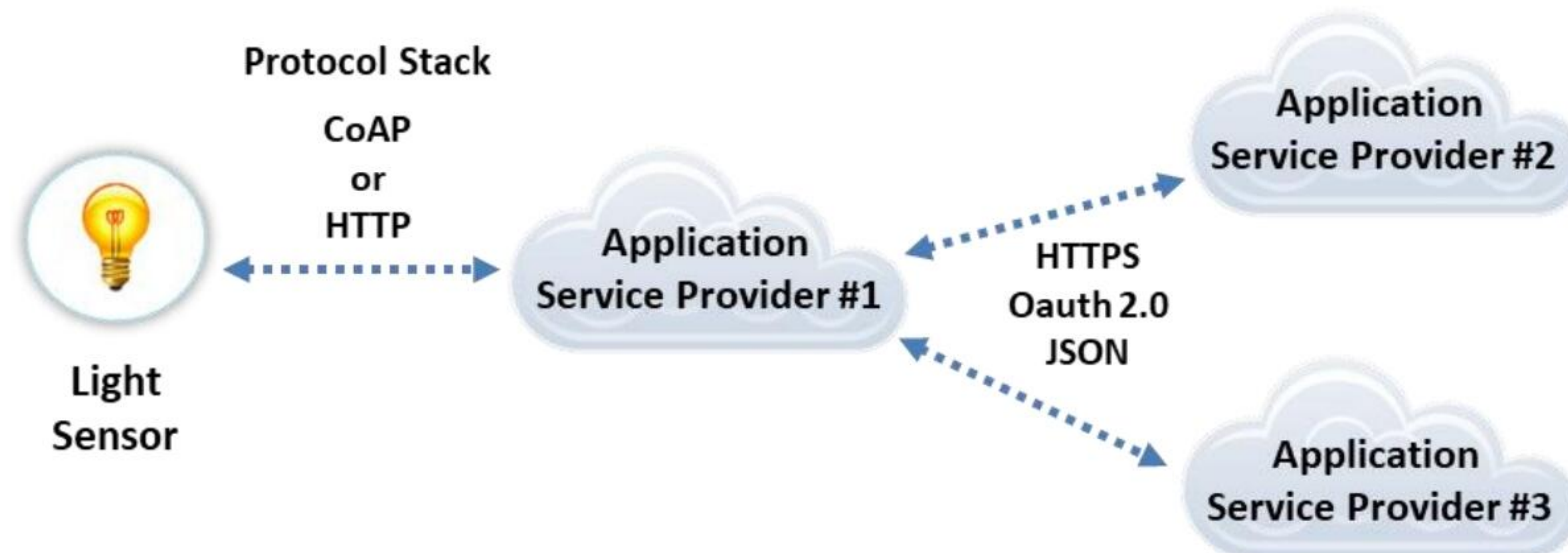
Figure 18.6: IoT back-end data-sharing model
