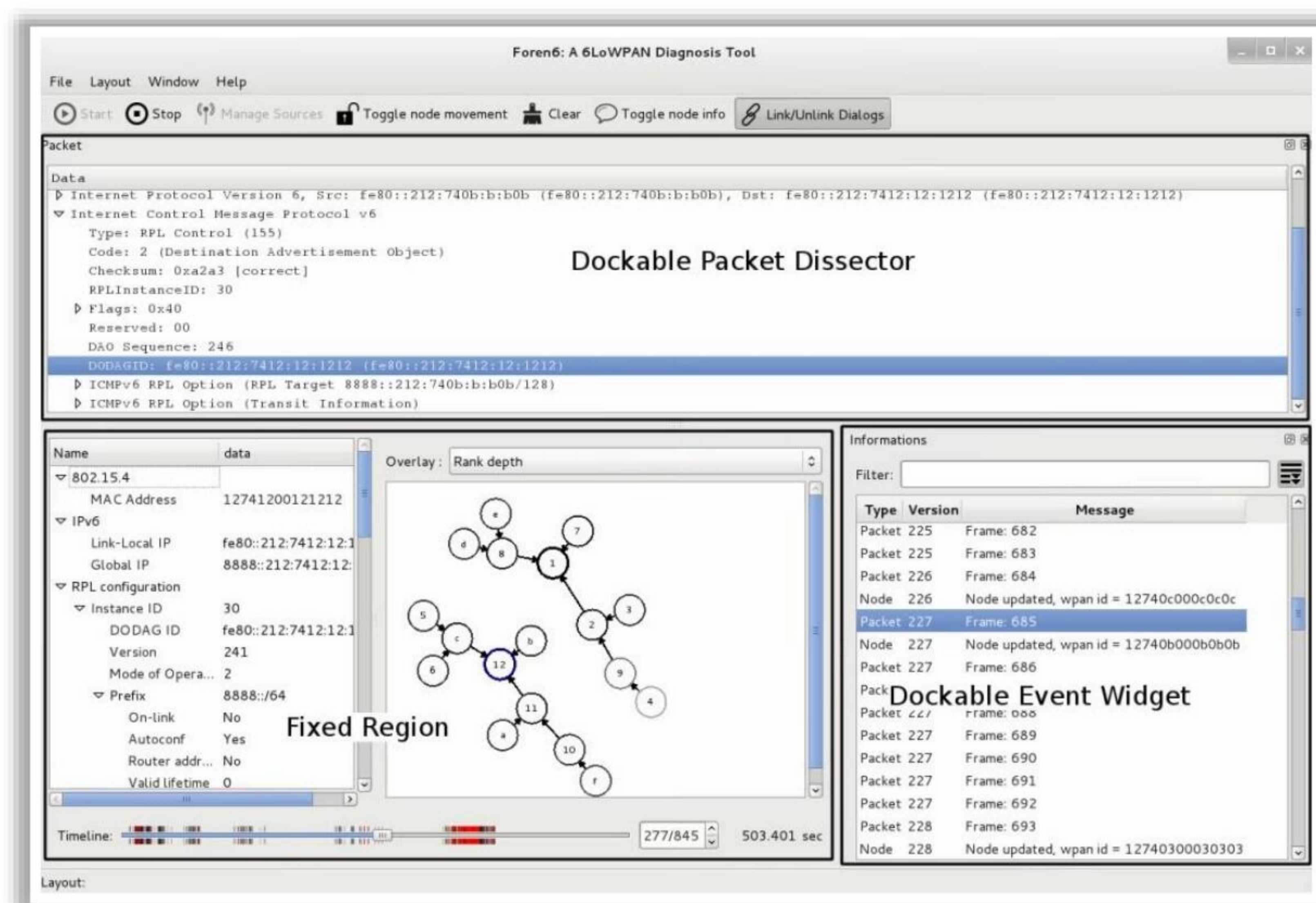
Figure 18.35: Screenshot of Foren6 showing various result panes
