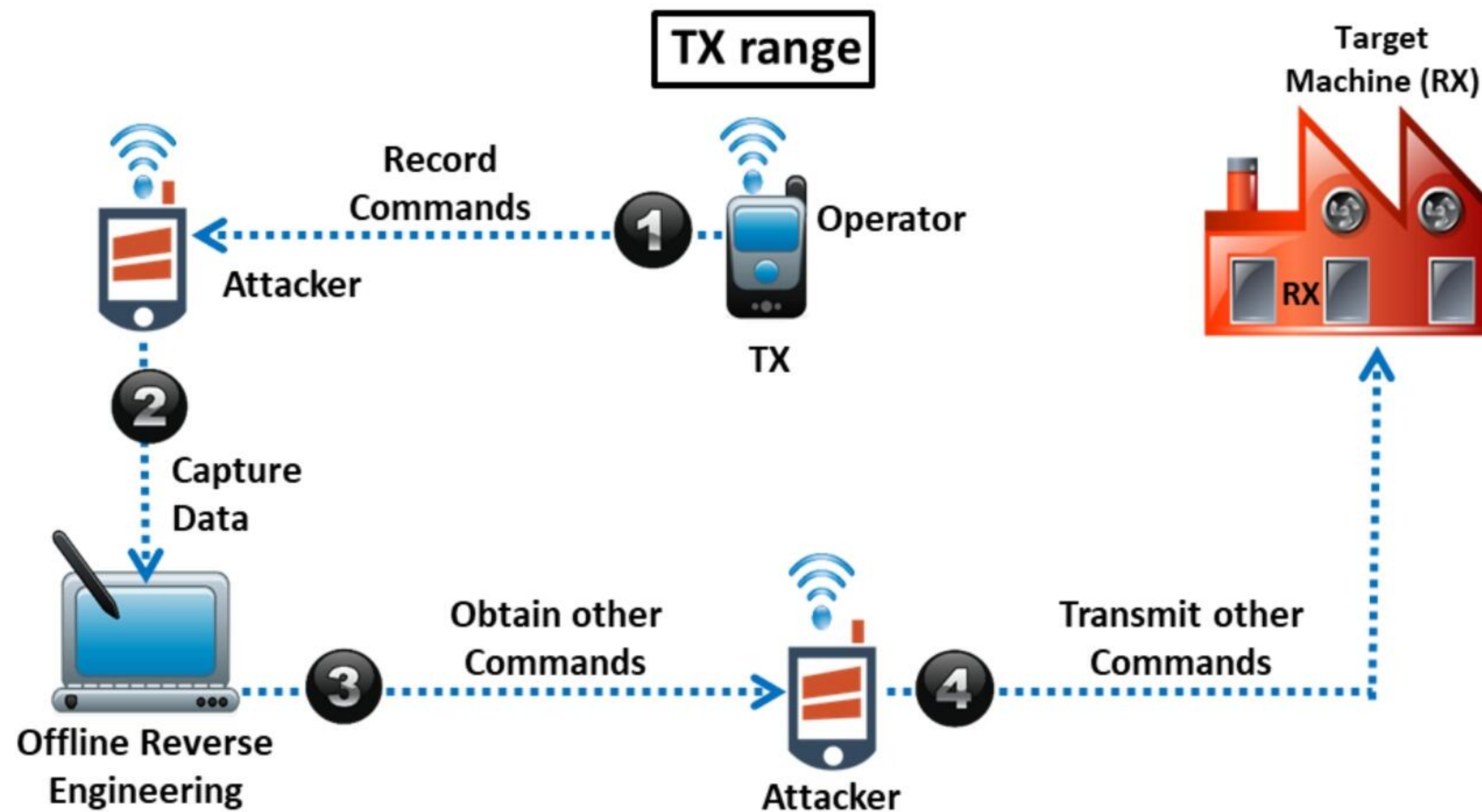
Figure 18.84: Command injection attack on industrial systems
