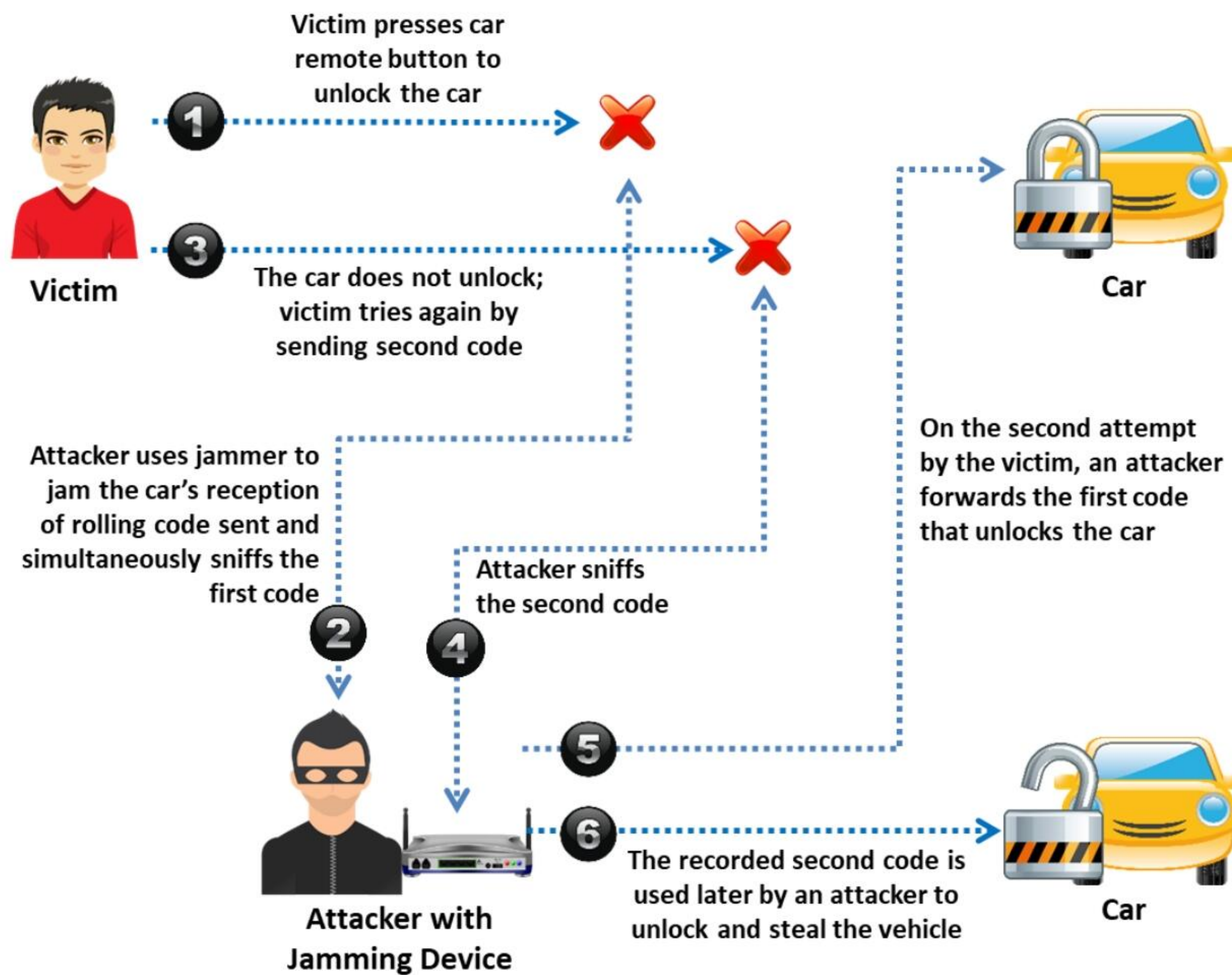
Figure 18.11: Illustration of rolling-code attack
