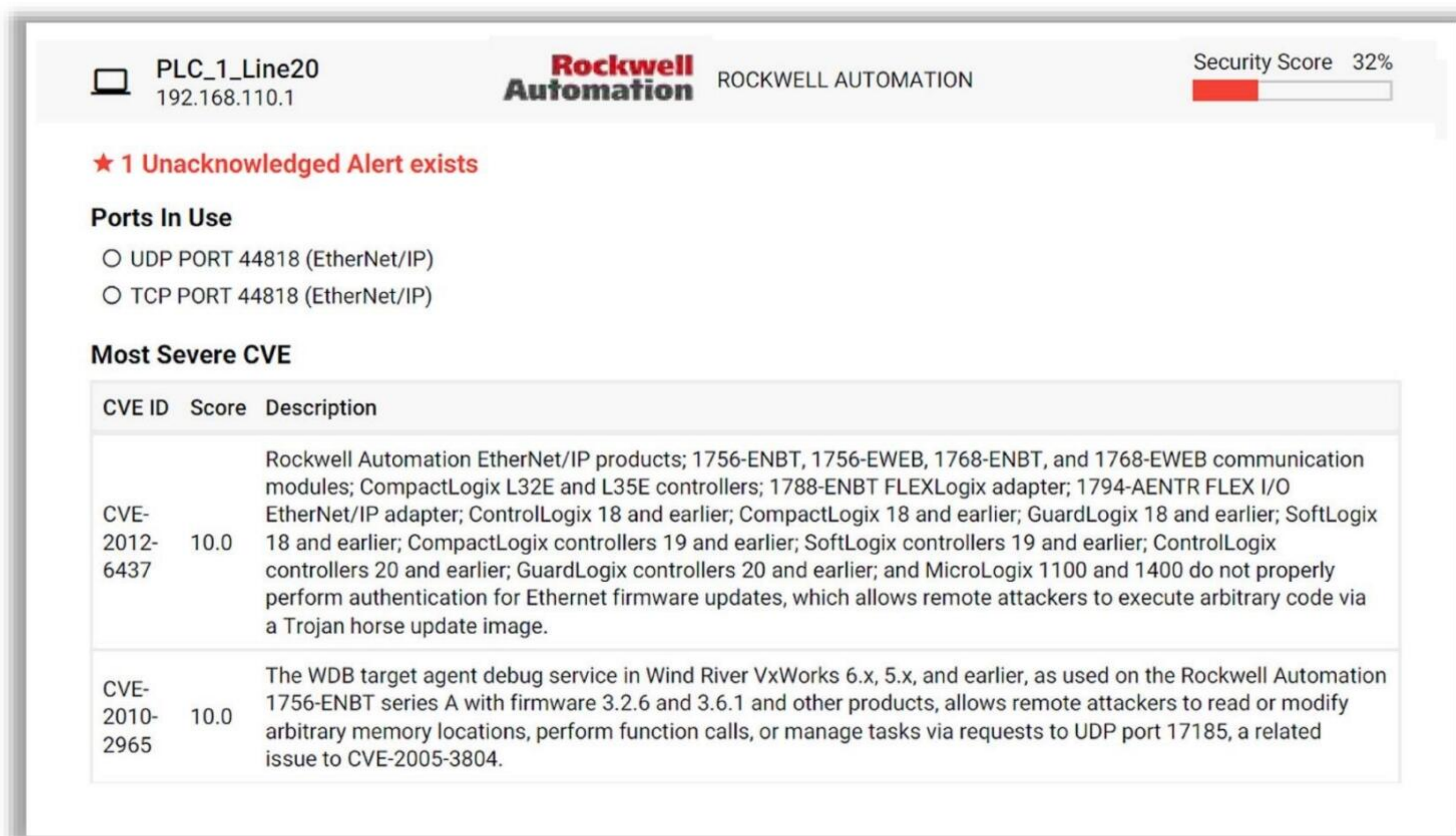
Figure 18.121: Screenshot of Microsoft Defender for IoT
