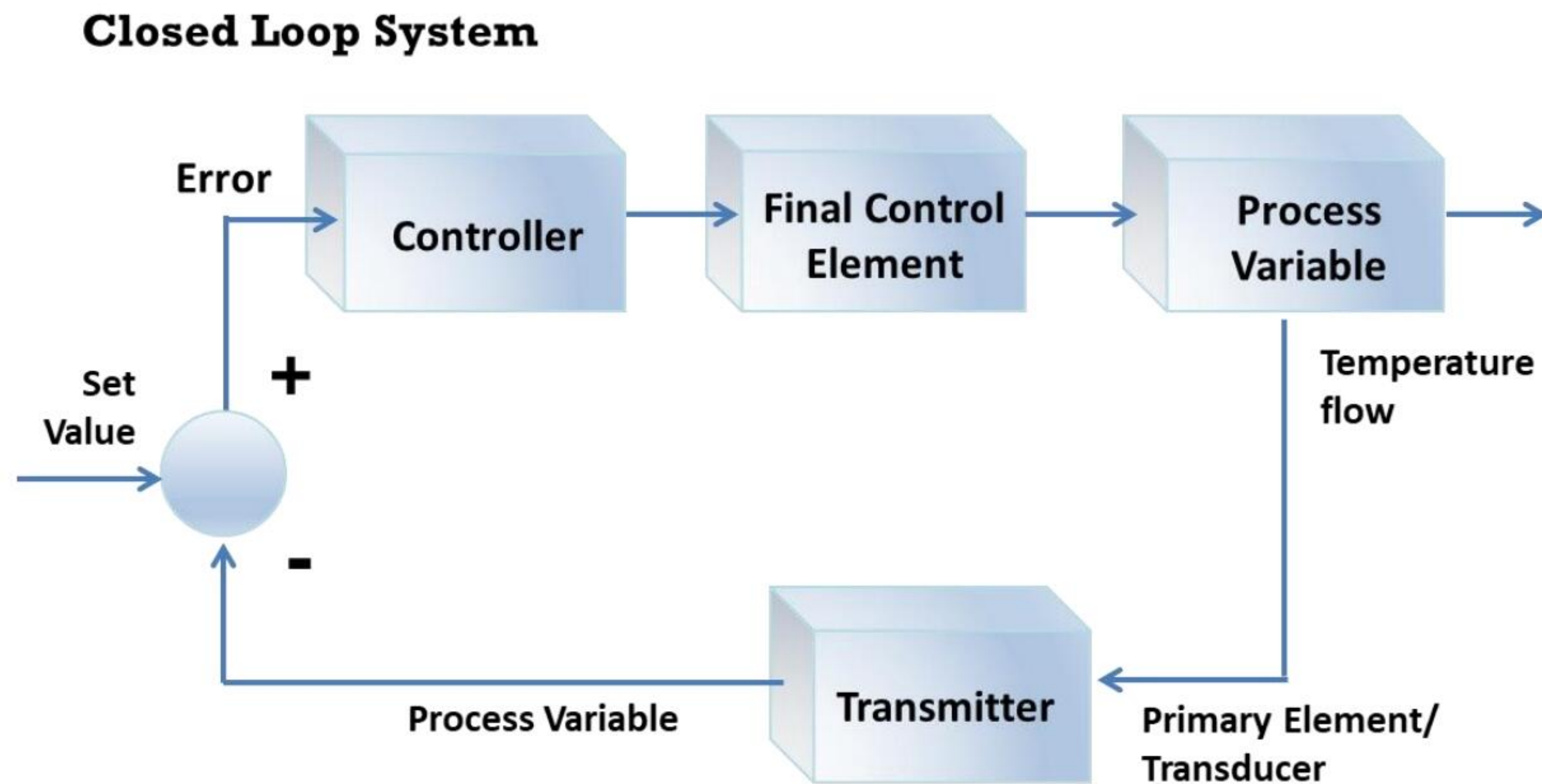
Figure 18.77: BPCS architecture
