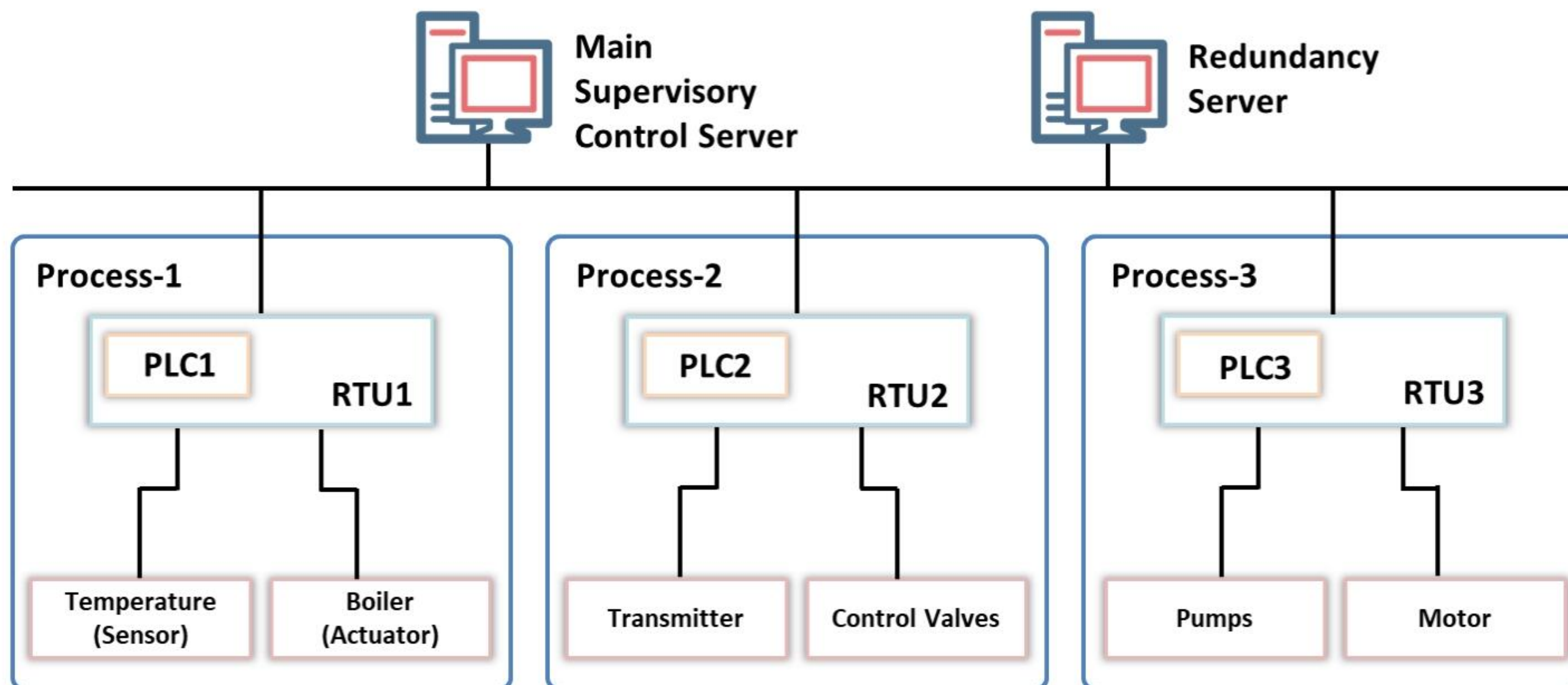
Figure 18.74: DCS architecture
