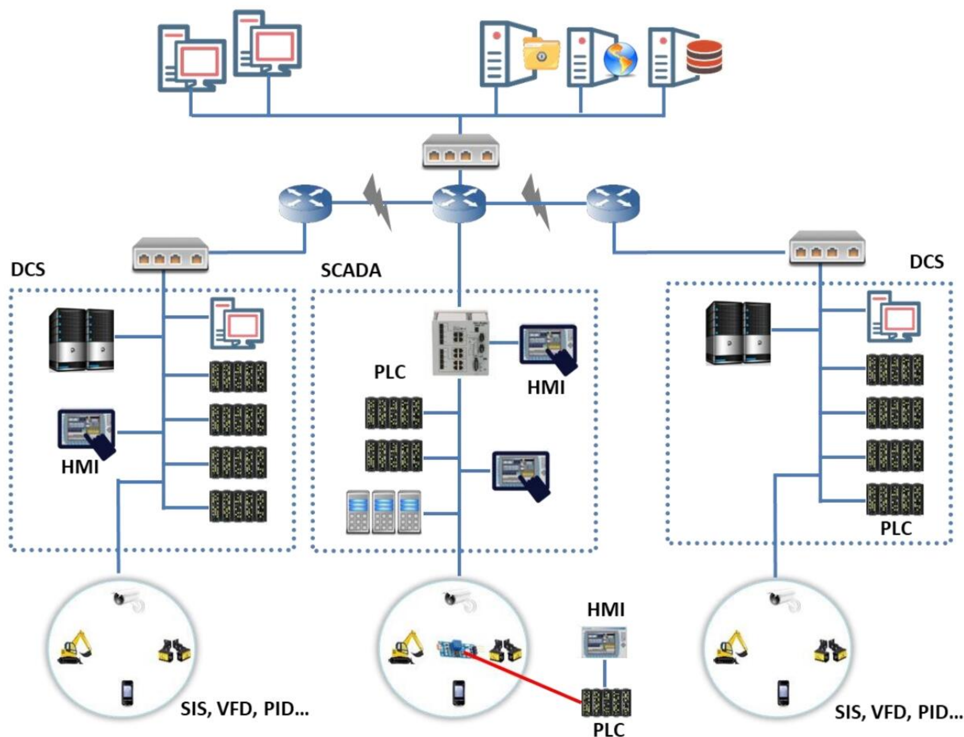
Figure 18.73: ICS architecture
