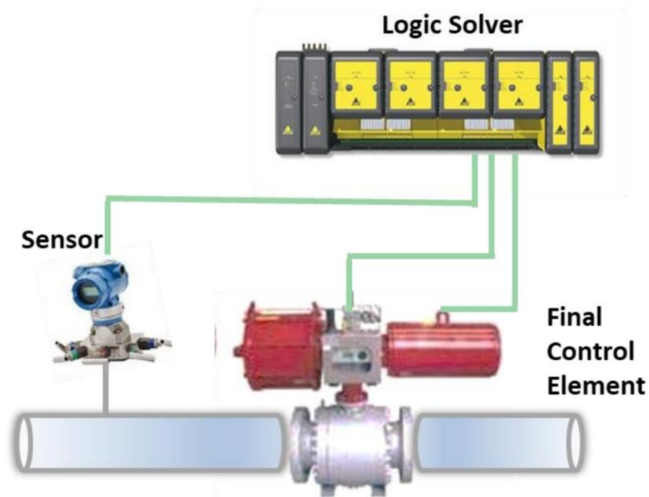
Figure 18.79: SIS architecture
