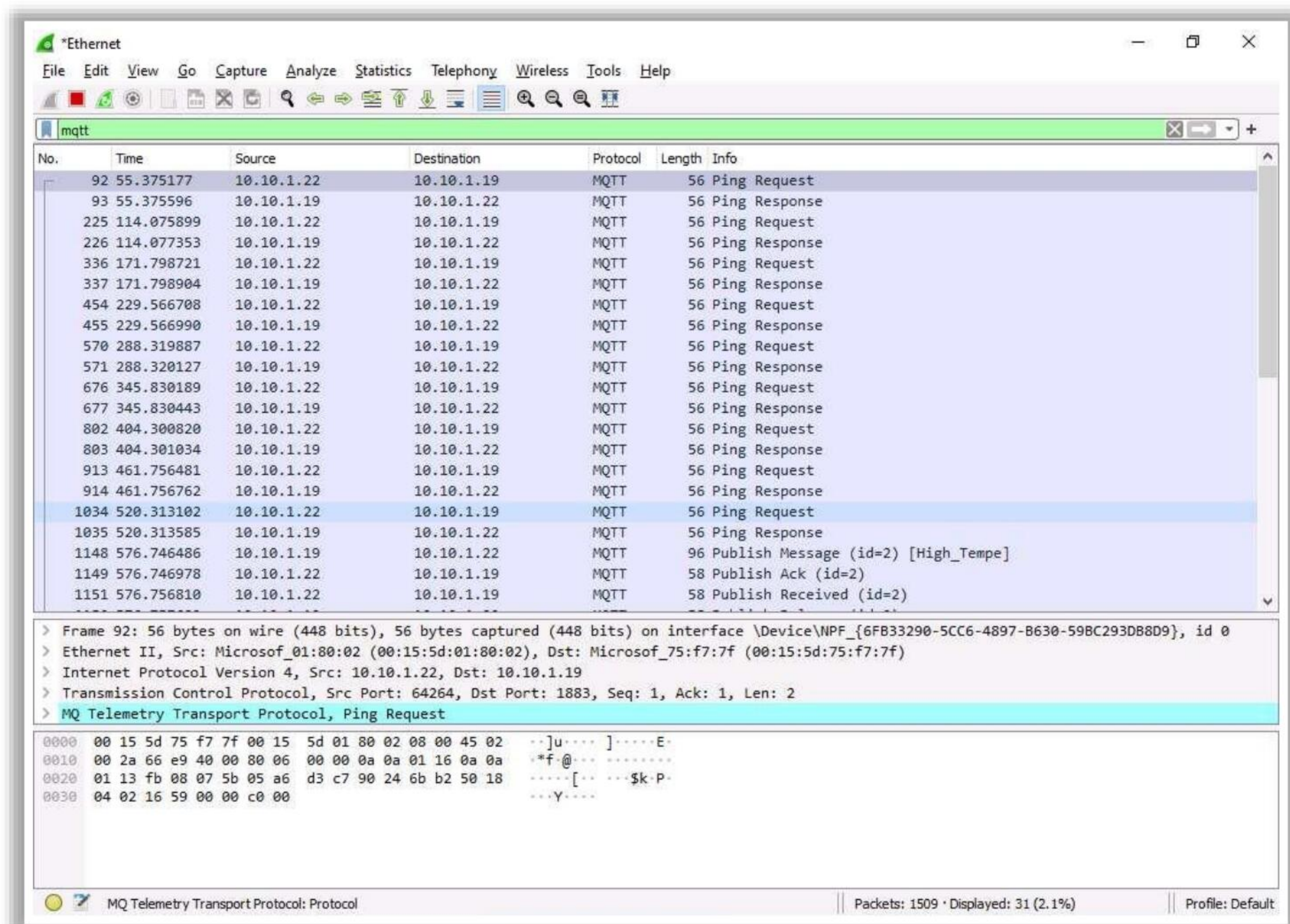
Figure 18.36: Screenshot of Wireshark
