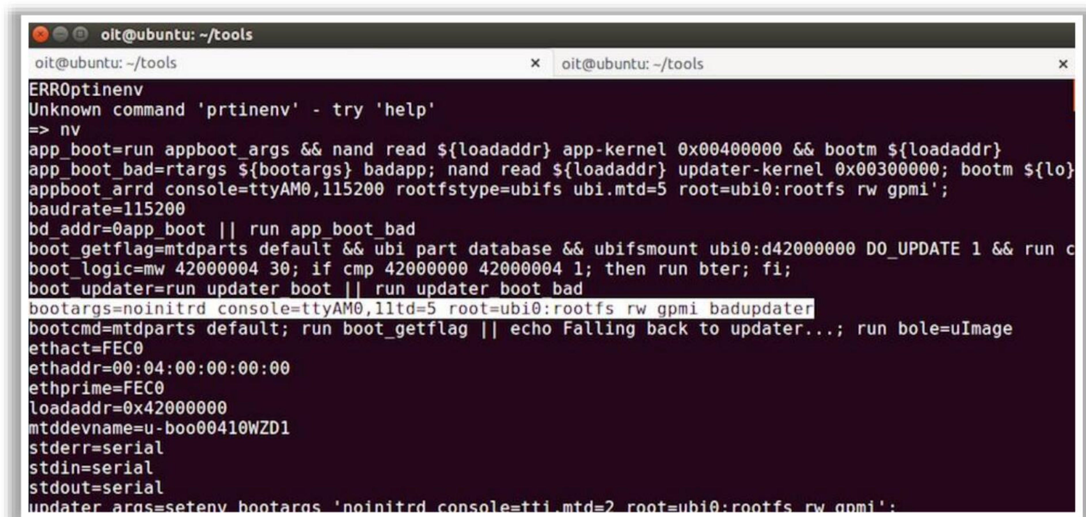
Figure 18.55: Screenshot showing the output of bootlogs on the console
