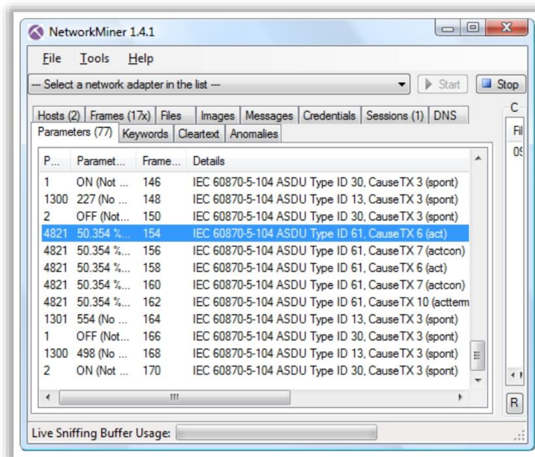
Figure 18.106: Screenshot of NetworkMiner
