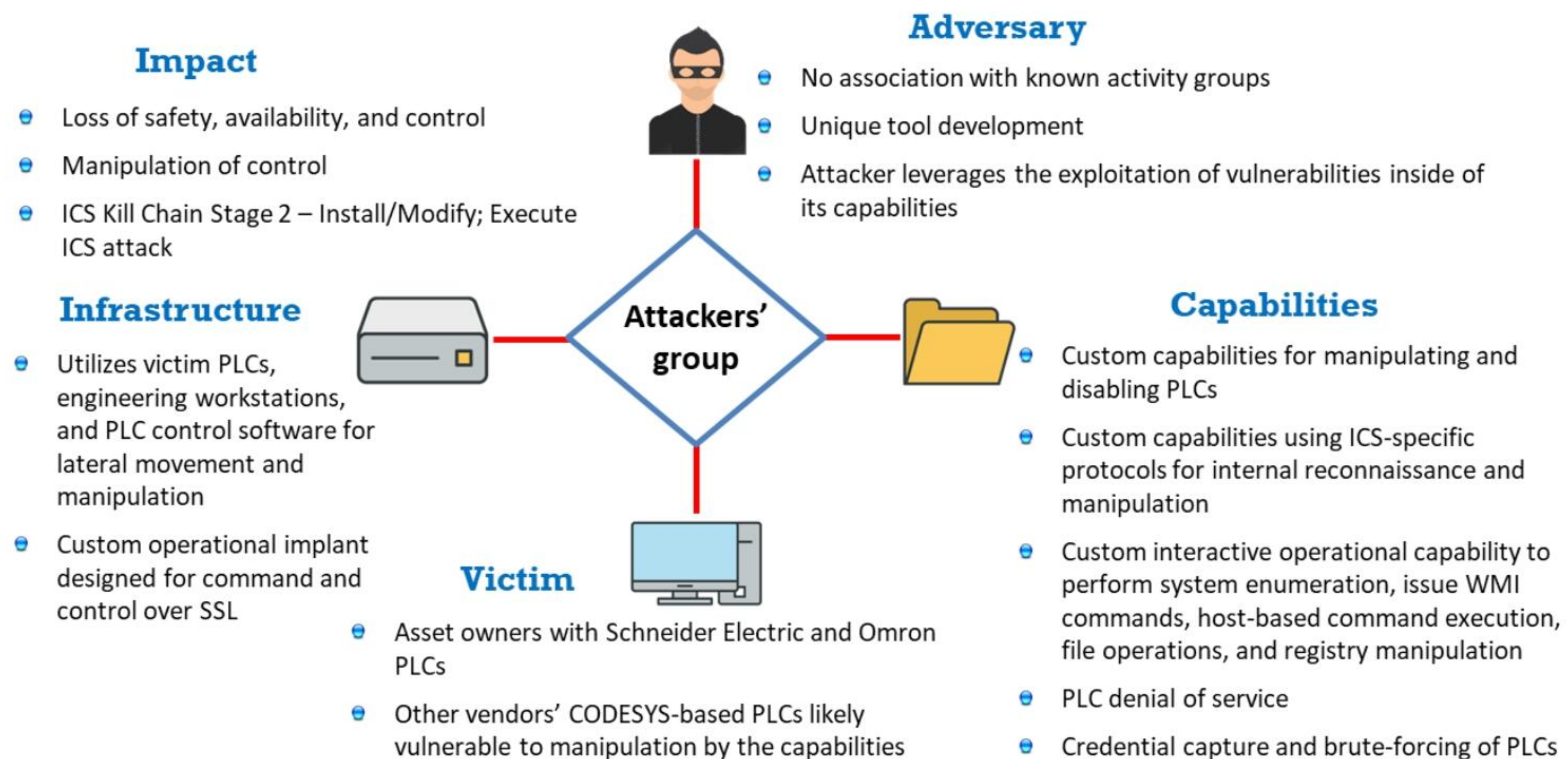
Figure 18.88: Functionality of PIPEDREAM
