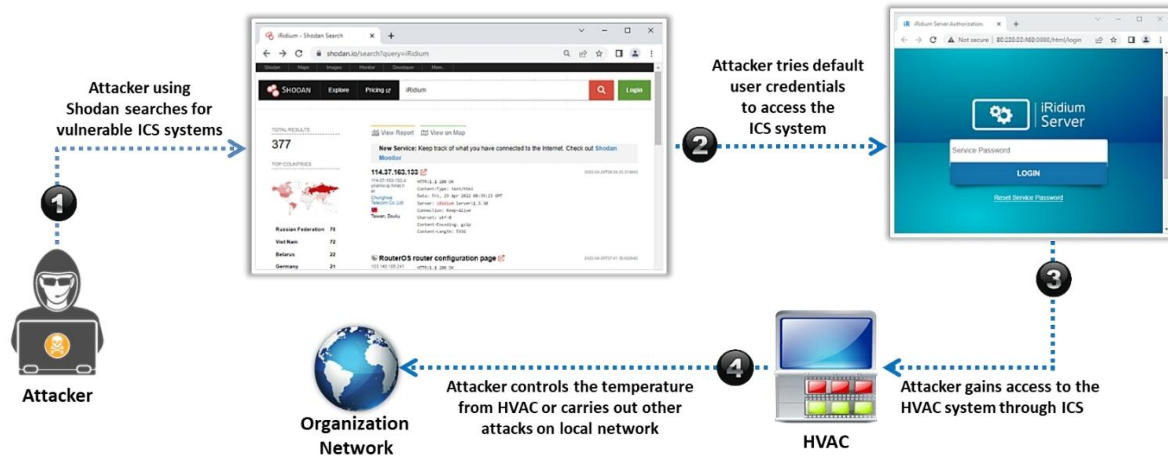
Figure 18.10: Exploiting HVAC system
