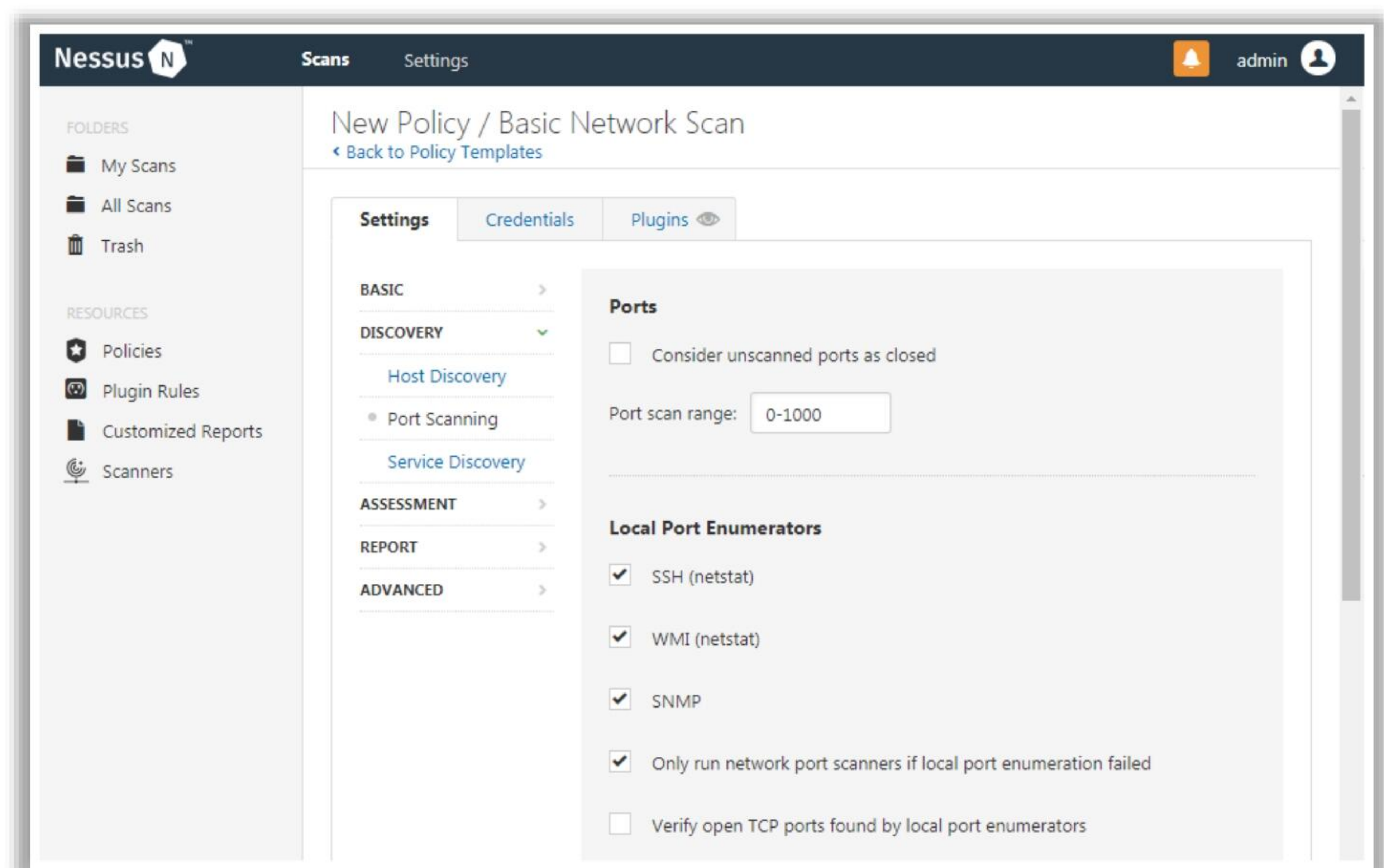
Figure 18.97: Screenshot of Nessus showing New Policy settings
