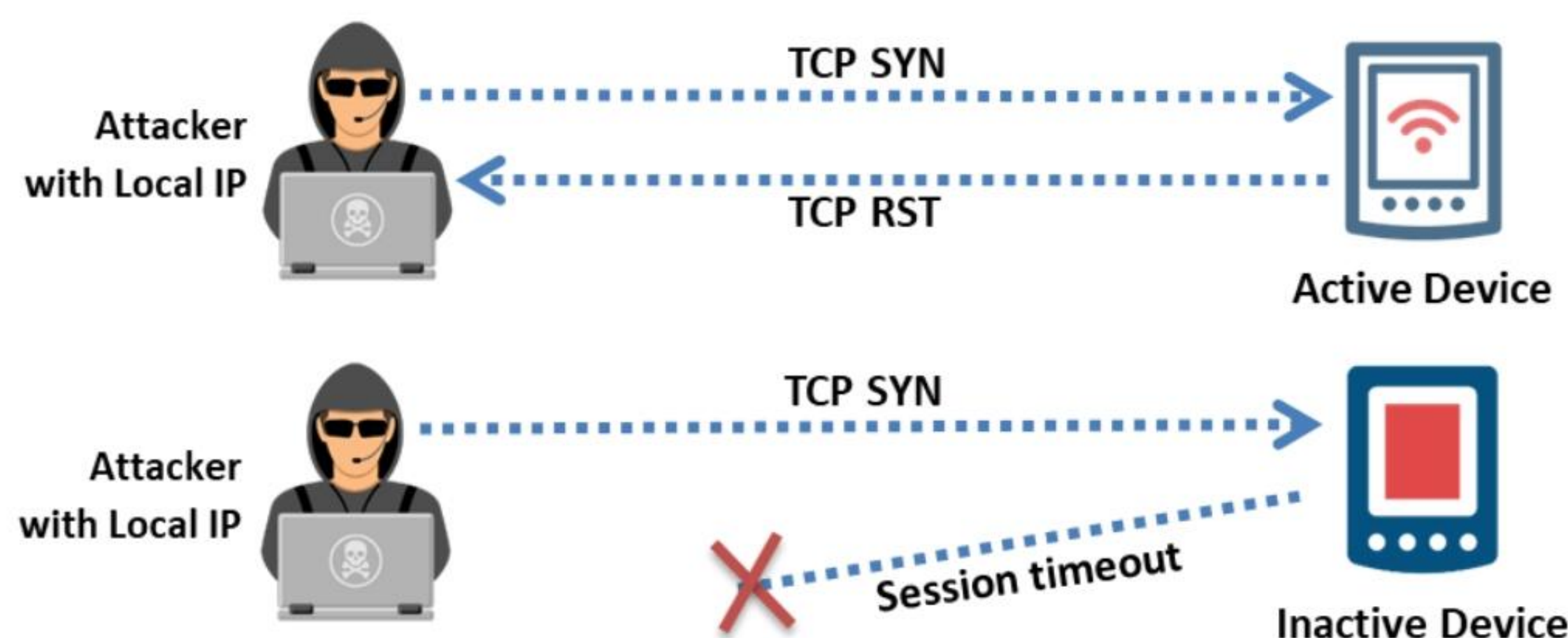
Figure 18.15: Discovering the local IoT devices
