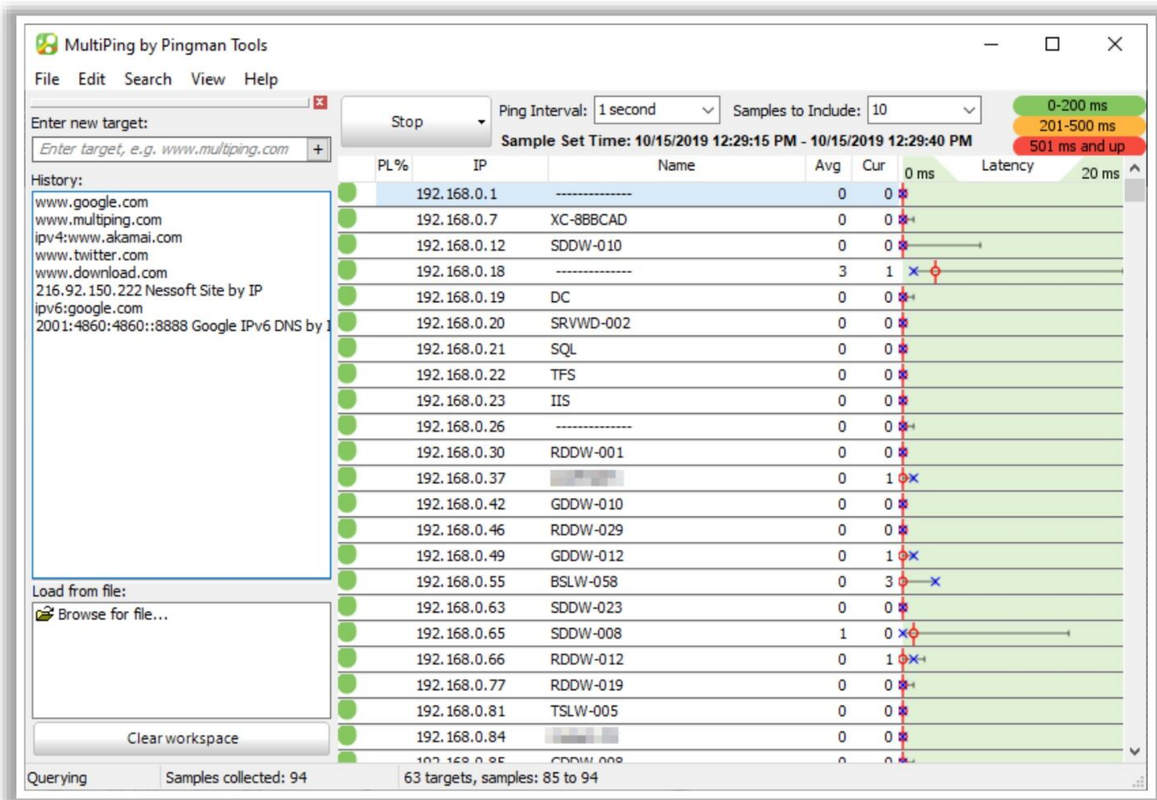
Figure 18.25: Scanning using MultiPing
