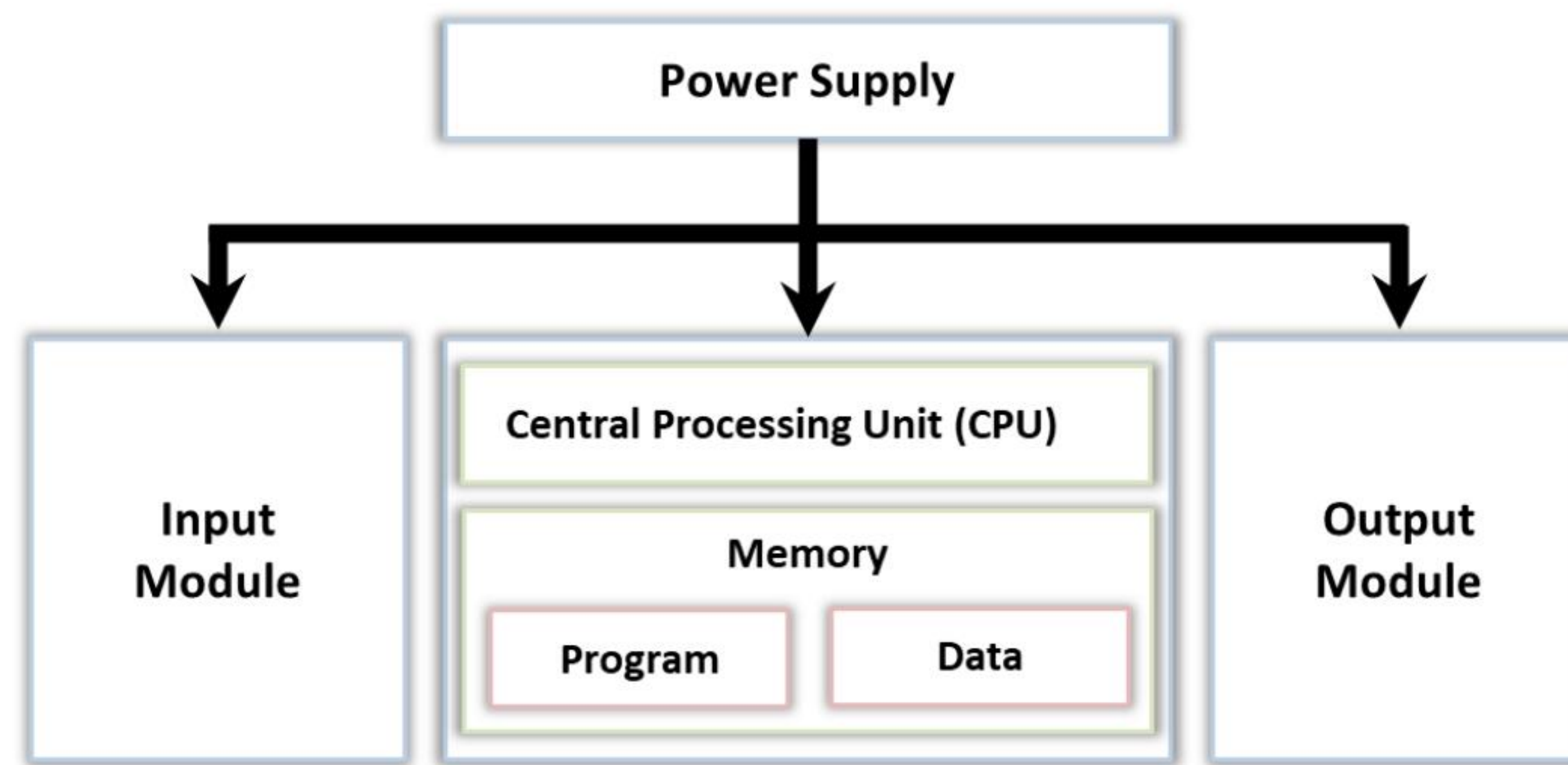
Figure 18.76: PLC architecture
