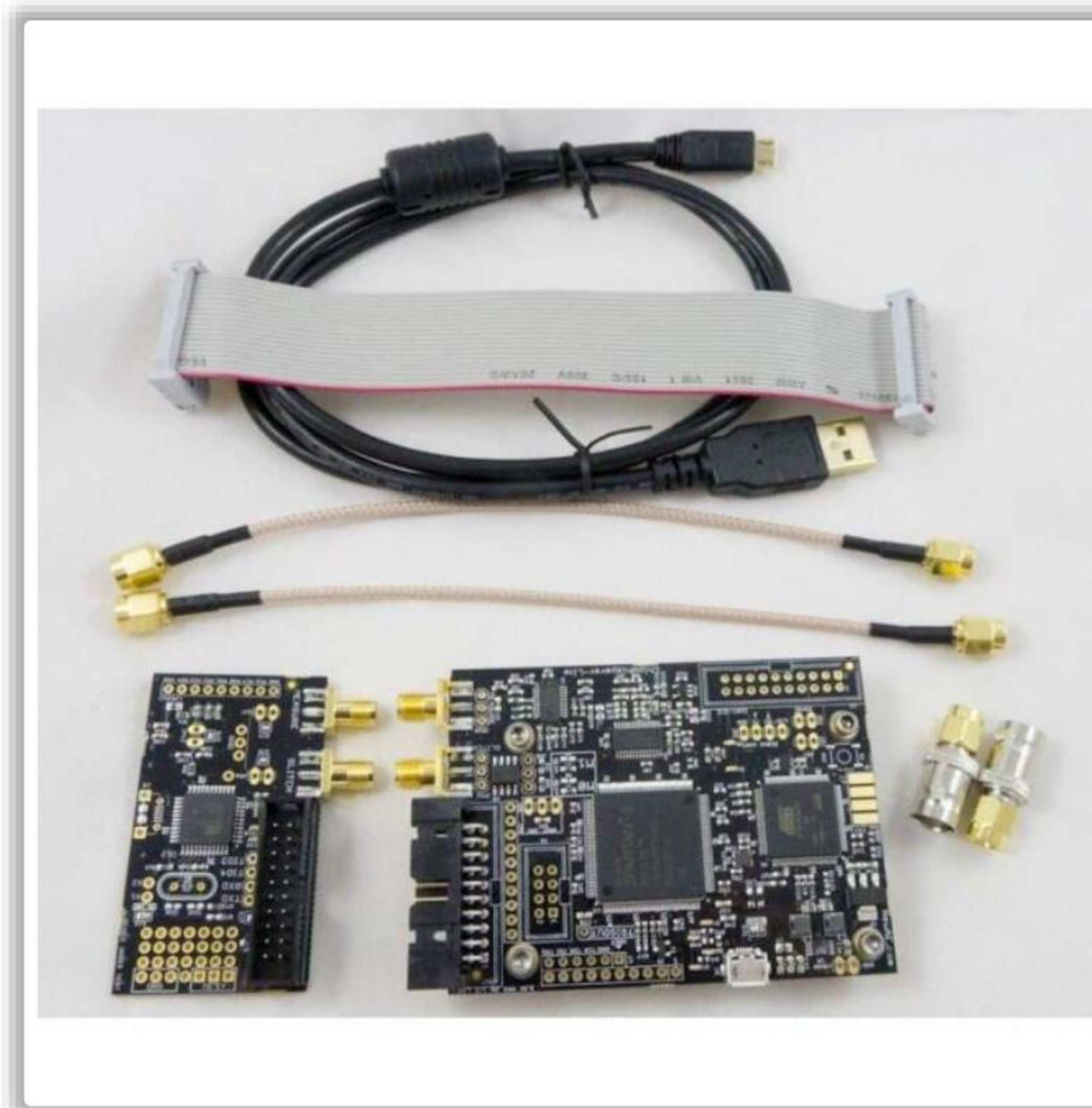
Figure 18.47: ChipWhisperer Lite
