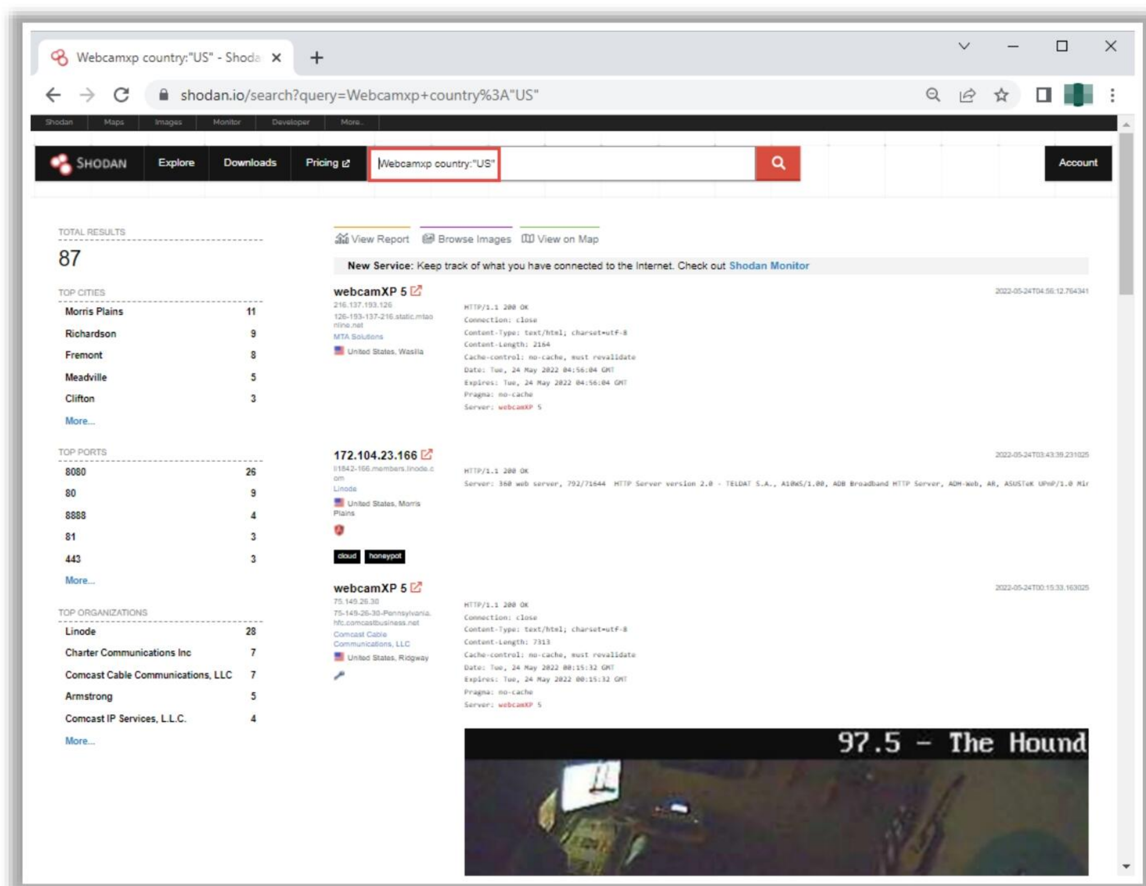
Figure 18.23: Information gathering using Shodan
