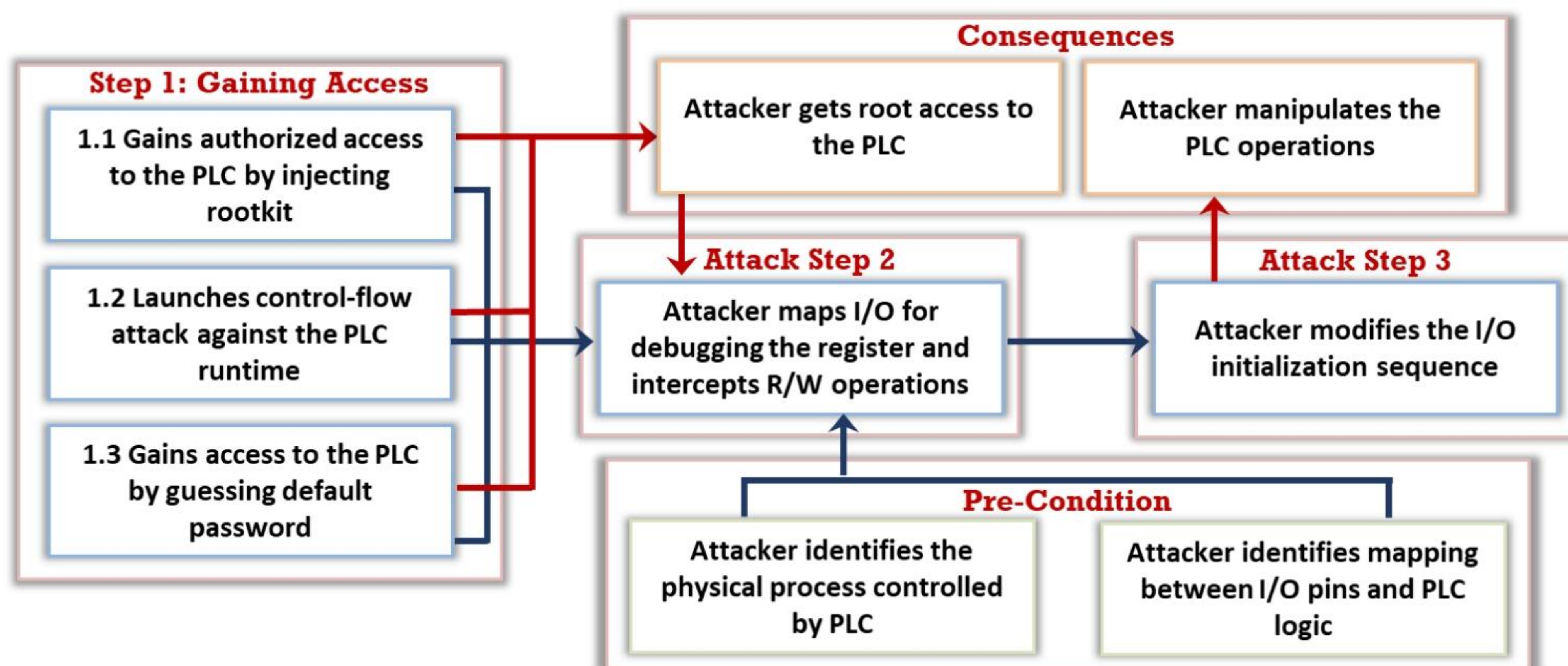
Figure 18.82: Hacking PLC through PLC rootkit attack
