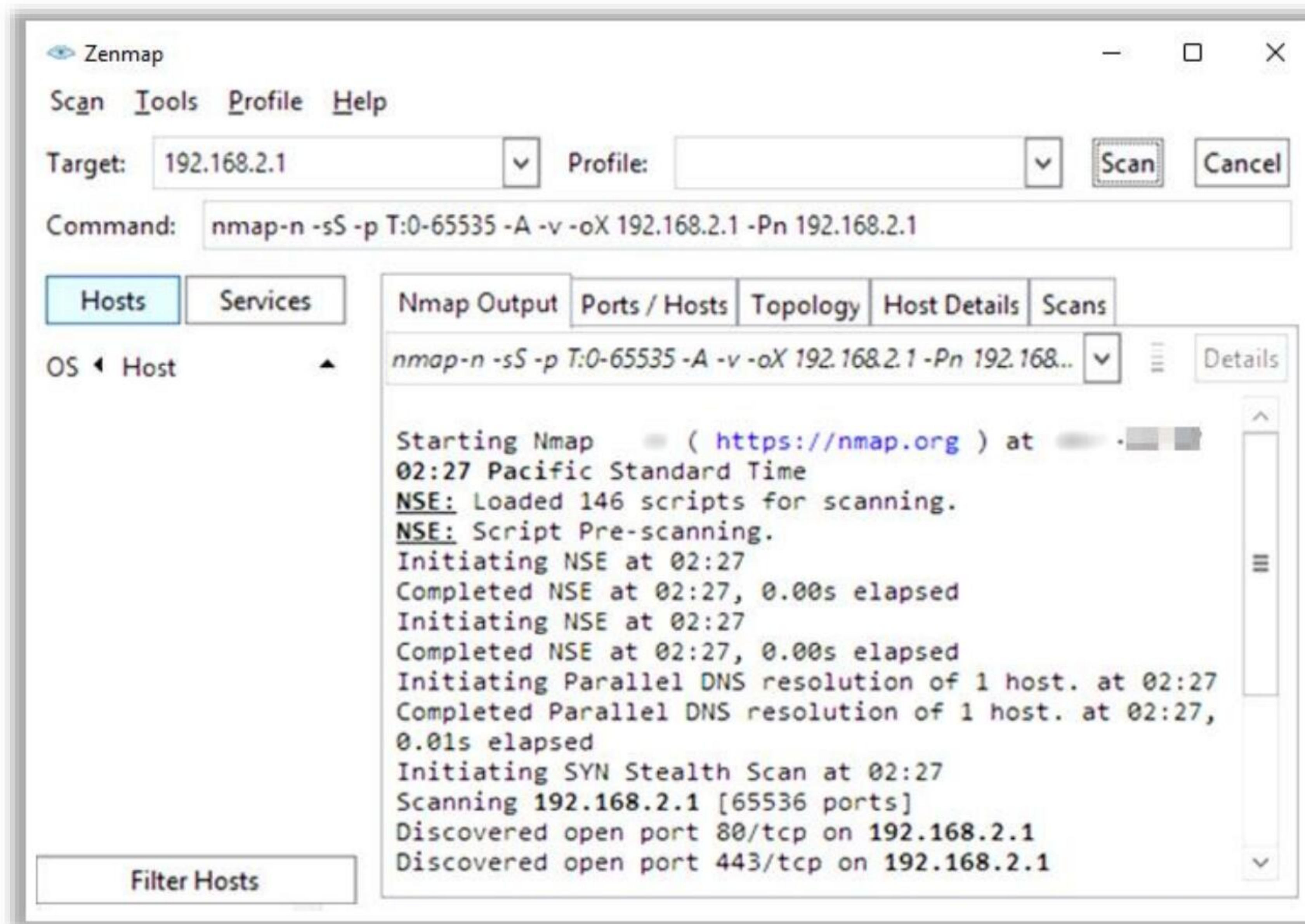
Figure 18.32: Scanning using Nmap
