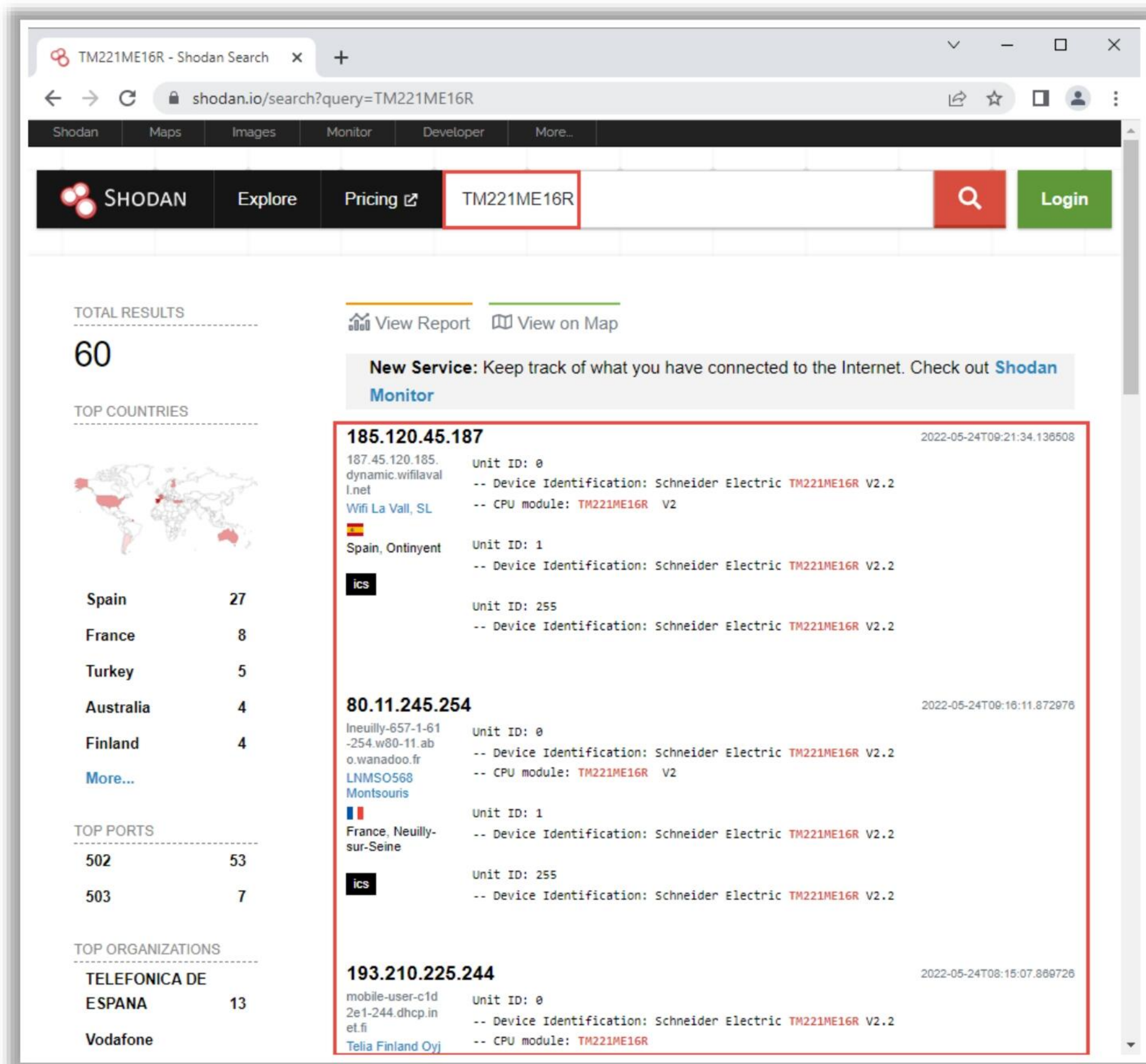
Figure 18.112: Screenshot of Shodan showing Schneider Electric TM221 PLCs
