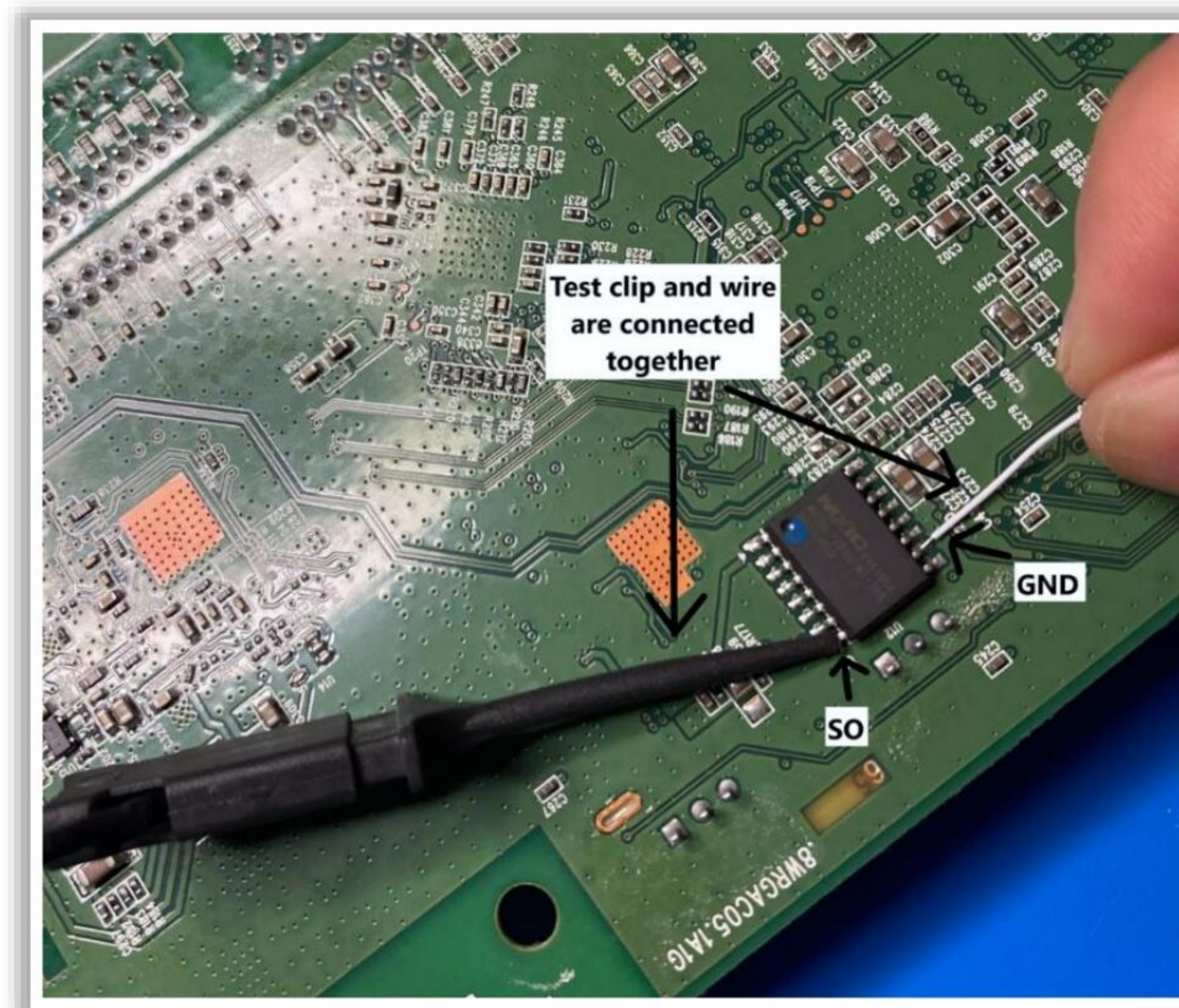
Figure 18.53: Screenshot showing NAND glitching
