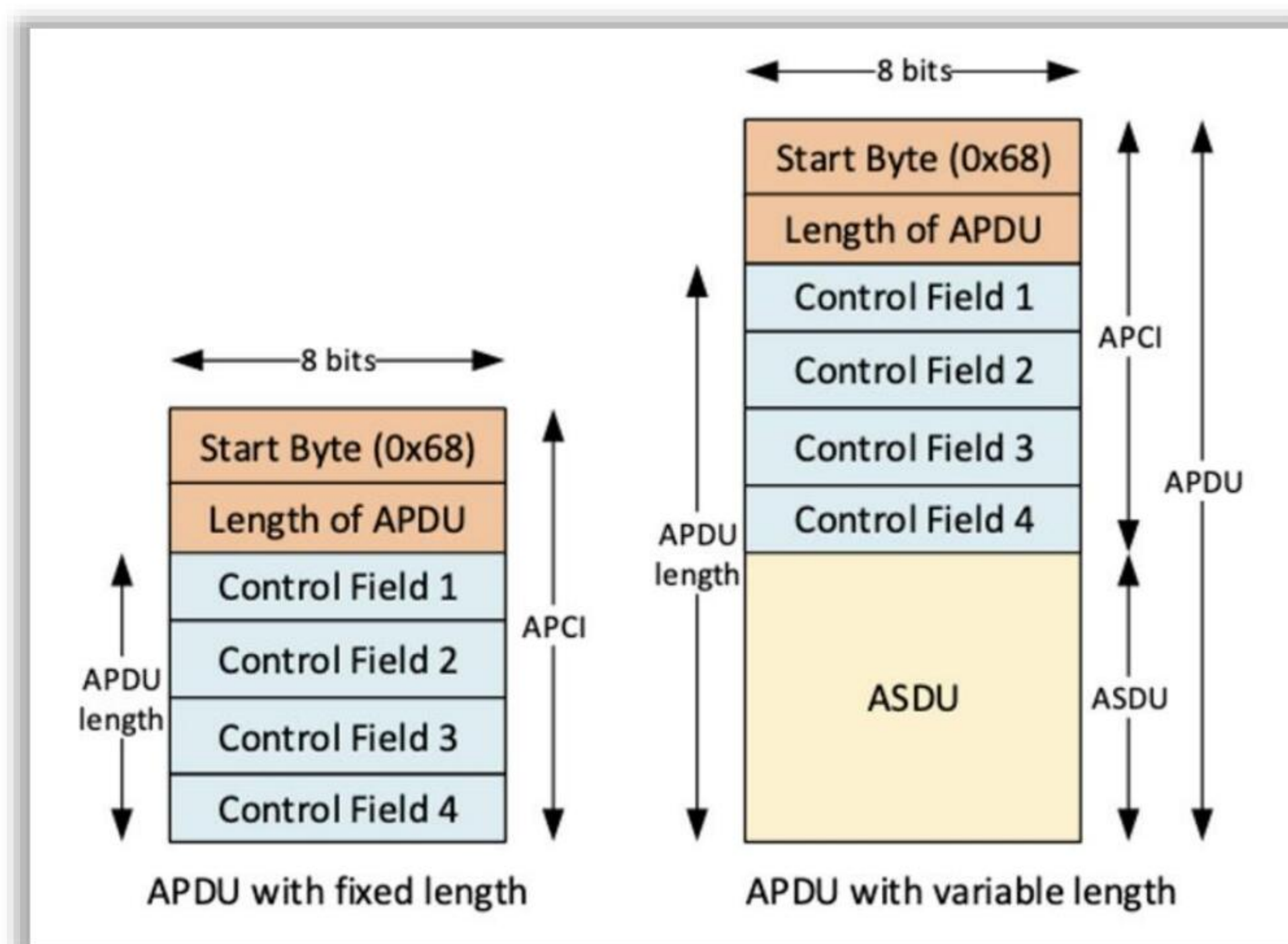
Figure 18.91: Frame format of APDU
