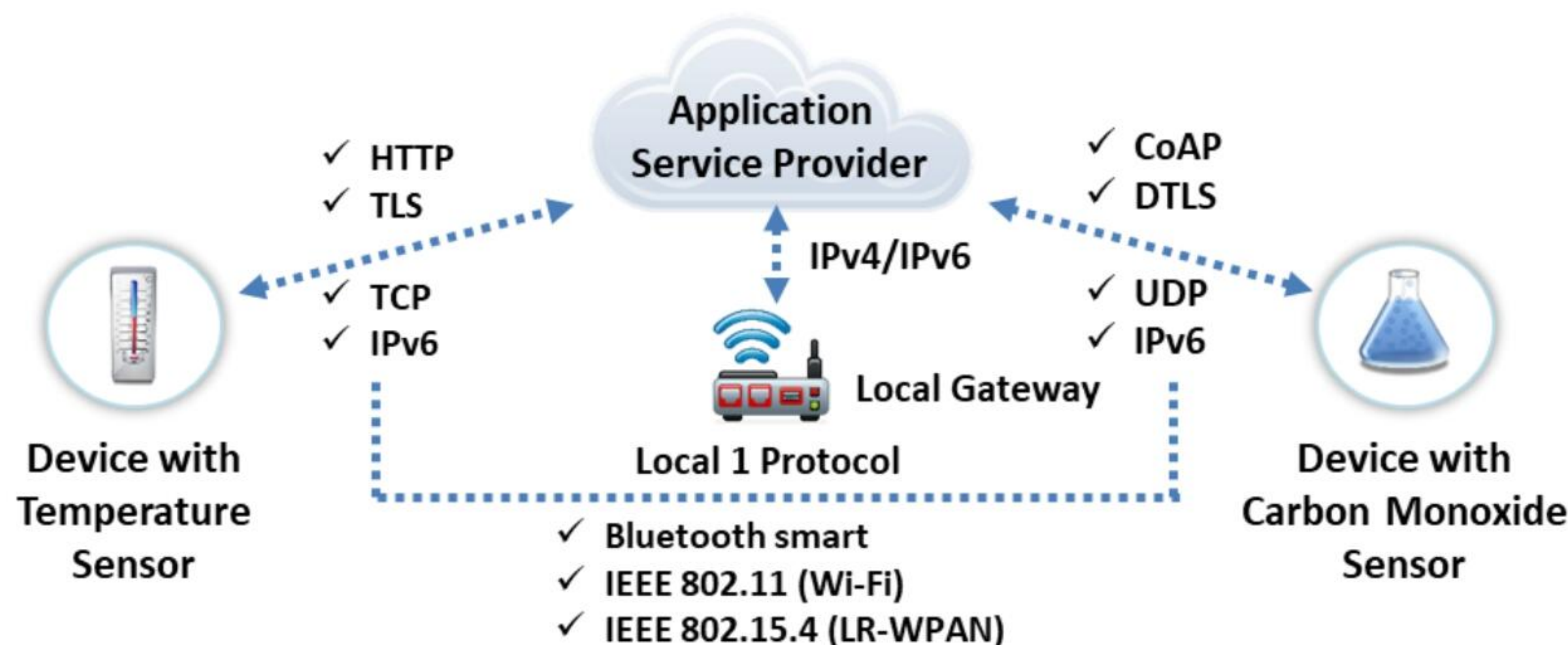
Figure 18.5: IoT device-to-gateway communication model
