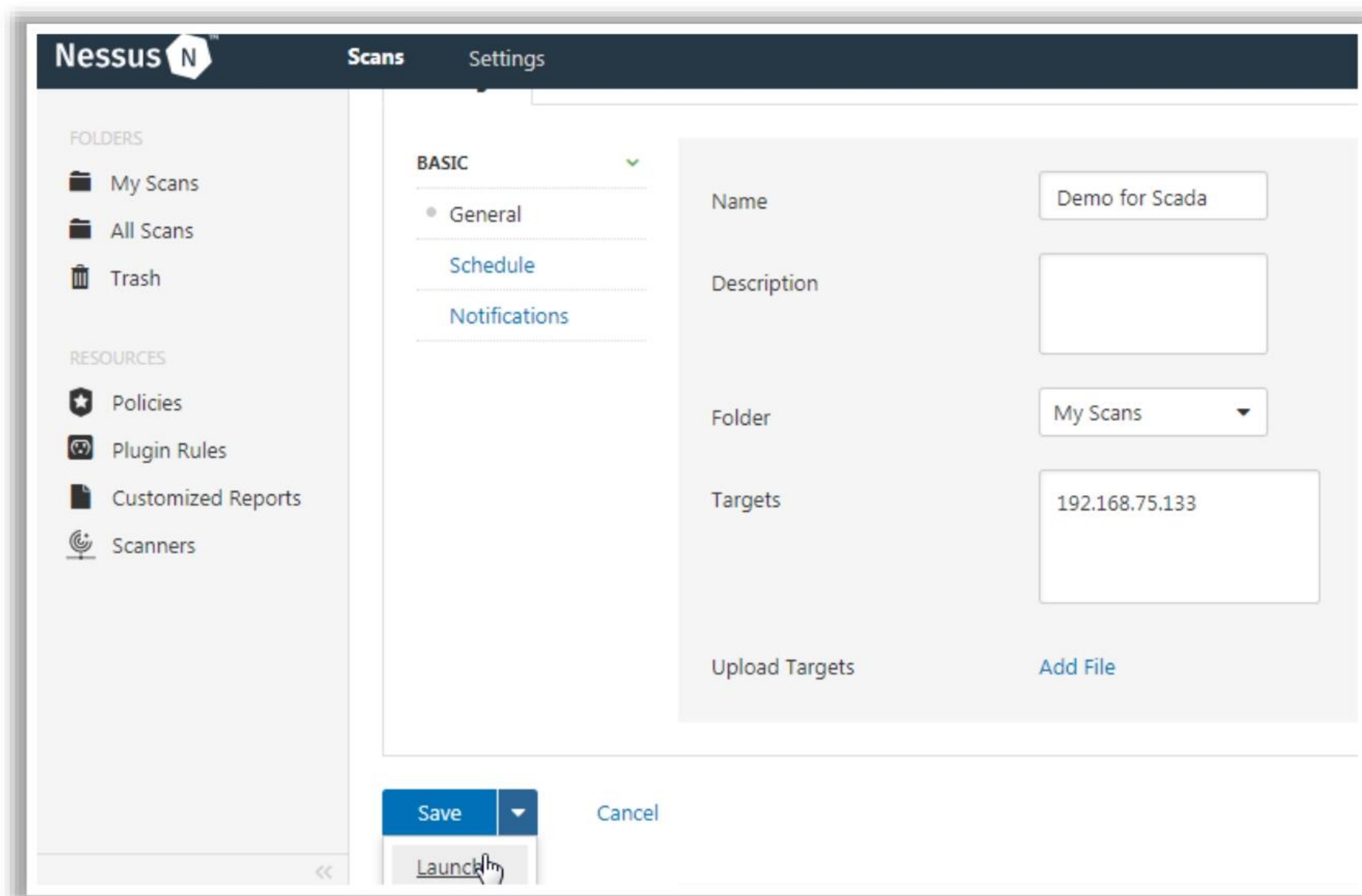
Figure 18.100: Screenshot of Nessus BASIC scan settings
