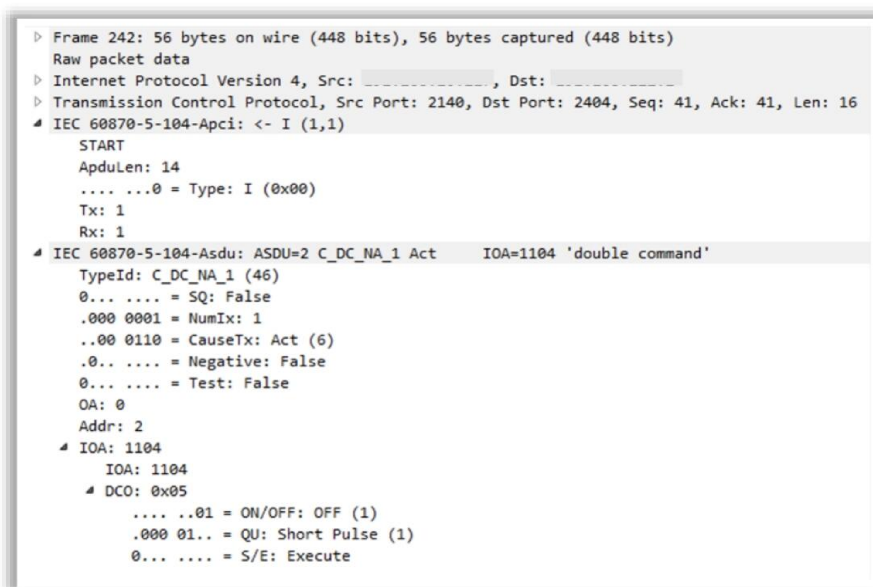
Figure 18.92: Screenshot displaying a crafted ASDU message
