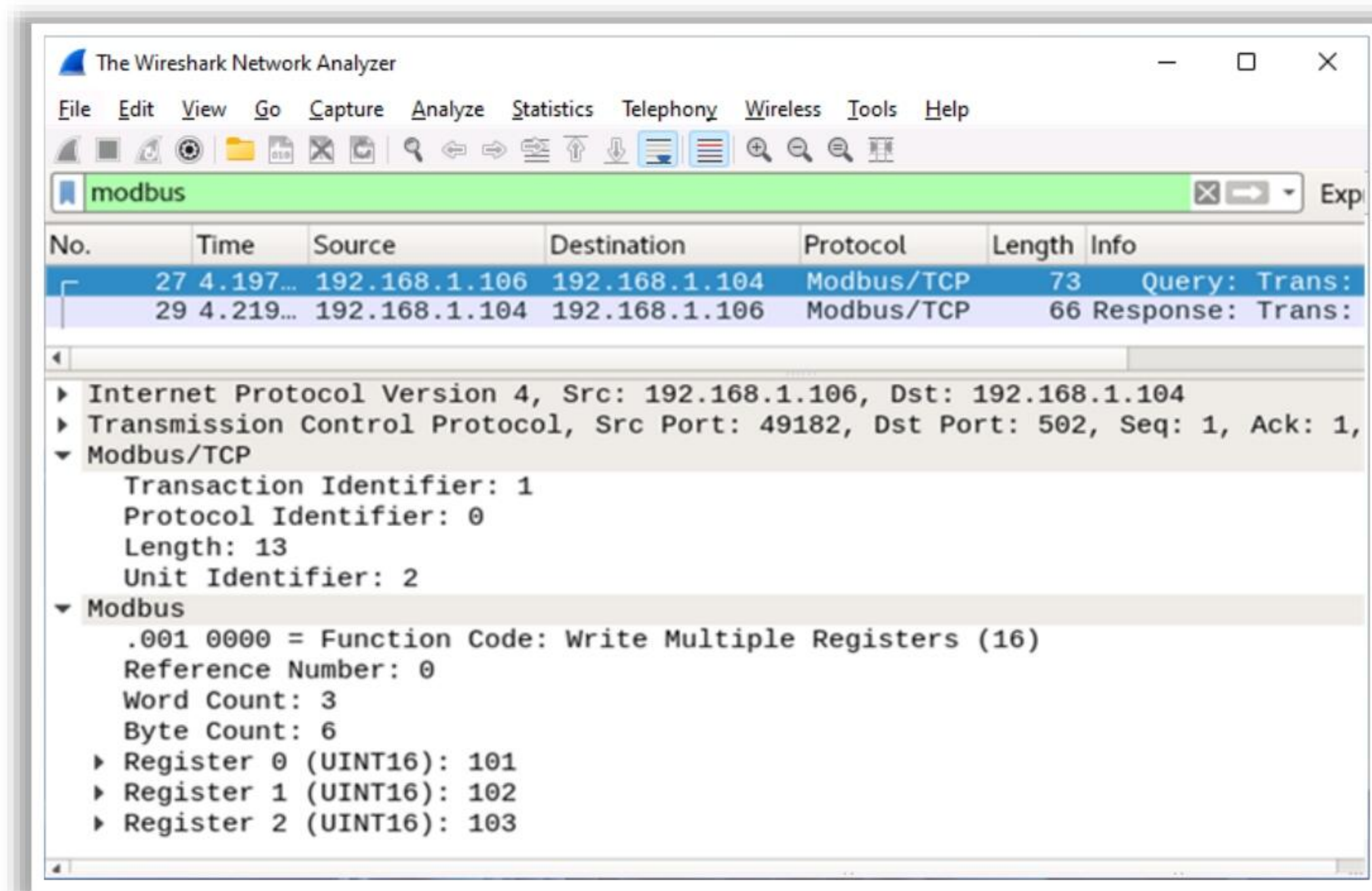
Figure 18.107: Screenshot of Wireshark
