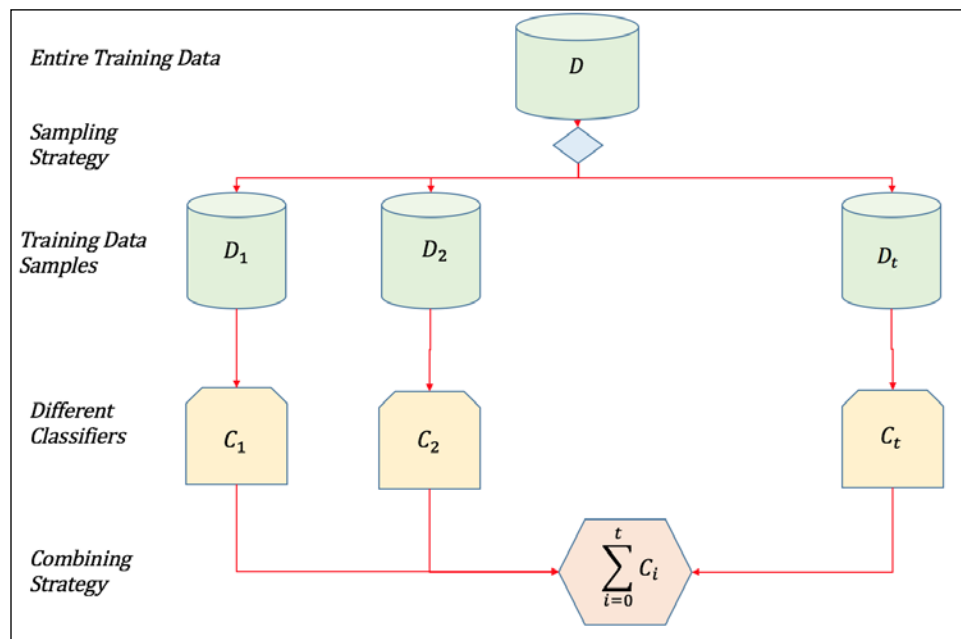
Figure 9: Illustration of ensemble learning strategies
