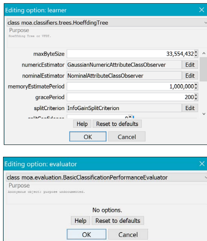
Figure 5. MOA graphical interface for prequential classification task. Within the Configure task, you must choose a learner, locate the data stream (details not shown), and select an evaluator
