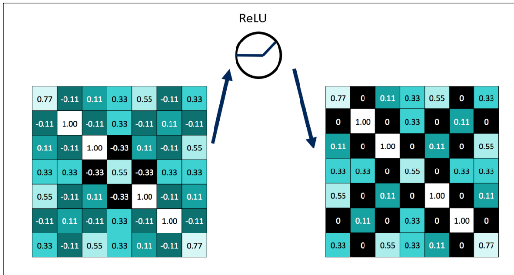
Figure 26: Transformation using ReLu.
