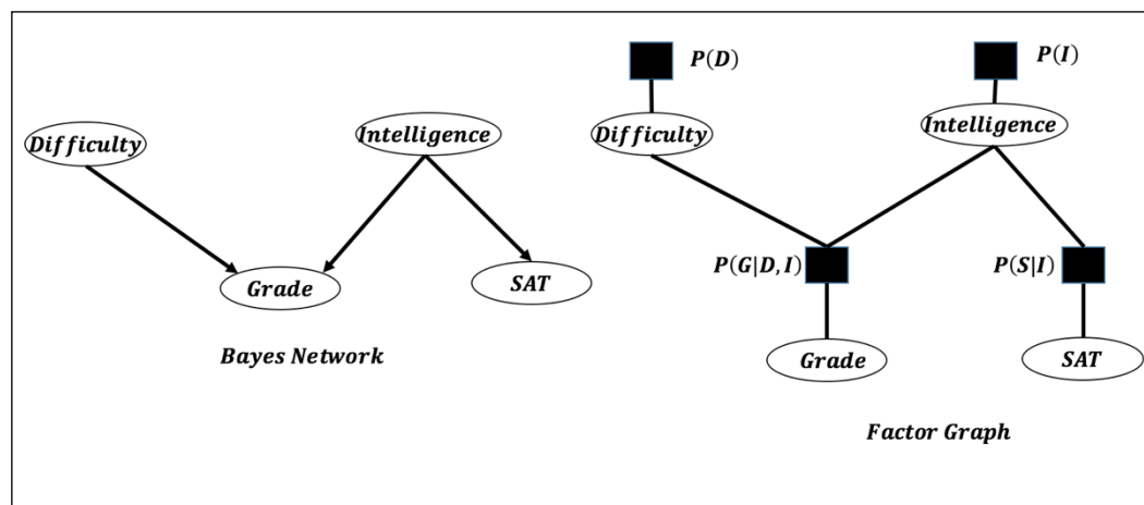
Figure 9. Factor graph of simplified "Student" network
