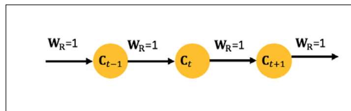
Figure 36: Building blocks of LSTM where the feedback matrix is set to 1.
