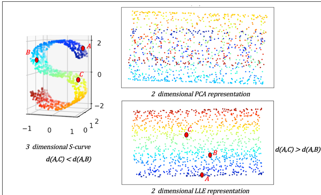
Figure 3: Data representation after PCA and manifold learning
