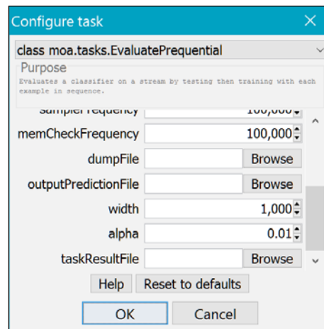
Figure 4. MOA graphical interface for configuring prequential evaluation for classification which includes setting the window width
