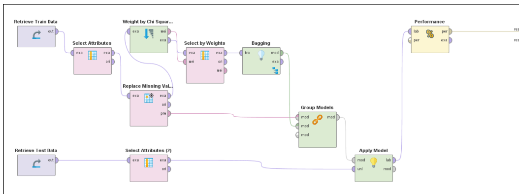
Figure 18: RapidMiner process diagram
