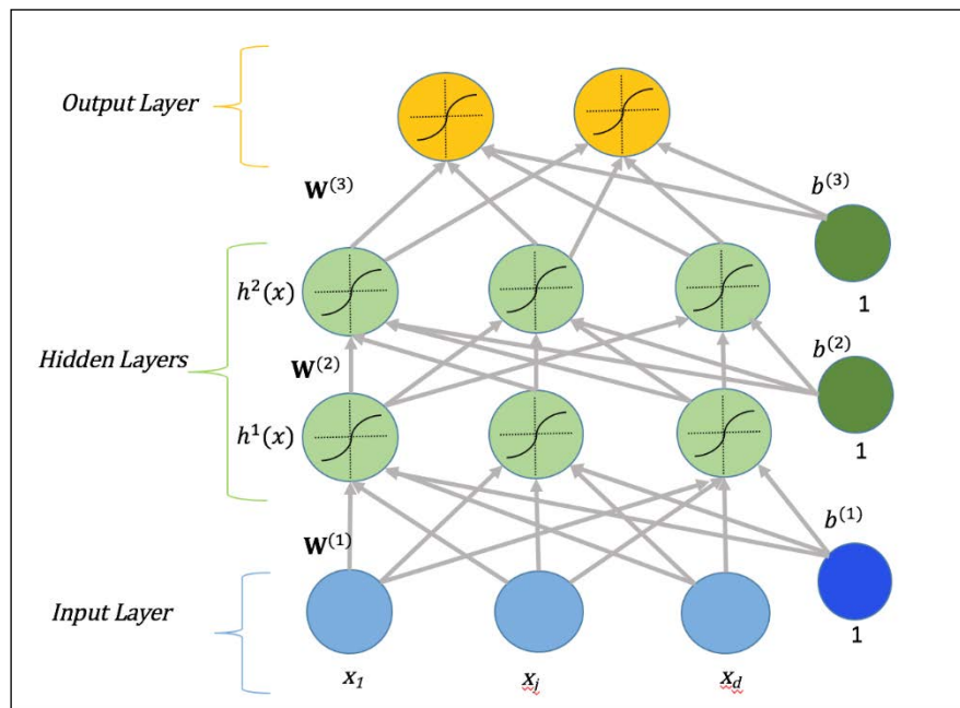
Figure 2. Multilayer neural network showing an input layer, two hidden layers, and an output layer.
