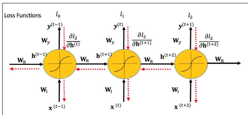
Figure 34: Backpropagation through time.
