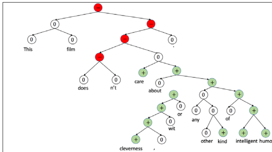
Figure 22: A complex sentence showing words with negative (as red circle), positive (green circle), and neutral (empty with 0) connected through RNN with overall negative sentiment.
