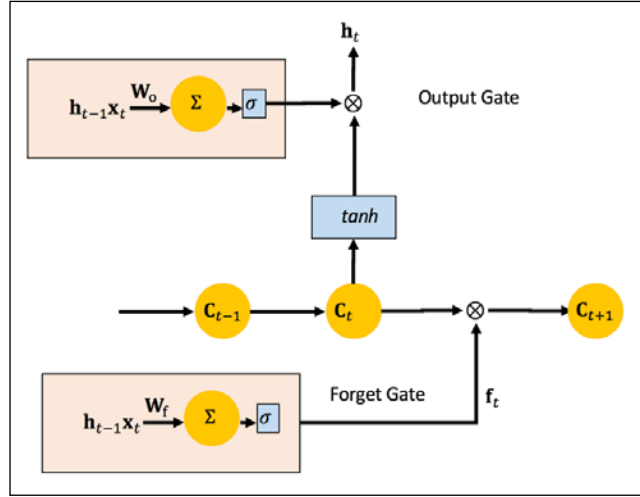
Figure 38: Building block Forget Gate addition to LSTM.
