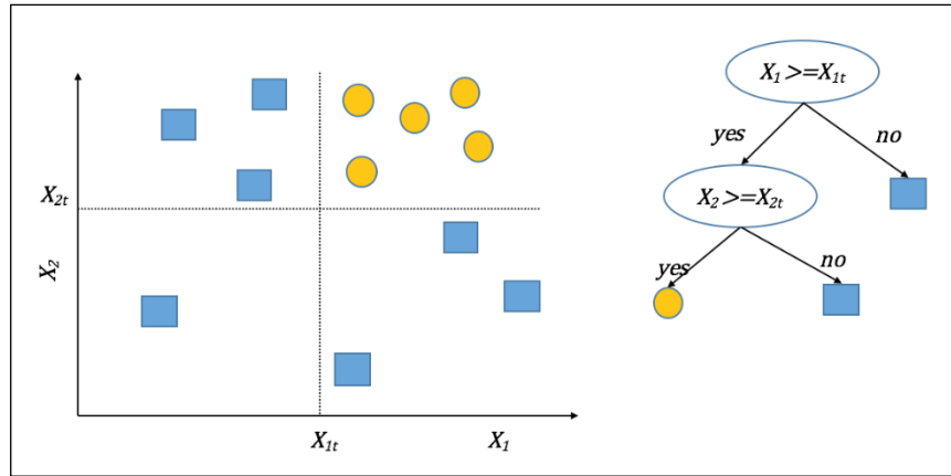
Figure 5: Shows a two-dimensional binary classification problem and a Decision Tree induced using splits at thresholds X_{1t} and X_{2t} , respectively
