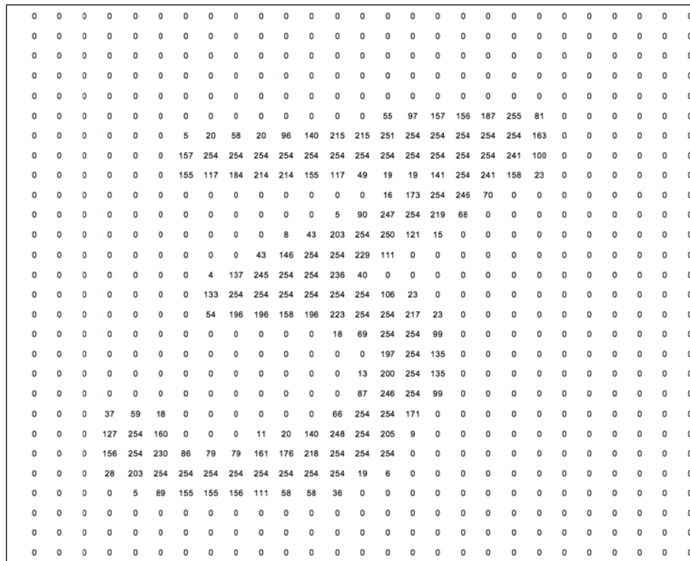
Figure 8: Showing digit 3 with pixel values distributed in a 28 by 28 matrix ranging from 0 to 254.
