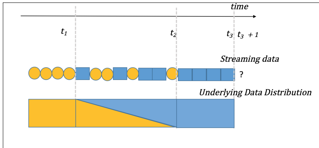
Figure 1 Concept drift illustrated by the gradual change in color from yellow to blue in the bottom panel. Sampled data reflects underlying change in data distribution, which must be detected and a new model learned.
