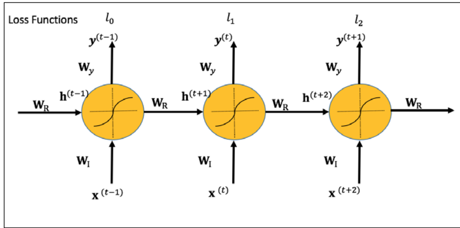
Figure 33: Chain of neurons with feedbacks connected together.
