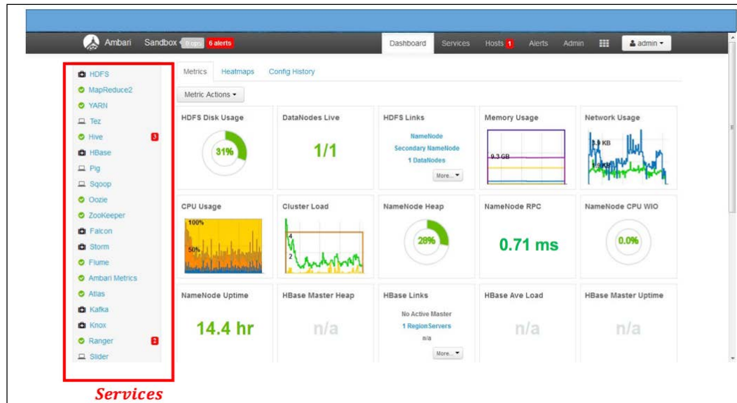
Figure 2: Ambari dashboard user interface
