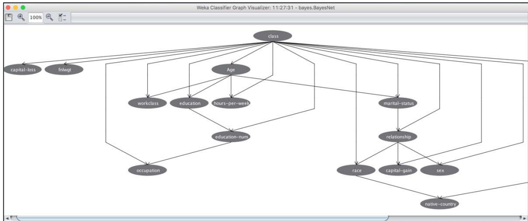
Figure 27: Visualization of learned structure of the Bayesian network.
