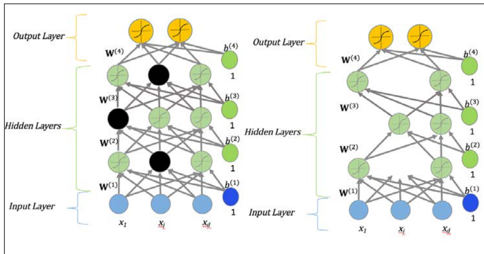
Figure 16: Deep learning with dropout indicated by dropping certain units with dark shading.
