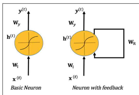
Figure 32: Difference between an artificial neuron and a neuron with feedback.
