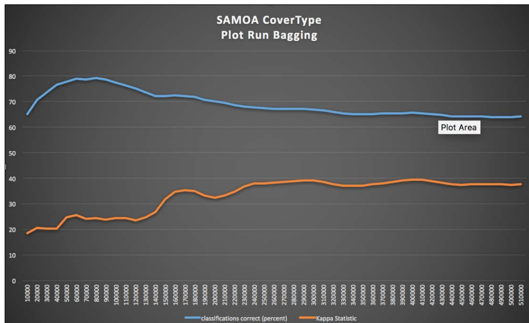
Figure 25: Bagging model performance
