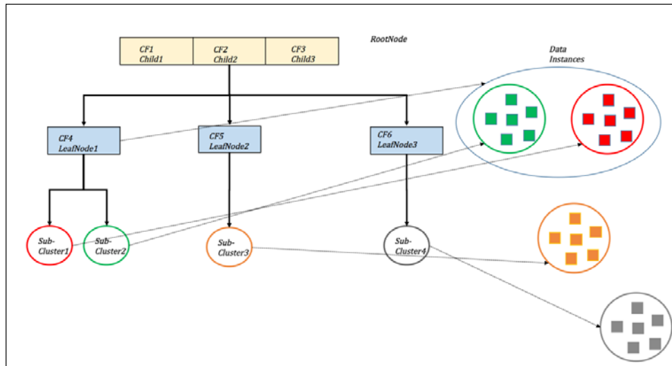
Figure 3 An example Clustering Feature Tree illustrating hierarchical structure.
