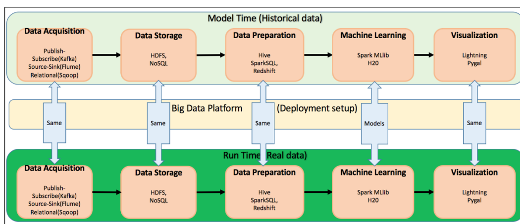
Figure 6: Model time and run time components for Big Data and providers
