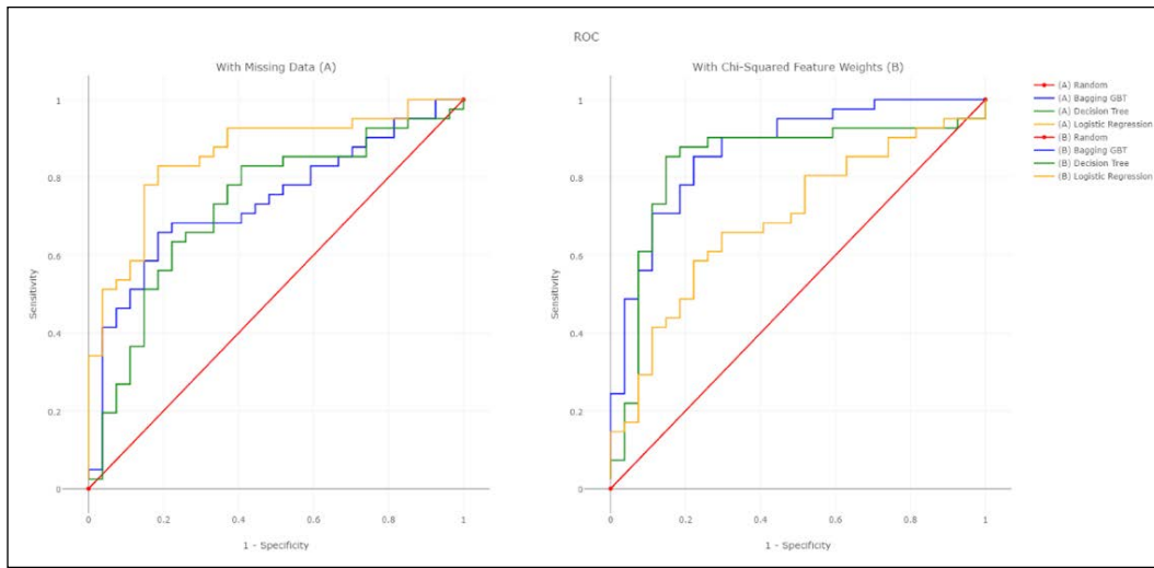
Figure 19: ROC Performance curves for experiment using Missing Data
