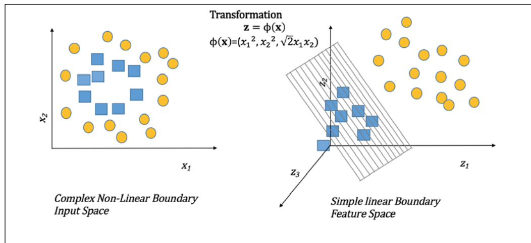
Figure 8: Kernel transformation illustrating how two-dimensional input space can be transformed using a polynomial transformation into a three-dimensional feature space where data is linearly separable.
