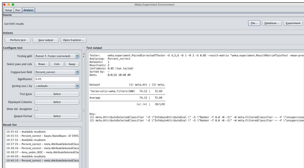
Figure 14: WEKA Experimenter results showing two algorithms compared on metric of percent correct or accuracy using paired-t test.
