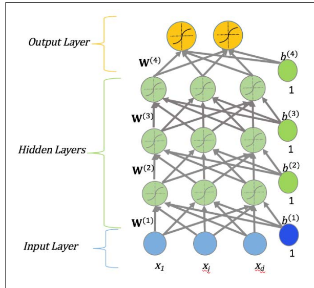
Figure 12: Final tuning or supervised learning.
