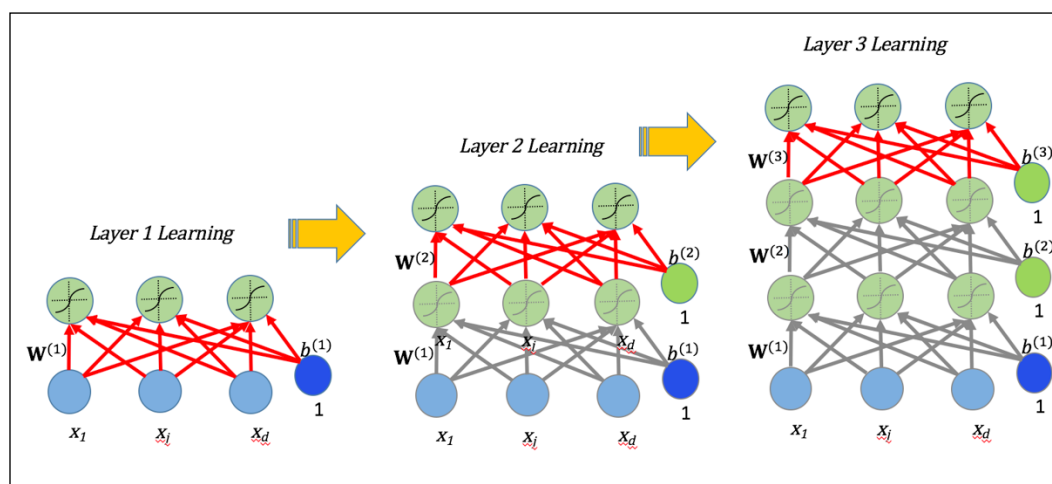
Figure 11: Layer wise incremental learning through unsupervised learning.
