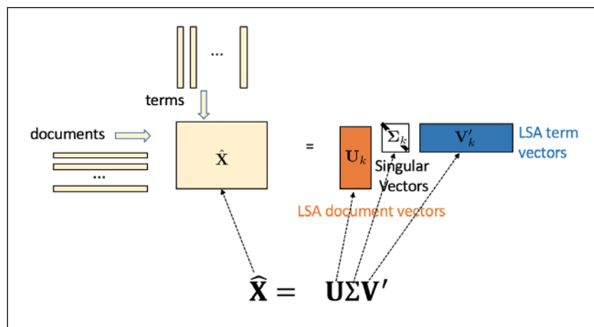
Figure 12: SVD factorization of input document-terms into LSA document vectors and LSA term vectors
