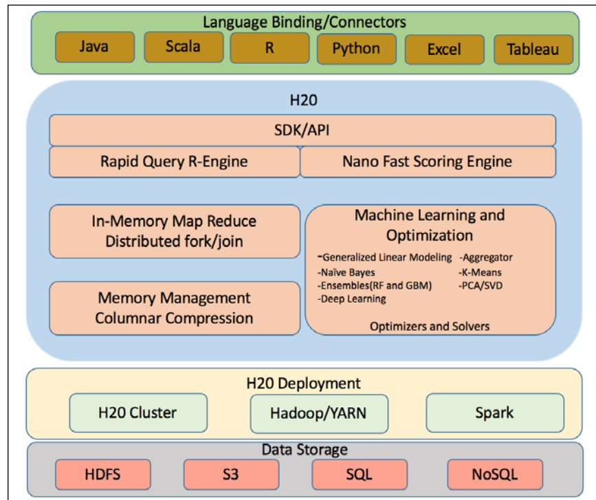
Figure 7: H2O high level architecture
