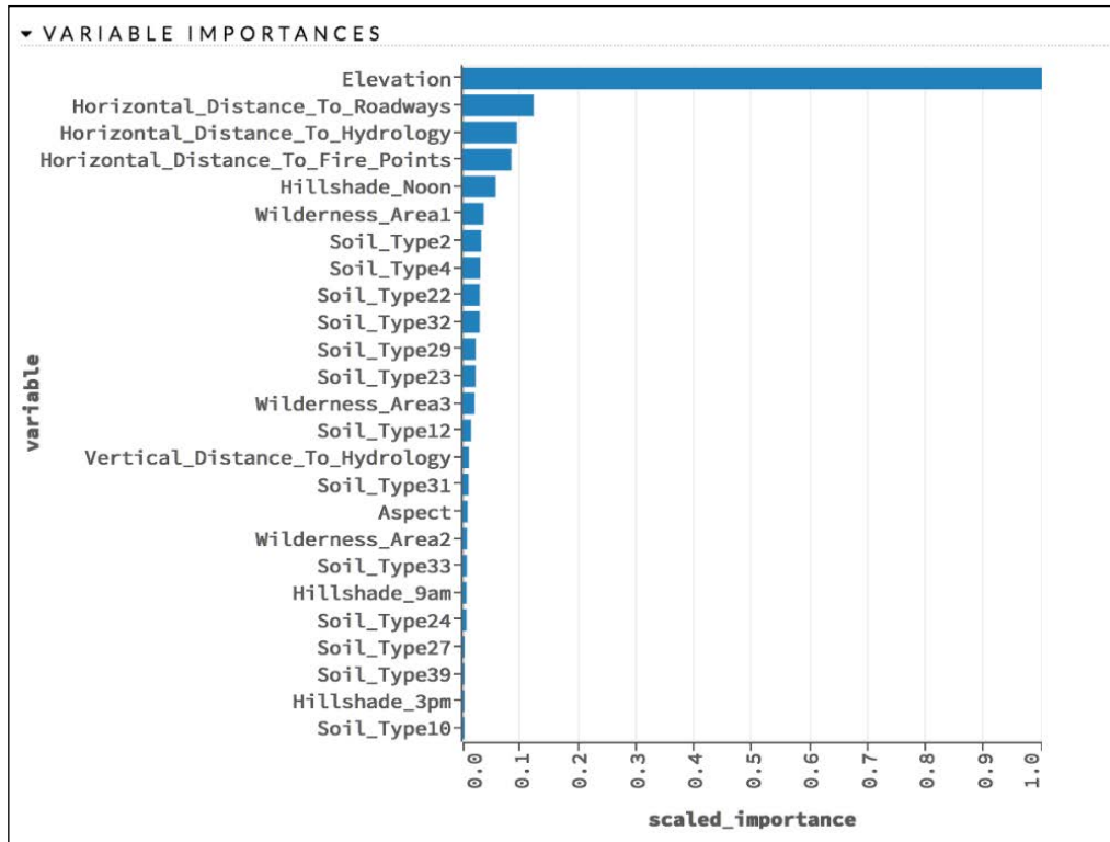
Figure 16: Feature selection using GLM
