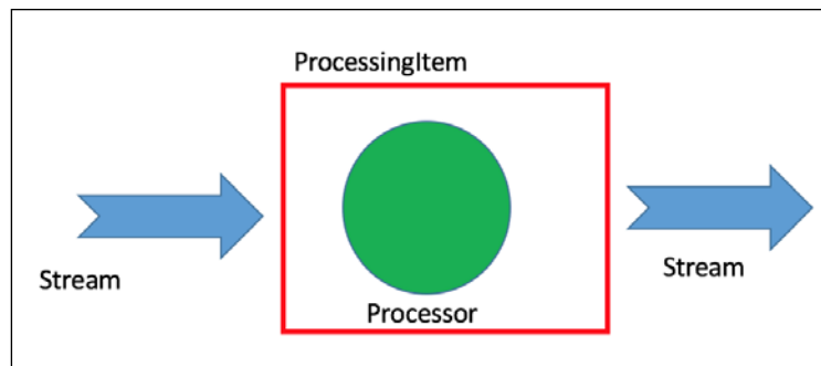
Figure 24: SAMOA processing data streams
