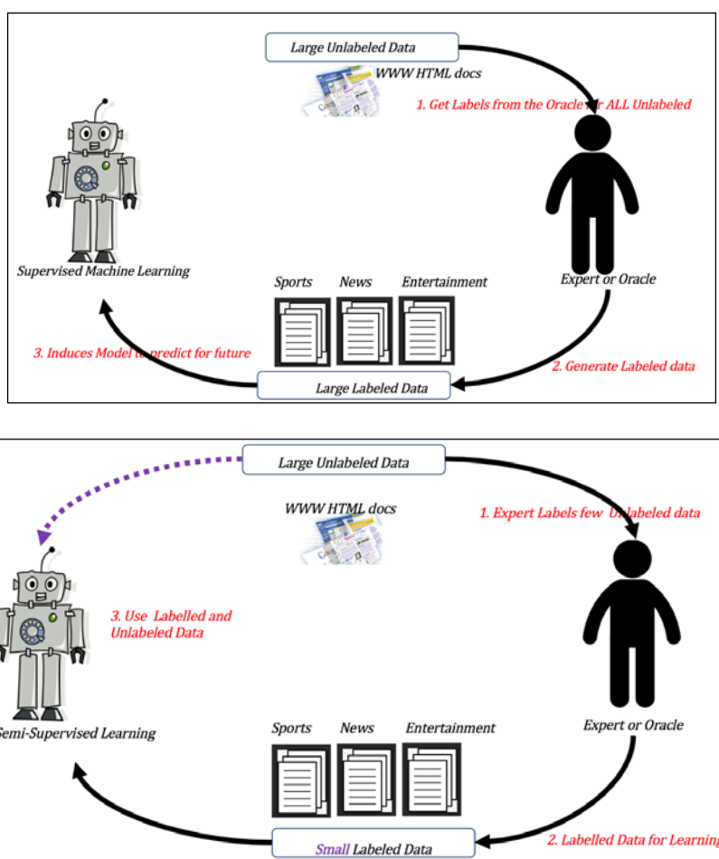
Figure 1. Semi-Supervised Learning process (bottom) contrasted with Supervised Learning (top) using classification of web documents as an example. The main difference is the amount of labeled data available for learning, highlighted by the qualifier "small" in the semi-supervised case.
