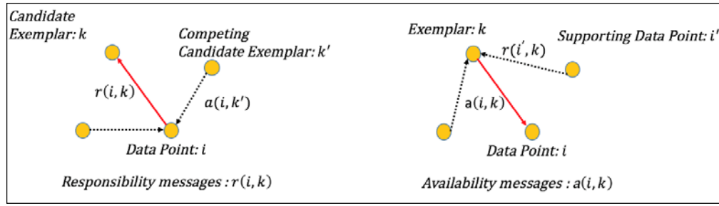
Figure 4: Message types used in Affinity Propagation
