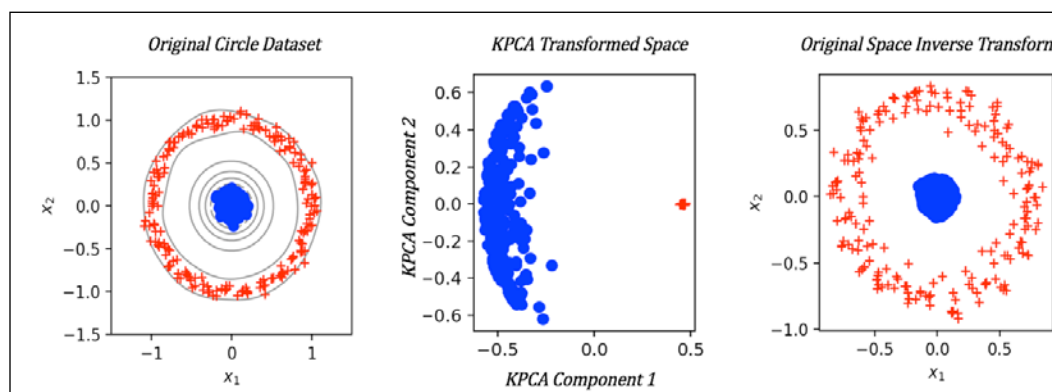
Figure 2: KPCA on Circle Dataset and Inverse Transform.
