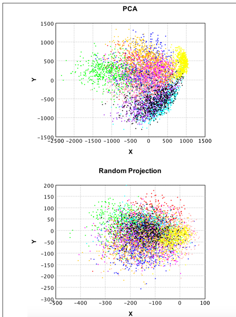
Figure 10: PCA and Random projection - representations in two dimensions using Smile API
