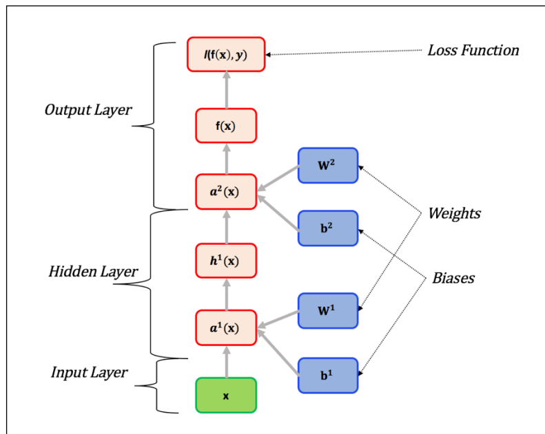
Figure 3: Neural network flow as a graph in feed forward.
