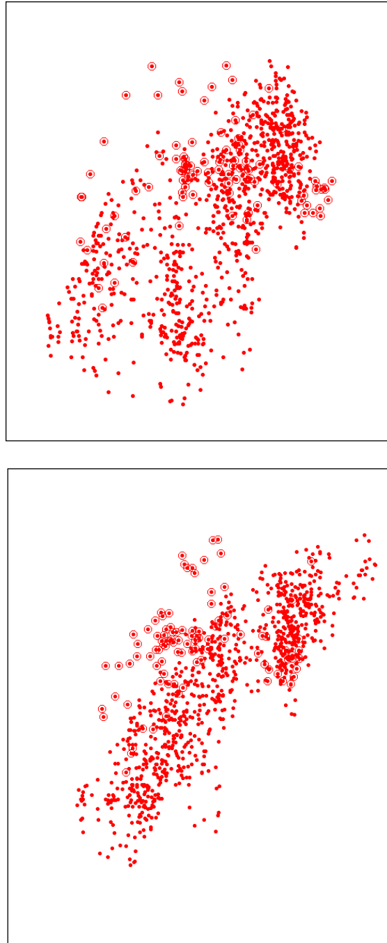
Figure 6. Outlier detection using Abstract-C, for three pairs of features, after processing all 45,300 instances
