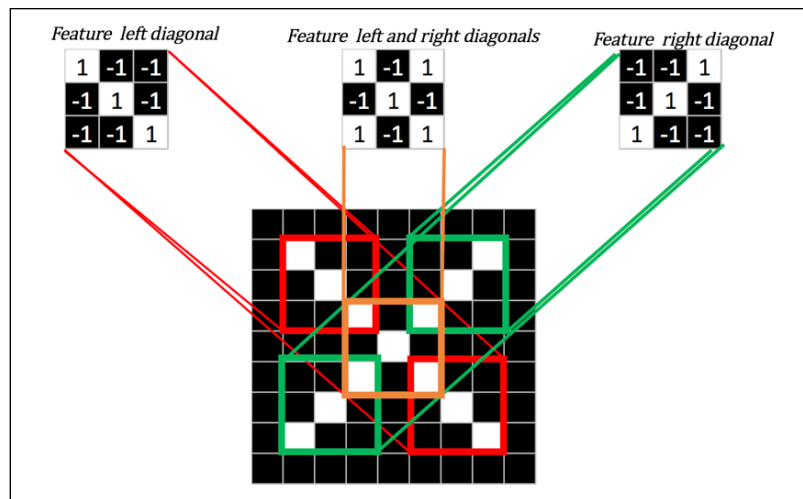
Figure 18: Common features represented in the image of character X.
