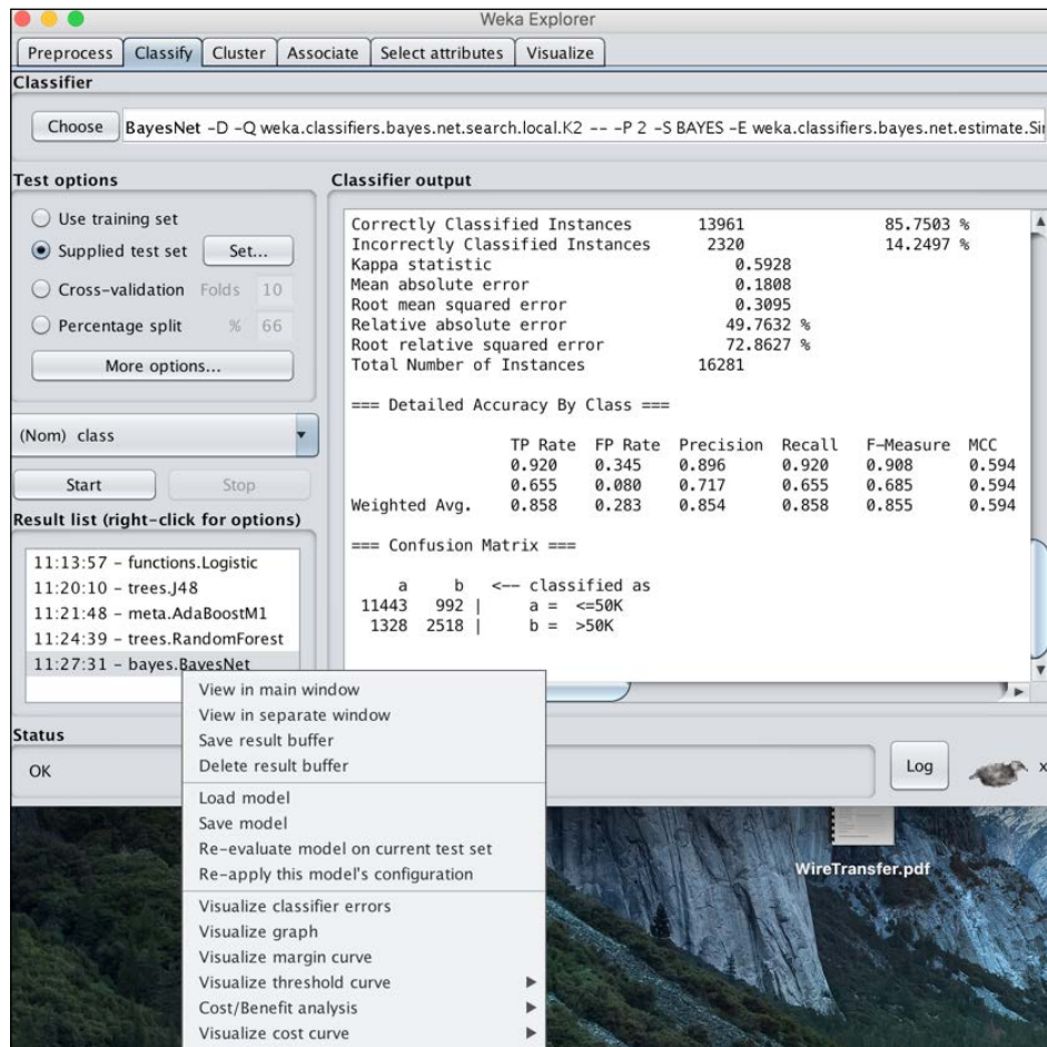
Figure 26. Weka Explorer – visualization menu
