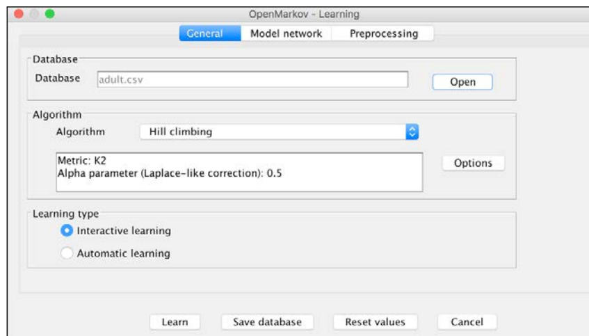
Figure 20. OpenMarkov GUI - Interactive learning, algorithm selection
