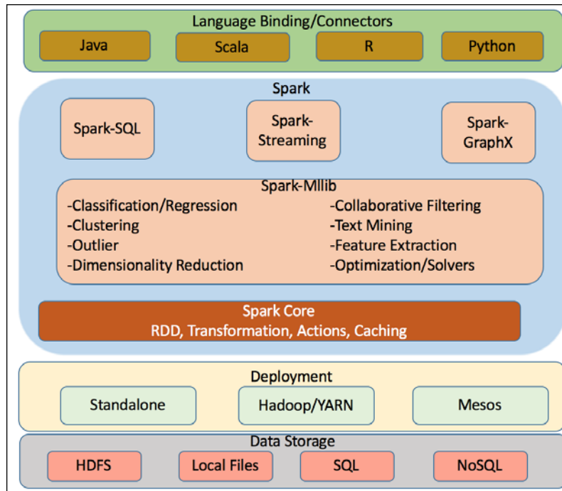
Figure 17: Apache Spark high level architecture
