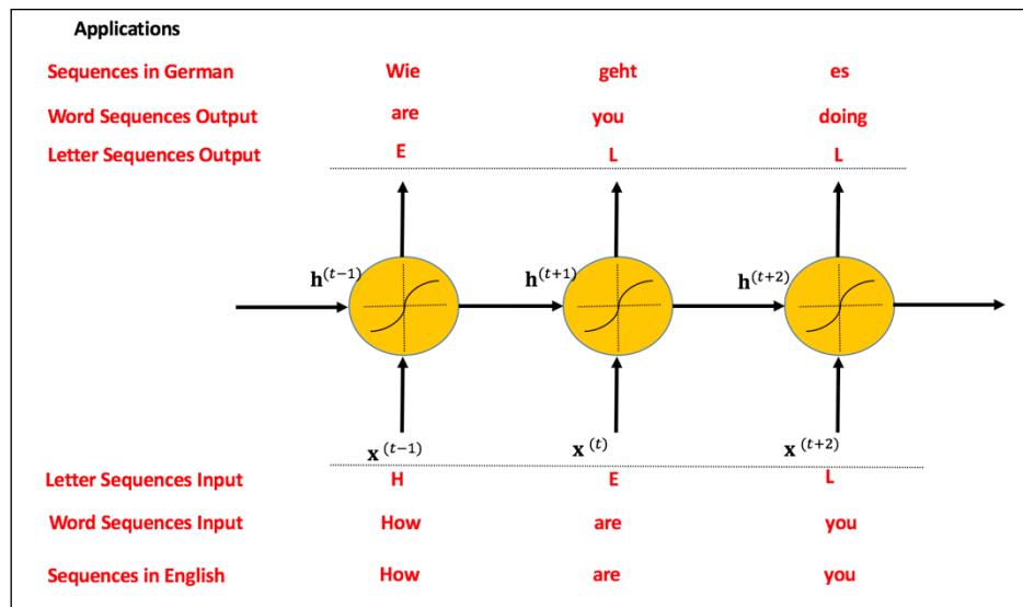
Figure 35: Showing some applications in next letter/word predictions using RNN structures.
