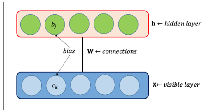
Figure 6: Connection between the visible layer and hidden layer.
