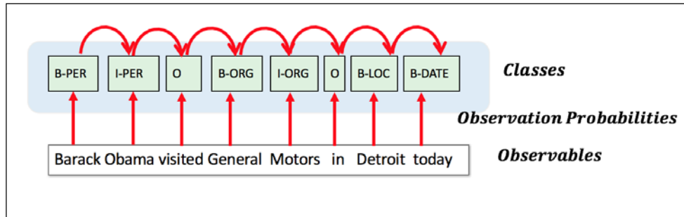
Figure 18 : Text Sequences and observation probabilities with labels
