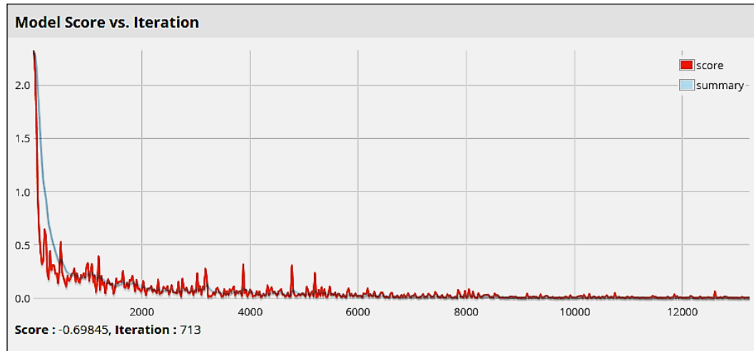
Figure 41: Training error as measured with number of iterations of training for the MLP model.
