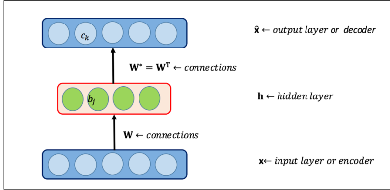
Figure 9: Autoencoder flow between layers
