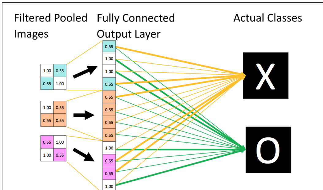
Figure 29: Fully connected layer as output of CNN.
