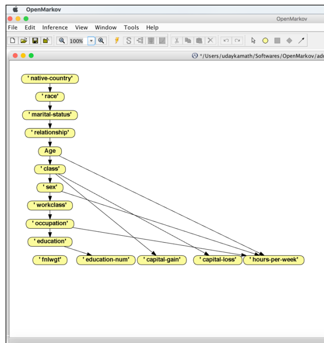
Figure 22. OpenMarkov GUI - Structure output
