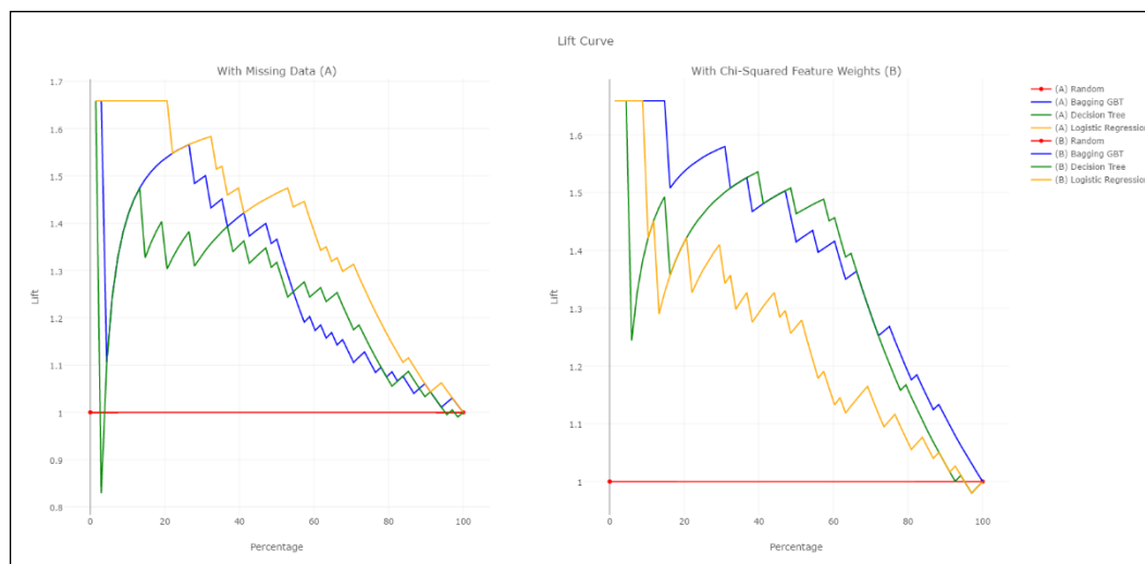
Figure 21: Lift performance curves for experiment using Missing Data
