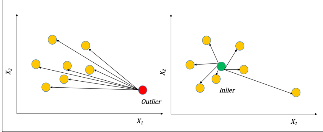
Figure 6: The ABOD method of distinguishing outliers from inliers
