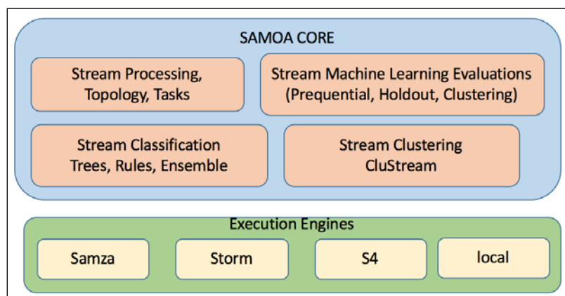
Figure 23: SAMOA high level architecture
