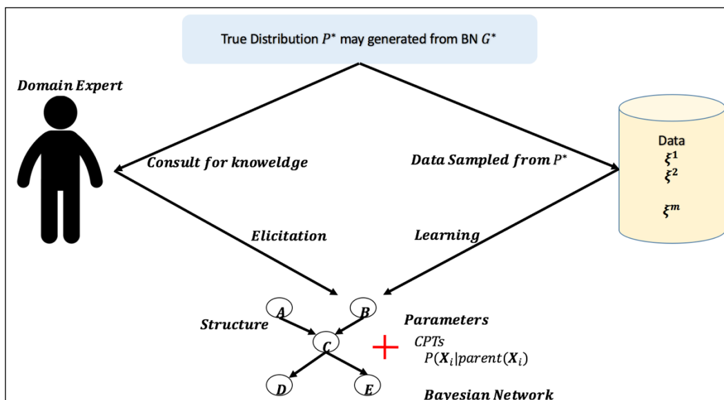
Figure 12. Elements of learning with Bayesian networks
