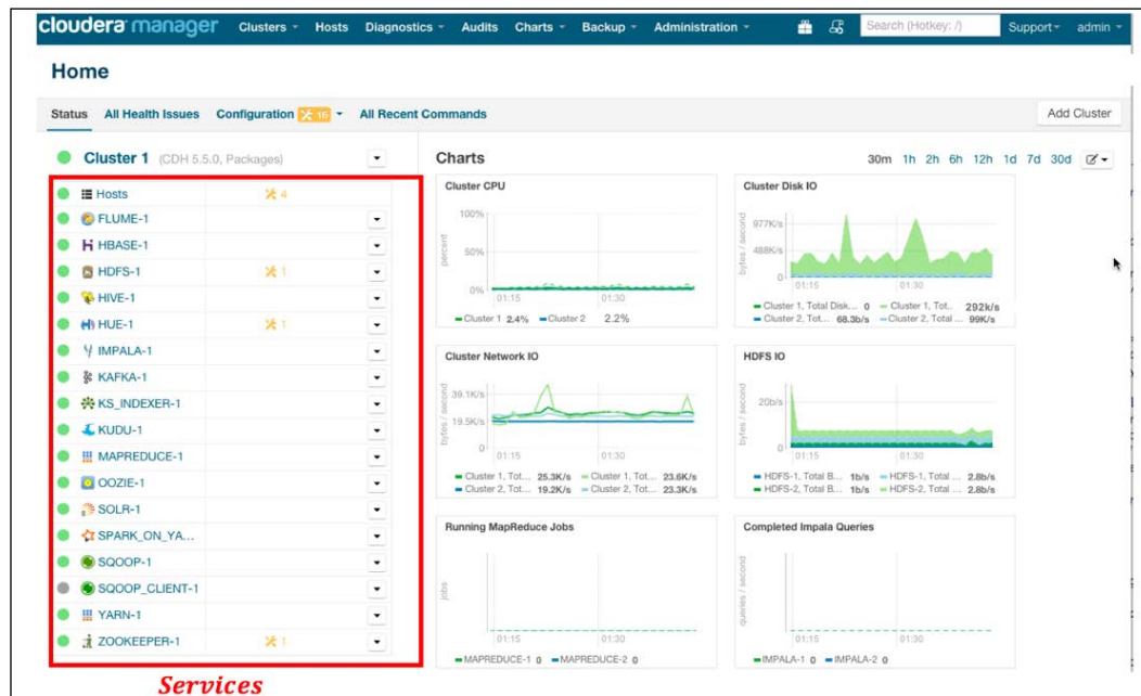
Figure 3: Cloudera Service Manager user interface
