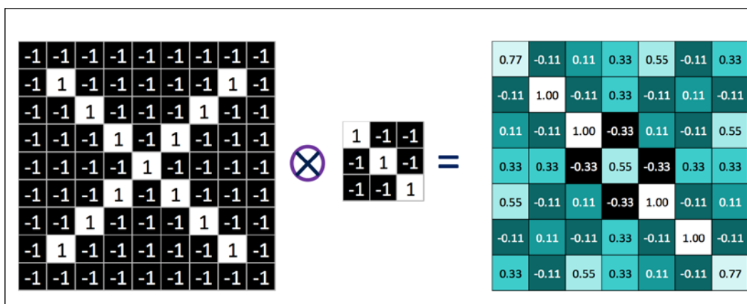
Figure 22: Transformation of the character image after a kernel and convolution operator.
