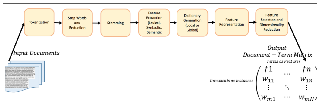
Figure 10: Text Processing components and the flow
