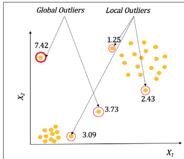
Figure 5: Density-based outlier detection methods are particularly suited for finding local as well as global outliers
