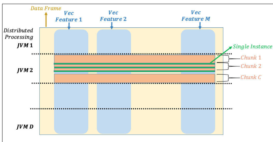
Figure 8: H2O distributed data processing using chunking
