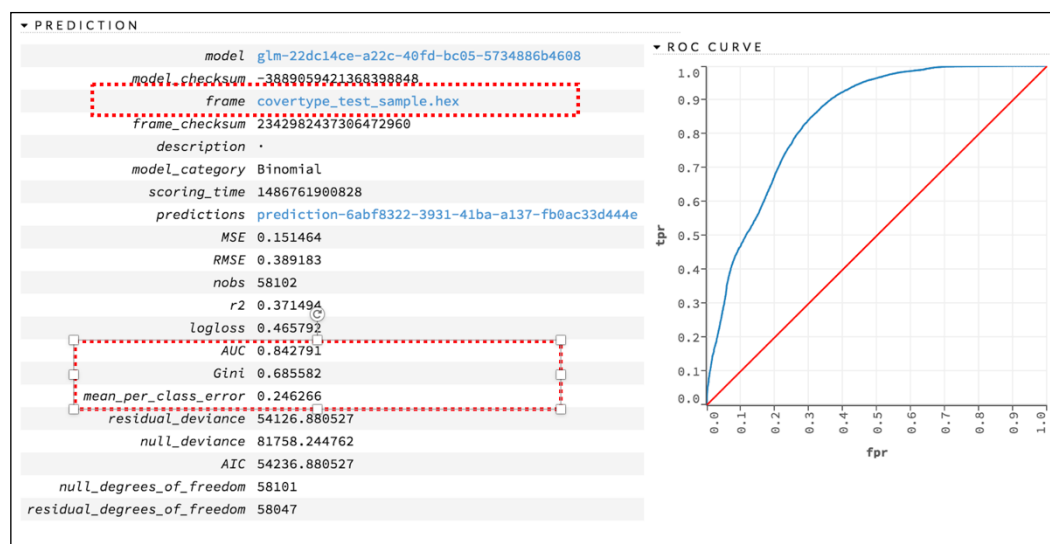
Figure 15: Running test data, predictions, and ROC curves
