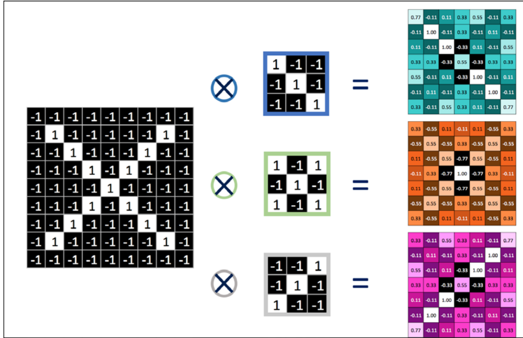
Figure 23: Different features run through the kernel giving a stack of images.
