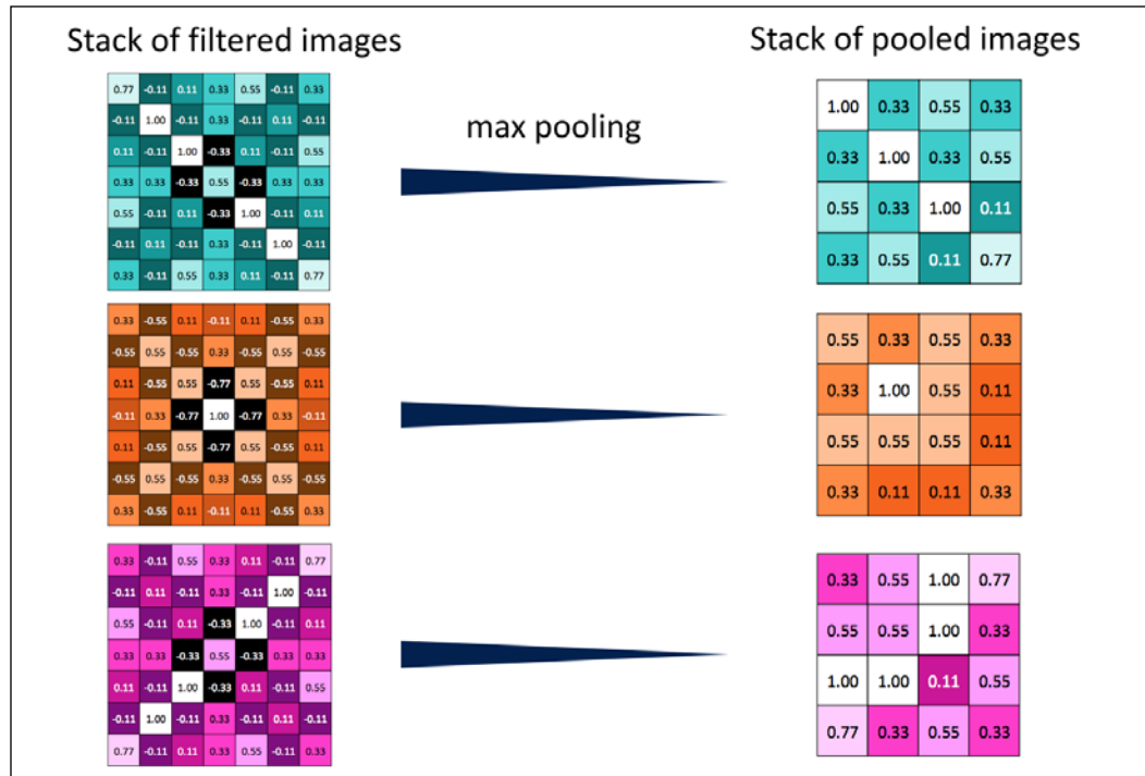
Figure 25: Transformation showing how a stack of filtered images is converted to pooled images.
