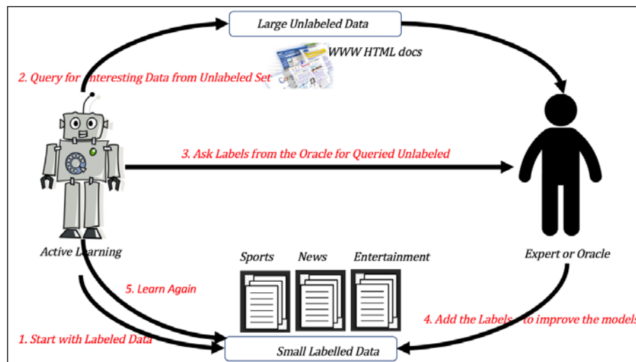
Figure 7. Active Machine Learning process contrasted with Supervised and Semi-Supervised Learning process.
