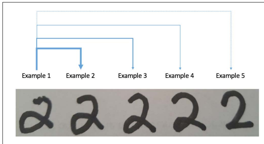
Figure 4. Transductive graph label propagation – classification of hand-written digits. Leftmost and rightmost images are labeled, others are unlabeled. Arrow thickness is a visual measure of similarity to labeled digit "2" on the left.
