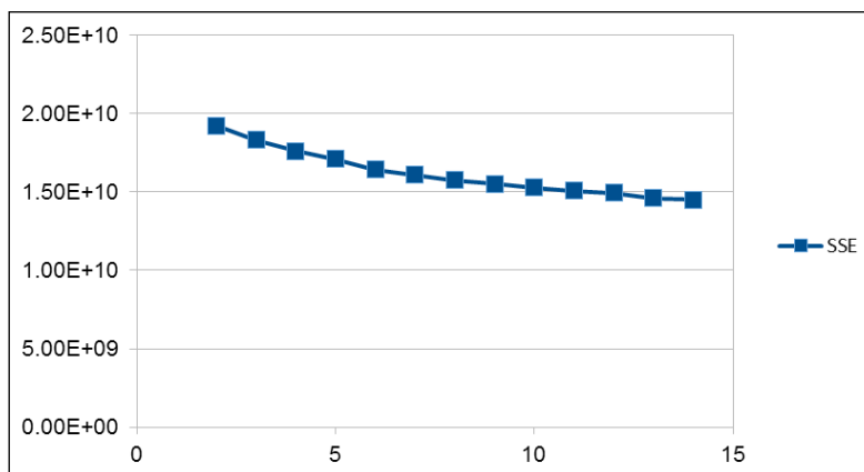
Figure 12: K-Means – using Sum of Squared Errors (SSE) to find optimal k , the number of clusters. An elbow in the curve, which is typically used to pick the optimal k value, is not particularly detectable in the plot.
