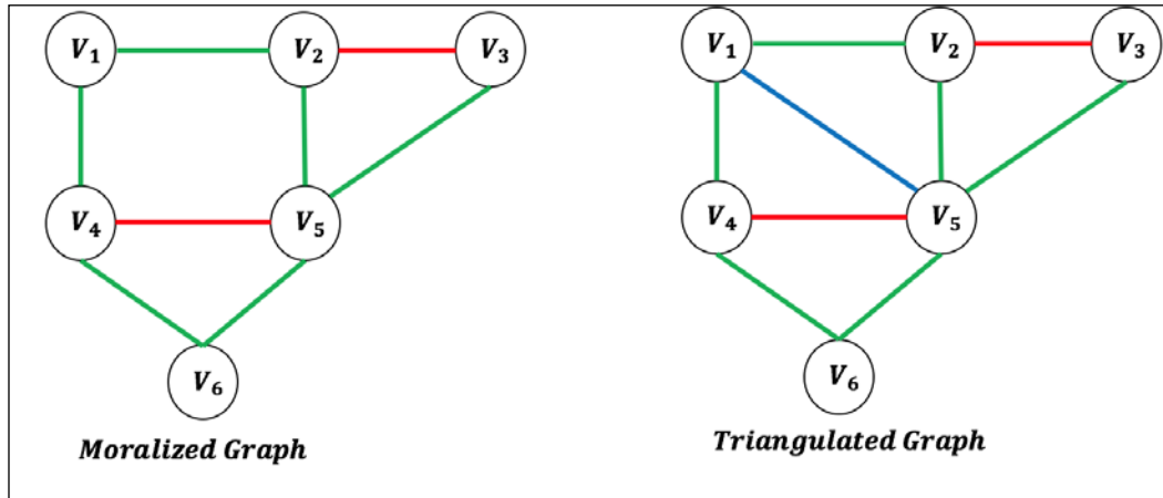
Figure 6. Graph triangulation with blue edge addition to convert a moralized graph to a chordal graph.
