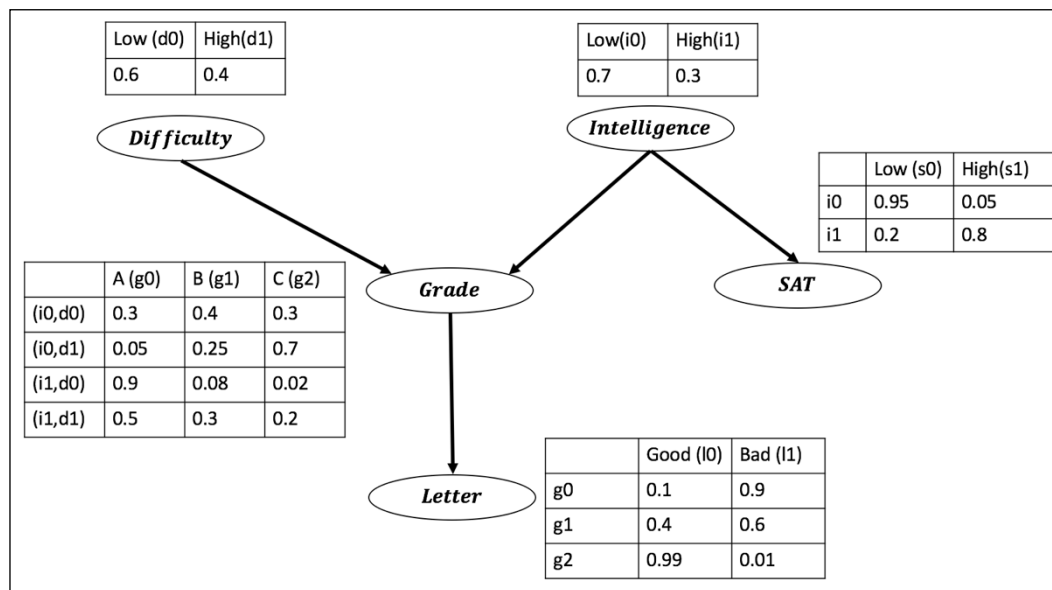
Figure 2. The "Student" network
