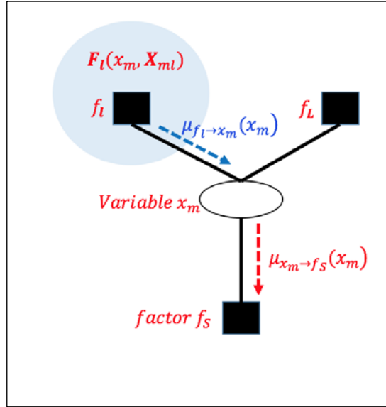
Figure 11. Message-passing from variable node to factor node
