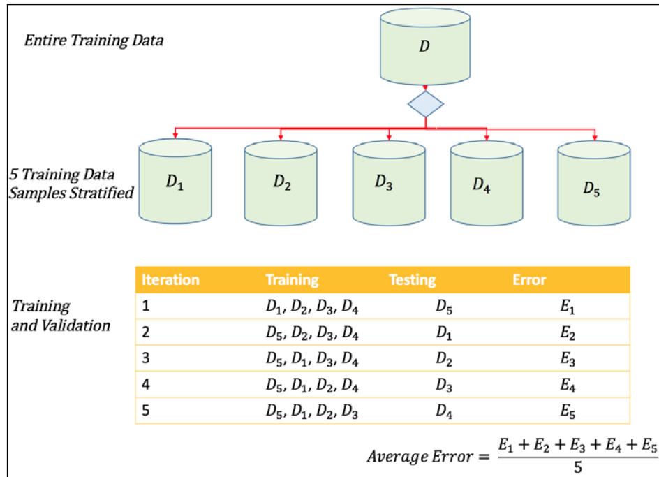
Figure 4: 5-fold cross-validation.
