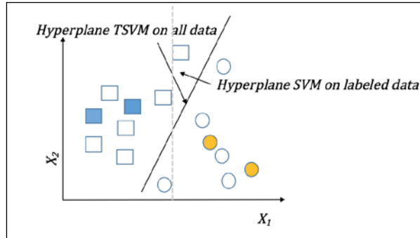
Figure 5. Transductive SVM
