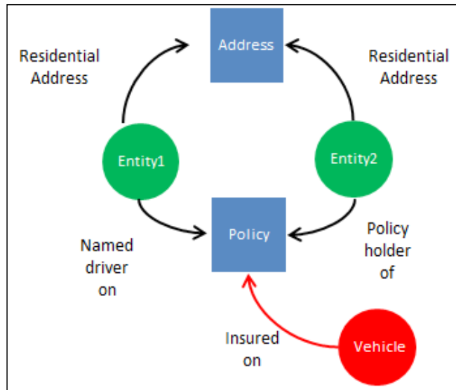
Insurance claim data, converted into a graph structure showing the relationship between vehicles, drivers, policies, and addresses
