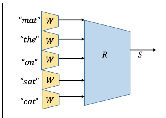
Figure 19: A modular neural network learning 5-gram words for valid-invalid classification
