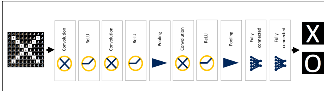
Figure 30: CNNs with all layers showing inputs and outputs.
