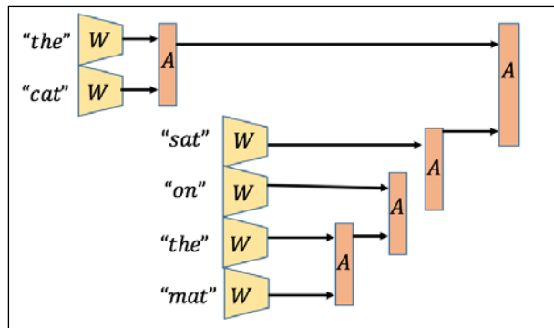
Figure 21: Recursive Neural Network showing how complex phrases can be learned.
