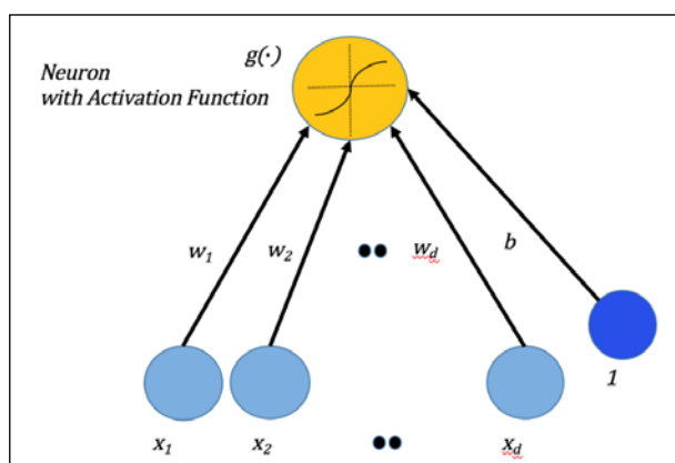
Figure 1. Perceptron with inputs, weights, and bias feeding to generate outputs.
