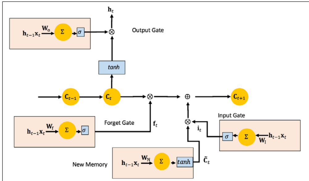
Figure 39: Building blocks New Gate and Input Gate added to complete LSTM.
