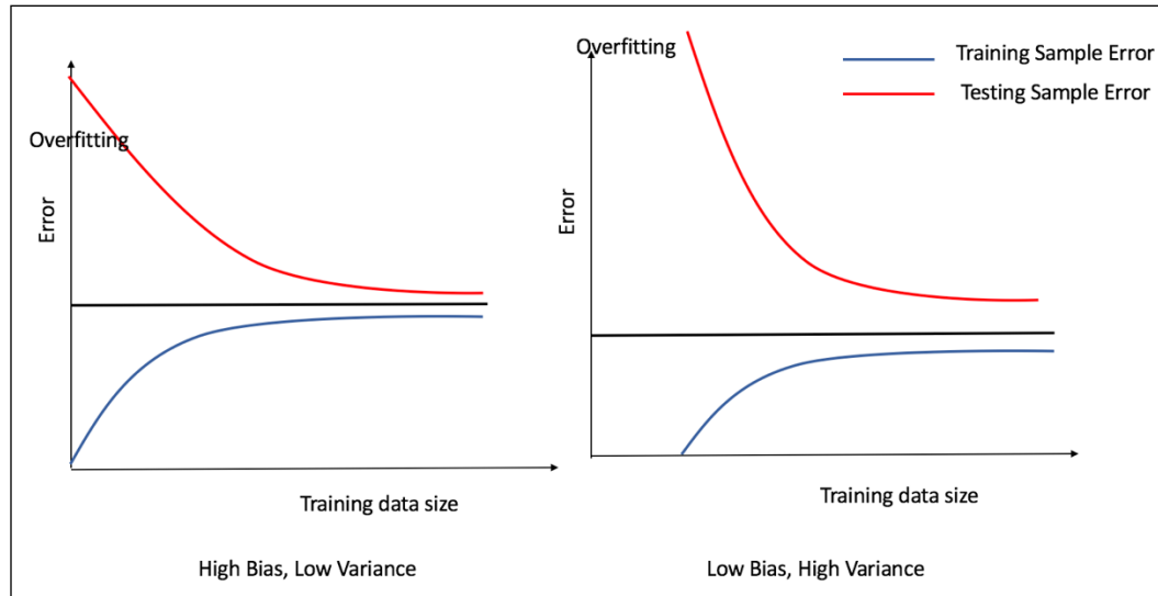
Figure 2: The training data relationship with error rate when the model complexity is fixed indicates different choices of models.
