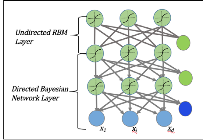
Figure 15: Deep belief network
