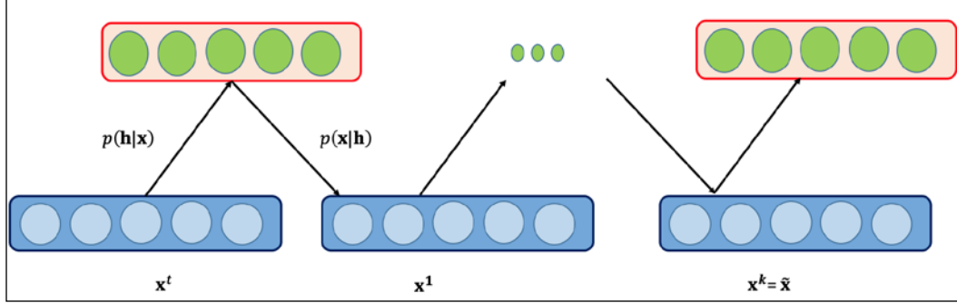
Figure 8: Graphical representation of sampling done between hidden and input layers.
