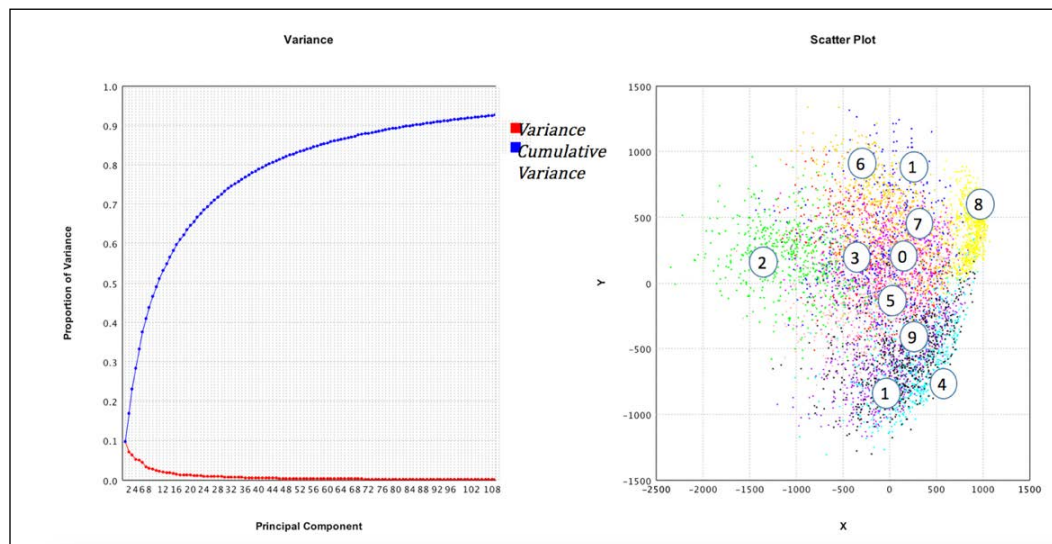
Figure 9: PCA on MNIST – On the left, we see that over 90 percent of variance in data is accounted for by fewer than half the original number of features; on the right, a representation of the data using the first two principal components.
