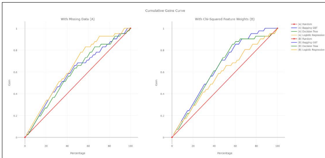
Figure 20: Cumulative Gains performance curves for experiment using Missing Data
