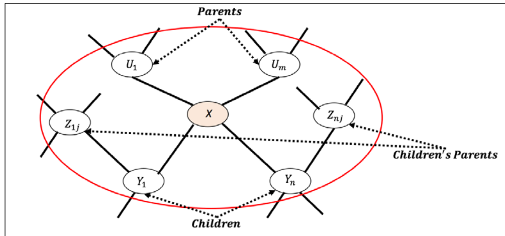
Figure 15. Markov blanket for Node X - its Parents, Children, and Children's Parents.
