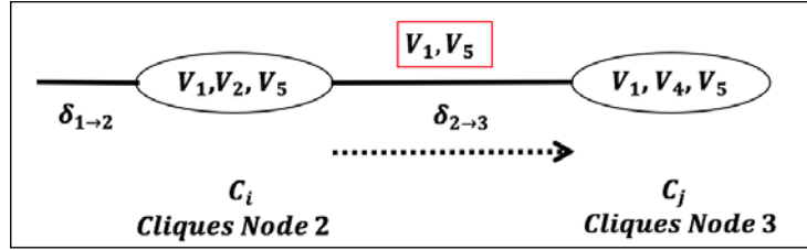
Figure 8. Message passing between nodes/cliques in Junction Tree
