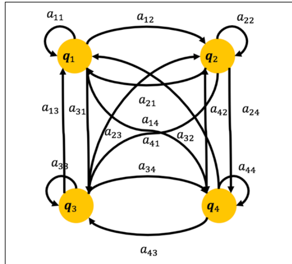
Figure 18. First-order Markov chain
