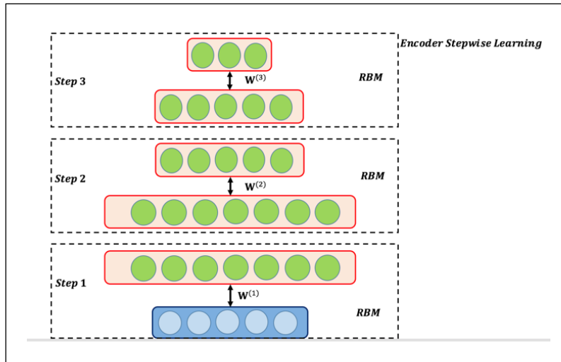
Figure 14: Stepwise learning in RBM
