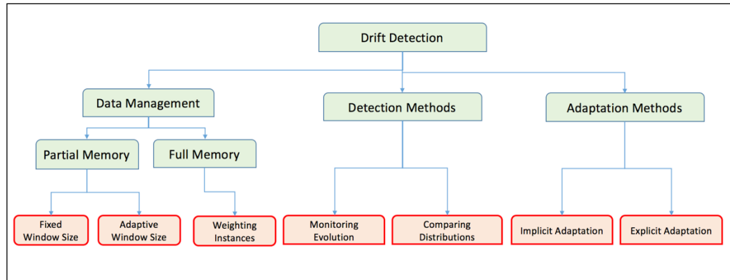
Figure 2 Categories of drift detection techniques
