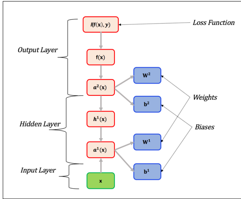
Figure 4: Neural network flow as a graph in back propagation.
