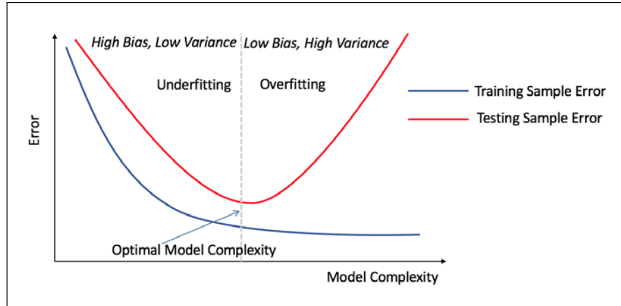
Figure 3: The Model Complexity relationship with Error rate, over the training and the testing data when training data size is fixed.
