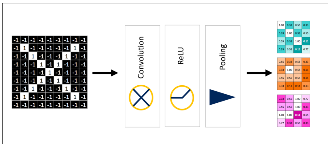
Figure 27: Basic Unit of CNN showing a combination of Convolution, ReLu, and Pooling.
