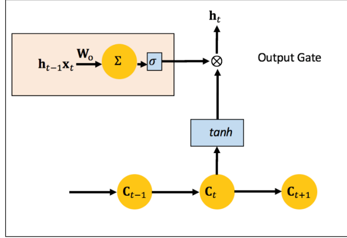
Figure 37: Building block Output Gate for LSTM.
