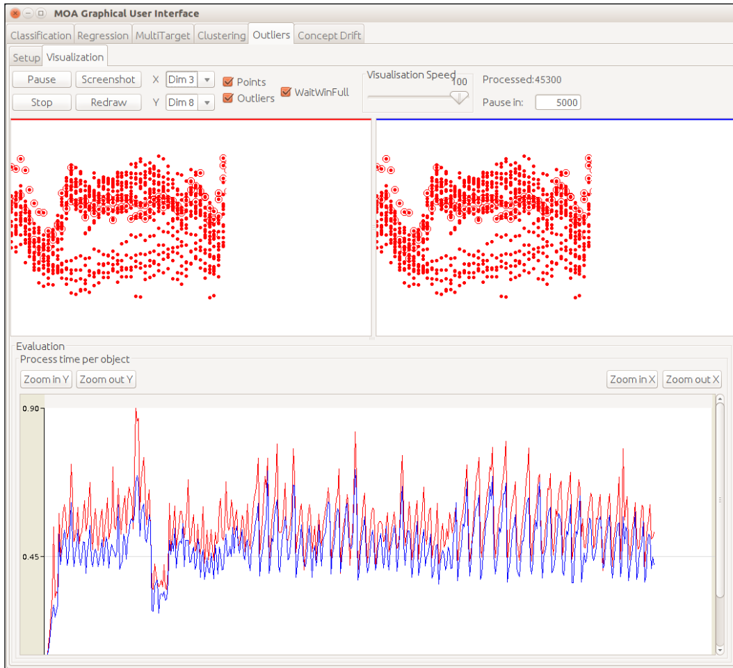
Figure 7. Visualization of outlier detection in MOA
