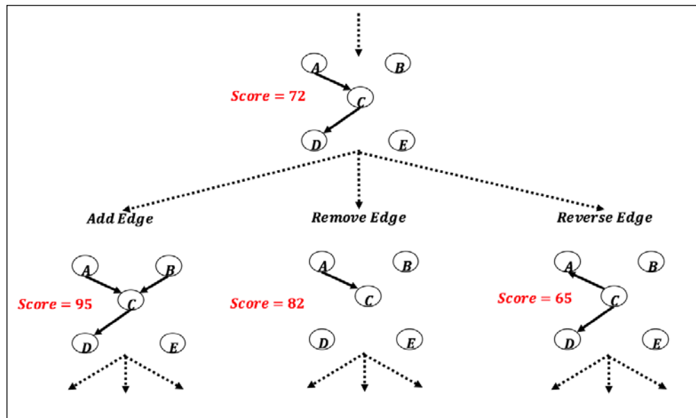
Figure 14. Search and Score
