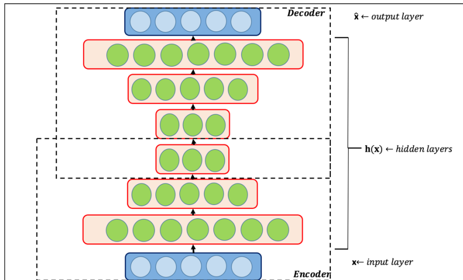
Figure 13: Deep Autoencoders
