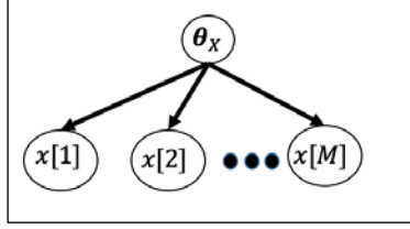
Figure 13. Single variable parameter learning
