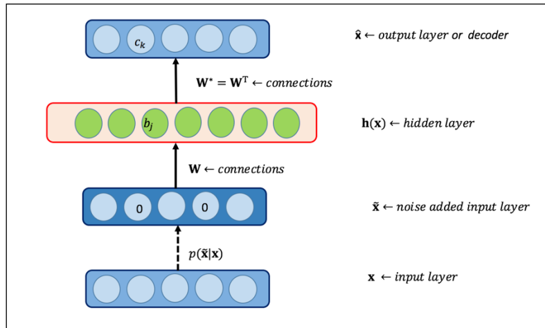
Figure 10: Denoising Autoencoder
