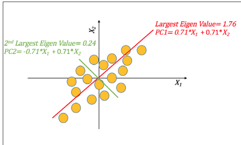
Figure 1: Principal Component Analysis
