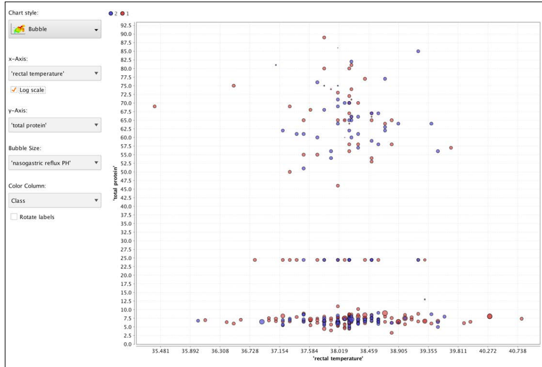
Figure 17: Bubble chart
