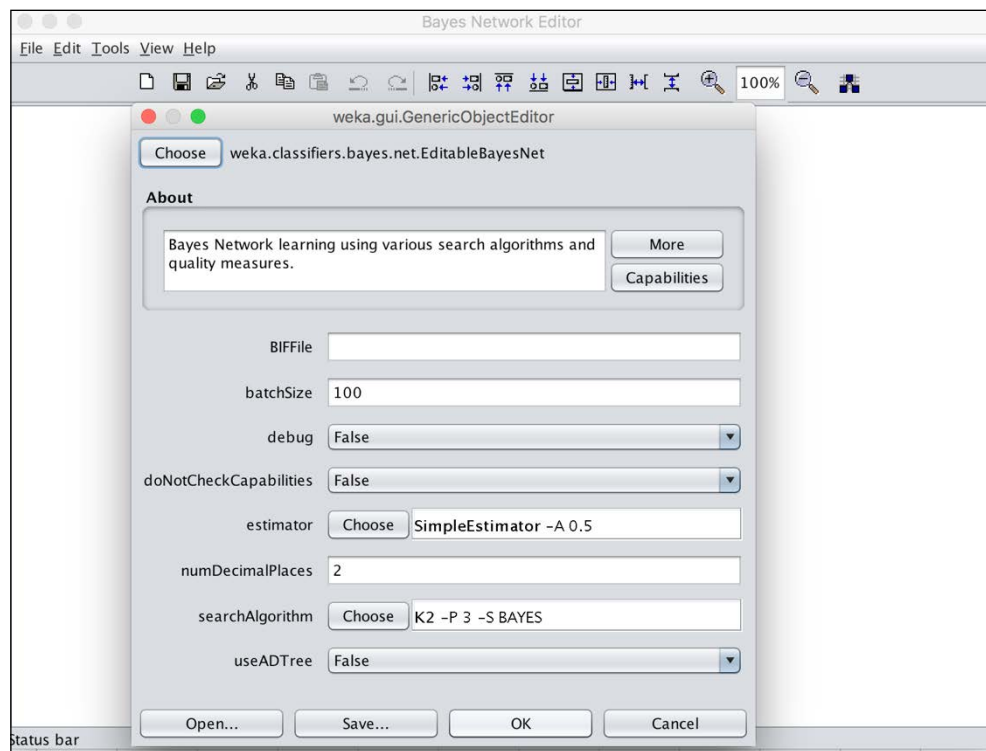
Figure 23. WEKA Bayes Network – configuring search algorithm
