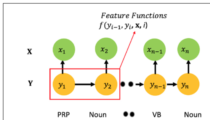
Figure 16: Conditional random fields mapped to the area of sequence prediction in the POS tagging domain.
