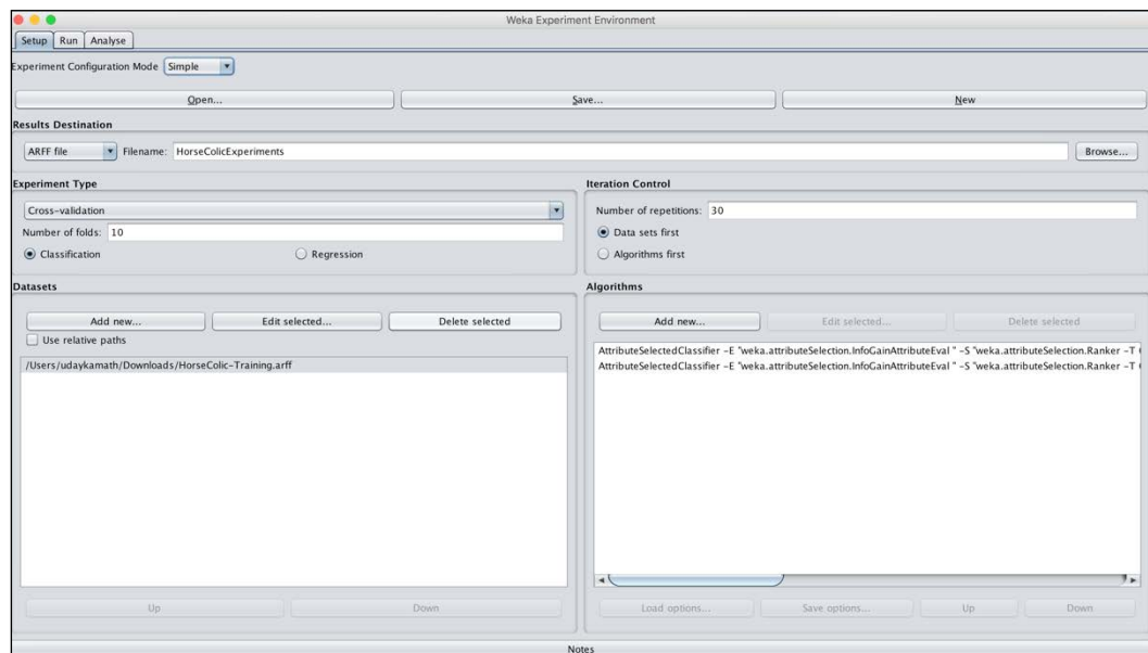
Figure 13: WEKA experimenter showing the process of using cross-validation runs with 30 repetitions with two algorithms.
