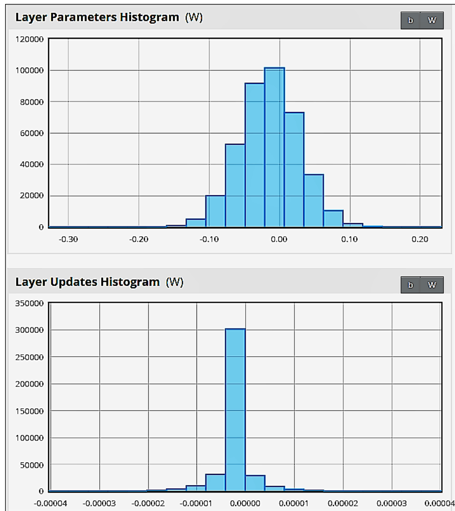
Figure 42: Histograms showing Layer parameters and update distribution.
