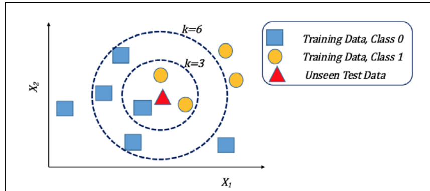
Figure 6: K-Nearest Neighbor illustrated using two-dimensional data with different choices of k.
