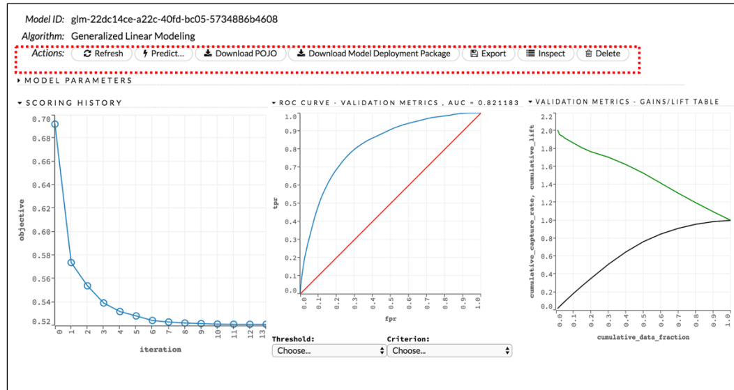
Figure 13: Modeling and validation ROC curves, objective functions, and lift/gain charts
