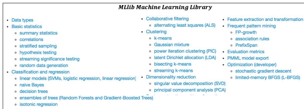
Figure 20: Apache Spark MLlib machine learning algorithms
