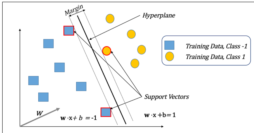
Figure 7: SVM Linear Hyperplane learned from training data that creates a maximum margin separation between two classes.
