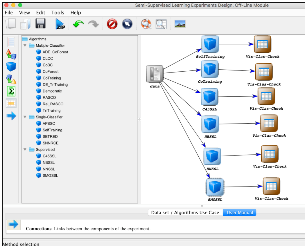
Figure 6: KEEL - wizard-based graphical interface
