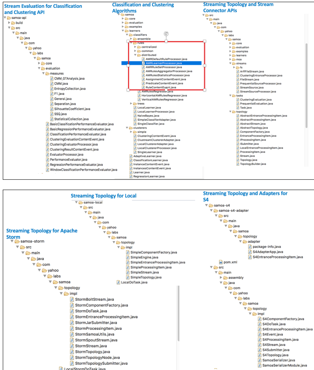
Figure 25: SAMOA machine learning algorithms
