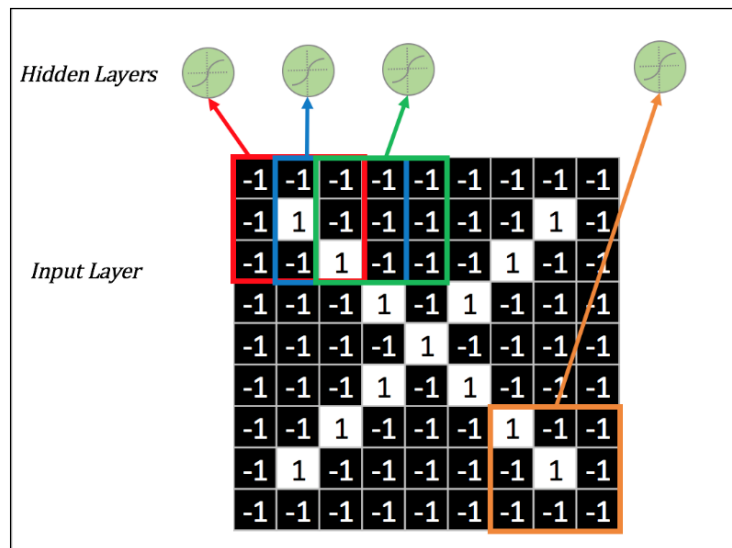
Figure 19: Concept of patches on the whole image.
