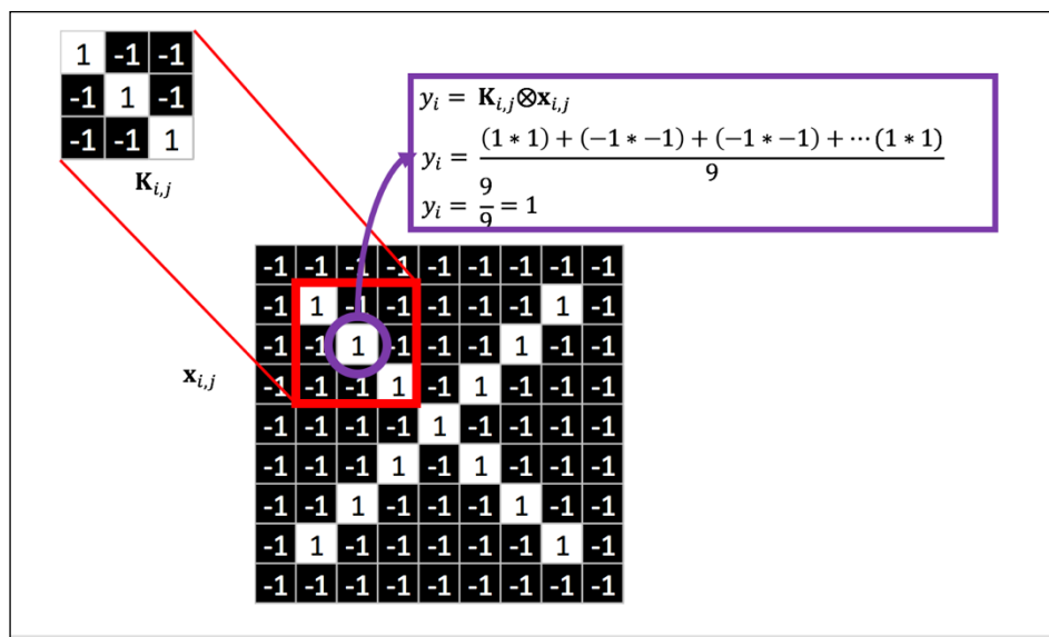
Figure 21: Discrete convolution step.
