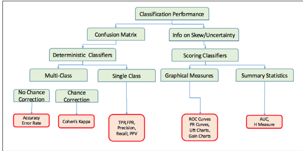
Figure 10: Model evaluation metrics for classification models
