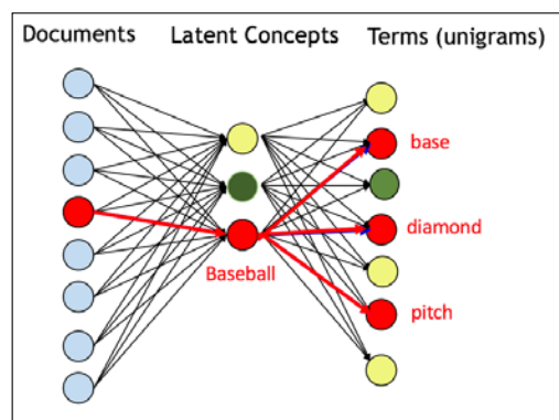
Figure 14: Latent concept of Baseball capturing the association between documents and related terms
