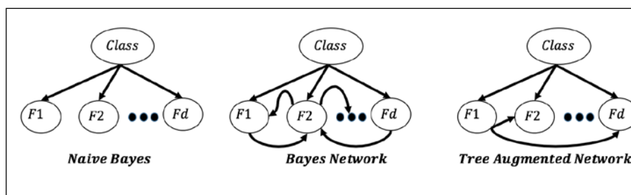
Figure 17. Tree augmented network showing comparison with Naïve Bayes and Bayes network and the constraint of one parent per node.
