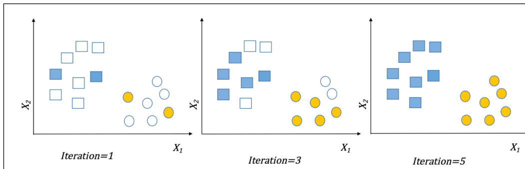
Figure 2. Self-training SSL in binary classification with some labeled data shown with blue rectangles and yellow circles. After various iterations, the unlabeled data gets mapped to the respective classes.
