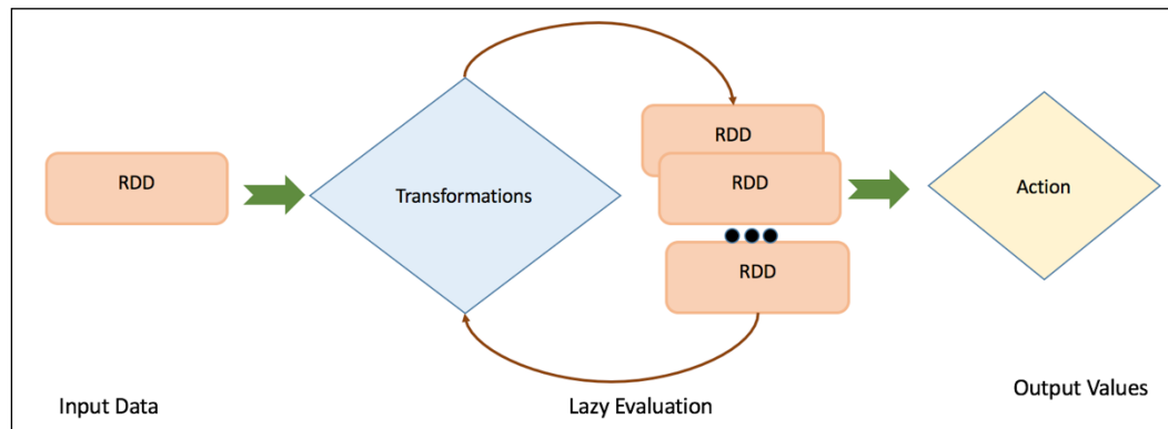
Figure 18: Apache Spark lineage graph
