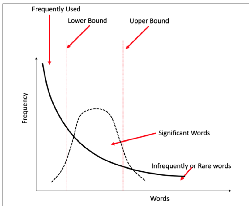
Figure 11: Word Frequency distribution, showing how frequently used, significant and rare words exist in corpus
