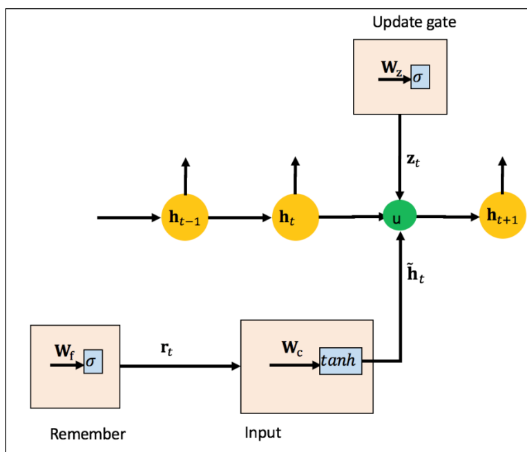
Figure 40: GRUs with Update unit.
