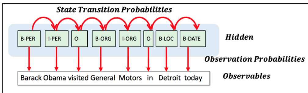
Figure 17: Text sequence and labels corresponding to NER in Hidden Markov Chain
