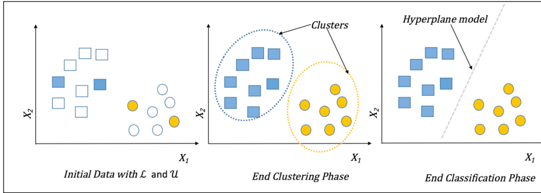
Figure 3. Clustering and label SSL – clustering followed by classification
