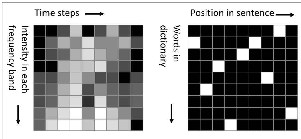
Figure 31: Illustration of mapping between temporal data, such as voice to spatial data, to an image.
