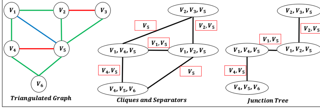
Figure 7. Formation of a Junction Tree
