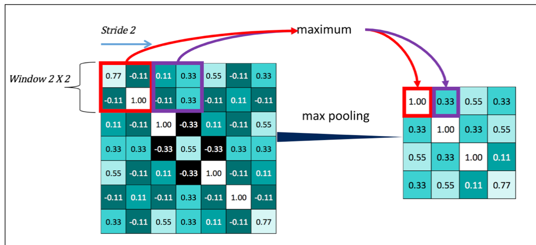
Figure 24: Max pooling, done using a window size of 2 X 2 and stride of 2, computes cell values with maximum for first as 1.0, 0.33 for next, and so on.
