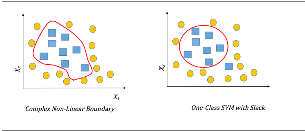
Figure 7: One-Class SVM for nonlinear boundaries
