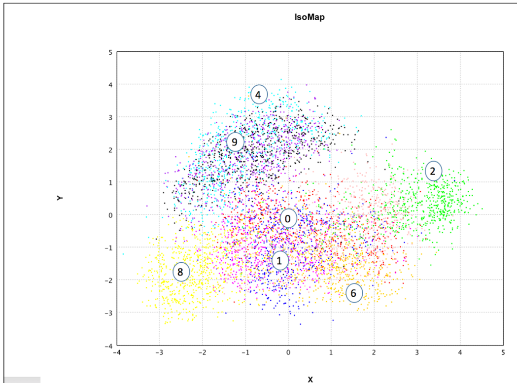
Figure 11: IsoMap – representation in two dimensions with k = 10 using Smile API
