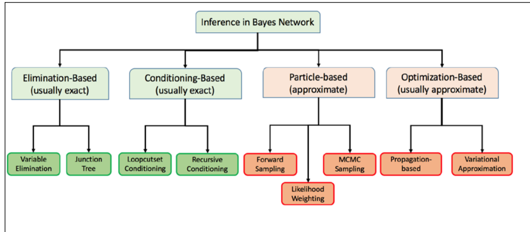
Figure 4. Exact and approximate inference techniques
