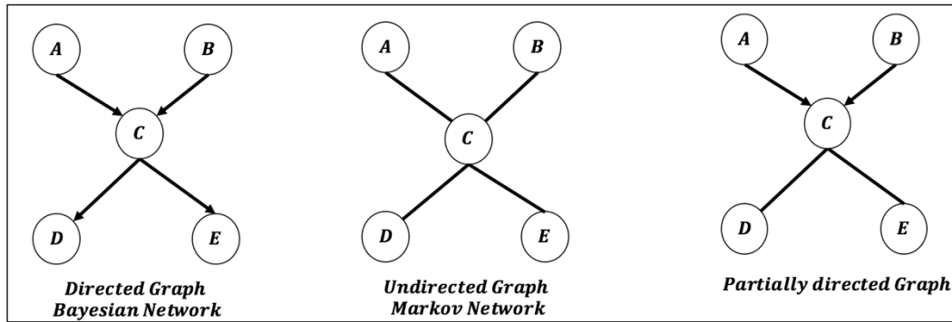
Figure 1. Directed, undirected, and partially-directed graphs
