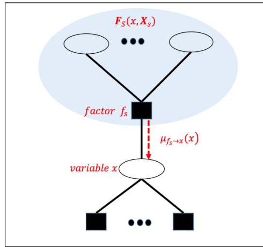
Figure 10. Message-passing from factor node to variable node
