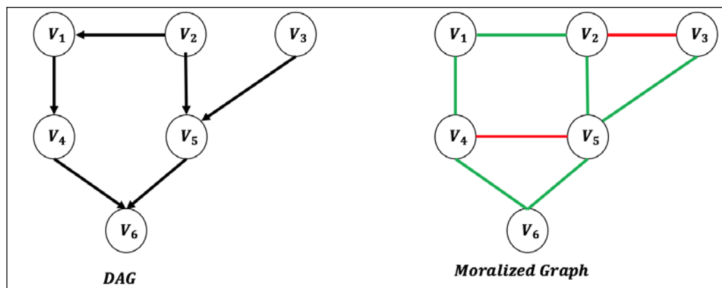
Figure 5. Graph moralization of DAG showing in green how the directional edges are changed and red edges showing new additions.
