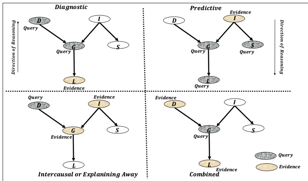
Figure 3. Reasoning patterns
