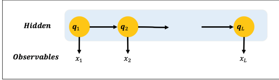
Figure 19. Hidden Markov model showing hidden variables and the observables.
