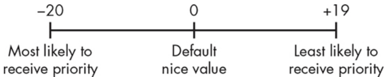
Figure 6-1: Niceness priority values
