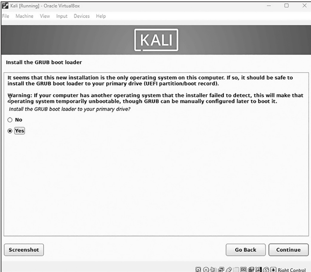
Figure 10: Installing GRUB
