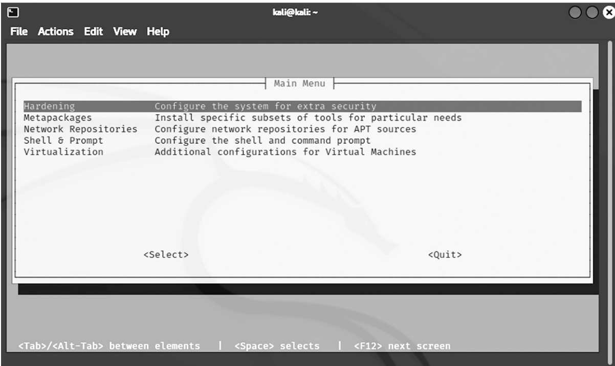
Figure 7-1: kali-tweaks
