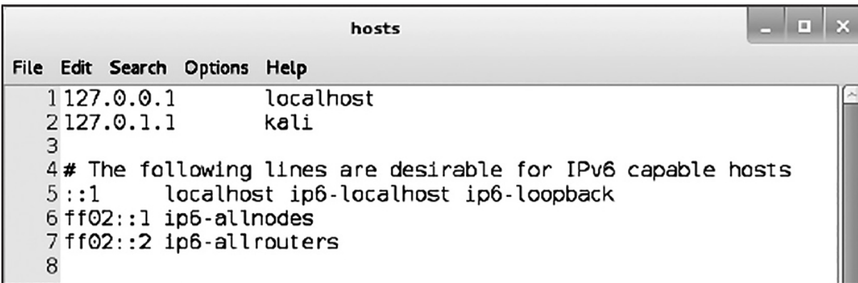
Figure 3-6: A default Kali hosts file
