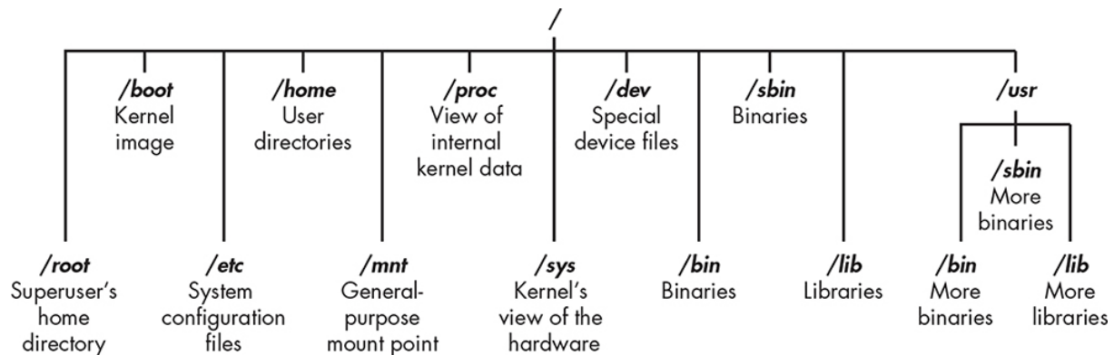
Figure 1-2: The Linux filesystem
