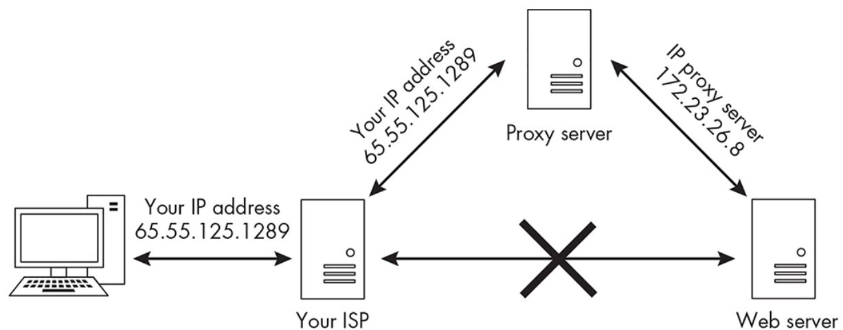
Figure 13-4: Running traffic through a proxy server
